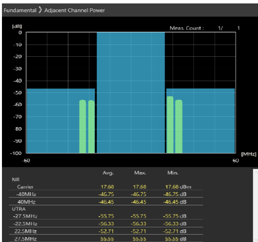
40MHz_30kHz_3680MHz-OFDM QPSK_RB1@105 -46.75,-46.45dB
