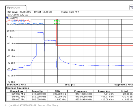
Band 5 3MHz/842.6/High QPSK 15@0 Band 5 5MHz/846.5/High QPSK 25@0
