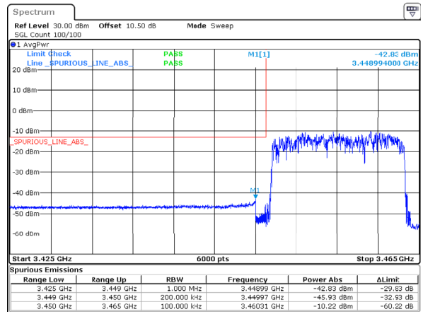
n77_1_15MHz_30kHz_3457.5MHz_DFT-s-OFDM QPSK_RB36@0
