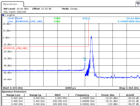
n77_1_15MHz_30kHz_3457.5MHz_DFT-s-OFDM QPSK_RB1@0
