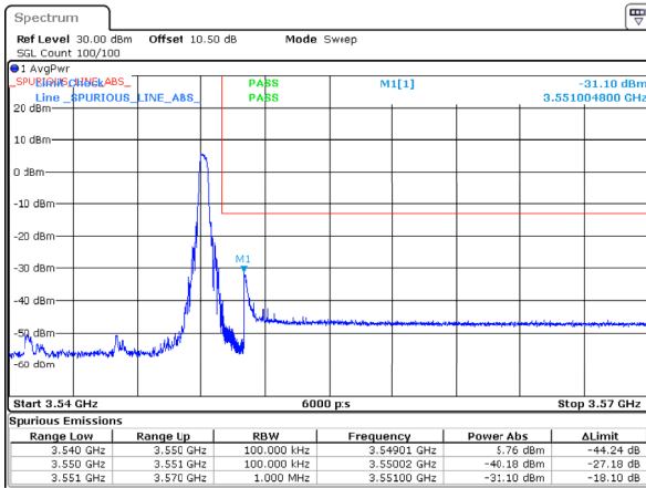
n77_1_10MHz_30kHz_3545MHz_DFT-s-OFDM QPSK_RB1@23
