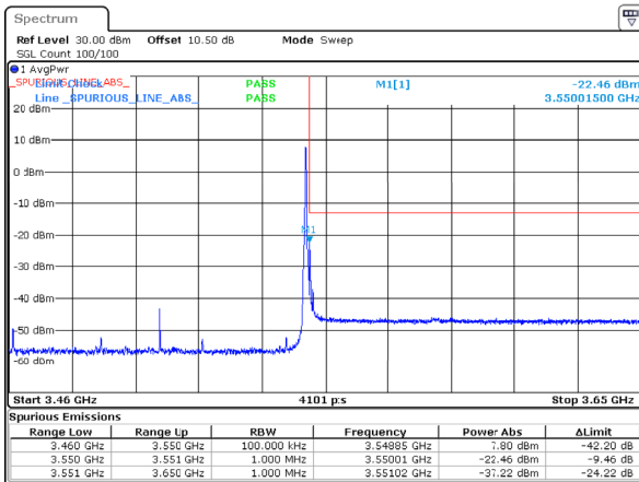
n77_1_90MHz_30kHz_3505MHz_DFT-s-OFDM QPSK_RB1@244
