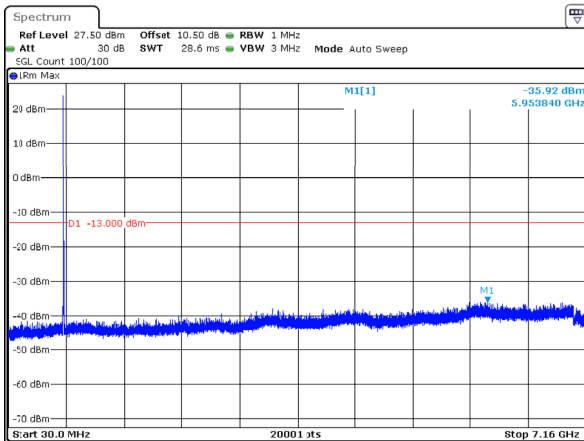
n12_5MHz_15kHz_707.5MHz_DFT-s-OFDM QPSK_RB1@24 -35.92dBm
