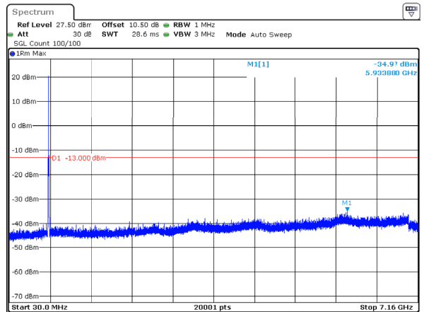
n12_5MHz_15kHz_707.5MHz_DFT-s-OFDM QPSK_RB25@0 -34.97dBm
