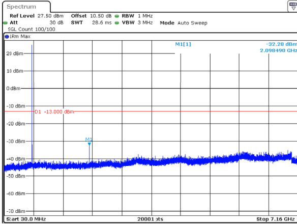
n12_5MHz_15kHz_701.5MHz_DFT-s-OFDM QPSK_RB1@0 -32.28dBm
