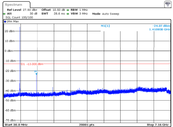
n12_5MHz_15kHz_707.5MHz_DFT-s-OFDM QPSK_RB1@0 -24.02dBm
