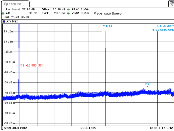
n12_10MHz_15kHz_704MHz_DFT-s-OFDM QPSK_RB1@51 -34.78dBm
