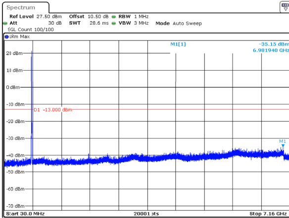
n12_5MHz_15kHz_713.5MHz_DFT-s-OFDM QPSK_RB25@0 -35.15dBm
