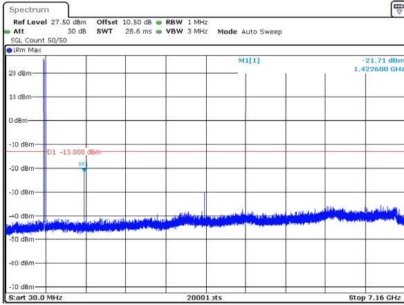
n12_5MHz_15kHz_713.5MHz_DFT-s-OFDM QPSK_RB1@0 -21.71dBm
