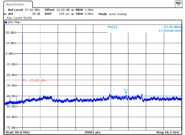
n38_5MHz_15kHz_2617.5MHz_DFT-s-OFDM QPSK_RB1@24 -37.45dBm
