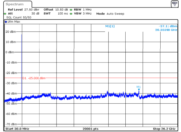
n38_40MHz_30kHz_2600MHz_DFT-s-OFDM QPSK_RB1@0 -37.11dBm
