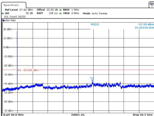
n38_10MHz_30kHz_2575MHz_DFT-s-OFDM QPSK_RB1@23 -37.33dBm
