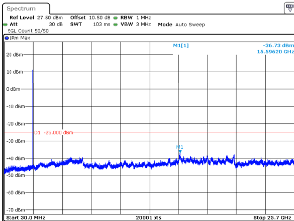
n7_5MHz_15kHz_2535MHz_DFT-s-OFDM QPSK_RB1@24 -36.73dBm
