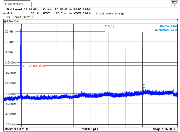
n12_5MHz_15kHz_701.5MHz_DFT-s-OFDM QPSK_RB1@24 -35.25dBm
