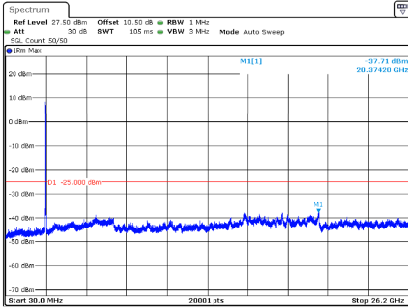
n38_40MHz_30kHz_2600MHz_DFT-s-OFDM QPSK_RB100@0 -37.71dBm
