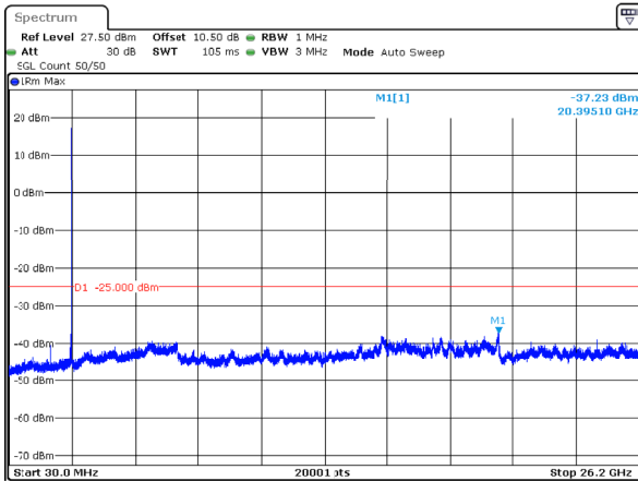
n38_40MHz_30kHz_2600MHz_DFT-s-OFDM QPSK_RB1@105 -37.23dBm
