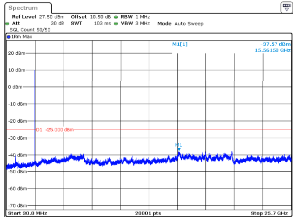
n7_5MHz_15kHz_2535MHz_DFT-s-OFDM QPSK_RB1@0 -37.57dBm
