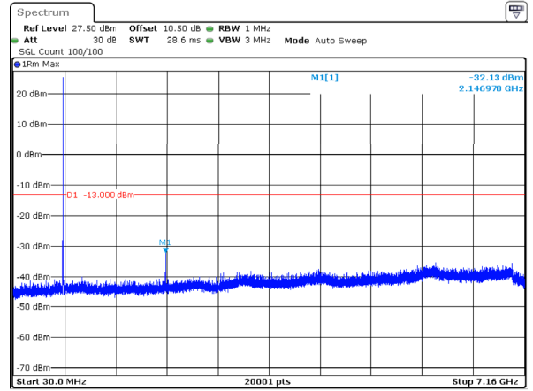
n12_5MHz_15kHz_713.5MHz_DFT-s-OFDM QPSK_RB1@24 -32.13dBm
