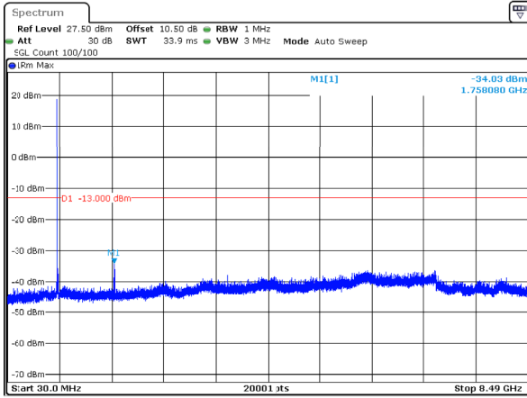
n5_15MHz_15kHz_841.5MHz_DFT-s-OFDM QPSK_RB1@0 -34.03dBm
