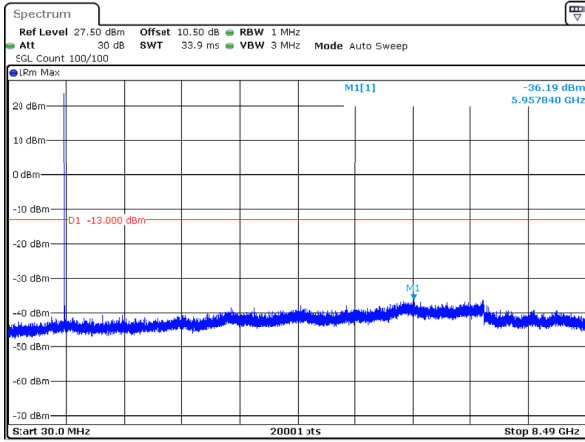
n5_5MHz_15kHz_846.5MHz_DFT-s-OFDM QPSK_RB1@0 -36.19dBm
