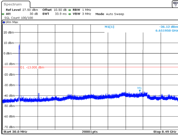
n5_20MHz_15kHz_836.5MHz_DFT-s-OFDM QPSK_RB100@0 -36.12dBm
