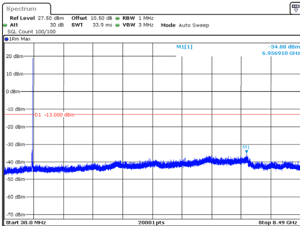
n5_20MHz_15kHz_836.5MHz_DFT-s-OFDM QPSK_RB1@105 -34.88dBm
