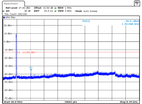
n5_20MHz_15kHz_834MHz_DFT-s-OFDM QPSK_RB100@0 -35.51dBm
