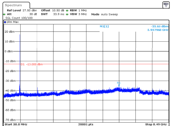
n5_20MHz_15kHz_834MHz_DFT-s-OFDM QPSK_RB1@105 -35.65dBm
