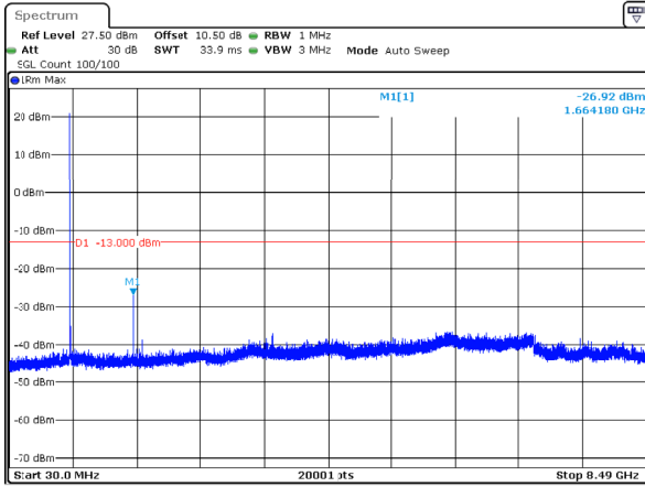
n5_10MHz_15kHz_836.5MHz_DFT-s-OFDM QPSK_RB1@0 -26.92dBm
