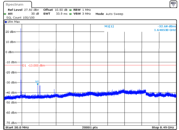
n5_10MHz_15kHz_829MHz_DFT-s-OFDM QPSK_RB1@0 -32.60dBm
