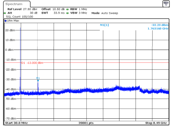
n5_10MHz_15kHz_836.5MHz_DFT-s-OFDM QPSK_RB1@51 -32.23dBm
