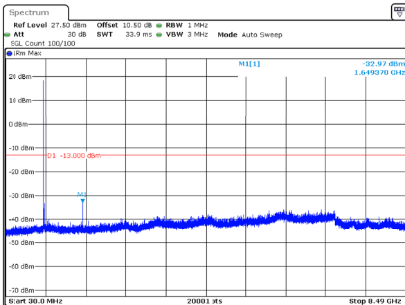
n5_20MHz_15kHz_834MHz_DFT-s-OFDM QPSK_RB1@0 -32.97dBm
