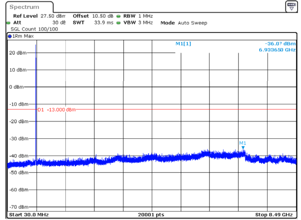
n5_5MHz_15kHz_846.5MHz_DFT-s-OFDM QPSK_RB1@24 -36.07dBm
