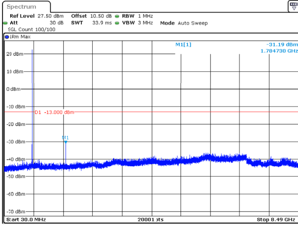
n5_10MHz_15kHz_829MHz_DFT-s-OFDM QPSK_RB1@51 -31.19dBm
