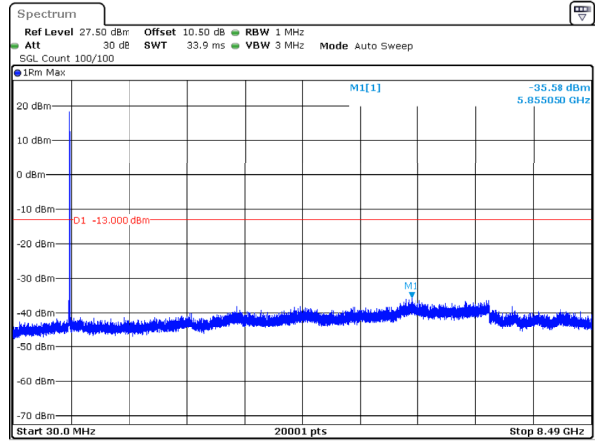
n5_15MHz_15kHz_841.5MHz_DFT-s-OFDM QPSK_RB1@78 -35.58dBm
