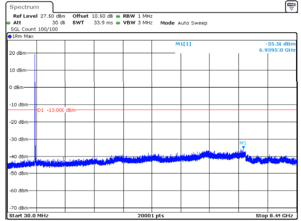
n5_20MHz_15kHz_836.5MHz_DFT-s-OFDM QPSK_RB1@0 -35.51dBm
