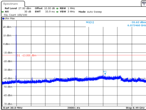
n5_10MHz_15kHz_844MHz_DFT-s-OFDM QPSK_RB1@51 -35.62dBm
