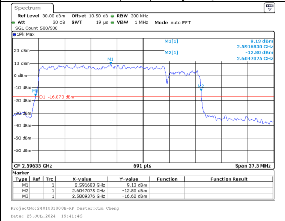
26%OBW Band 41 20MHz/2590.5/Mid 256QAM 100@0 Band 41 5MHz/2602.2/Mid 256QAM 25@0
