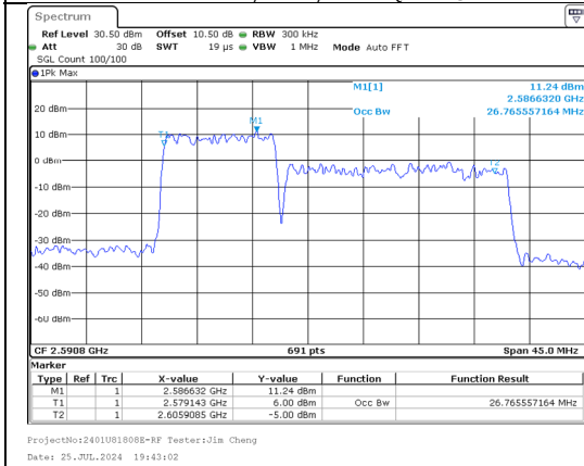
99%OBW Band 41 10MHz/2583.6/Mid QPSK 50@0 Band 41 20MHz/2598.0/Mid QPSK 100@0
