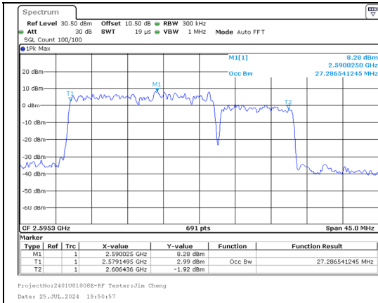
99%OBW Band 41 20MHz/2588.1/Mid 256QAM 100@0 Band 41 10MHz/2602.5/Mid 256QAM 50@0
