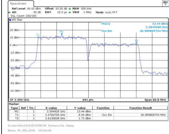
99%OBW Band 38 20MHz/2585.1/Mid 256QAM 100@0 Band 38 20MHz/2604.9/Mid 256QAM 100@0
