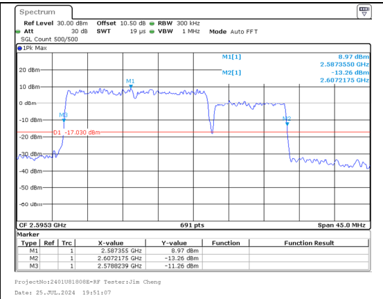
26%OBW Band 41 20MHz/2588.1/Mid 256QAM 100@0 Band 41 10MHz/2602.5/Mid 256QAM 50@0
