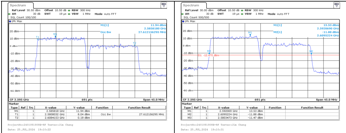
99%OBW Band 38 15MHz/2587.5/Mid 64QAM 75@0 Band 38 15MHz/2602.5/Mid 64QAM 75@0
