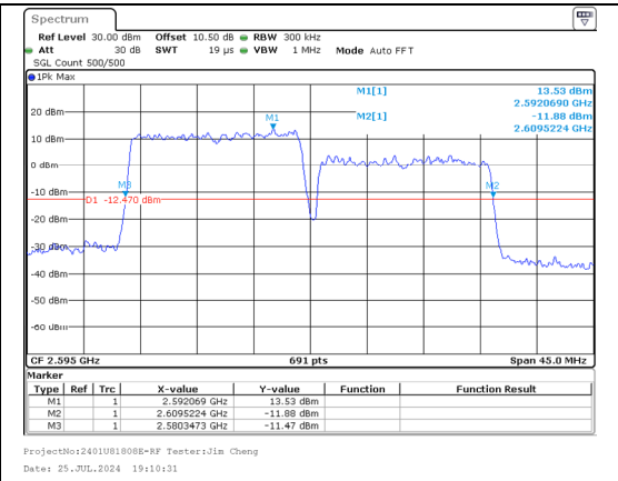
26%OBW Band 38 15MHz/2587.5/Mid 64QAM 75@0 Band 38 15MHz/2602.5/Mid 64QAM 75@0
