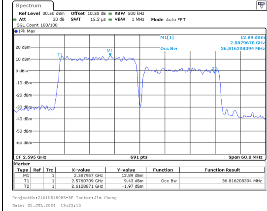
99%OBW Band 38 20MHz/2585.1/Mid 64QAM 100@0 Band 38 20MHz/2604.9/Mid 64QAM 100@0
