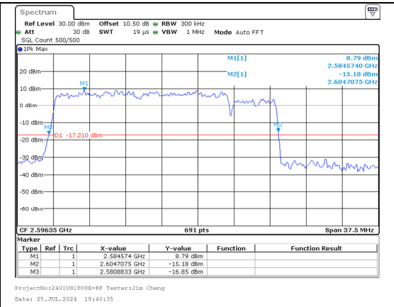
26%OBW Band 41 20MHz/2590.5/Mid 64QAM 100@0 Band 41 5MHz/2602.2/Mid 64QAM 25@0
