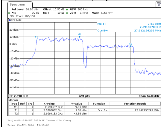
99%OBW Band 41 15MHz/2585.5/Mid 16QAM 75@0 Band 41 15MHz/2600.5/Mid 16QAM 75@0
