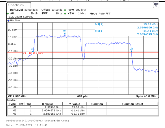
26%OBW Band 38 15MHz/2587.5/Mid 256QAM 75@0 Band 38 15MHz/2602.5/Mid 256QAM 75@0
