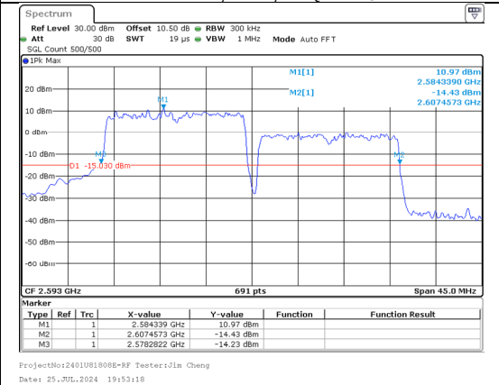
26%OBW Band 41 15MHz/2585.5/Mid 16QAM 75@0 Band 41 15MHz/2600.5/Mid 16QAM 75@0
