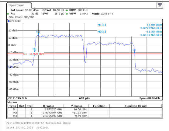
26%OBW Band 38 20MHz/2585.1/Mid 16QAM 100@0 Band 38 20MHz/2604.9/Mid 16QAM 100@0
