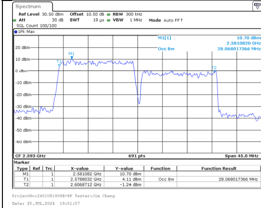
99%OBW Band 41 15MHz/2585.5/Mid QPSK 75@0 Band 41 15MHz/2600.5/Mid QPSK 75@0
