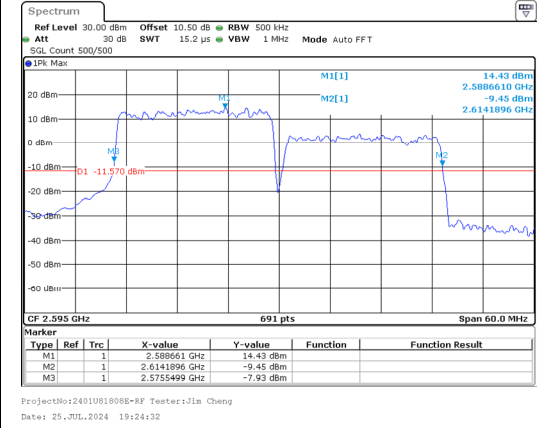
26%OBW Band 38 20MHz/2585.1/Mid 256QAM 100@0 Band 38 20MHz/2604.9/Mid 256QAM 100@0
