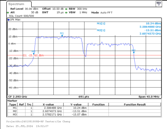
26%OBW Band 41 15MHz/2585.5/Mid QPSK 75@0 Band 41 15MHz/2600.5/Mid QPSK 75@0
