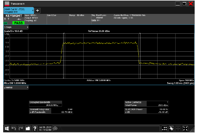
n78_3_70MHz_30kHz_3750MHz_DFT-s-OFDM 64 QAM_RB180@0 66.578MHz
