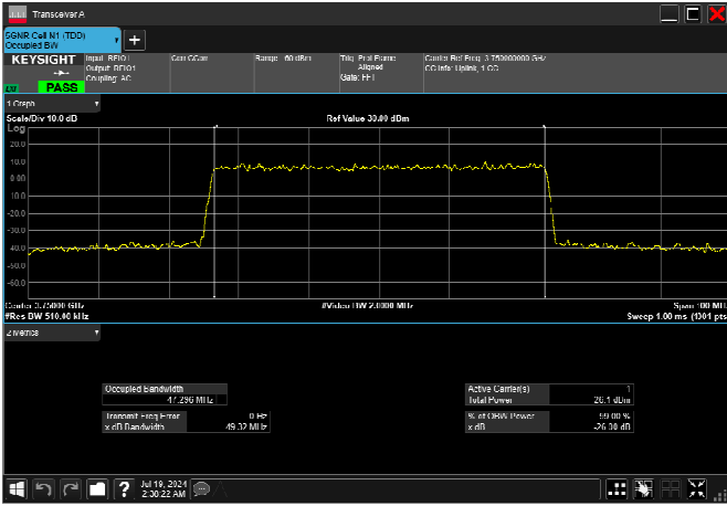
n78_3_50MHz_30kHz_3750MHz_CP-OFDM 256 QAM_RB133@0 47.287MHz
