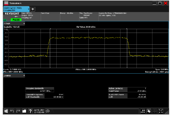
n78_3_60MHz_30kHz_3750MHz_CP-OFDM 16 QAM_RB162@0 57.681MHz
