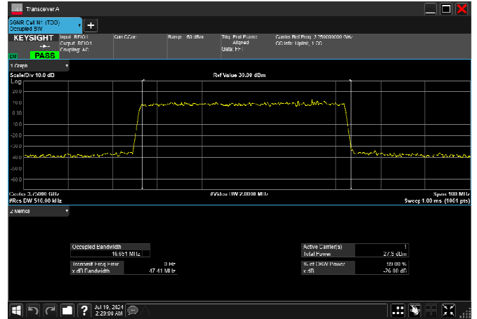
n78_3_50MHz_30kHz_3750MHz_DFT-s-OFDM 64 QAM_RB128@0 46.656MHz
