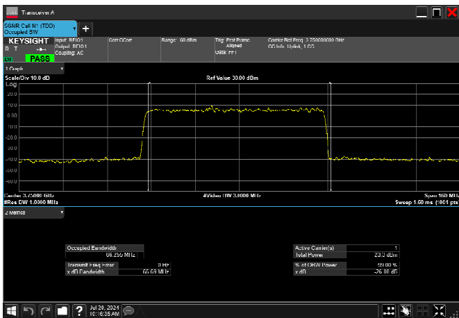
n78_3_70MHz_30kHz_3750MHz_DFT-s-OFDM 256 QAM_RB180@0 66.255MHz
