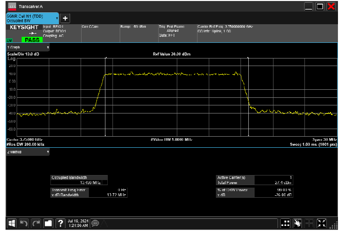
n78_3_15MHz_30kHz_3750MHz_DFT-s-OFDM 64 QAM_RB36@0 13.469MHz
