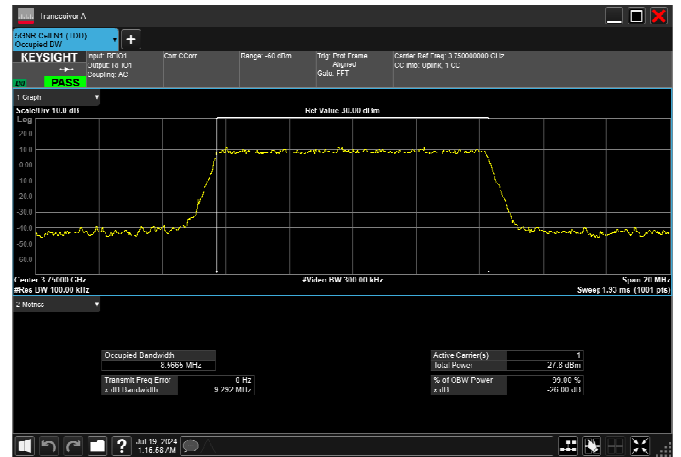
n78_3_10MHz_30kHz_3750MHz_DFT-s-OFDM 16 QAM_RB24@0 8.573MHz
