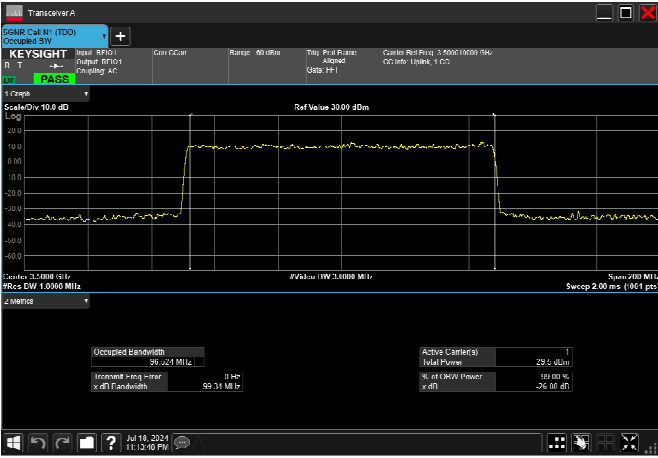
n78_1_100MHz_30kHz_3500MHz_DFT-s-OFDM 16 QAM_RB270@0 96.125MHz
