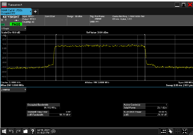
n78_1_100MHz_30kHz_3500MHz_DFT-s-OFDM 256 QAM_RB270@0 96.103MHz
