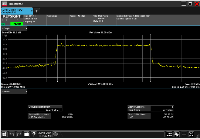
n78_1_100MHz_30kHz_3500MHz_CP-OFDM 16 QAM_RB273@0 97.271MHz
