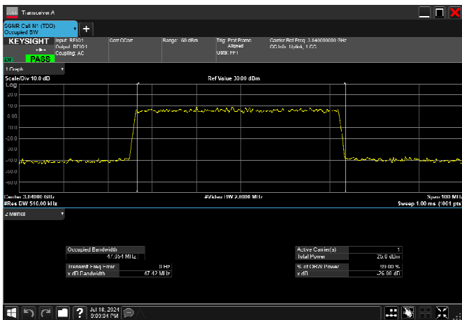
n77_3_50MHz_30kHz_3840MHz_DFT-s-OFDM 256 QAM_RB128@0 47.054MHz
