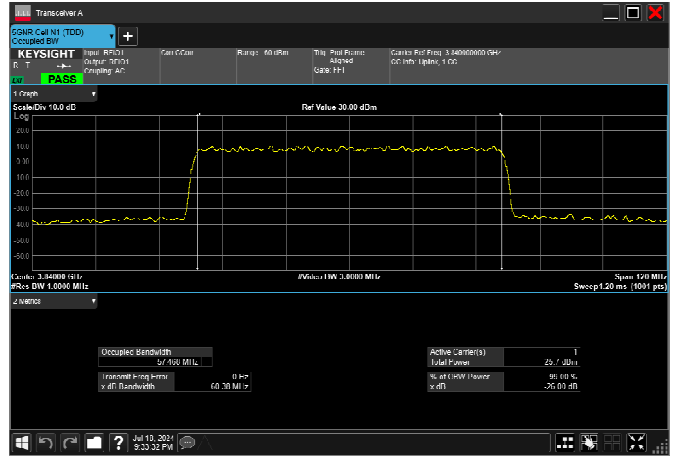
n77_3_60MHz_30kHz_3840MHz_CP-OFDM 16 QAM_RB162@0 57.657MHz
