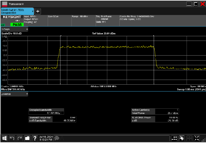
n77_3_50MHz_30kHz_3840MHz_CP-OFDM 256 QAM_RB133@0 47.286MHz
