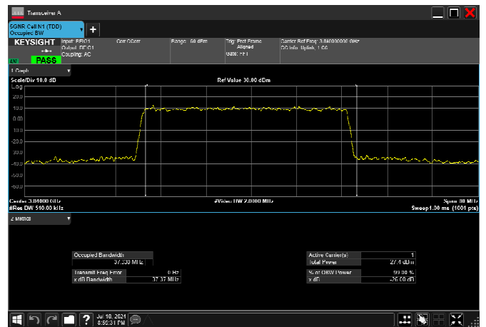
n77_3_40MHz_30kHz_3840MHz_DFT-s-OFDM 16 QAM_RB100@0 37.330MHz
