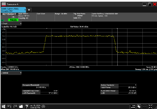
n77_3_40MHz_30kHz_3840MHz_DFT-s-OFDM QPSK_RB100@0 37.640MHz
