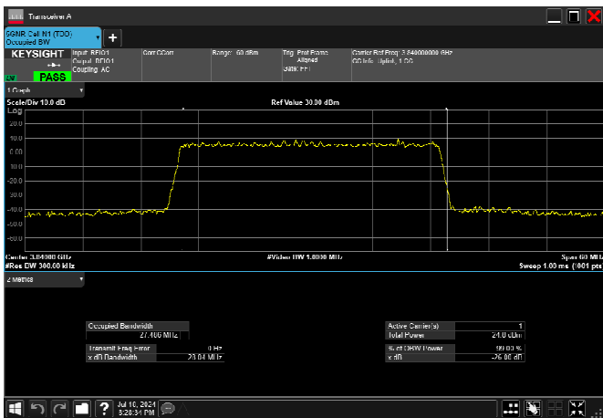
n77_3_30MHz_30kHz_3840MHz_DFT-s-OFDM 256 QAM_RB75@0 27.486MHz
