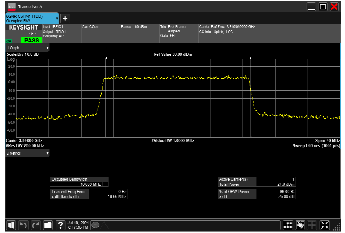
n77_3_20MHz_30kHz_3840MHz_CP-OFDM 16 QAM_RB51@0 18.170MHz
