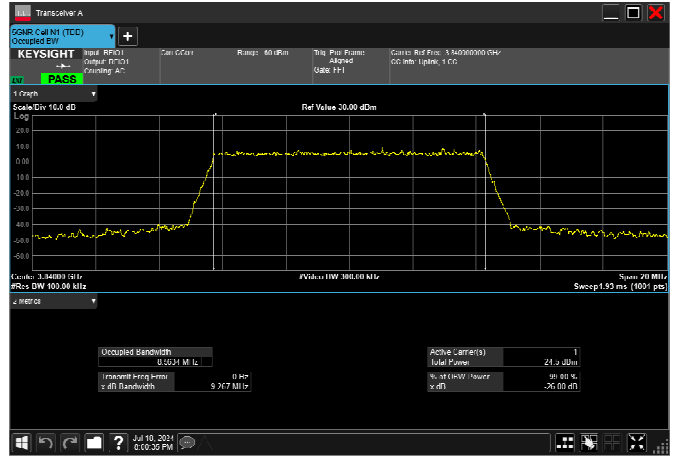
n77_3_10MHz_30kHz_3840MHz_CP-OFDM 16 QAM_RB24@0 8.571MHz
