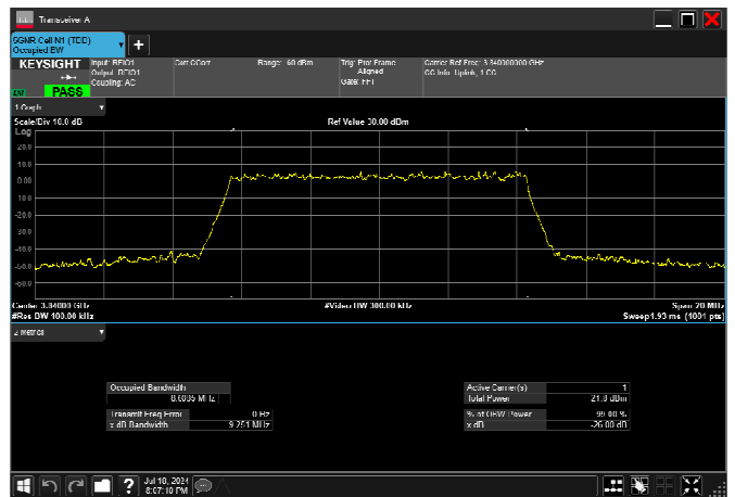
n77_3_10MHz_30kHz_3840MHz_CP-OFDM 256 QAM_RB24@0 8.608MHz
