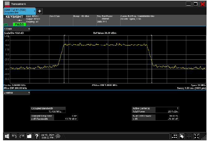
n77_3_15MHz_30kHz_3840MHz_DFT-s-OFDM 64 QAM_RB36@0 13.465MHz
