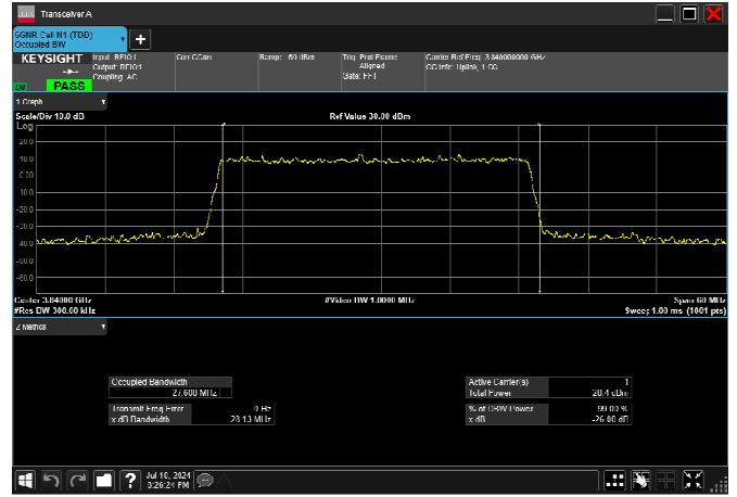
n77_3_30MHz_30kHz_3840MHz_DFT-s-OFDM 64 QAM_RB75@0 27.620MHz
