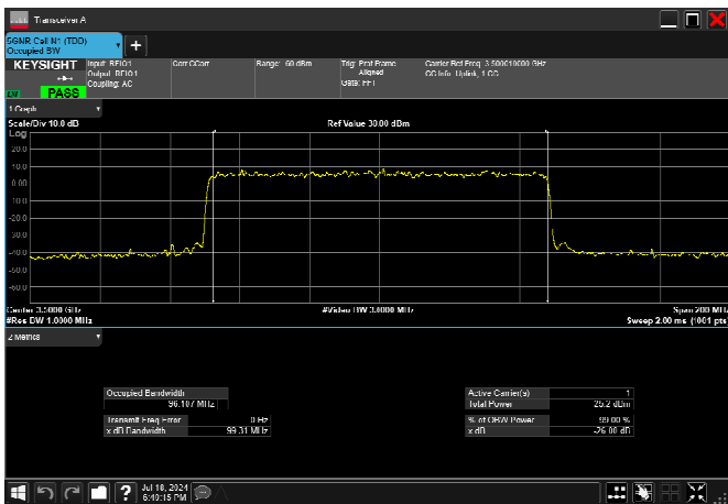
n77_1_100MHz_30kHz_3500MHz_DFT-s-OFDM 256 QAM_RB270@0 96.107MHz
