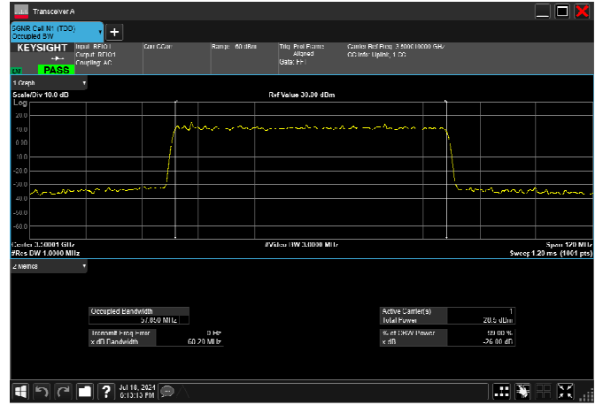
n77_1_60MHz_30kHz_3500MHz_DFT-s-OFDM 64 QAM_RB162@0 57.894MHz
