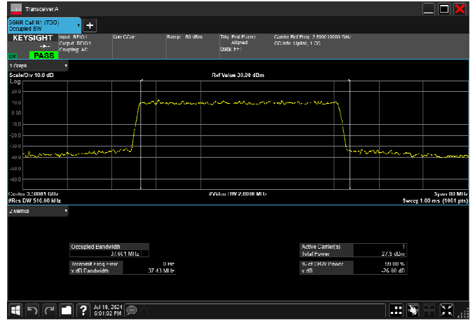
n77_1_40MHz_30kHz_3500MHz_DFT-s-OFDM 64 QAM_RB100@0 37.169MHz
