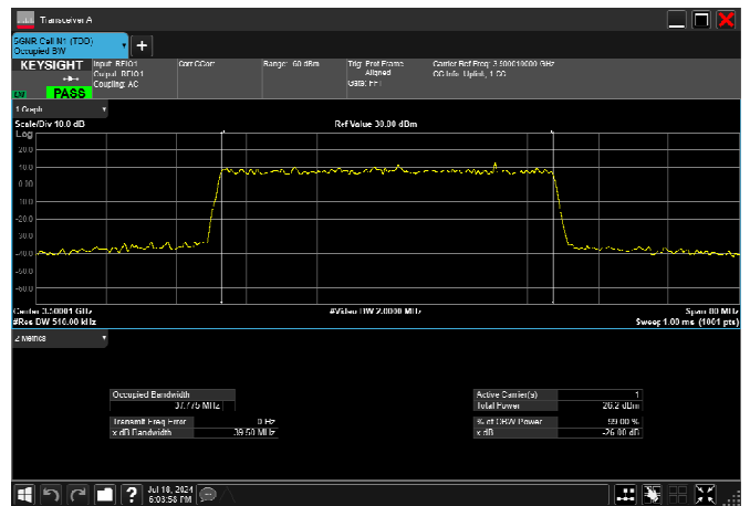
n77_1_40MHz_30kHz_3500MHz_CP-OFDM QPSK_RB106@0 37.775MHz
