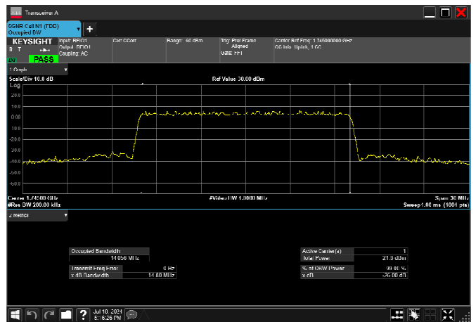
n66_15MHz_15kHz_1745MHz_CP-OFDM 256 QAM_RB79@0 14.056MHz
