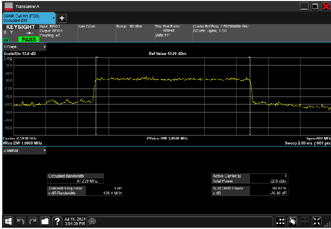
n41_100MHz_30kHz_2592.99MHz_CP-OFDM 16 QAM_RB273@0 97.239MHz
