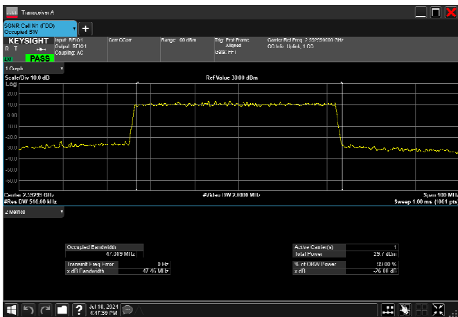
n41_50MHz_30kHz_2592.99MHz_DFT-s-OFDM 256 QAM_RB128@0 47.009MHz
