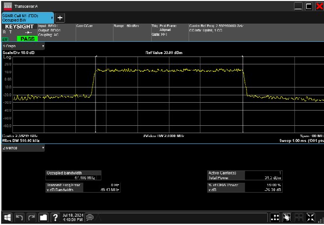
n41_50MHz_30kHz_2592.99MHz_CP-OFDM 256 QAM_RB133@0 47.410MHz
