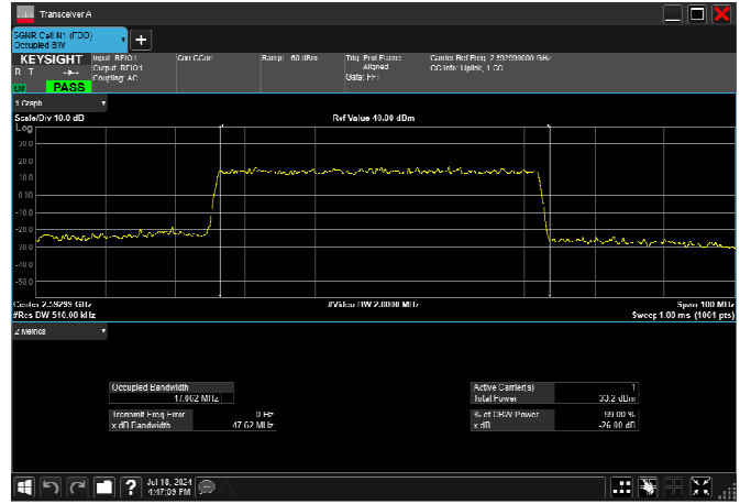
n41_50MHz_30kHz_2592.99MHz_DFT-s-OFDM 64 QAM_RB128@0 47.015MHz
