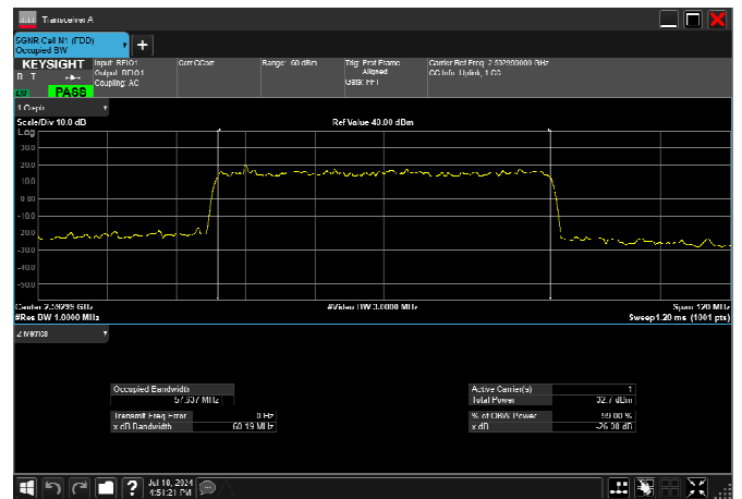
n41_60MHz_30kHz_2592.99MHz_DFT-s-OFDM 16 QAM_RB162@0 57.637MHz
