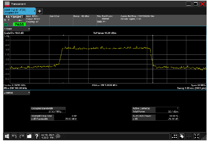
n41_30MHz_30kHz_2592.99MHz_DFT-s-OFDM 64 QAM_RB75@0 27.628MHz
