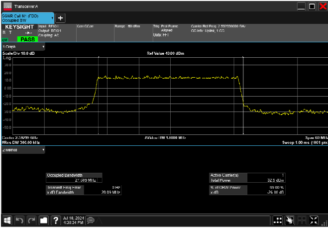
n41_30MHz_30kHz_2592.99MHz_DFT-s-OFDM 16 QAM_RB75@0 27.736MHz
