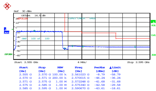
15MHz_High_16QAM_75@0
