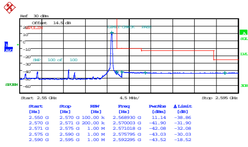
20MHz_High_16QAM_1@99
