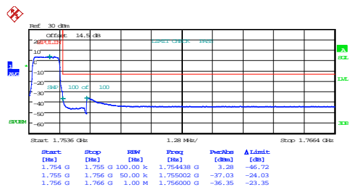
1.4MHz_High_QPSK_6@0
