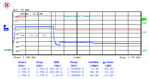
10MHz_High_QPSK_50@0
