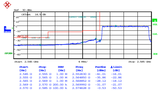
15MHz_Low_QPSK_75@0
