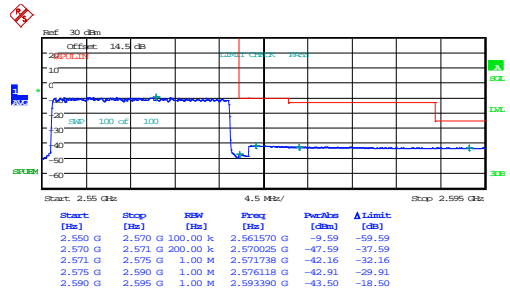
20MHz_High_16QAM_100@0
