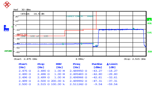
15MHz_Low_16QAM_75@0
