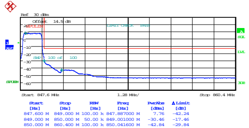
1.4MHz_High_QPSK_6@0
