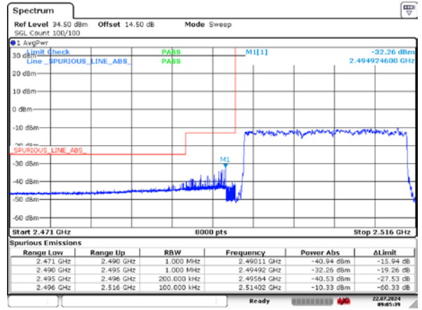
20MHz_Low_16QAM_100@0
