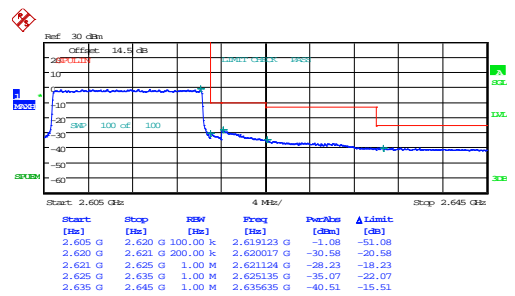
15MHz_High_QPSK_75@0
