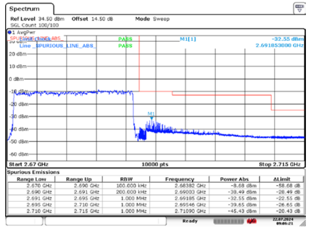
20MHz_High_QPSK_100@0
