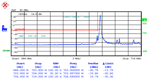
10MHz_Low_16QAM_1@0
