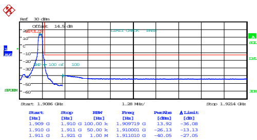
1.4MHz_High_QPSK_1@5
