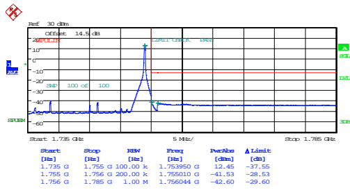
20MHz_High_QPSK_1@99
