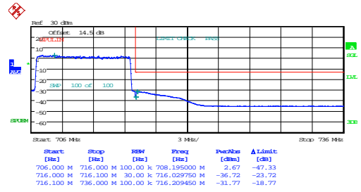
10MHz_High_16QAM_50@0
