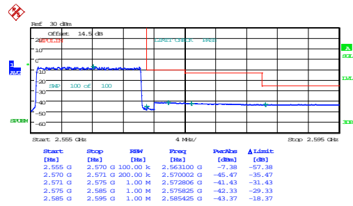
15MHz_High_QPSK_75@0
