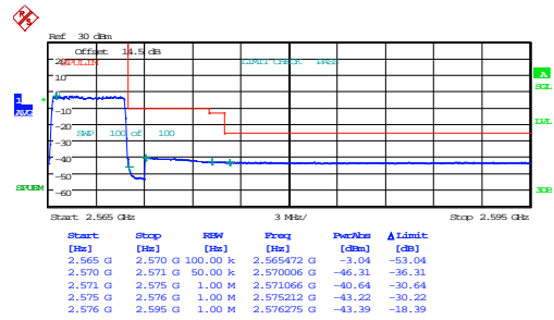
5MHz_High_QPSK_25@0
