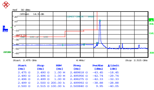
15MHz_Low_16QAM_1@0
