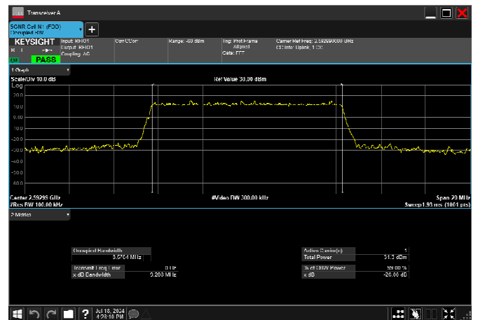
n41_10MHz_30kHz_2592.99MHz_DFT-s-OFDM 16 QAM_RB24@0 8.570MHz
