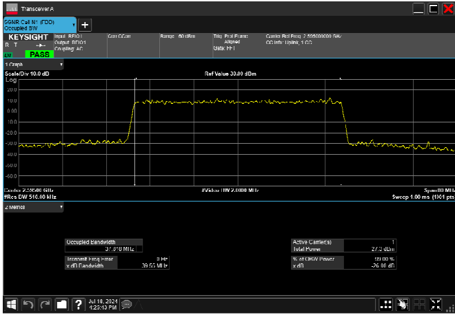
n38_40MHz_30kHz_2595MHz_CP-OFDM 16 QAM_RB106@0 37.818MHz
