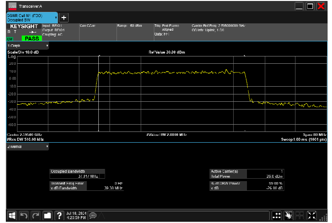
n38_40MHz_30kHz_2595MHz_CP-OFDM 64 QAM_RB106@0 37.817MHz
