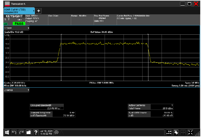
n38_25MHz_30kHz_2595MHz_DFT-s-OFDM 64 QAM_RB64@0 22.946MHz
