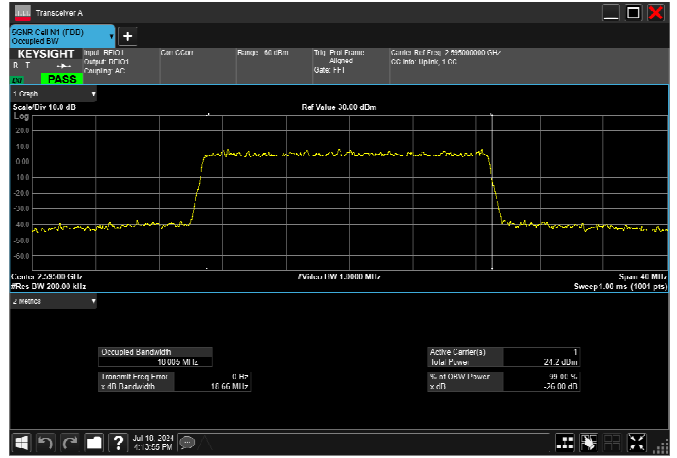
n38_20MHz_30kHz_2595MHz_CP-OFDM 16 QAM_RB51@0 18.182MHz
