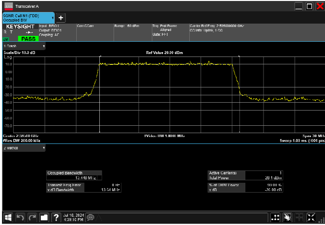
n38_15MHz_30kHz_2595MHz_DFT-s-OFDM 16 QAM_RB36@0 13.515MHz
