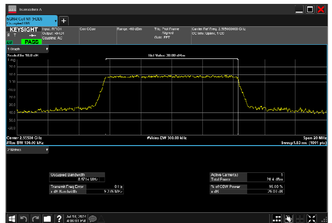
n38_10MHz_30kHz_2595MHz_DFT-s-OFDM 16 QAM_RB24@0 8.571MHz
