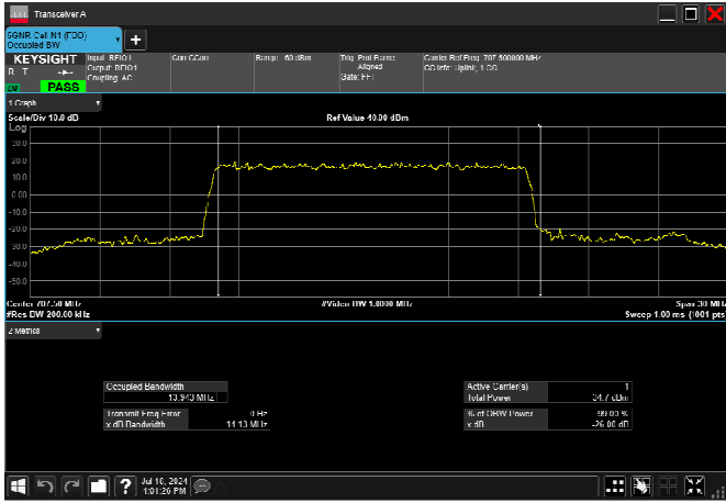
n12_15MHz_15kHz_707.5MHz_DFT-s-OFDM 16 QAM_RB75@0 13.943MHz
