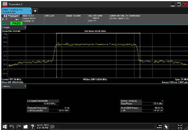
n12_15MHz_15kHz_707.5MHz_DFT-s-OFDM 256 QAM_RB75@0 13.935MHz
