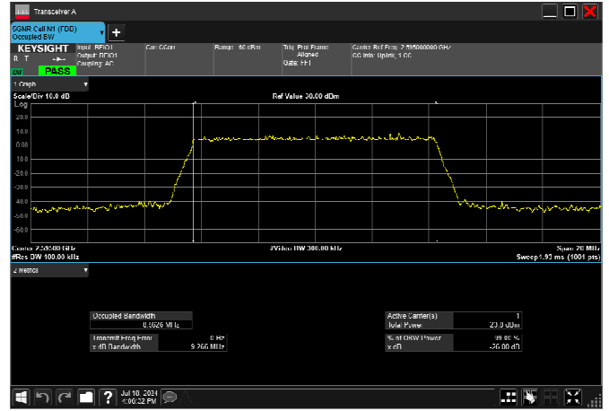
n38_10MHz_30kHz_2595MHz_CP-OFDM 16 QAM_RB24@0 8.574MHz
