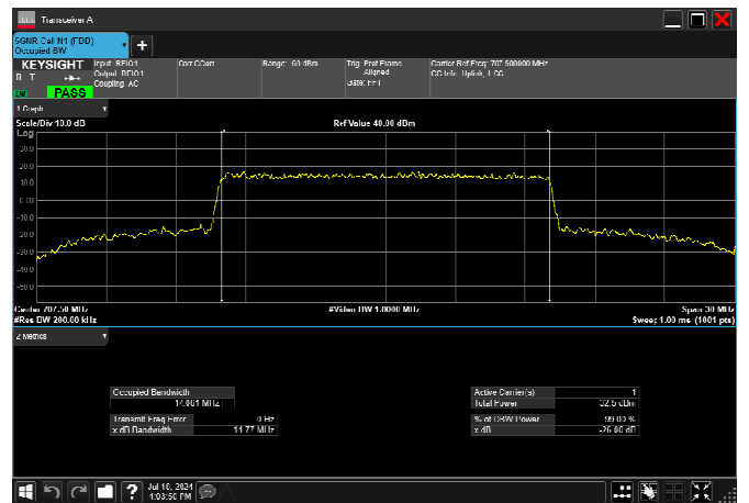
n12_15MHz_15kHz_707.5MHz_CP-OFDM QPSK_RB79@0 14.061MHz
