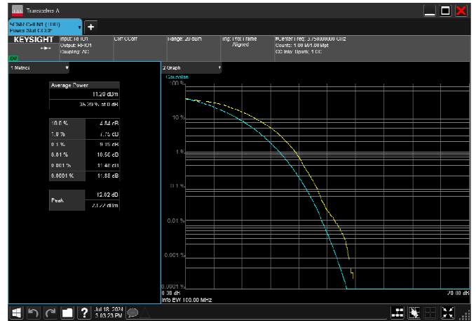
n78_3_100MHz_30kHz_3750MHz_CP-OFDM 16 QAM_RB273@0 10.97dB
