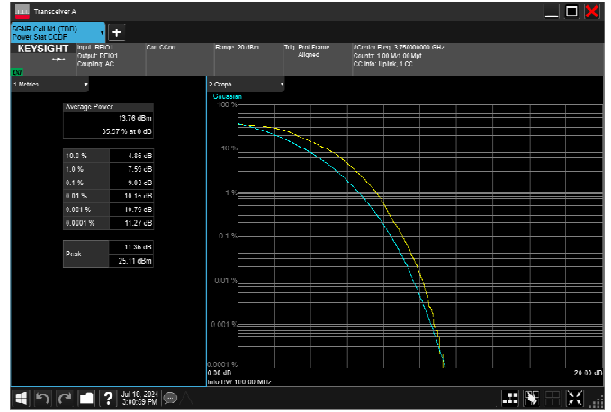
n78_3_100MHz_30kHz_3750MHz_DFT-s-OFDM 256 QAM_RB270@0 9.19dB
