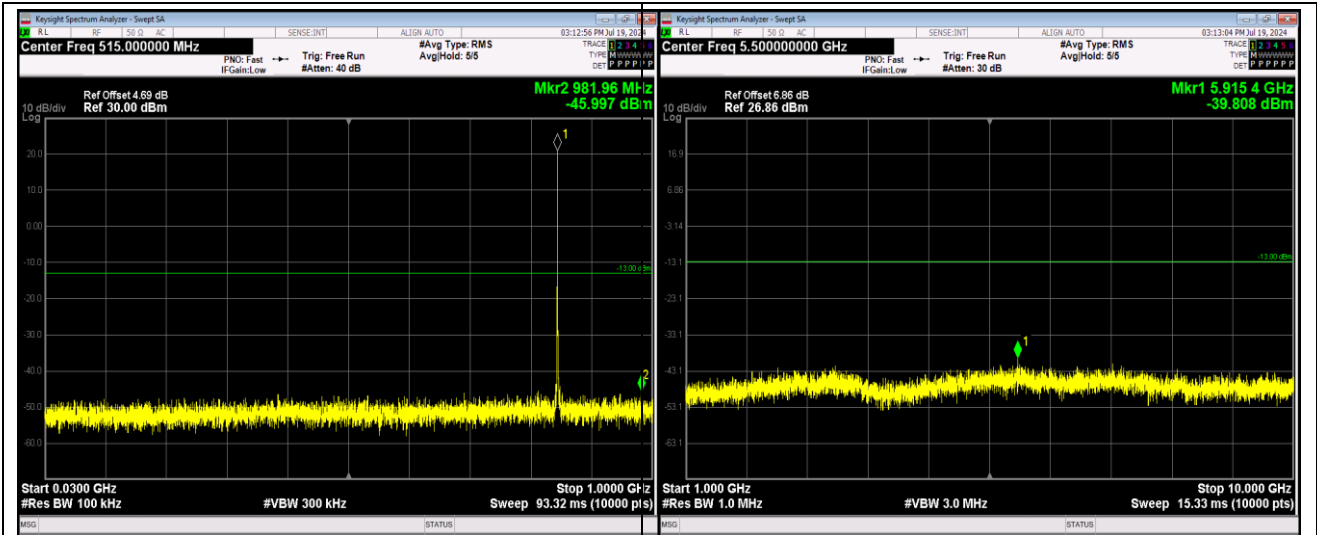
Band26-1.4MHz-64QAM-26697-1RB#0-Range1:30 ~1000MHz
