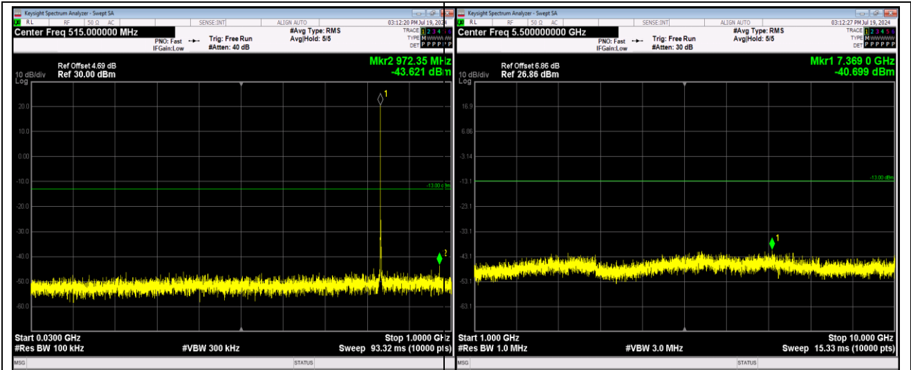
Band26-1.4MHz-64QAM-27033-1RB#0-Range1:30 ~1000MHz
