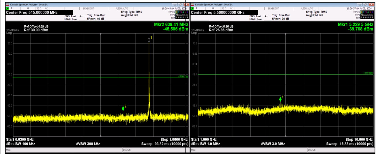
Band13-5MHz-16QAM-23255-1RB#0-Range1:30~1000MHz
