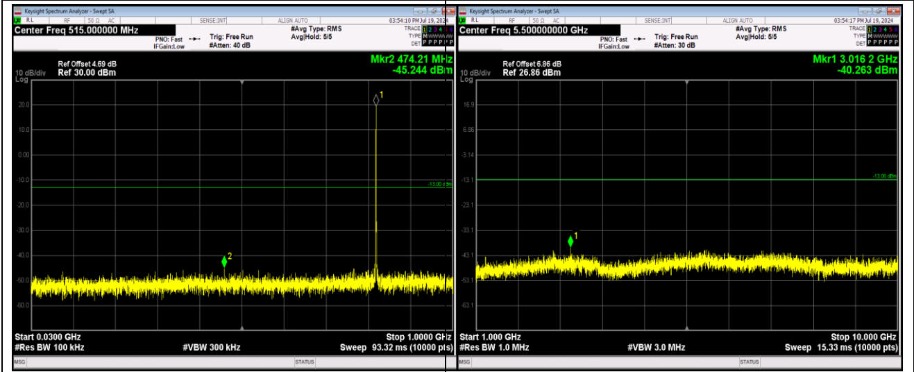
Band26-1.4MHz-16QAM-26783-1RB#0-Range1:30 ~1000MHz
