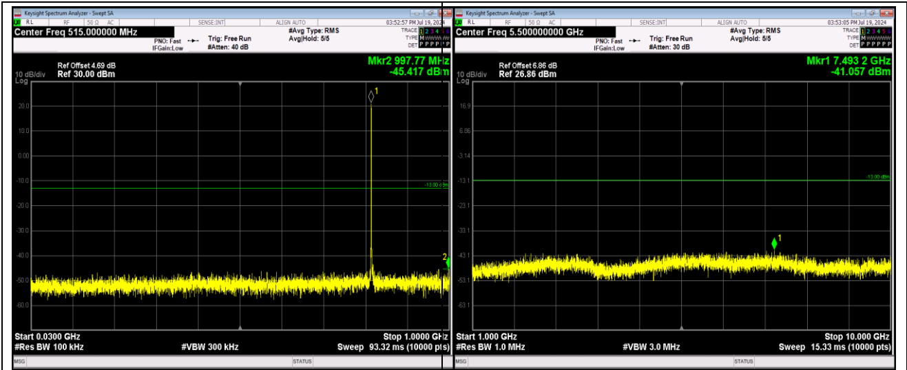
Band26-1.4MHz-QPSK-26783-1RB#0-Range1:30~1000MHz
