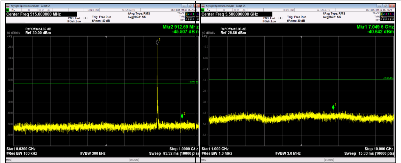
Band13-10MHz-QPSK-23230-1RB#0-Range1:30~1000MHz
