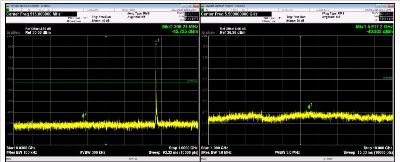
Band13-5MHz-16QAM-23230-1RB#0-Range1:30~1000MHz
