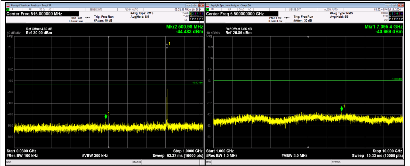
Band26-1.4MHz-64QAM-26740-1RB#0-Range1:30 ~1000MHz
