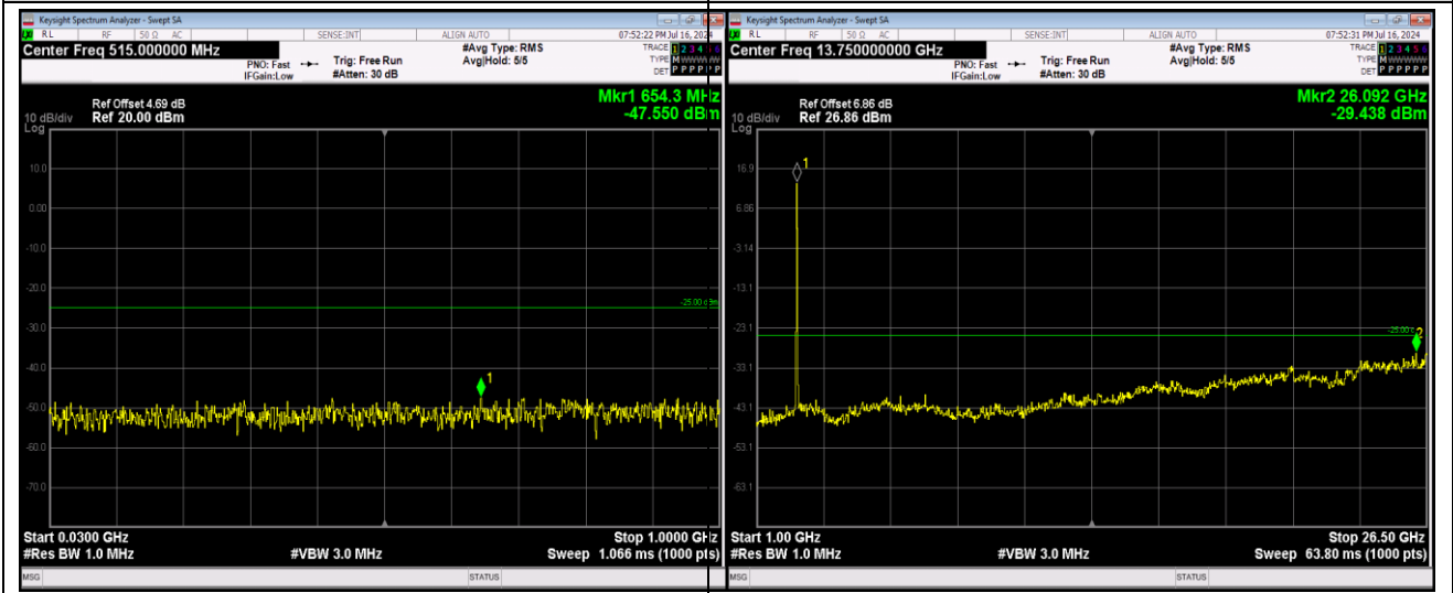
Band7-20MHz-64QAM-21100-1RB#0-Range1:30~1000MHz
