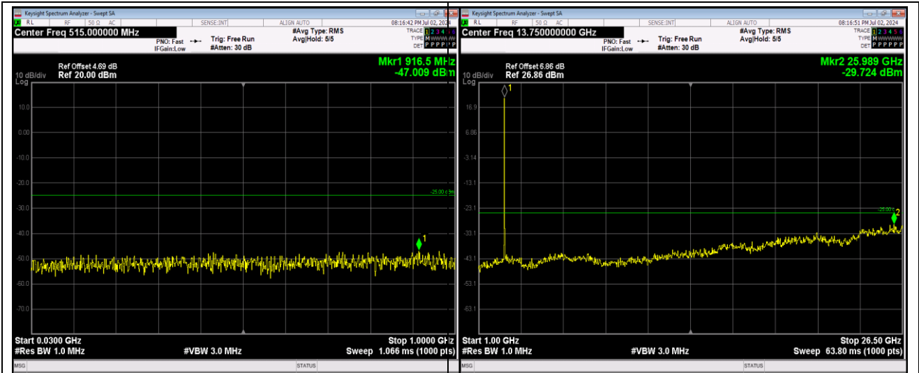
Band7-20MHz-64QAM-20850-1RB#0-Range1:30~1000MHz
