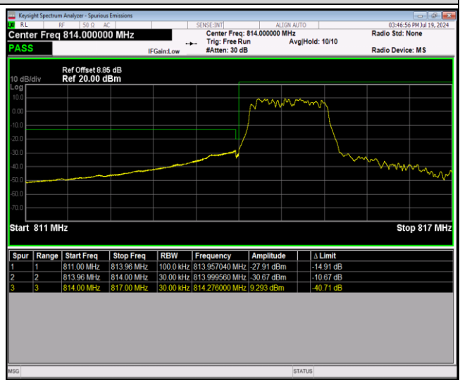
Band26-1.4MHz-16QAM-26783-1RB#5
