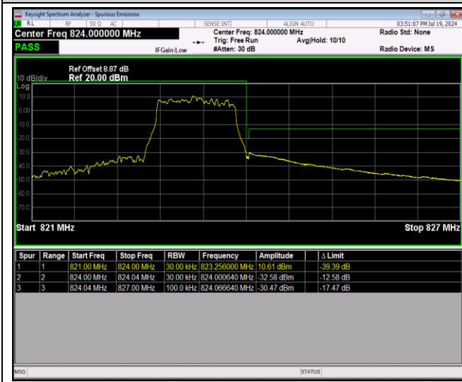
Band26-1.4MHz-16QAM-26797-1RB#5
