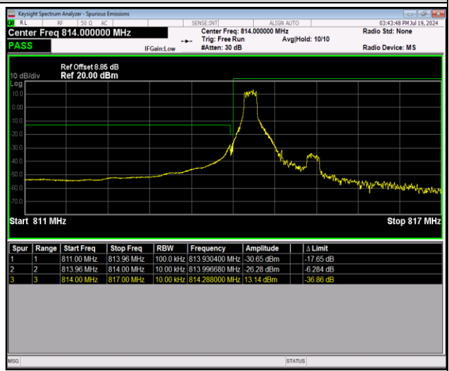
Band26-1.4MHz-16QAM-26697-6RB#0
