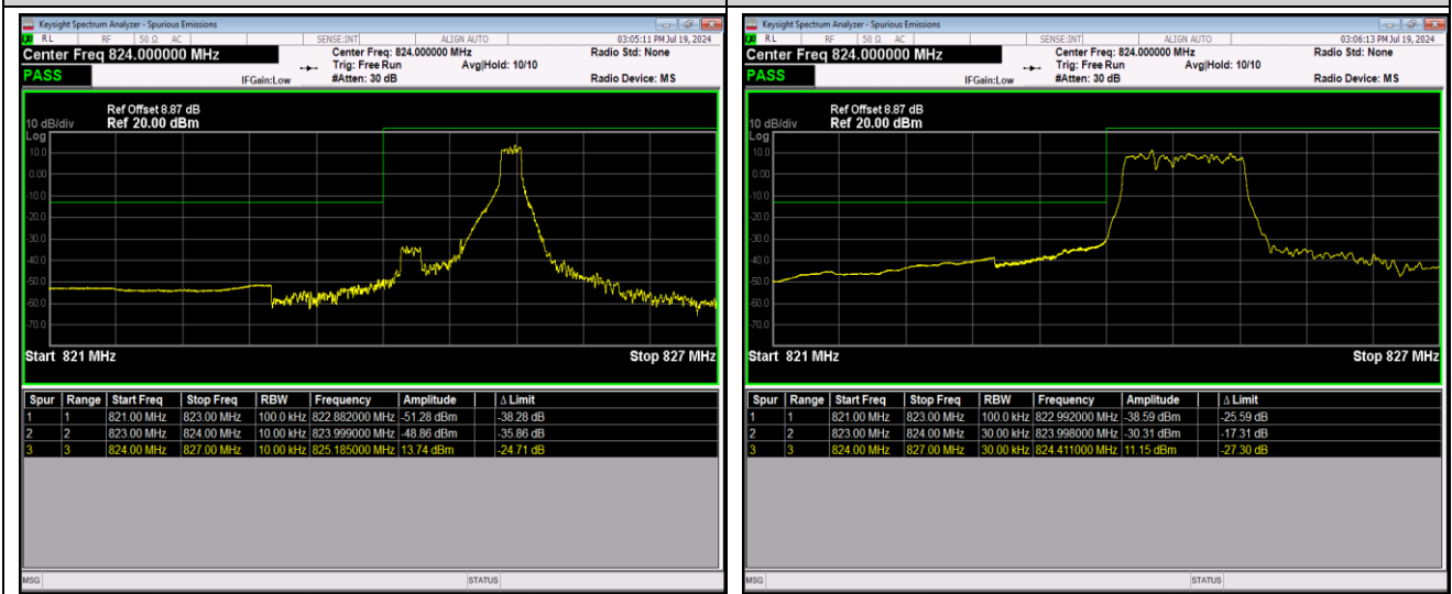
Band26-1.4MHz-QPSK-27033-1RB#0
