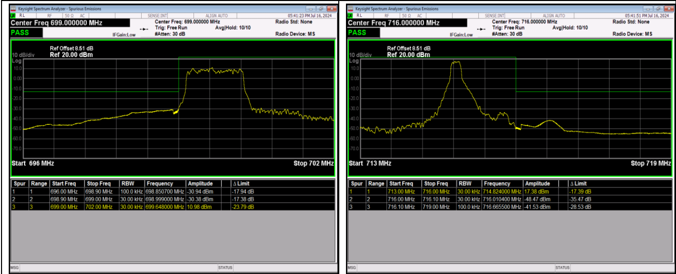
Band12-1.4MHz-64QAM-23173-1RB#5
