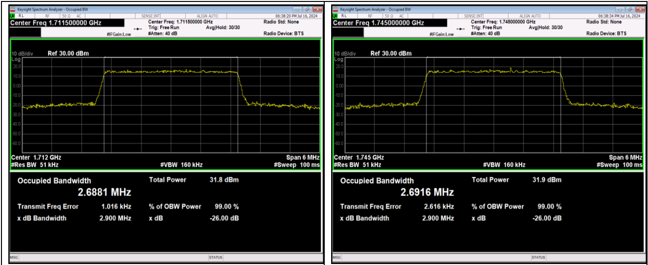
Band66-3MHz-64QAM-132657-15RB#0
