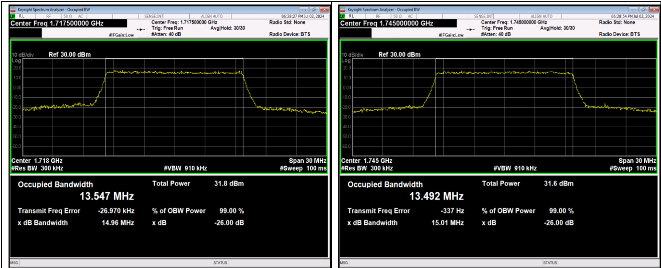
Band66-15MHz-16QAM-132597-75RB#0
