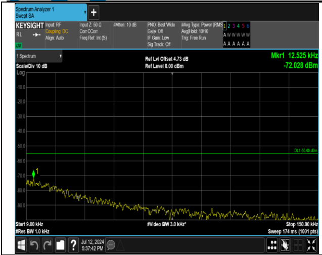
7-7-20MHz-20MHz-QPSK-QPSK-20850-21048-100RB#0-100RB#0-0.009~0.15MHz-PASS
