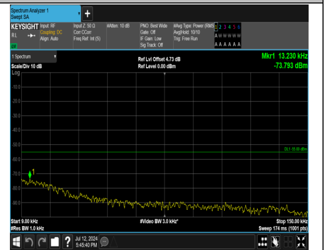
7-7-20MHz-20MHz-16QAM-16QAM-21001-21199-1RB#99-0RB#0-0.009~0.15MHz-PASS
