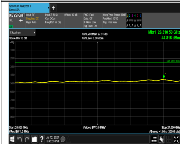
7-7-20MHz-20MHz-16QAM-16QAM-21001-21199-1RB#99 -ORB#0-20000~27000MHz-PASS
