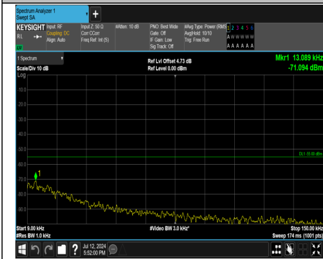
7-7-20MHz-20MHz-16QAM-16QAM-21001-21199-100RB# 0-100RB#0-0.009~0.15MHz-PASS
