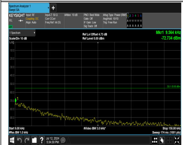
7-7-20MHz-20MHz-QPSK-QPSK-20850-21048-1RB#0-1R B#99-0.009~0.15MHz-PASS
