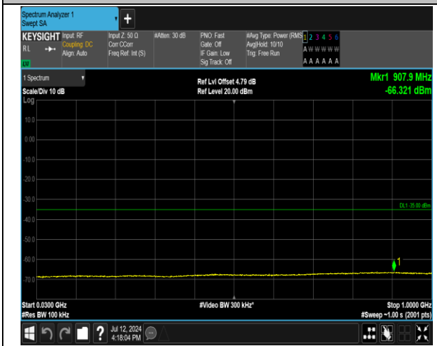
7-7-20MHz-15MHz-QPSK-QPSK-21201-21372-100RB#0-75RB#0-30~1000MHz-PASS
