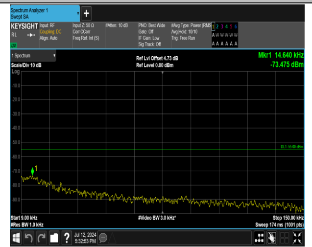
7-7-20MHz-20MHz-16QAM-16QAM-20850-21048-1RB#99-0RB#0-0.009~0.15MHz-PASS
