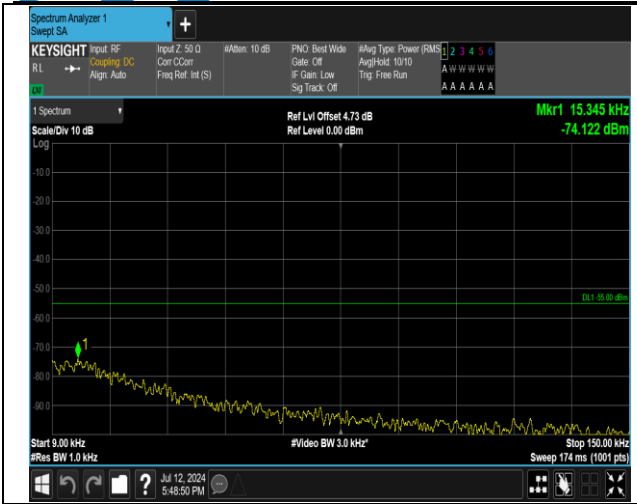
7-7-20MHz-20MHz-16QAM-16QAM-21001-21199-1RB#0-1RB#99-0.009~0.15MHz-PASS
