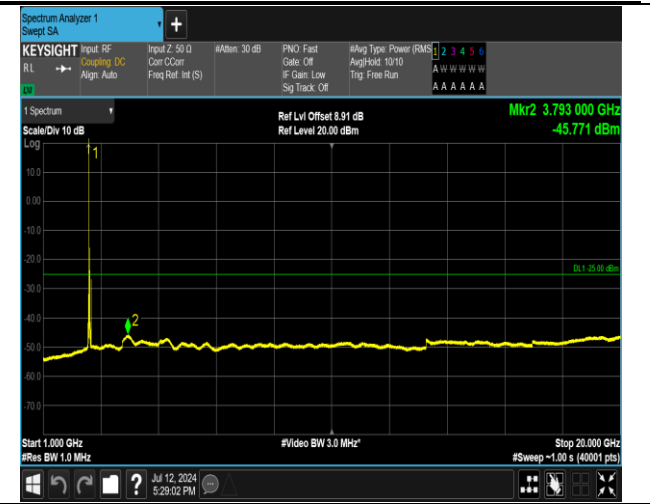
7-7-20MHz-20MHz-QPSK-QPSK-20850-21048-1RB#0-0R B#0-1000~20000MHz-PASS
