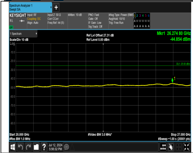
7-7-20MHz-20MHz-16QAM-16QAM-21152-21350-1RB#0-ORB#0-20000~27000MHz-PASS
