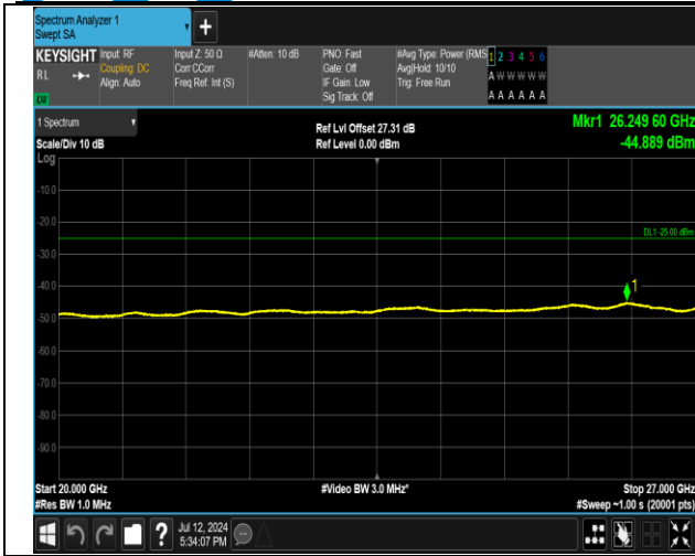
7-7-20MHz-20MHz-16QAM-16QAM-20850-21048-1RB#9 9-0RB#0-20000~27000MHz-PASS
