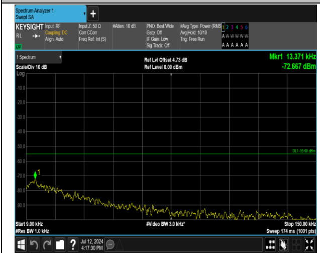
7-7-20MHz-15MHz-QPSK-QPSK-21201-21372-100RB#0-0-75RB#0-0.009~0.15MHz-PASS
