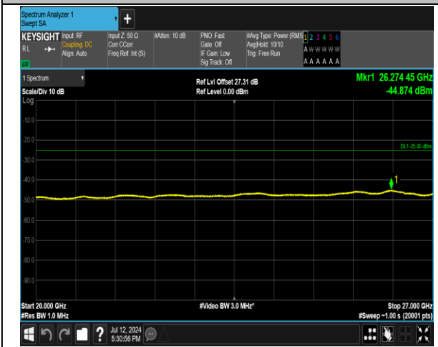
7-7-20MHz-20MHz-16QAM-16QAM-20850-21048-1RB#0-ORB#0-20000~27000MHz-PASS
