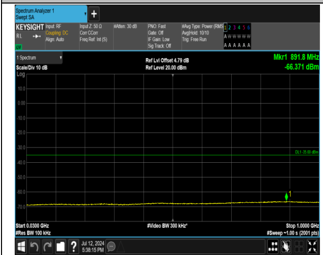
7-7-20MHz-20MHz-QPSK-QPSK-20850-21048-100RB#0-100RB#0-30~1000MHz-PASS
