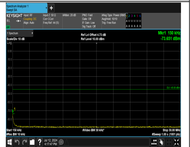
7-7-20MHz-15MHz-QPSK-QPSK-21201-21372-100RB#0-0-75RB#0-0.15~30MHz-PASS
