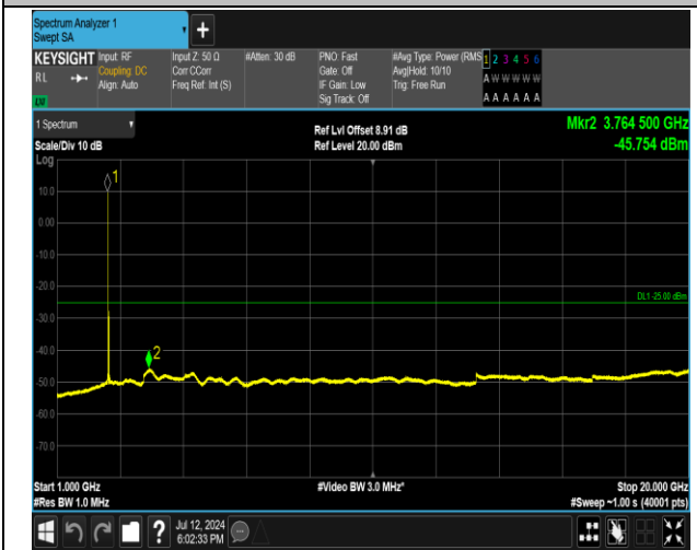
7-7-20MHz-20MHz-16QAM-16QAM-21152-21350-1RB#0-1RB#99-1000~20000MHz-PASS
