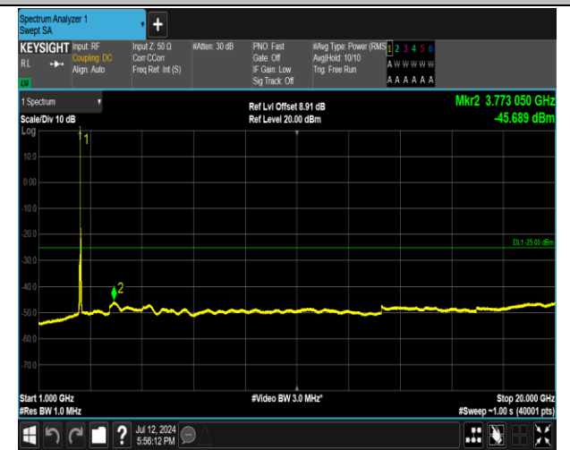
7-7-20MHz-20MHz-16QAM-16QAM-21152-21350-1RB#0- ORB#0-1000~20000MHz-PASS
