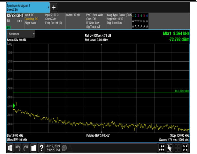
7-7-20MHz-20MHz-16QAM-16QAM-21001-21199-1RB#0-ORB#0-0.009~0.15MHz-PASS
