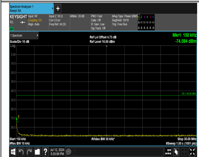
7-7-20MHz-20MHz-16QAM-16QAM-20850-21048-1RB#9-0RB#0-0.15~30MHz-PASS
