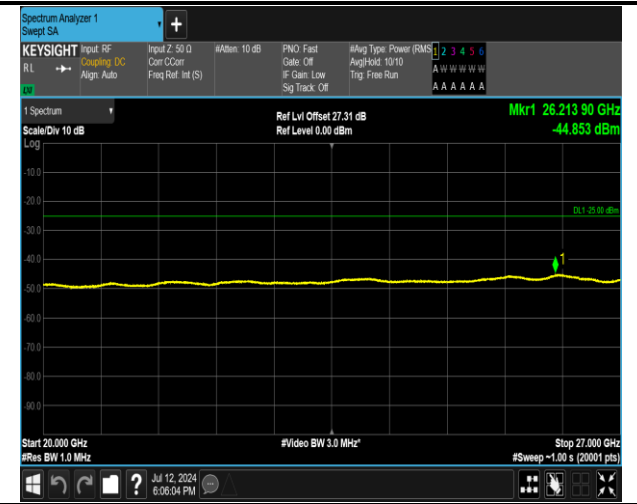
7-7-20MHz-20MHz-16QAM-16QAM-21152-21350-100RB# 0-100RB#0-20000~27000MHz-PASS
