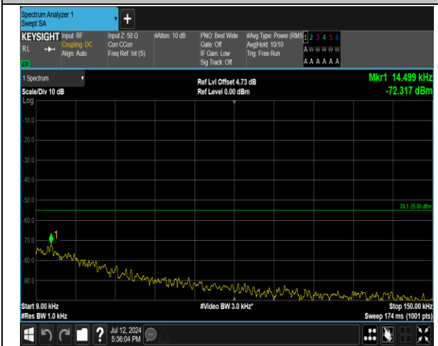
7-7-20MHz-20MHz-16QAM-16QAM-20850-21048-1RB#0-1RB#99-0.009~0.15MHz-PASS
