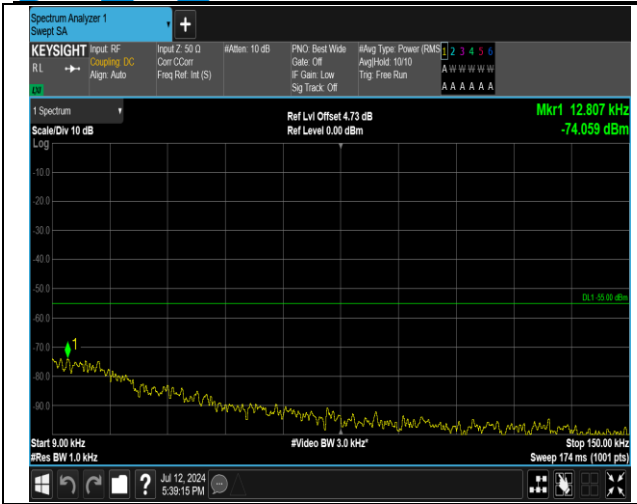
7-7-20MHz-20MHz-16QAM-16QAM-20850-21048-100RB #0-100RB#0-0.009~0.15MHz-PASS
