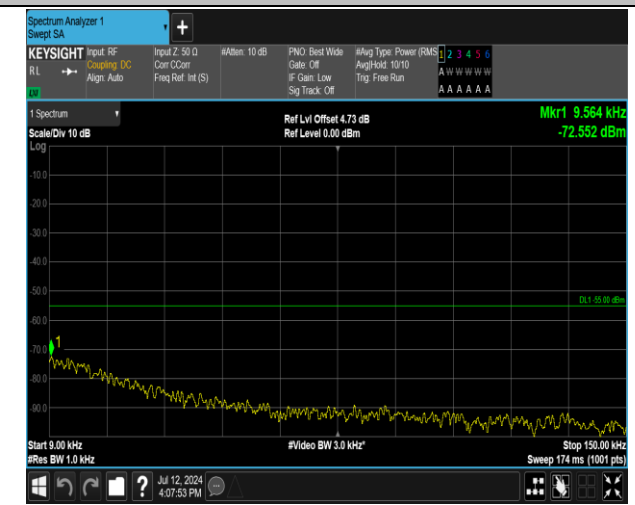
7-7-20MHz-15MHz-QPSK-QPSK-21201-21372-1RB#0-0RB#0-0.009~0.15MHz-PASS
