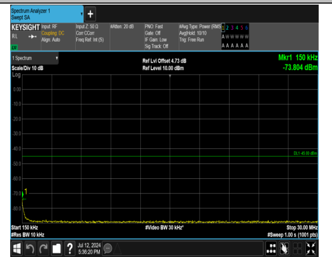
7-7-20MHz-20MHz-16QAM-16QAM-20850-21048-1RB#0-1RB#99-0.15~30MHz-PASS
