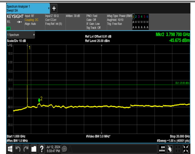
7-7-20MHz-20MHz-16QAM-16QAM-20850-21048-1RB#99-0RB#0-1000~20000MHz-PASS
