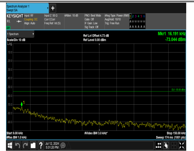
7-7-20MHz-20MHz-QPSK-QPSK-20850-21048-1RB#99-0 RB#0-0.009~0.15MHz-PASS
