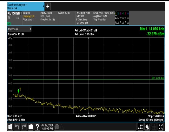
7-7-20MHz-15MHz-QPSK-QPSK-21201-21372-1RB#99-0 RB#0-0.009~0.15MHz-PASS
