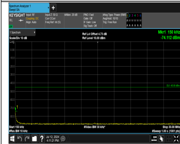
7-7-20MHz-15MHz-QPSK-QPSK-21201-21372-1RB#99-0 RB#0-0.15~30MHz-PASS
