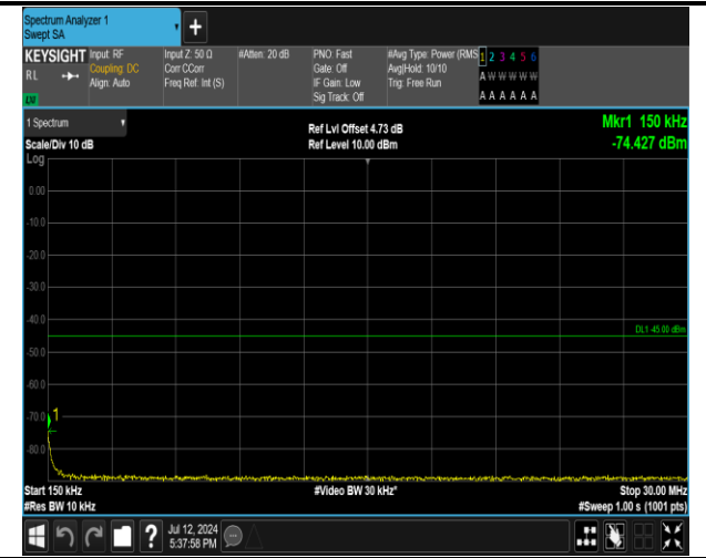
7-7-20MHz-20MHz-QPSK-QPSK-20850-21048-100RB#0-100RB#0-0.15~30MHz-PASS
