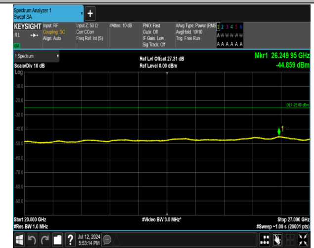
7-7-20MHz-20MHz-16QAM-16QAM-21001-21199-100RB# 0-100RB#0-20000~27000MHz-PASS
