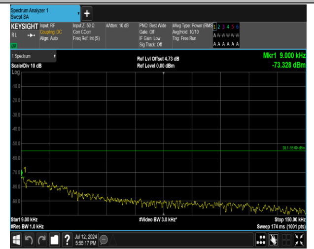
7-7-20MHz-20MHz-16QAM-16QAM-21152-21350-1RB#0- ORB#0-0.009~0.15MHz-PASS
