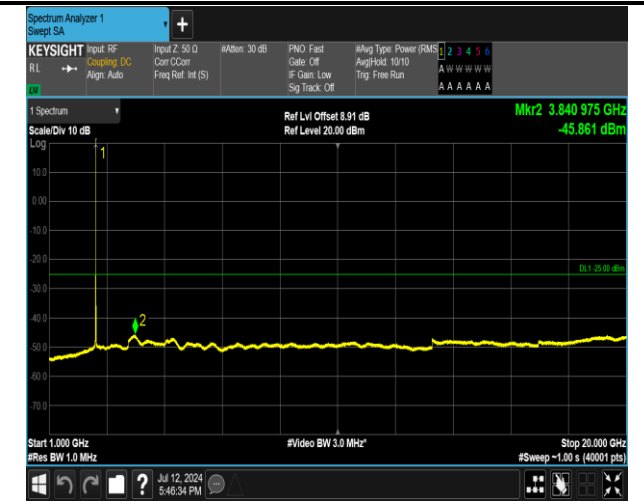
7-7-20MHz-20MHz-16QAM-16QAM-21001-21199-1RB#99 -ORB#0-1000~20000MHz-PASS
