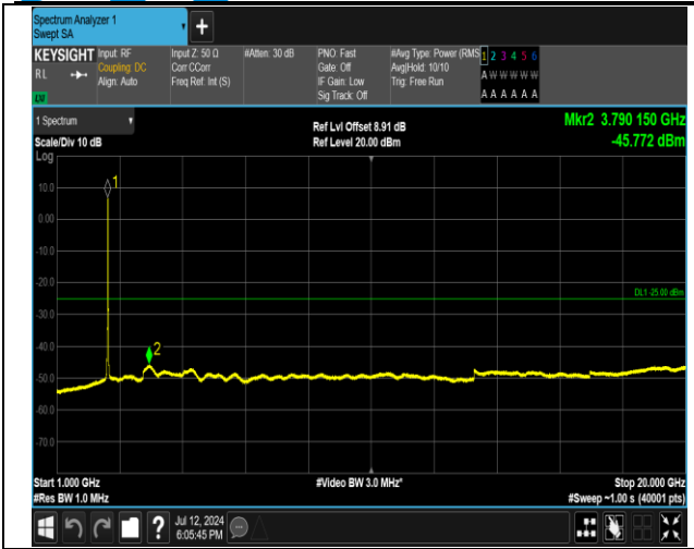
7-7-20MHz-20MHz-16QAM-16QAM-21152-21350-100RB# 0-100RB#0-1000~20000MHz-PASS
