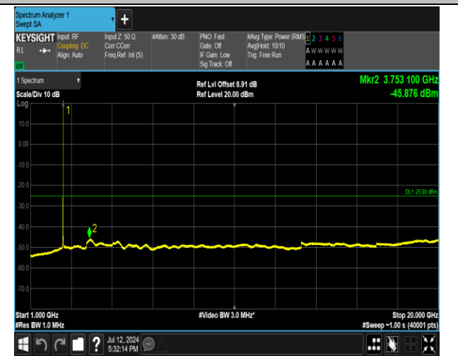
7-7-20MHz-20MHz-QPSK-QPSK-20850-21048-1RB#99-0 RB#0-1000~20000MHz-PASS
