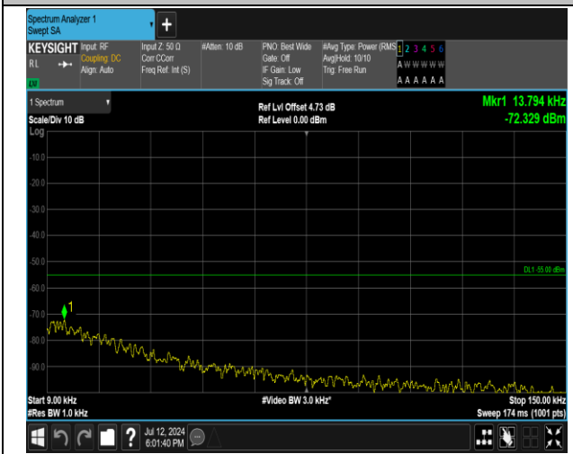
7-7-20MHz-20MHz-16QAM-16QAM-21152-21350-1RB#0-1RB#99-0.009~0.15MHz-PASS
