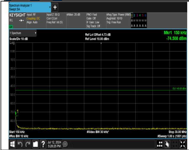
7-7-20MHz-20MHz-QPSK-QPSK-20850-21048-1RB#0-0R B#0-0.15~30MHz-PASS
