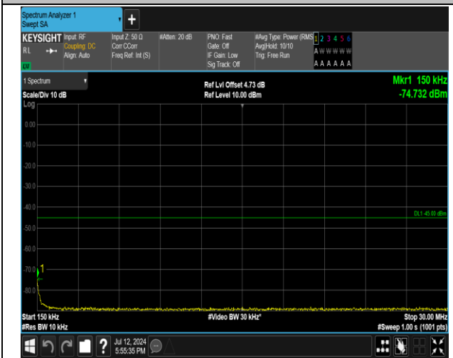
7-7-20MHz-20MHz-16QAM-16QAM-21152-21350-1RB#0- ORB#0-0.15~30MHz-PASS
