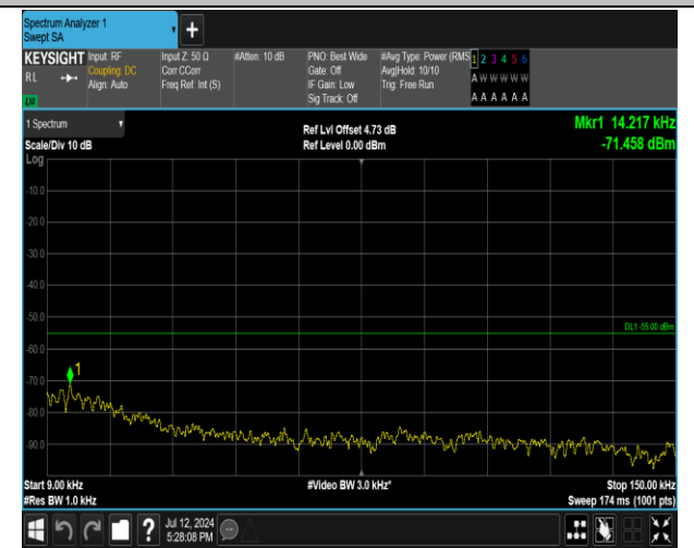
7-7-20MHz-20MHz-QPSK-QPSK-20850-21048-1RB#0-0RB#0-0.009~0.15MHz-PASS
