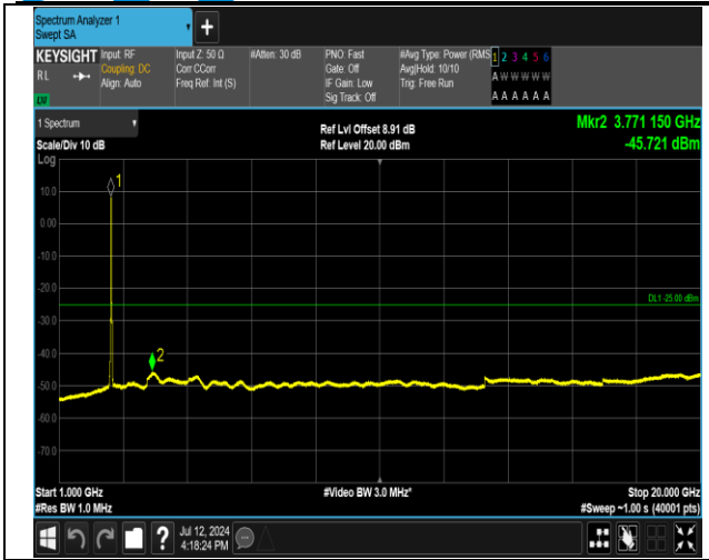
7-7-20MHz-15MHz-QPSK-QPSK-21201-21372-100RB#0-75RB#0-1000~20000MHz-PASS
