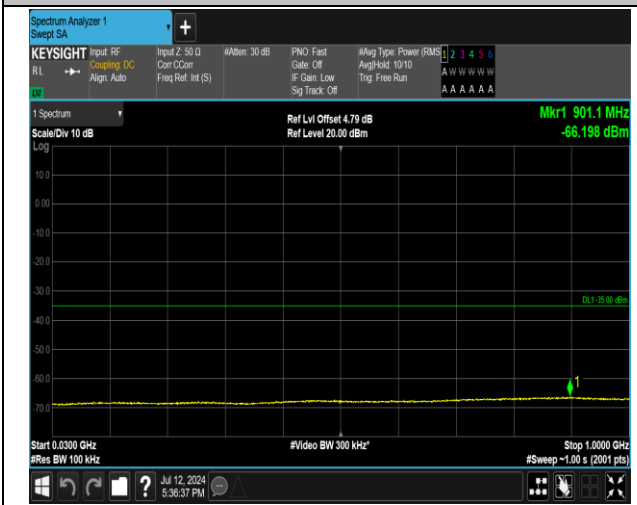
7-7-20MHz-20MHz-16QAM-16QAM-20850-21048-1RB#0-1RB#99-30~1000MHz-PASS
