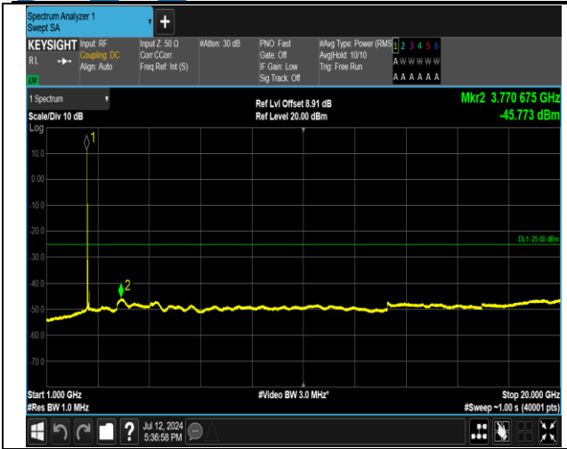
7-7-20MHz-20MHz-16QAM-16QAM-20850-21048-1RB#0-1RB#99-1000~20000MHz-PASS
