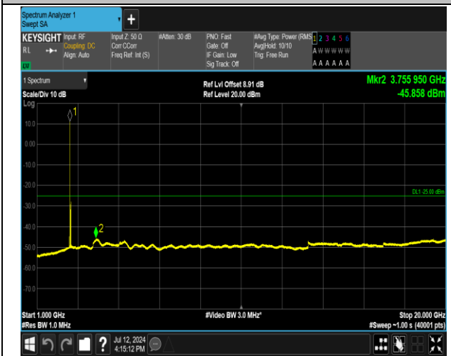
7-7-20MHz-15MHz-QPSK-QPSK-21201-21372-1RB#0-1R B#74-1000~20000MHz-PASS
