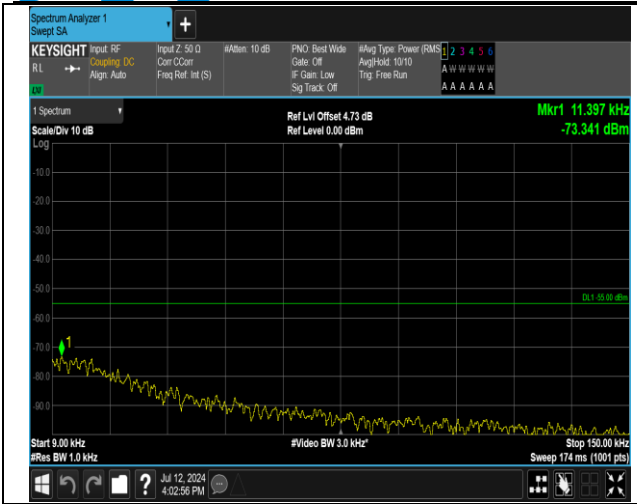
7-7-20MHz-15MHz-16QAM-16QAM-21026-21197-1RB#0-1RB#74-0.009~0.15MHz-PASS
