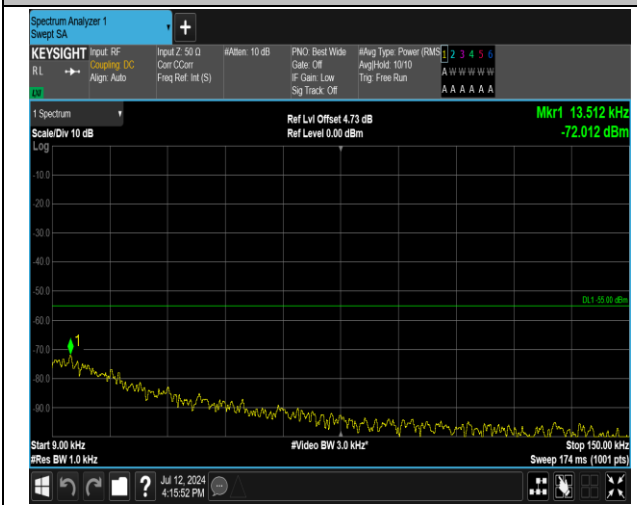
7-7-20MHz-15MHz-16QAM-16QAM-21201-21372-1RB#0-1RB#74-0.009~0.15MHz-PASS
