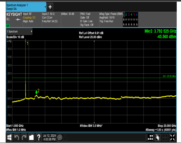
7-7-20MHz-15MHz-16QAM-16QAM-21026-21197-1RB#99 -ORB#0-1000~20000MHz-PASS
