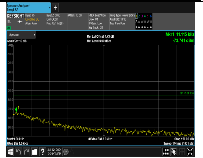
7-7-20MHz-10MHz-QPSK-QPSK-21251-21395-1RB#99-0 RB#0-0.009~0.15MHz-PASS
