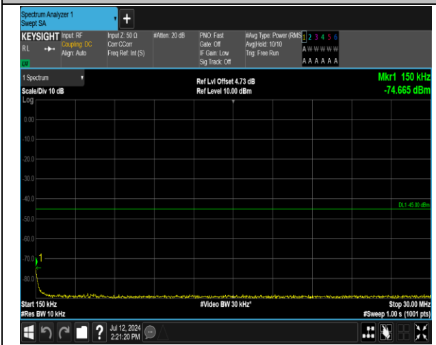
7-7-20MHz-10MHz-QPSK-QPSK-21251-21395-1RB#99-0 RB#0-0.15~30MHz-PASS
