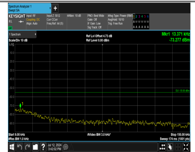
7-7-20MHz-15MHz-QPSK-QPSK-20850-21021-1RB#0-0RB#0-0.009~0.15MHz-PASS
