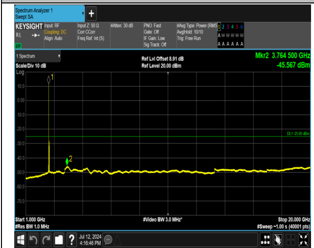
7-7-20MHz-15MHz-16QAM-16QAM-21201-21372-1RB#0-1RB#74-1000~20000MHz-PASS
