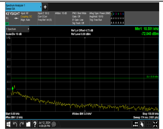
7-7-20MHz-15MHz-16QAM-16QAM-21201-21372-1RB#0- ORB#0-0.009~0.15MHz-PASS
