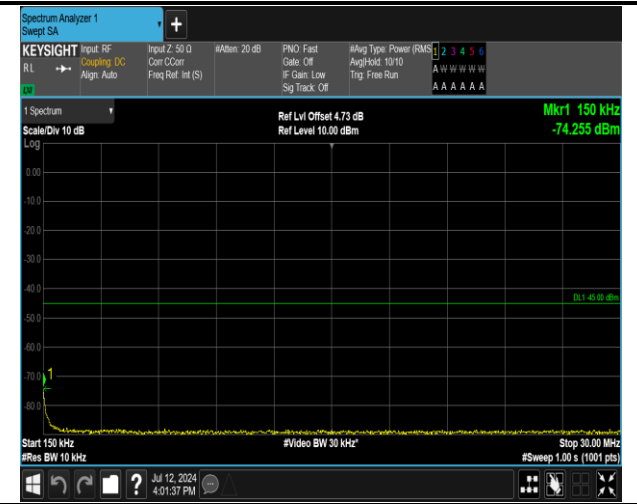
7-7-20MHz-15MHz-QPSK-QPSK-21026-21197-1RB#0-1R B#74-0.15~30MHz-PASS
