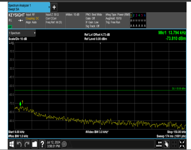
7-7-20MHz-15MHz-16QAM-16QAM-21026-21197-1RB#0-ORB#0-0.009~0.15MHz-PASS
