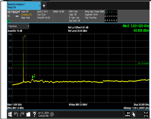
7-7-20MHz-15MHz-QPSK-QPSK-20850-21021-1RB#0-1R B#74-1000~20000MHz-PASS
