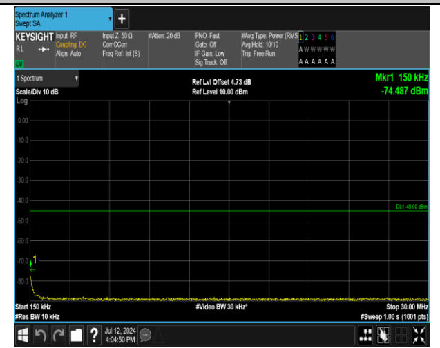
7-7-20MHz-15MHz-QPSK-QPSK-21026-21197-100RB#0-75RB#0-0.15~30MHz-PASS
