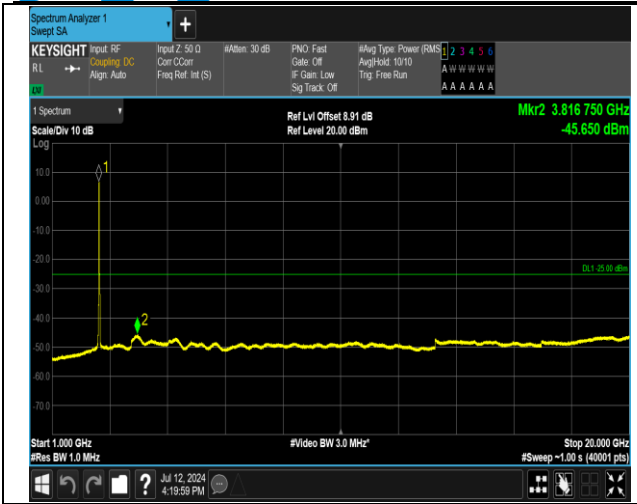
7-7-20MHz-15MHz-16QAM-16QAM-21201-21372-100RB #0-75RB#0-1000~20000MHz-PASS
