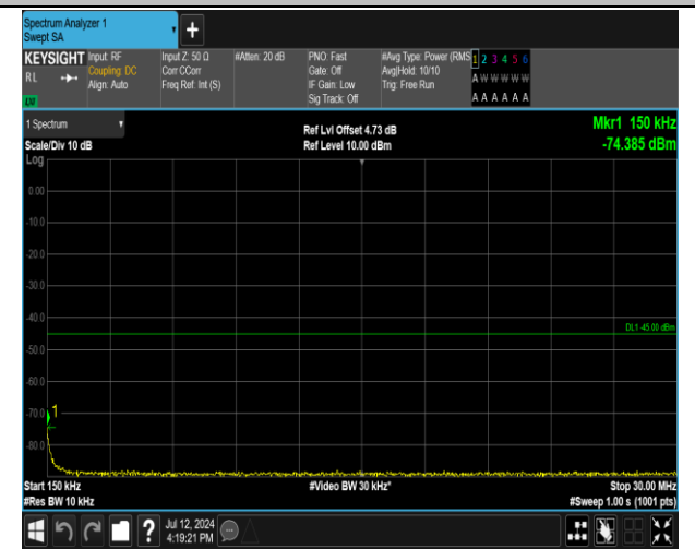
7-7-20MHz-15MHz-16QAM-16QAM-21201-21372-100RB# 0-75RB#0-0.15~30MHz-PASS
