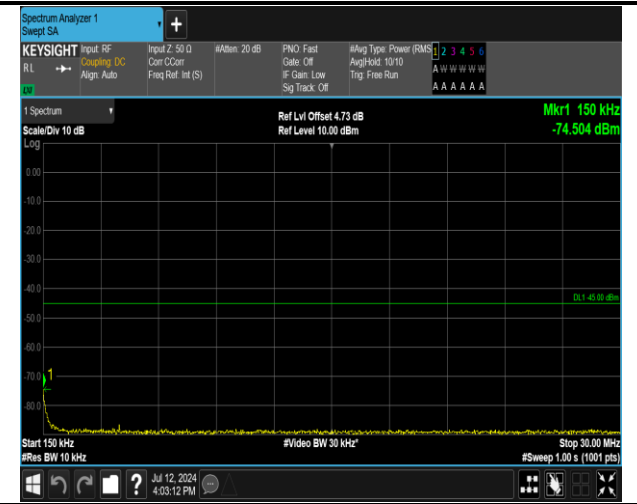
7-7-20MHz-15MHz-16QAM-16QAM-21026-21197-1RB#0-1RB#74-0.15~30MHz-PASS
