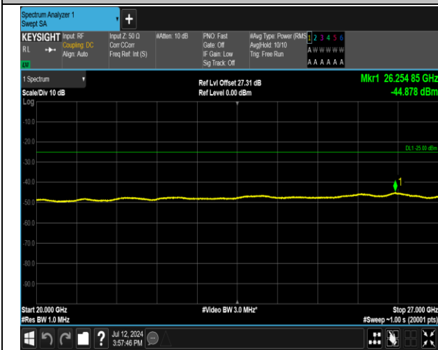
7-7-20MHz-15MHz-16QAM-16QAM-21026-21197-1RB#0-ORB#0-20000~27000MHz-PASS
