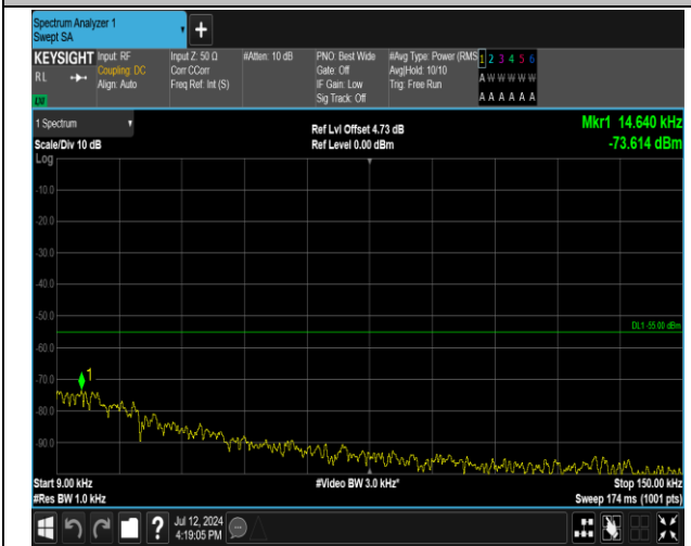
7-7-20MHz-15MHz-16QAM-16QAM-21201-21372-100RB #0-75RB#0-0.009~0.15MHz-PASS
