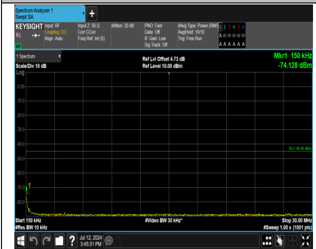
7-7-20MHz-15MHz-QPSK-QPSK-20850-21021-1RB#99-0 RB#0-0.15~30MHz-PASS
