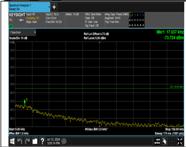
7-7-20MHz-15MHz-16QAM-16QAM-20850-21021-100RB #0-75RB#0-0.009~0.15MHz-PASS
