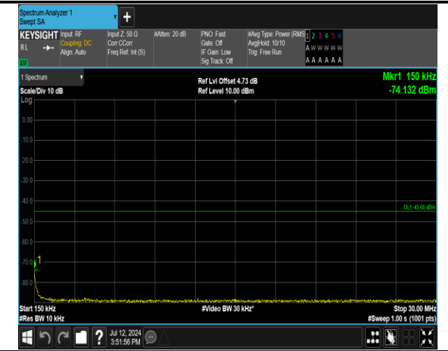
7-7-20MHz-15MHz-QPSK-QPSK-20850-21021-100RB#0-75RB#0-0.15~30MHz-PASS
