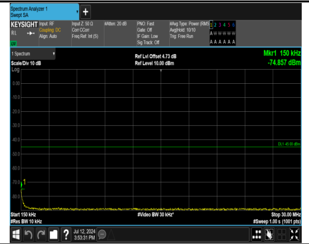
7-7-20MHz-15MHz-16QAM-16QAM-20850-21021-100RB# 0-75RB#0-0.15~30MHz-PASS
