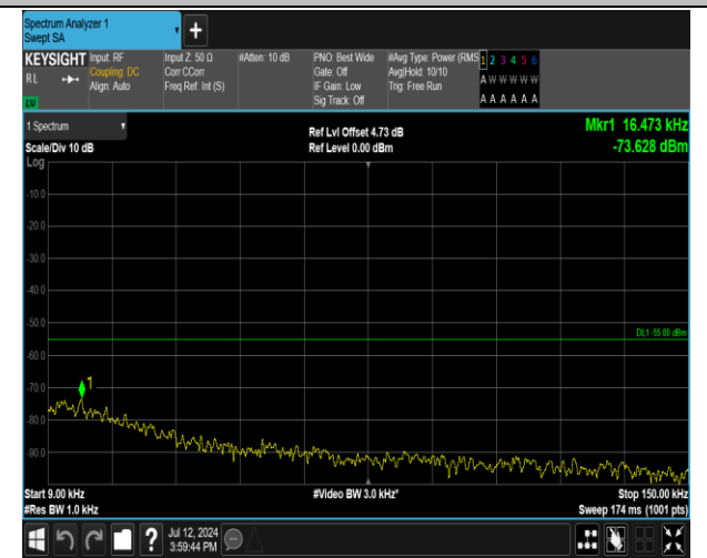
7-7-20MHz-15MHz-16QAM-16QAM-21026-21197-1RB#99-0RB#0-0.009~0.15MHz-PASS
