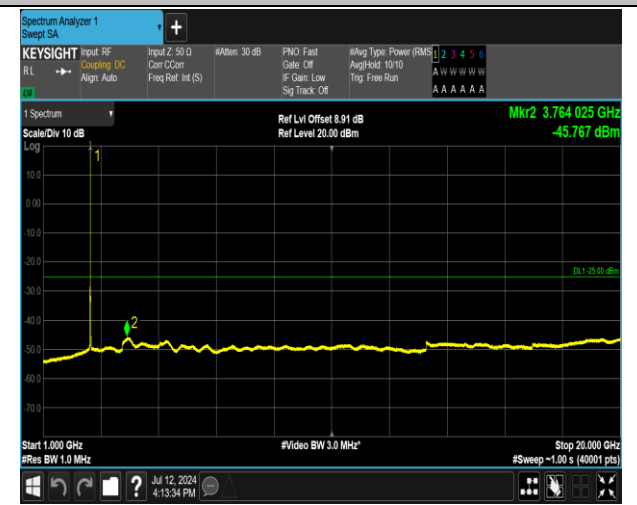
7-7-20MHz-15MHz-16QAM-16QAM-21201-21372-1RB#99-0RB#0-1000~20000MHz-PASS
