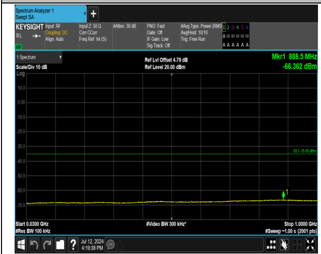
7-7-20MHz-15MHz-16QAM-16QAM-21201-21372-100RB #0-75RB#0-30~1000MHz-PASS
