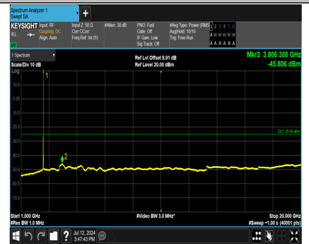
7-7-20MHz-15MHz-16QAM-16QAM-20850-21021-1RB#99-0RB#0-1000~20000MHz-PASS
