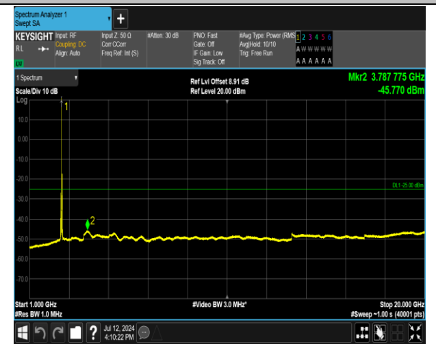
7-7-20MHz-15MHz-16QAM-16QAM-21201-21372-1RB#0- ORB#0-1000~20000MHz-PASS
