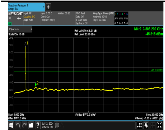
7-7-20MHz-15MHz-QPSK-QPSK-20850-21021-100RB#0-75RB#0-1000~20000MHz-PASS
