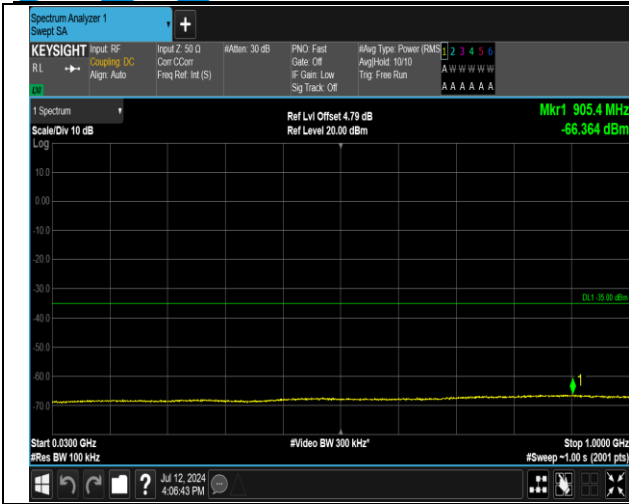
7-7-20MHz-15MHz-16QAM-16QAM-21026-21197-100RB#-0-75RB#0-30~1000MHz-PASS
