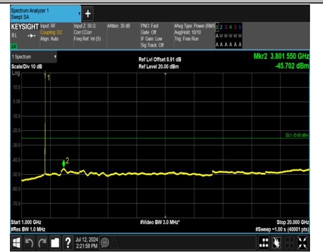
7-7-20MHz-10MHz-QPSK-QPSK-21251-21395-1RB#99-0 RB#0-1000~20000MHz-PASS
