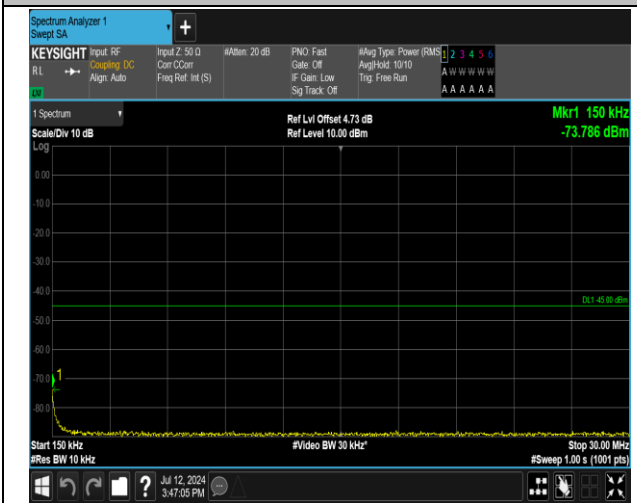
7-7-20MHz-15MHz-16QAM-16QAM-20850-21021-1RB#9-0RB#0-0.15~30MHz-PASS
