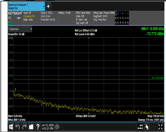
7-7-20MHz-15MHz-QPSK-QPSK-21026-21197-1RB#0-1R B#74-0.009~0.15MHz-PASS
