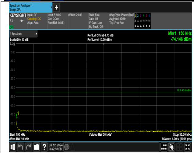
7-7-20MHz-15MHz-QPSK-QPSK-20850-21021-1RB#0-0R B#0-0.15~30MHz-PASS
