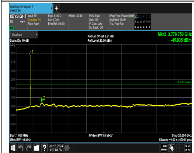
7-7-20MHz-15MHz-16QAM-16QAM-21026-21197-100RB# 0-75RB#0-1000~20000MHz-PASS
