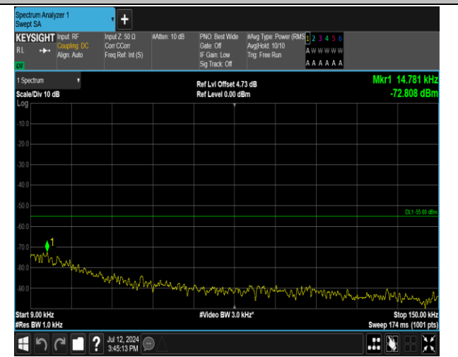
7-7-20MHz-15MHz-QPSK-QPSK-20850-21021-1RB#99-0 RB#0-0.009~0.15MHz-PASS
