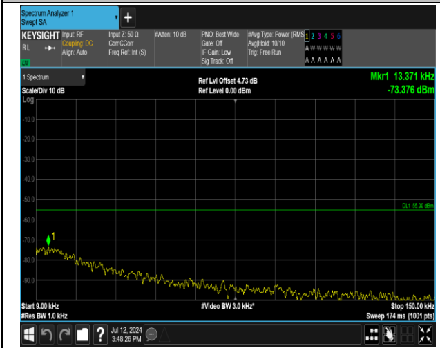
7-7-20MHz-15MHz-QPSK-QPSK-20850-21021-1RB#0-1R B#74-0.009~0.15MHz-PASS
