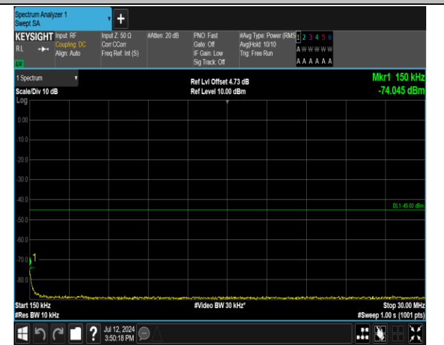
7-7-20MHz-15MHz-16QAM-16QAM-20850-21021-1RB#0-1RB#74-0.15~30MHz-PASS
