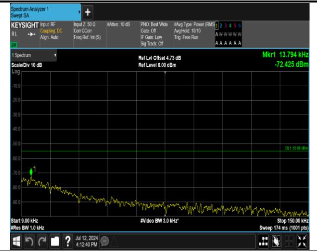
7-7-20MHz-15MHz-16QAM-16QAM-21201-21372-1RB#99-0RB#0-0.009~0.15MHz-PASS
