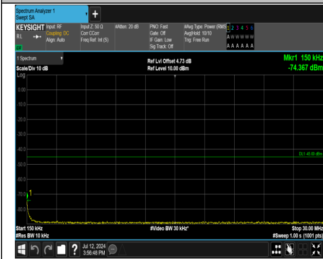
7-7-20MHz-15MHz-16QAM-16QAM-21026-21197-1RB#0-ORB#0-0.15~30MHz-PASS
