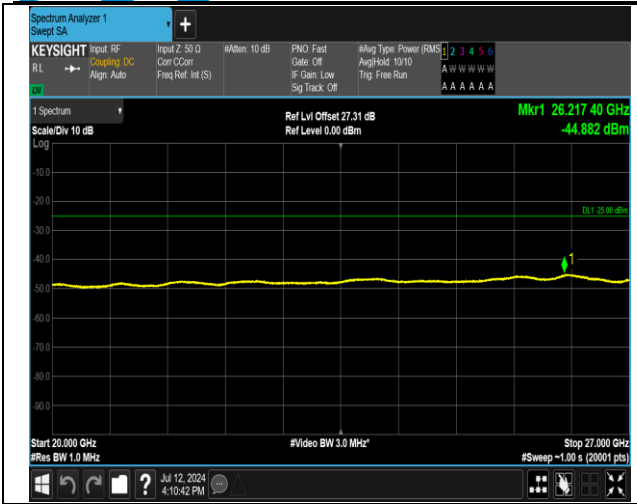
7-7-20MHz-15MHz-16QAM-16QAM-21201-21372-1RB#0-ORB#0-20000~27000MHz-PASS
