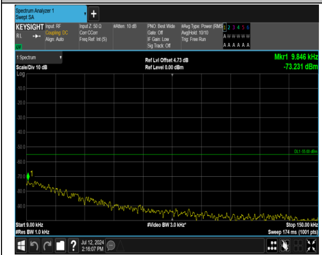
7-7-20MHz-10MHz-16QAM-16QAM-21051-21195-100RB# 0-50RB#0-0.009~0.15MHz-PASS
