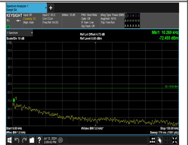
7-7-20MHz-10MHz-16QAM-16QAM-21051-21195-1RB#99-0RB#0-0.009~0.15MHz-PASS
