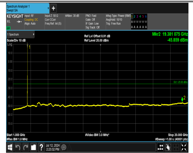
7-7-20MHz-10MHz-16QAM-16QAM-21251-21395-1RB#99-0RB#0-1000~20000MHz-PASS
