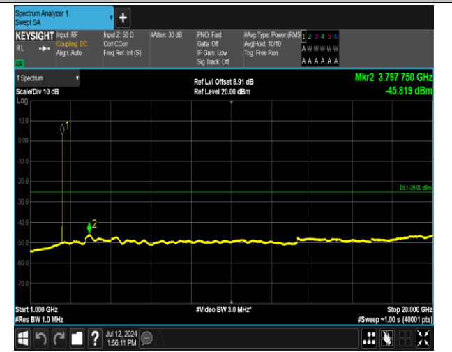
7-7-20MHz-10MHz-QPSK-QPSK-20850-20994-1RB#99-0 RB#0-1000~20000MHz-PASS
