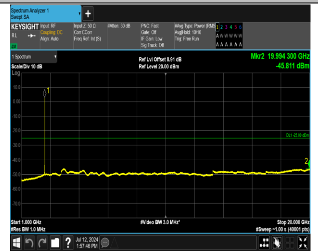
7-7-20MHz-10MHz-16QAM-16QAM-20850-20994-1RB#99-0RB#0-1000~20000MHz-PASS
