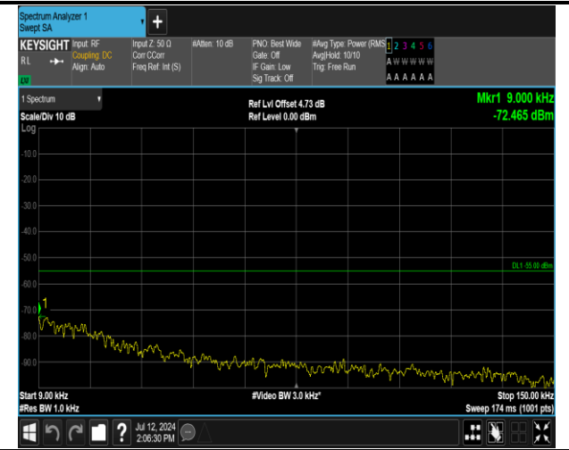
7-7-20MHz-10MHz-16QAM-16QAM-21051-21195-1RB#0-ORB#0-0.009~0.15MHz-PASS
