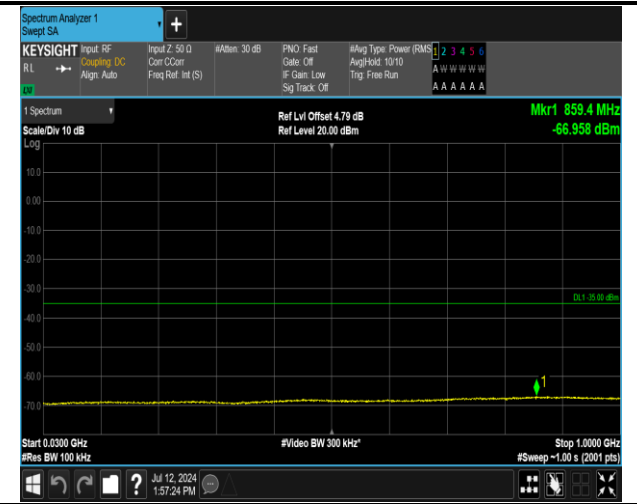
7-7-20MHz-10MHz-16QAM-16QAM-20850-20994-1RB#99 -0RB#0-30~1000MHz-PASS
