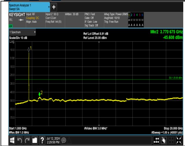
7-7-20MHz-10MHz-16QAM-16QAM-21251-21395-100RB #0-50RB#0-1000~20000MHz-PASS
