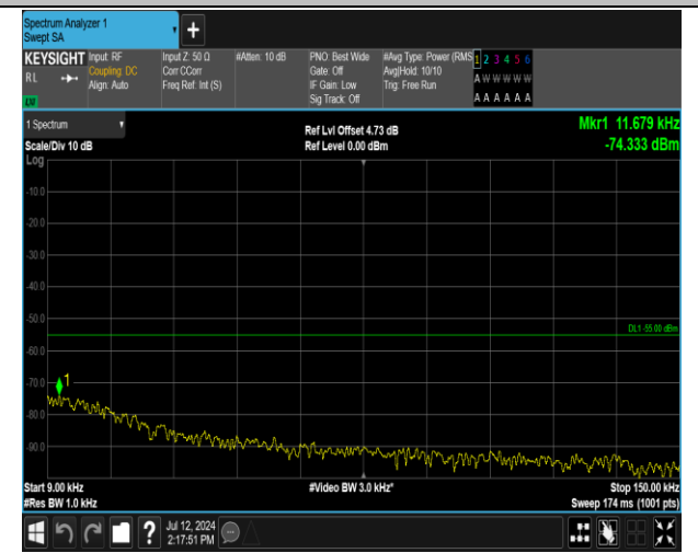
7-7-20MHz-10MHz-QPSK-QPSK-21251-21395-1RB#0-0RB#0-0.009~0.15MHz-PASS
