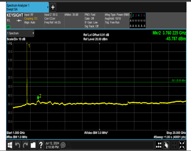
7-7-20MHz-10MHz-16QAM-16QAM-21051-21195-1RB#99 -ORB#0-1000~20000MHz-PASS
