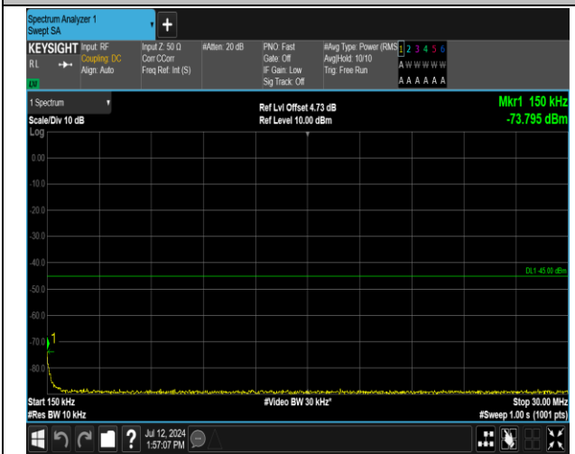
7-7-20MHz-10MHz-16QAM-16QAM-20850-20994-1RB#9-0RB#0-0.15~30MHz-PASS
