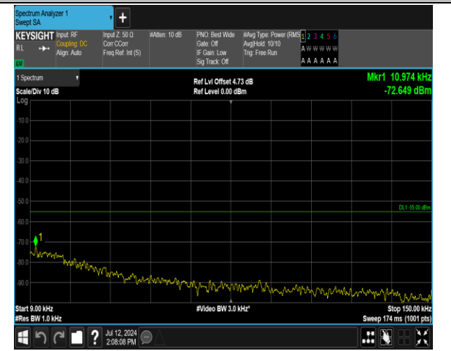
7-7-20MHz-10MHz-QPSK-QPSK-21051-21195-1RB#99-0 RB#0-0.009~0.15MHz-PASS
