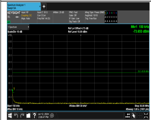
7-7-20MHz-10MHz-16QAM-16QAM-21051-21195-1RB#0-ORB#0-0.15~30MHz-PASS
