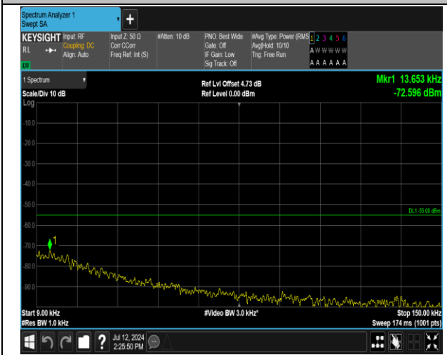
7-7-20MHz-10MHz-16QAM-16QAM-21251-21395-1RB#0-1RB#49-0.009~0.15MHz-PASS
