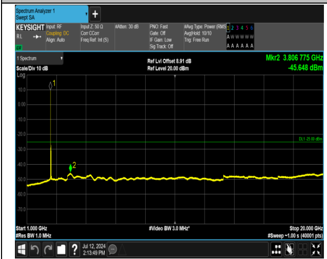
7-7-20MHz-10MHz-16QAM-16QAM-21051-21195-1RB#0-1RB#49-1000~20000MHz-PASS
