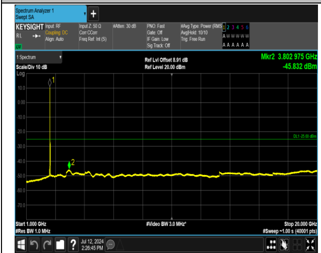
7-7-20MHz-10MHz-16QAM-16QAM-21251-21395-1RB#0-1RB#49-1000~20000MHz-PASS
