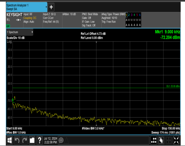
7-7-20MHz-10MHz-16QAM-16QAM-21251-21395-1RB#99-0RB#0-0.009~0.15MHz-PASS
