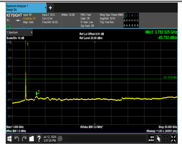
7-7-20MHz-10MHz-16QAM-16QAM-21051-21195-1RB#0-ORB#0-1000~20000MHz-PASS
