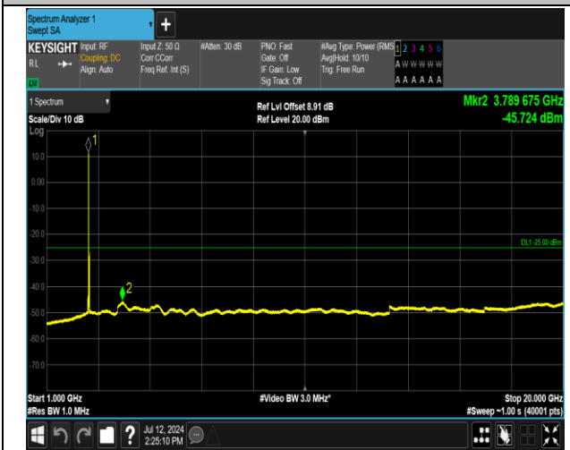
7-7-20MHz-10MHz-QPSK-QPSK-21251-21395-1RB#0-1R B#49-1000~20000MHz-PASS
