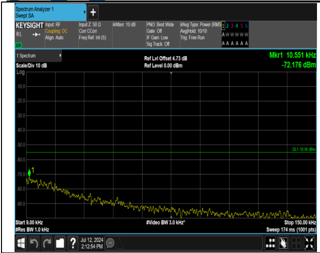
7-7-20MHz-10MHz-16QAM-16QAM-21051-21195-1RB#0-1RB#49-0.009~0.15MHz-PASS
