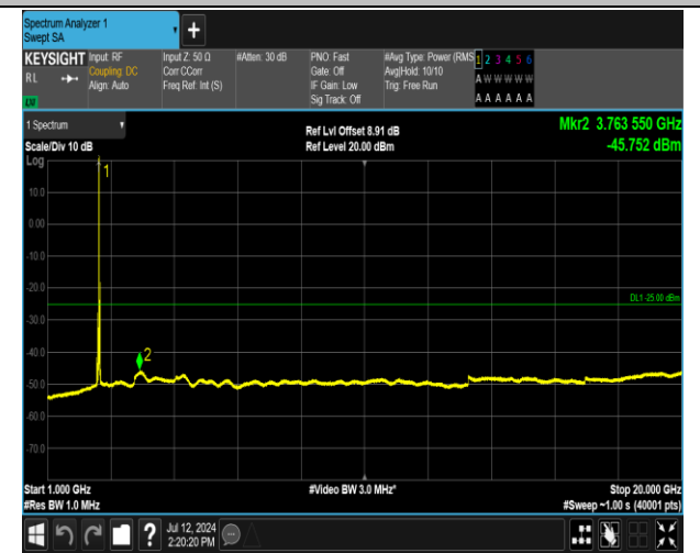
7-7-20MHz-10MHz-16QAM-16QAM-21251-21395-1RB#0- ORB#0-1000~20000MHz-PASS
