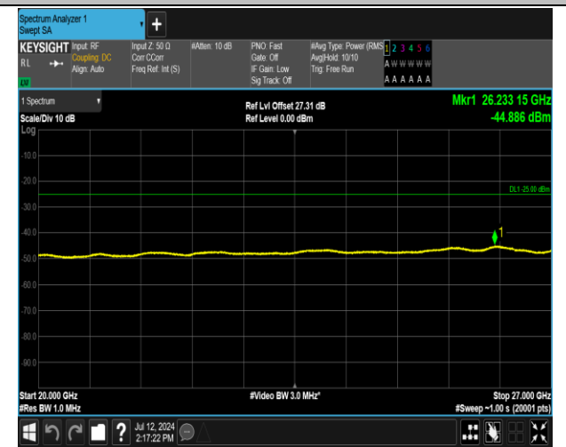
7-7-20MHz-10MHz-16QAM-16QAM-21051-21195-100RB# 0-50RB#0-20000~27000MHz-PASS
