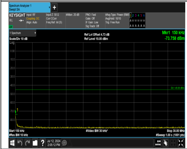
7-7-20MHz-10MHz-QPSK-QPSK-21051-21195-1RB#0-0RB#0-0.15~30MHz-PASS
