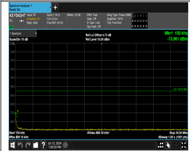
7-7-20MHz-10MHz-QPSK-QPSK-20850-20994-1RB#99-0 RB#0-0.15~30MHz-PASS
