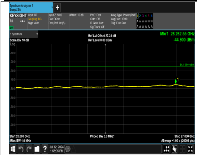
7-7-20MHz-10MHz-16QAM-16QAM-20850-20994-1RB#9 9-0RB#0-20000~27000MHz-PASS
