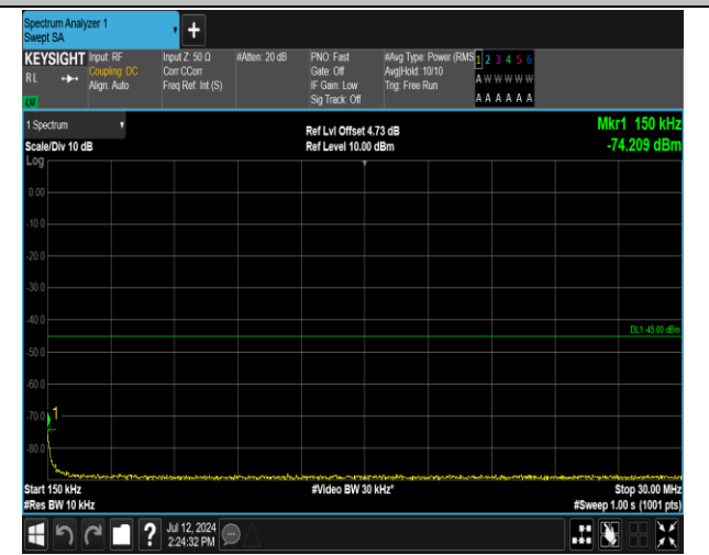
7-7-20MHz-10MHz-QPSK-QPSK-21251-21395-1RB#0-1R B#49-0.15~30MHz-PASS
