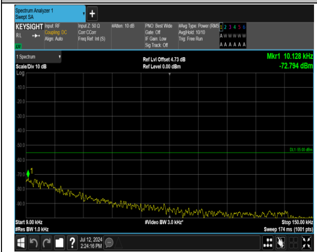
7-7-20MHz-10MHz-QPSK-QPSK-21251-21395-1RB#0-1R B#49-0.009~0.15MHz-PASS
