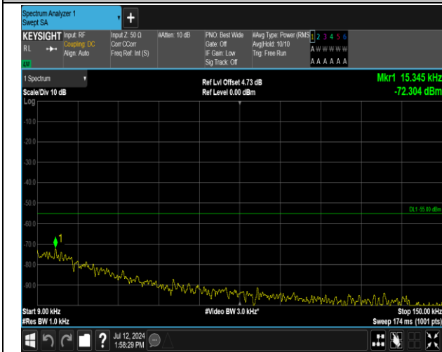
7-7-20MHz-10MHz-QPSK-QPSK-20850-20994-1RB#0-1R B#49-0.009~0.15MHz-PASS
