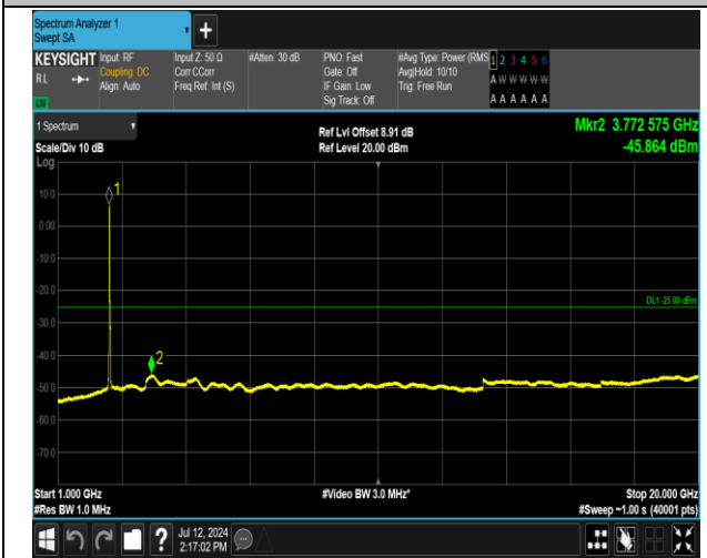
7-7-20MHz-10MHz-16QAM-16QAM-21051-21195-100RB# 0-50RB#0-1000~20000MHz-PASS
