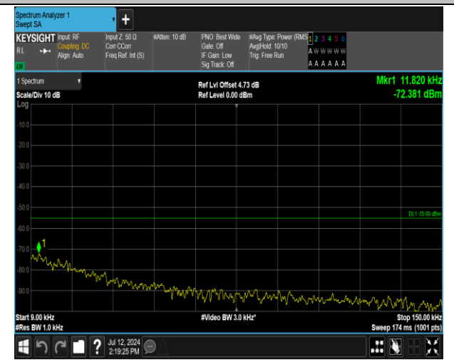
7-7-20MHz-10MHz-16QAM-16QAM-21251-21395-1RB#0- ORB#0-0.009~0.15MHz-PASS
