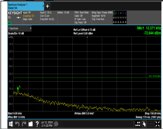
7-7-20MHz-10MHz-QPSK-QPSK-21051-21195-1RB#0-1R B#49-0.009~0.15MHz-PASS
