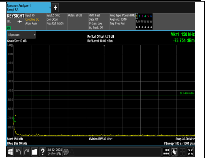
7-7-20MHz-10MHz-16QAM-16QAM-21051-21195-1RB#0-1RB#49-0.15~30MHz-PASS
