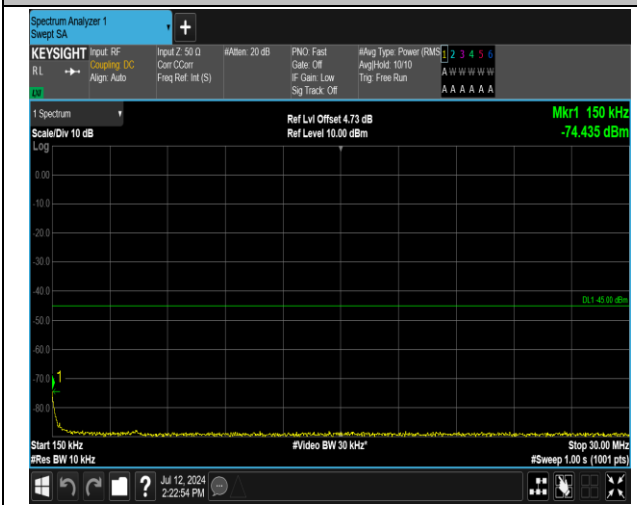
7-7-20MHz-10MHz-16QAM-16QAM-21251-21395-1RB#9-9-0RB#0-0.15~30MHz-PASS
