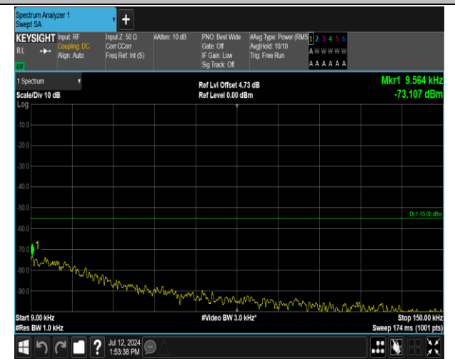
7-7-20MHz-10MHz-16QAM-16QAM-20850-20994-1RB#0- ORB#0-0.009~0.15MHz-PASS
