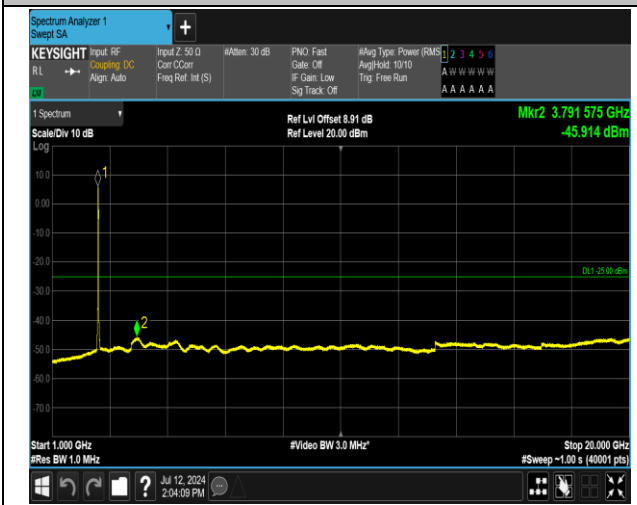
7-7-20MHz-10MHz-16QAM-16QAM-20850-20994-100RB #0-50RB#0-1000~20000MHz-PASS
