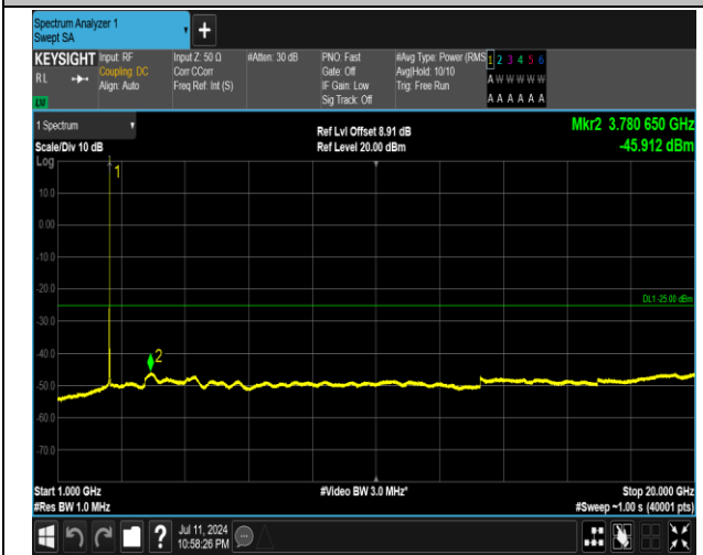
7-7-15MHz-20MHz-16QAM-16QAM-21179-21350-1RB#74-0RB#0-1000~20000MHz-PASS
