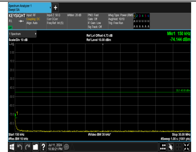
7-7-15MHz-20MHz-QPSK-QPSK-20828-20999-1RB#74-0 RB#0-0.15~30MHz-PASS
