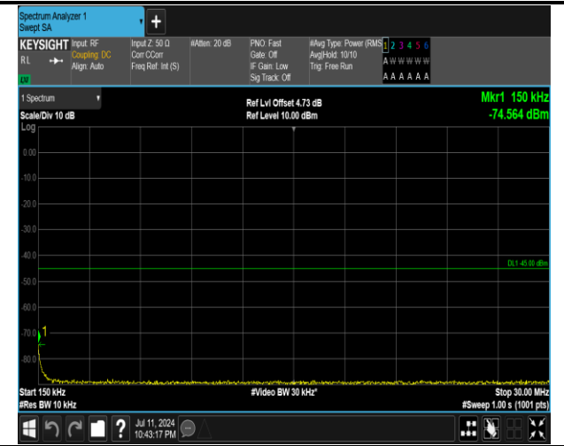
7-7-15MHz-20MHz-QPSK-QPSK-21003-21174-1RB#74-0 RB#0-0.15~30MHz-PASS
