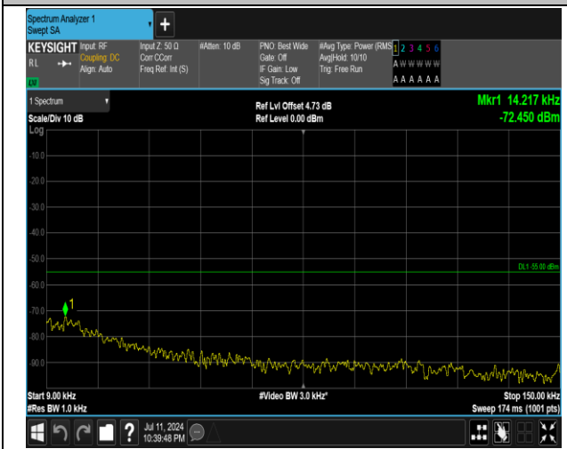
7-7-15MHz-20MHz-QPSK-QPSK-21003-21174-1RB#0-0R B#0-0.009~0.15MHz-PASS
