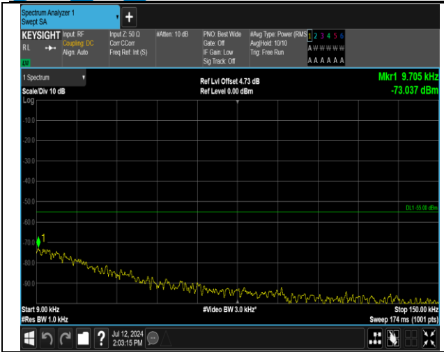
7-7-20MHz-10MHz-16QAM-16QAM-20850-20994-100RB #0-50RB#0-0.009~0.15MHz-PASS
