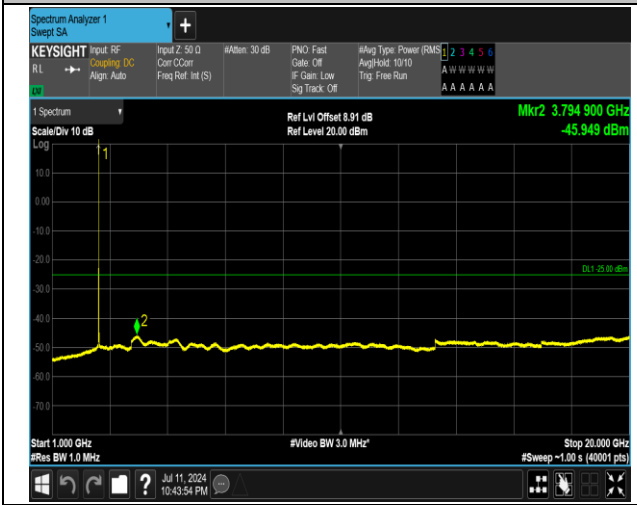
7-7-15MHz-20MHz-QPSK-QPSK-21003-21174-1RB#74-0 RB#0-1000~20000MHz-PASS
