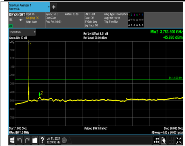
7-7-15MHz-20MHz-QPSK-QPSK-21179-21350-1RB#0-0R B#0-1000~20000MHz-PASS
