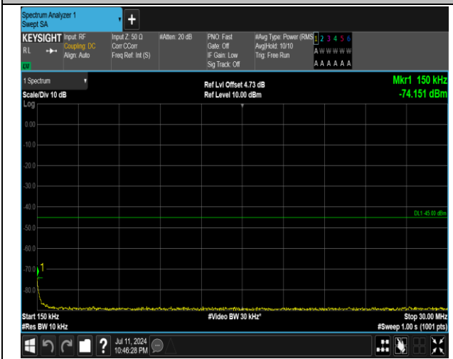
7-7-15MHz-20MHz-QPSK-QPSK-21003-21174-1RB#0-1R B#99-0.15~30MHz-PASS
