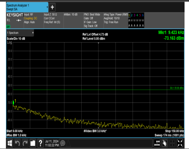
7-7-15MHz-20MHz-QPSK-QPSK-21179-21350-75RB#0-10 ORB#0-0.009~0.15MHz-PASS
