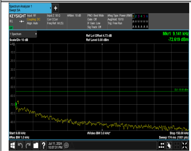
7-7-15MHz-20MHz-16QAM-16QAM-21179-21350-1RB#74-0RB#0-0.009~0.15MHz-PASS
