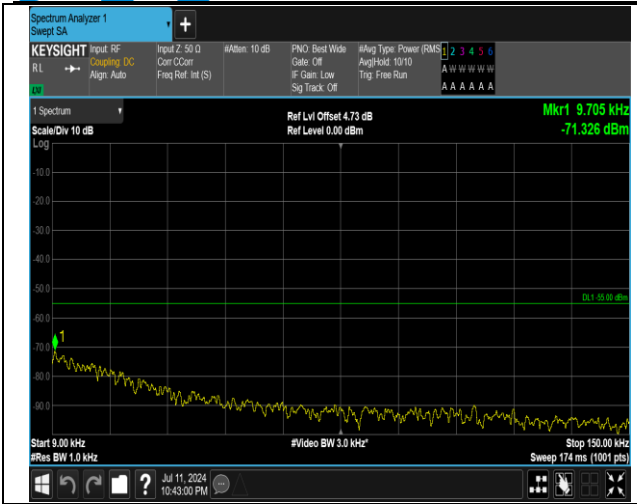
7-7-15MHz-20MHz-QPSK-QPSK-21003-21174-1RB#74-0 RB#0-0.009~0.15MHz-PASS
