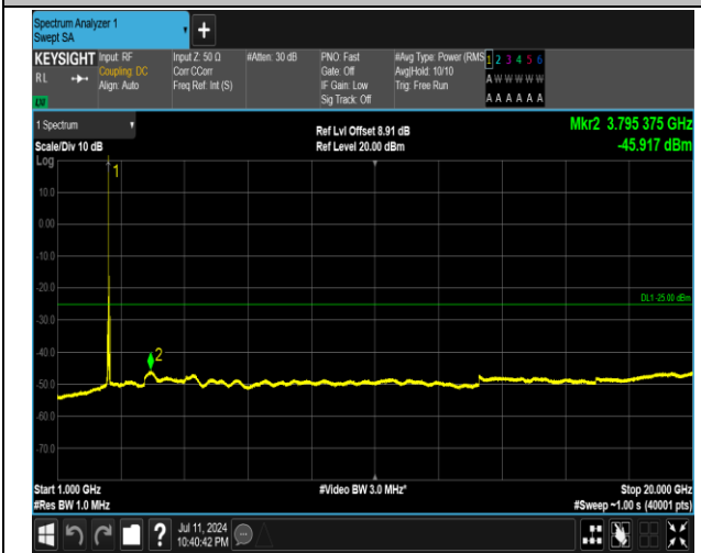
7-7-15MHz-20MHz-QPSK-QPSK-21003-21174-1RB#0-0R B#0-1000~20000MHz-PASS
