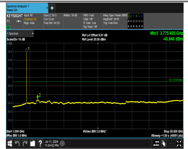
7-7-15MHz-20MHz-16QAM-16QAM-21179-21350-75RB#0 -100RB#0-1000~20000MHz-PASS
