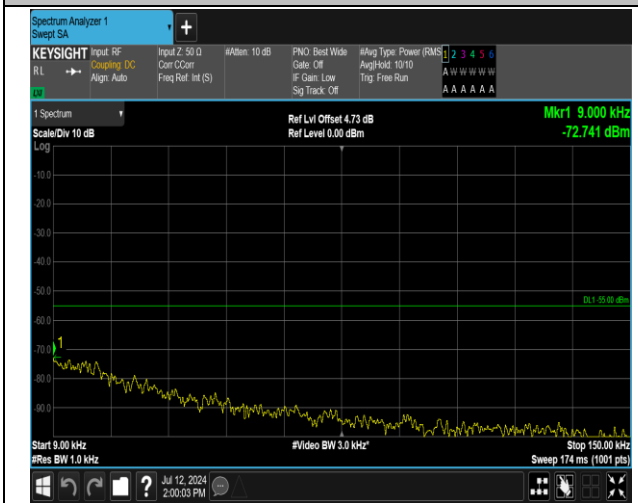
7-7-20MHz-10MHz-16QAM-16QAM-20850-20994-1RB#0-1RB#49-0.009~0.15MHz-PASS
