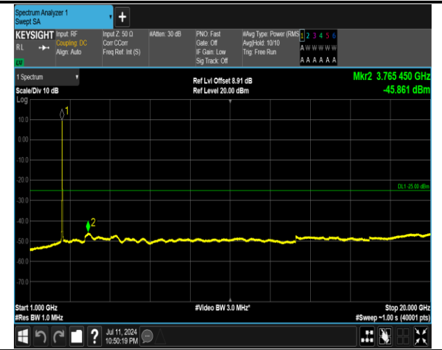
7-7-15MHz-20MHz-QPSK-QPSK-21003-21174-75RB#0-10 0RB#0-1000~20000MHz-PASS
