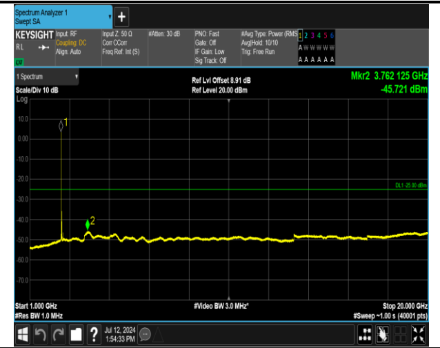
7-7-20MHz-10MHz-16QAM-16QAM-20850-20994-1RB#0-ORB#0-1000~20000MHz-PASS
