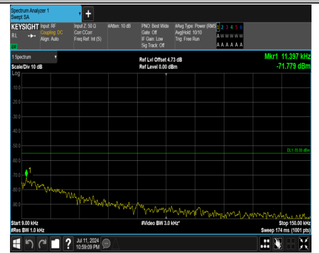
7-7-15MHz-20MHz-QPSK-QPSK-21179-21350-1RB#0-1R B#99-0.009~0.15MHz-PASS
