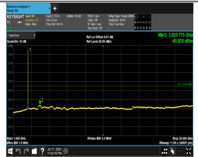
7-7-15MHz-20MHz-QPSK-QPSK-21179-21350-75RB#0-10 ORB#0-1000~20000MHz-PASS
