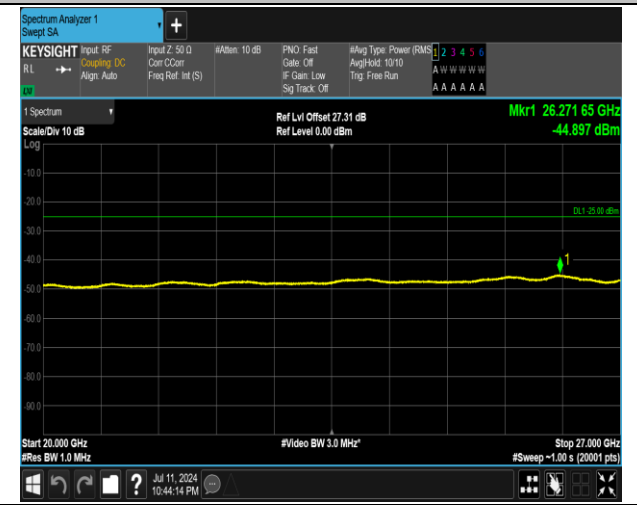
7-7-15MHz-20MHz-QPSK-QPSK-21003-21174-1RB#74-0 RB#0-20000~27000MHz-PASS
