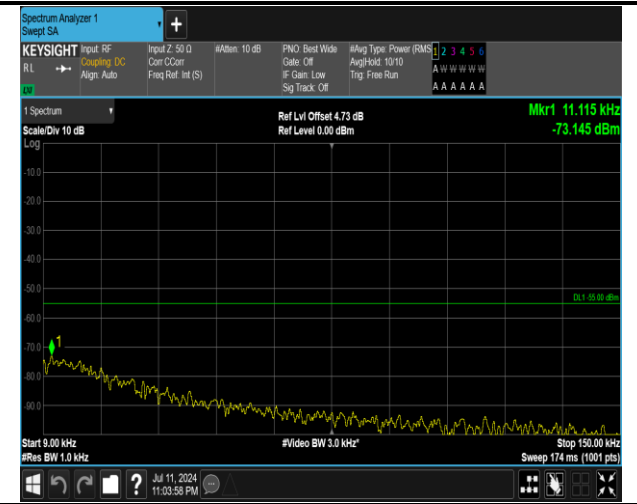
7-7-15MHz-20MHz-16QAM-16QAM-21179-21350-75RB#0 -100RB#0-0.009~0.15MHz-PASS
