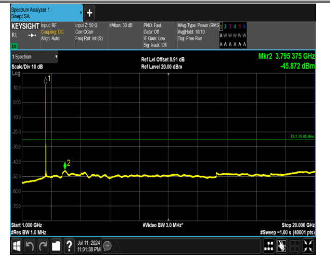
7-7-15MHz-20MHz-16QAM-16QAM-21179-21350-1RB#0-1RB#99-1000~20000MHz-PASS
