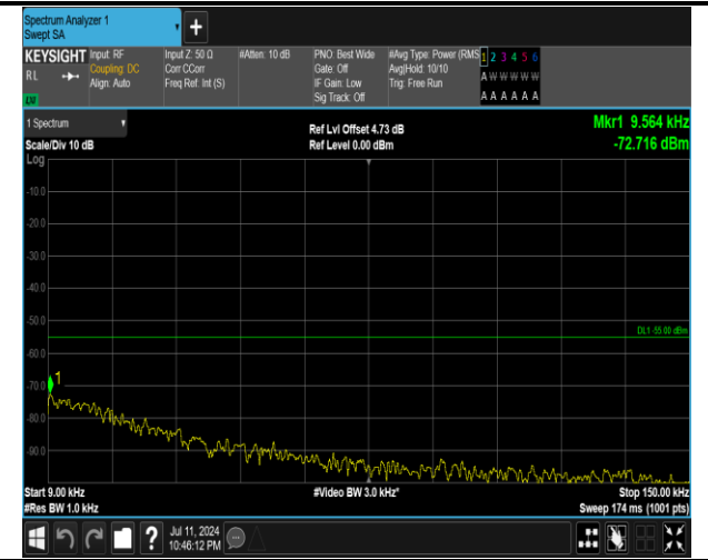
7-7-15MHz-20MHz-QPSK-QPSK-21003-21174-1RB#0-1R B#99-0.009~0.15MHz-PASS
