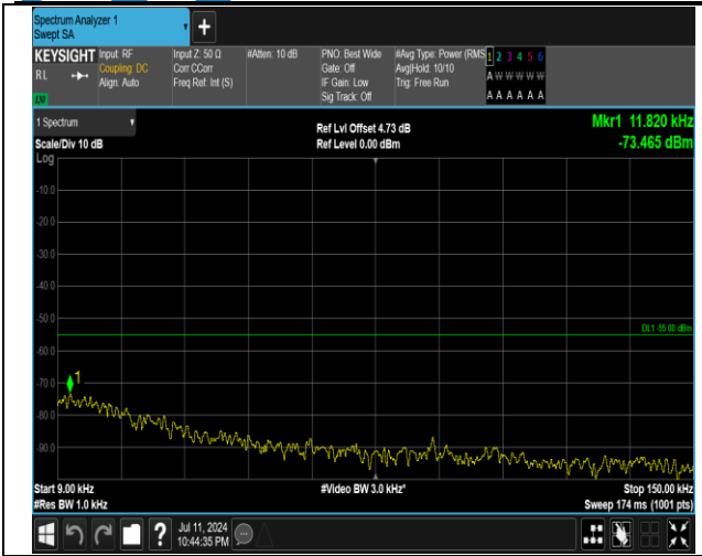
7-7-15MHz-20MHz-16QAM-16QAM-21003-21174-1RB#74 -ORB#0-0.009~0.15MHz-PASS
