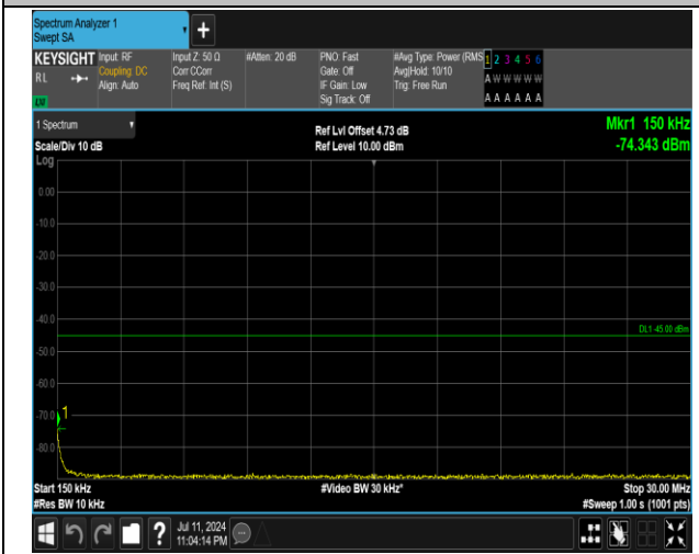
7-7-15MHz-20MHz-16QAM-16QAM-21179-21350-75RB#0 -100RB#0-0.15~30MHz-PASS
