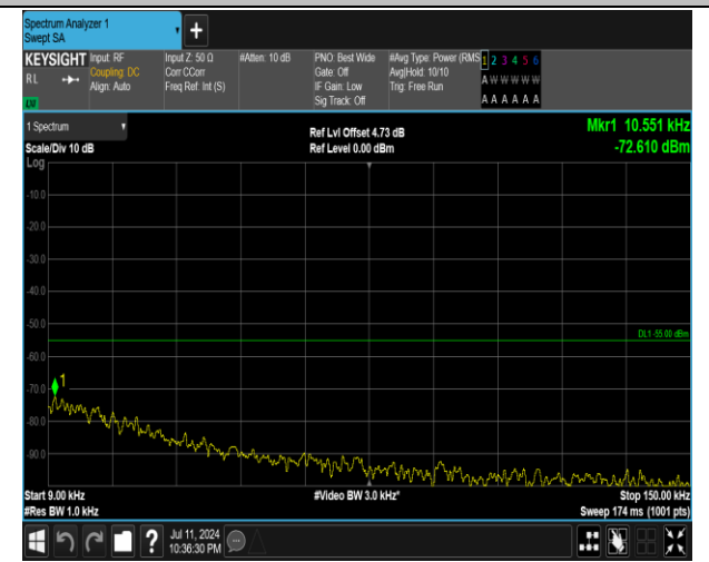
7-7-15MHz-20MHz-QPSK-QPSK-20828-20999-75RB#0-10 ORB#0-0.009~0.15MHz-PASS
