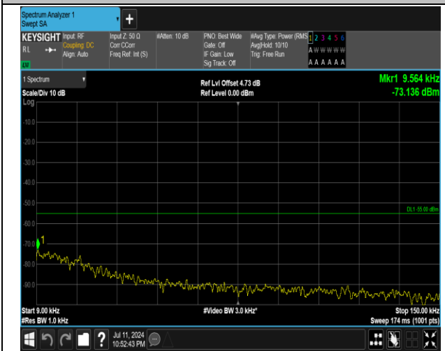
7-7-15MHz-20MHz-QPSK-QPSK-21179-21350-1RB#0-0R B#0-0.009~0.15MHz-PASS
