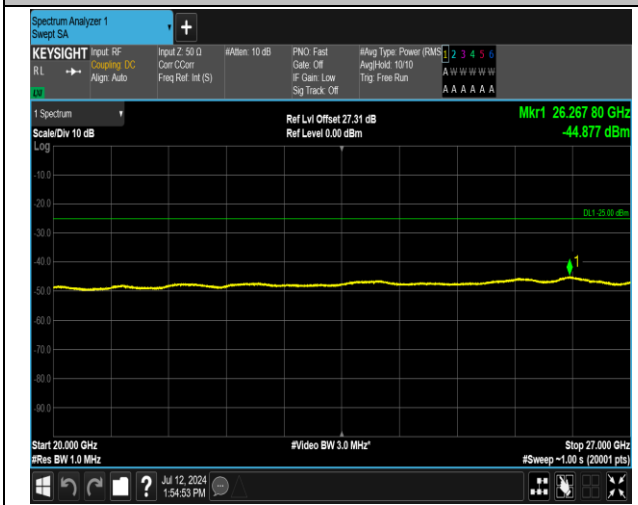
7-7-20MHz-10MHz-16QAM-16QAM-20850-20994-1RB#0-ORB#0-20000~27000MHz-PASS
