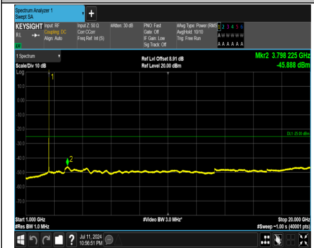
7-7-15MHz-20MHz-QPSK-QPSK-21179-21350-1RB#74-0 RB#0-1000~20000MHz-PASS
