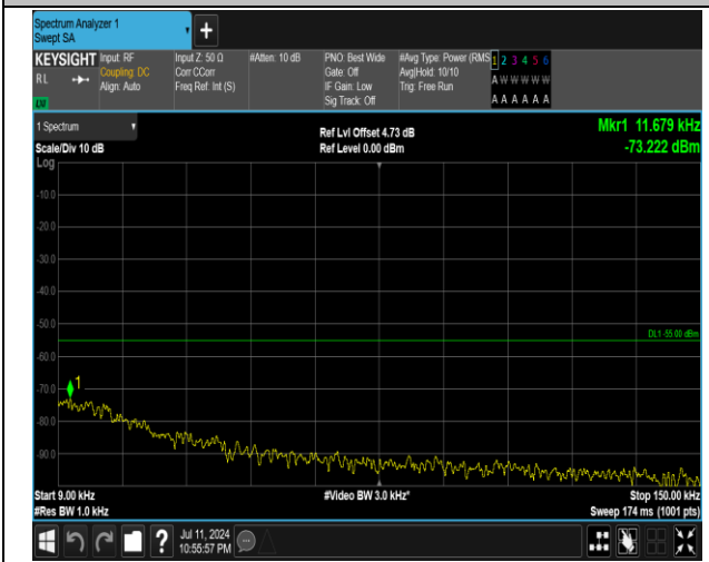
7-7-15MHz-20MHz-QPSK-QPSK-21179-21350-1RB#74-0 RB#0-0.009~0.15MHz-PASS
