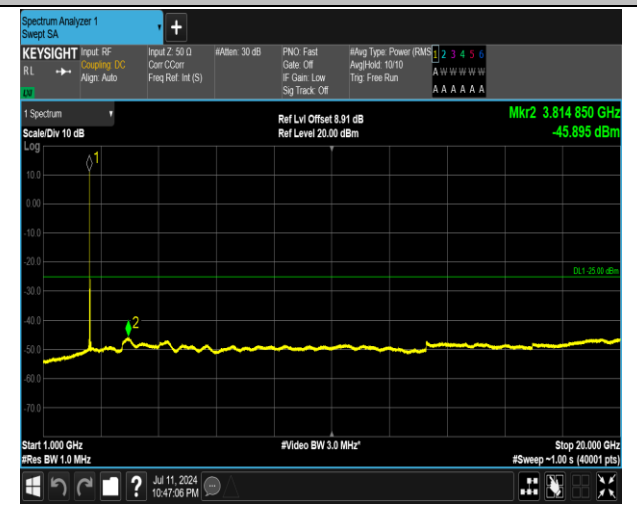
7-7-15MHz-20MHz-QPSK-QPSK-21003-21174-1RB#0-1R B#99-1000~20000MHz-PASS
