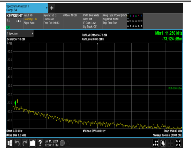
7-7-15MHz-20MHz-QPSK-QPSK-20828-20999-1RB#0-1R B#99-0.009~0.15MHz-PASS
