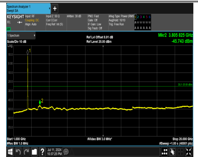
7-7-15MHz-20MHz-QPSK-QPSK-20828-20999-75RB#0-10 ORB#0-1000~20000MHz-PASS
