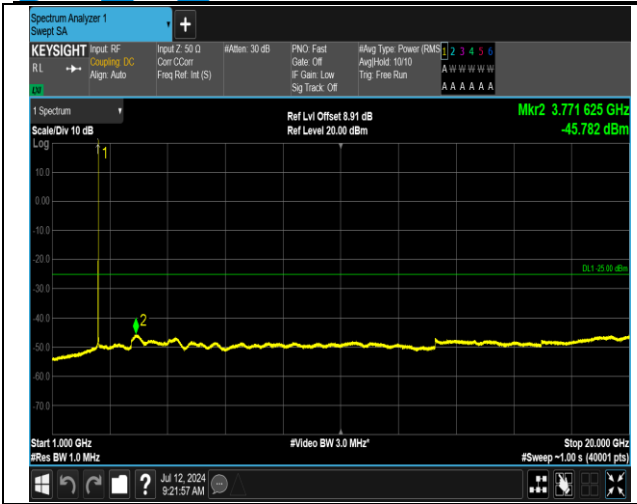
7-7-15MHz-15MHz-QPSK-QPSK-20825-20975-1RB#74-0 RB#0-1000~20000MHz-PASS
