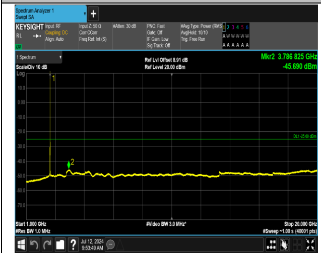
7-7-15MHz-15MHz-16QAM-16QAM-21225-21375-1RB#74-0-ORB#0-1000~20000MHz-PASS
