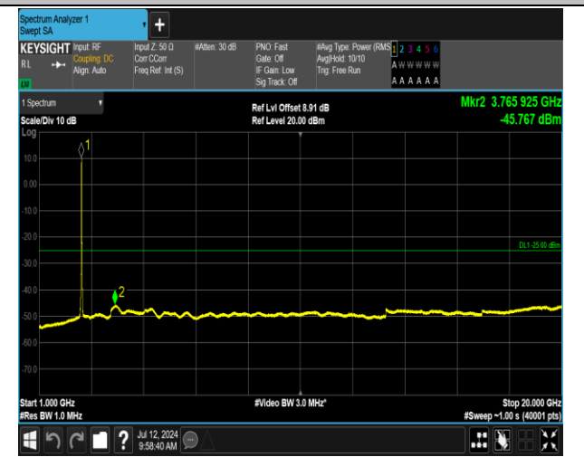
7-7-15MHz-15MHz-QPSK-QPSK-21225-21375-75RB#0-75 RB#0-1000~20000MHz-PASS
