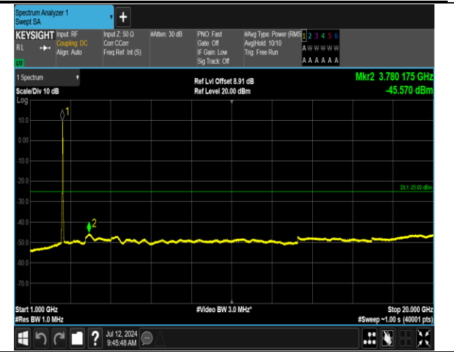
7-7-15MHz-15MHz-QPSK-QPSK-21025-21175-75RB#0-75 RB#0-1000~20000MHz-PASS
