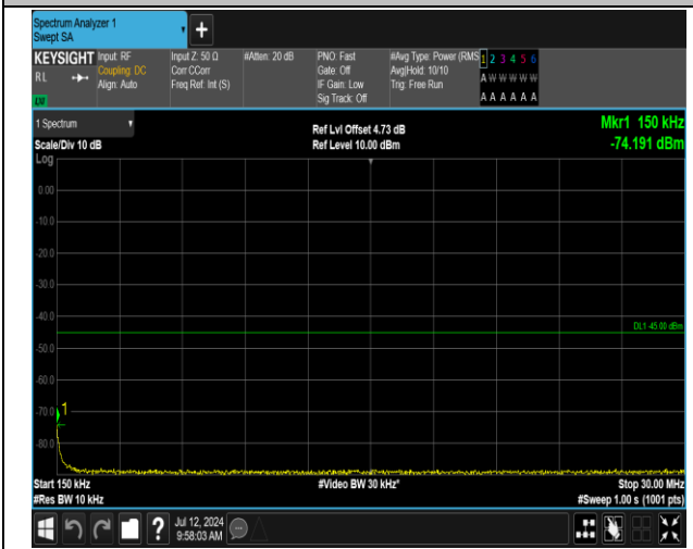
7-7-15MHz-15MHz-QPSK-QPSK-21225-21375-75RB#0-7 5RB#0-0.15~30MHz-PASS
