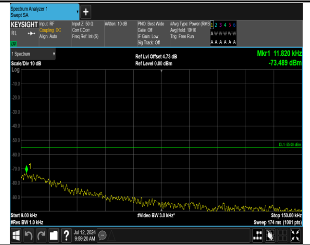
7-7-15MHz-15MHz-16QAM-16QAM-21225-21375-75RB#0 -75RB#0-0.009~0.15MHz-PASS
