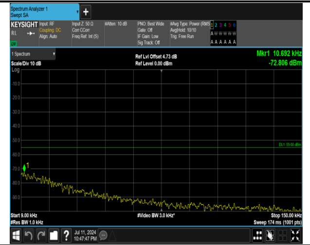
7-7-15MHz-20MHz-16QAM-16QAM-21003-21174-1RB#0-1RB#99-0.009~0.15MHz-PASS
