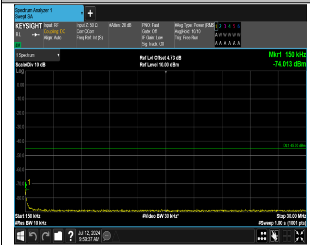
7-7-15MHz-15MHz-16QAM-16QAM-21225-21375-75RB#0 0-75RB#0-0.15~30MHz-PASS
