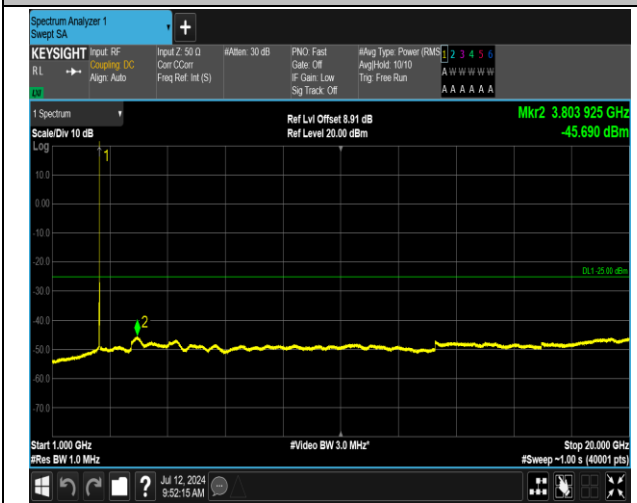
7-7-15MHz-15MHz-QPSK-QPSK-21225-21375-1RB#74-0 RB#0-1000~20000MHz-PASS
