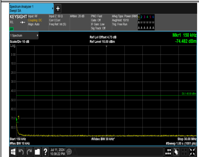
7-7-15MHz-20MHz-16QAM-16QAM-20828-20999-75RB#0 0-100RB#0-0.15~30MHz-PASS
