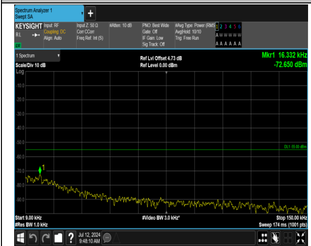
7-7-15MHz-15MHz-QPSK-QPSK-21225-21375-1RB#0-0R B#0-0.009~0.15MHz-PASS
