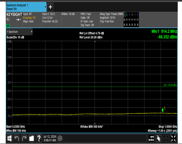
7-7-15MHz-15MHz-16QAM-16QAM-21225-21375-1RB#0-1RB#74-30~1000MHz-PASS
