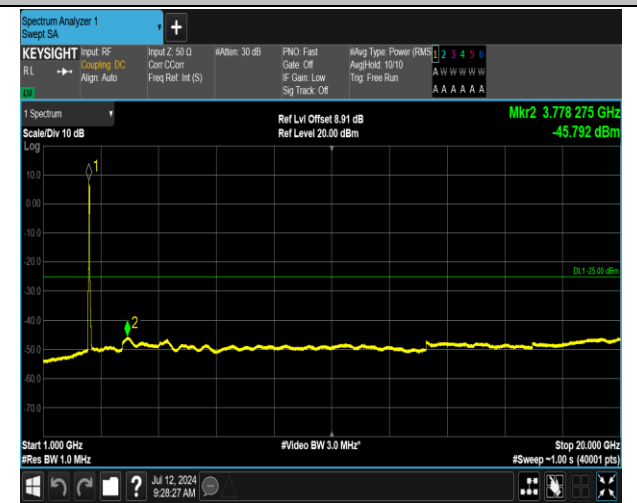
7-7-15MHz-15MHz-QPSK-QPSK-20825-20975-75RB#0-75 RB#0-1000~20000MHz-PASS
