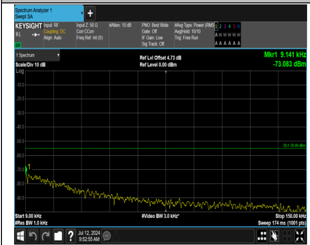
7-7-15MHz-15MHz-16QAM-16QAM-21225-21375-1RB#74-0-ORB#0-0.009~0.15MHz-PASS
