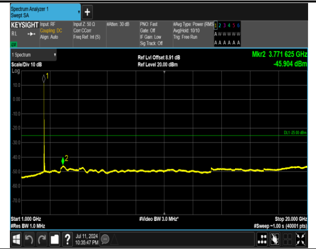
7-7-15MHz-20MHz-16QAM-16QAM-20828-20999-1RB#0-1RB#99-1000~20000MHz-PASS
