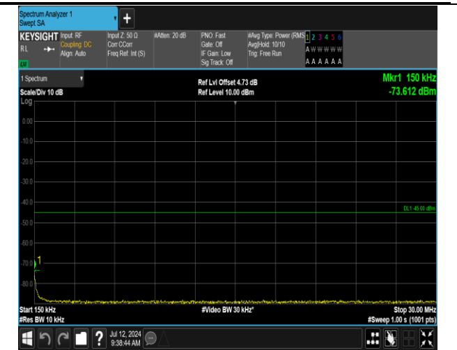
7-7-15MHz-15MHz-QPSK-QPSK-21025-21175-1RB#74-0 RB#0-0.15~30MHz-PASS
