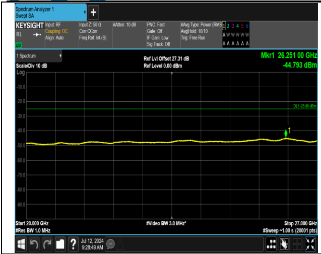
7-7-15MHz-15MHz-QPSK-QPSK-20825-20975-75RB#0-7 5RB#0-20000~27000MHz-PASS
