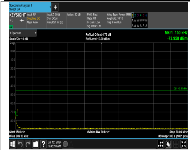
7-7-15MHz-15MHz-QPSK-QPSK-21025-21175-75RB#0-7 5RB#0-0.15~30MHz-PASS
