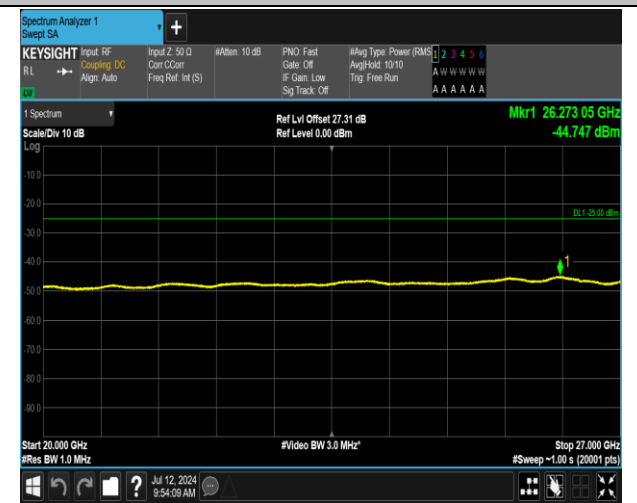
7-7-15MHz-15MHz-16QAM-16QAM-21225-21375-1RB#74-0-ORB#0-20000~27000MHz-PASS
