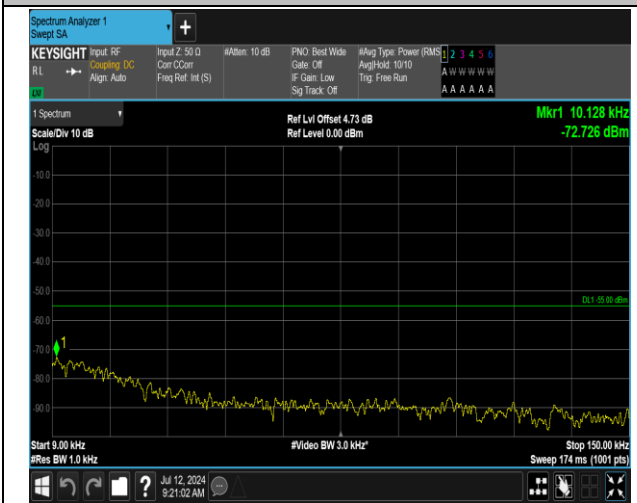
7-7-15MHz-15MHz-QPSK-QPSK-20825-20975-1RB#74-0 RB#0-0.009~0.15MHz-PASS
