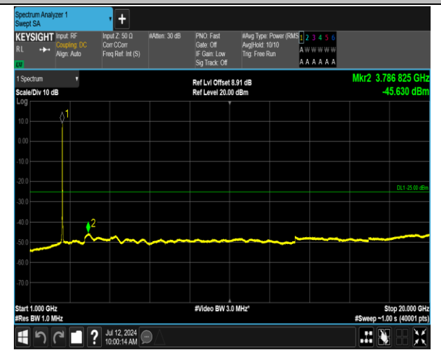
7-7-15MHz-15MHz-16QAM-16QAM-21225-21375-75RB#0 -75RB#0-1000~20000MHz-PASS
