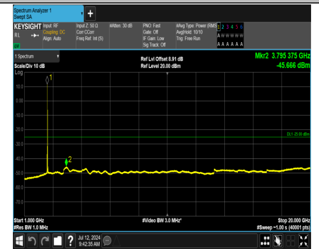
7-7-15MHz-15MHz-QPSK-QPSK-21025-21175-1RB#0-1R B#74-1000~20000MHz-PASS
