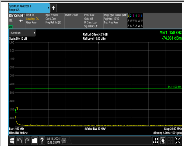
7-7-15MHz-20MHz-16QAM-16QAM-21003-21174-1RB#0-1RB#99-0.15~30MHz-PASS
