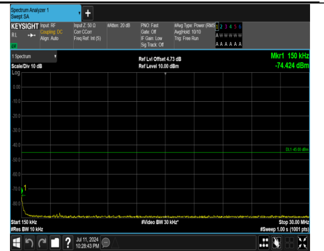
7-7-15MHz-20MHz-16QAM-16QAM-20828-20999-1RB#0-ORB#0-0.15~30MHz-PASS
