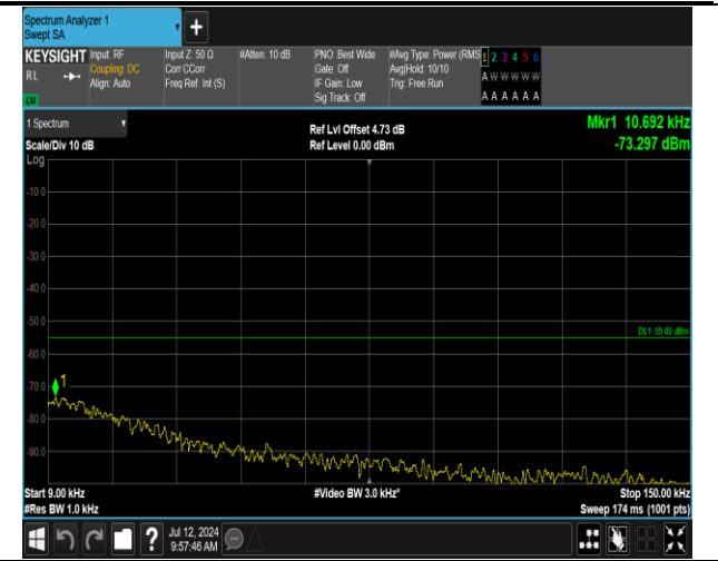
7-7-15MHz-15MHz-QPSK-QPSK-21225-21375-75RB#0-75 RB#0-0.009~0.15MHz-PASS
