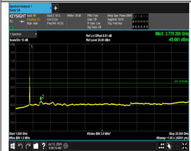
7-7-15MHz-15MHz-QPSK-QPSK-21025-21175-1RB#0-0R B#0-1000~20000MHz-PASS
