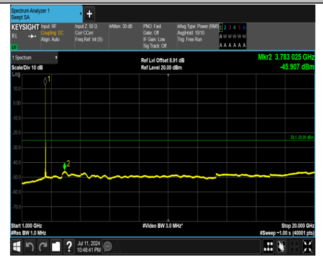
7-7-15MHz-20MHz-16QAM-16QAM-21003-21174-1RB#0-1RB#99-1000~20000MHz-PASS
