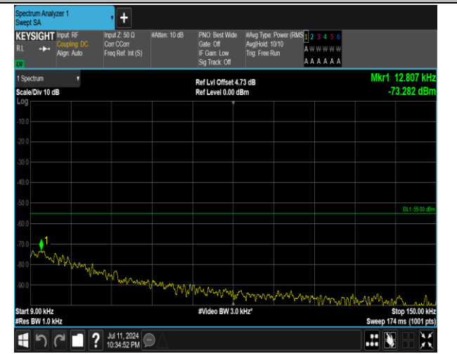
7-7-15MHz-20MHz-16QAM-16QAM-20828-20999-1RB#0-1RB#99-0.009~0.15MHz-PASS
