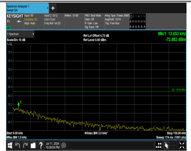
7-7-15MHz-20MHz-16QAM-16QAM-20828-20999-75RB#0 -100RB#0-0.009~0.15MHz-PASS
