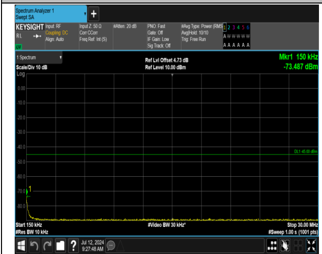
7-7-15MHz-15MHz-QPSK-QPSK-20825-20975-75RB#0-7 5RB#0-0.15~30MHz-PASS
