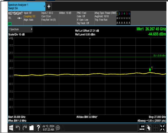
7-7-15MHz-15MHz-16QAM-16QAM-21225-21375-1RB#0-1RB#74-20000~27000MHz-PASS
