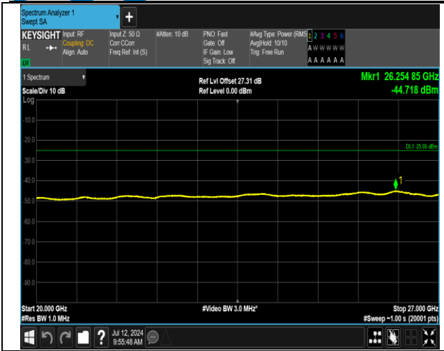
7-7-15MHz-15MHz-QPSK-QPSK-21225-21375-1RB#0-1R B#74-20000~27000MHz-PASS
