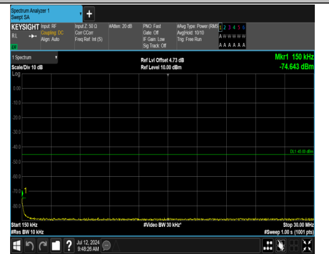
7-7-15MHz-15MHz-QPSK-QPSK-21225-21375-1RB#0-0R B#0-0.15~30MHz-PASS
