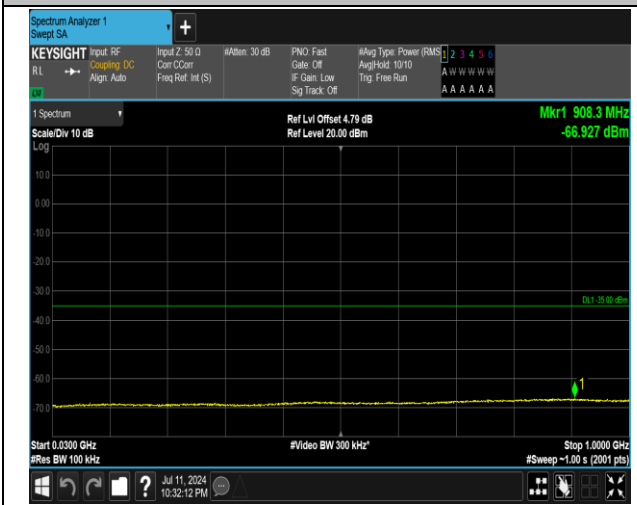
7-7-15MHz-20MHz-16QAM-16QAM-20828-20999-1RB#7 4-0RB#0-30~1000MHz-PASS
