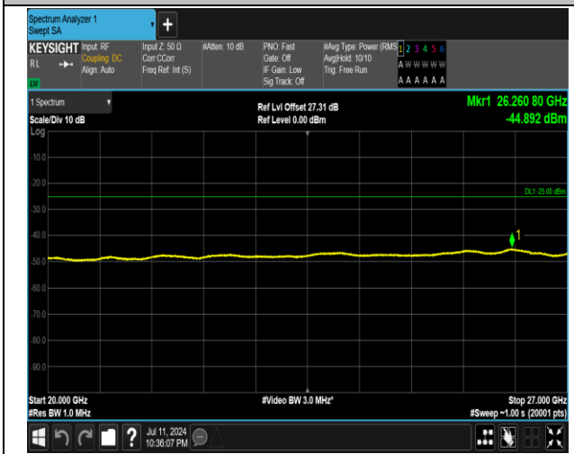
7-7-15MHz-20MHz-16QAM-16QAM-20828-20999-1RB#0-1RB#99-20000~27000MHz-PASS
