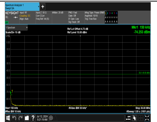
7-7-15MHz-15MHz-QPSK-QPSK-20825-20975-1RB#74-0 RB#0-0.15~30MHz-PASS
