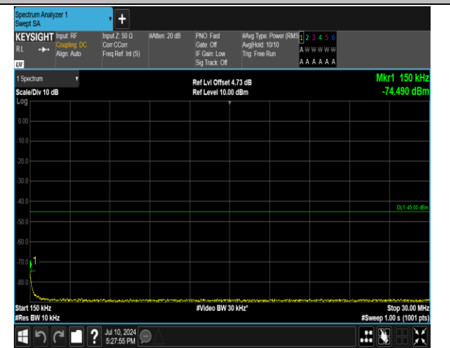
7-7-15MHz-10MHz-QPSK-QPSK-21277-21397-1RB#0-0R B#0-0.15~30MHz-PASS
