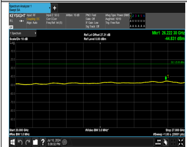
7-7-15MHz-10MHz-QPSK-QPSK-21277-21397-75RB#0-5 ORB#0-20000~27000MHz-PASS
