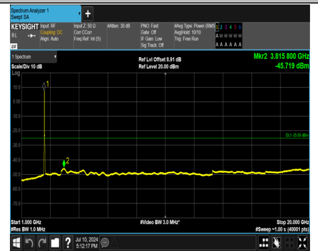
7-7-15MHz-10MHz-QPSK-QPSK-20825-20945-75RB#0-50 RB#0-1000~20000MHz-PASS
