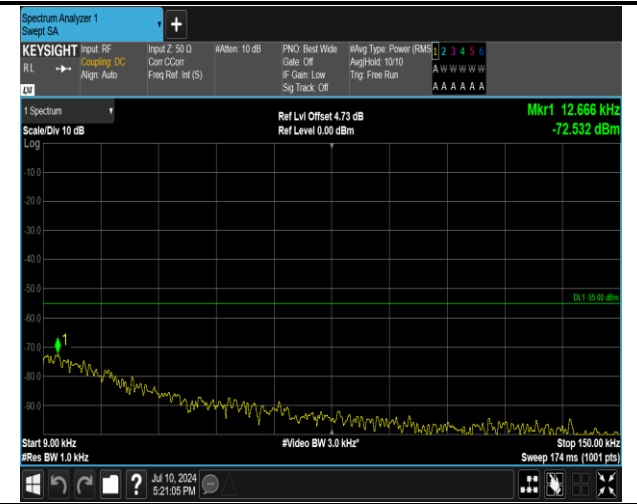
7-7-15MHz-10MHz-QPSK-QPSK-21051-21171-1RB#0-1R B#49-0.009~0.15MHz-PASS
