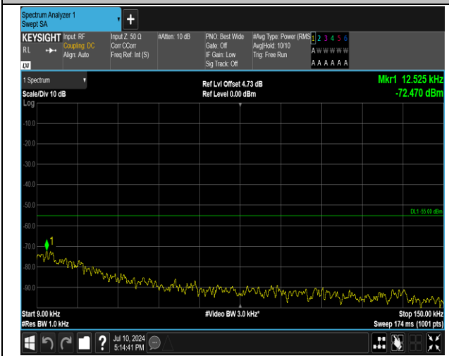
7-7-15MHz-10MHz-QPSK-QPSK-21051-21171-1RB#0-0R B#0-0.009~0.15MHz-PASS
