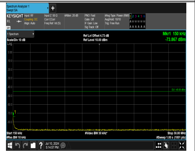
7-7-15MHz-10MHz-QPSK-QPSK-21051-21171-1RB#0-0R B#0-0.15~30MHz-PASS
