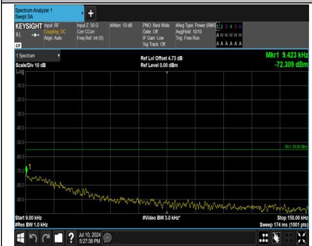
7-7-15MHz-10MHz-QPSK-QPSK-21277-21397-1RB#0-0R B#0-0.009~0.15MHz-PASS
