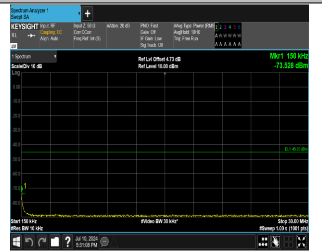
7-7-15MHz-10MHz-QPSK-QPSK-21277-21397-1RB#74-0 RB#0-0.15~30MHz-PASS
