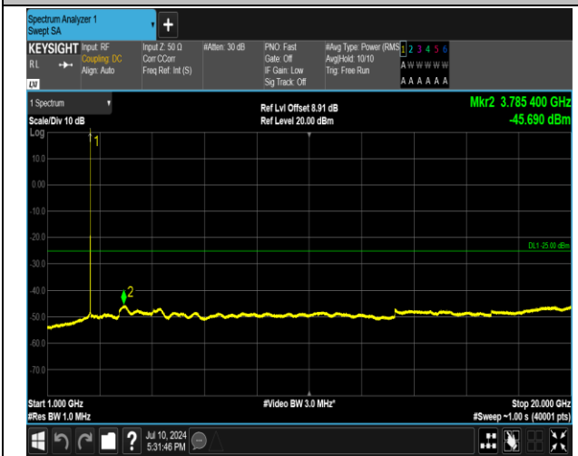
7-7-15MHz-10MHz-QPSK-QPSK-21277-21397-1RB#74-0 RB#0-1000~20000MHz-PASS
