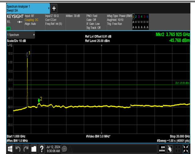
7-7-15MHz-15MHz-16QAM-16QAM-20825-20975-75RB#0 -75RB#0-1000~20000MHz-PASS
