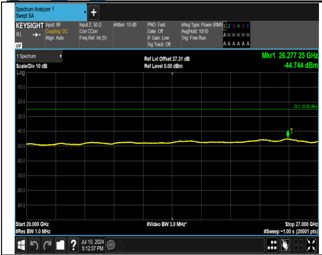
7-7-15MHz-10MHz-QPSK-QPSK-20825-20945-75RB#0-5 ORB#0-20000~27000MHz-PASS
