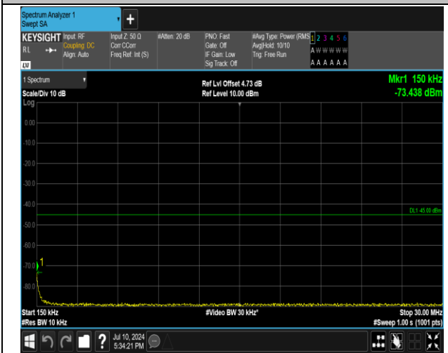
7-7-15MHz-10MHz-QPSK-QPSK-21277-21397-1RB#0-1R B#49-0.15~30MHz-PASS
