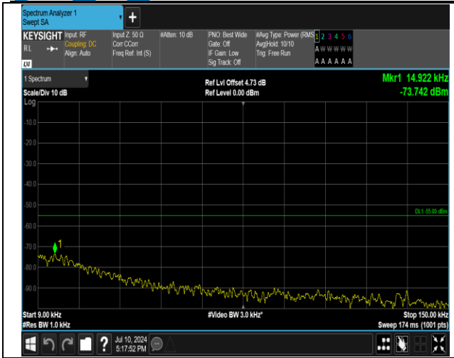
7-7-15MHz-10MHz-QPSK-QPSK-21051-21171-1RB#74-0 RB#0-0.009~0.15MHz-PASS
