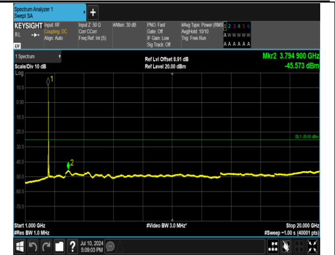
7-7-15MHz-10MHz-QPSK-QPSK-20825-20945-1RB#0-1R B#49-1000~20000MHz-PASS
