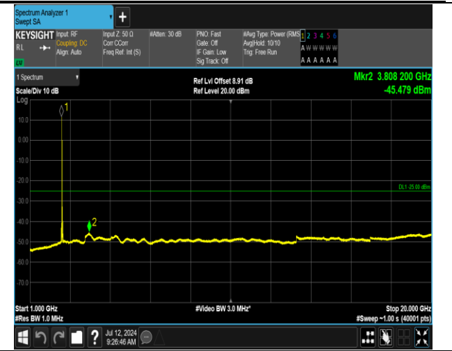
7-7-15MHz-15MHz-16QAM-16QAM-20825-20975-1RB#0-1RB#74-1000~20000MHz-PASS
