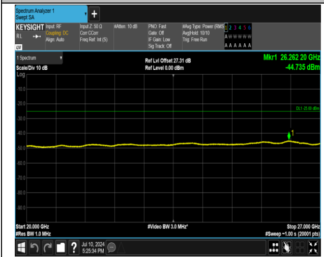
7-7-15MHz-10MHz-QPSK-QPSK-21051-21171-75RB#0-5 ORB#0-20000~27000MHz-PASS
