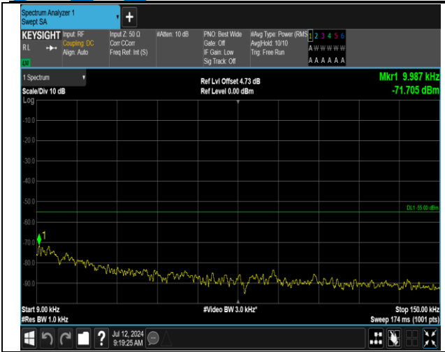
7-7-15MHz-15MHz-16QAM-16QAM-20825-20975-1RB#0-ORB#0-0.009~0.15MHz-PASS
