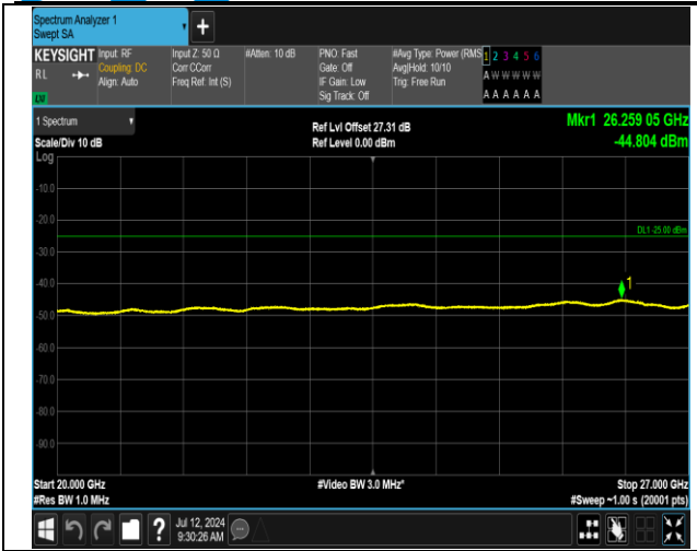
7-7-15MHz-15MHz-16QAM-16QAM-20825-20975-75RB#0-0-75RB#0-20000~27000MHz-PASS
