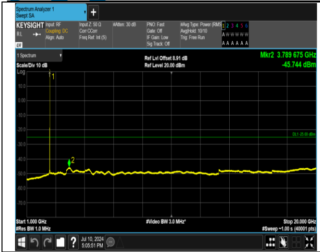
7-7-15MHz-10MHz-QPSK-QPSK-20825-20945-1RB#74-0 RB#0-1000~20000MHz-PASS
