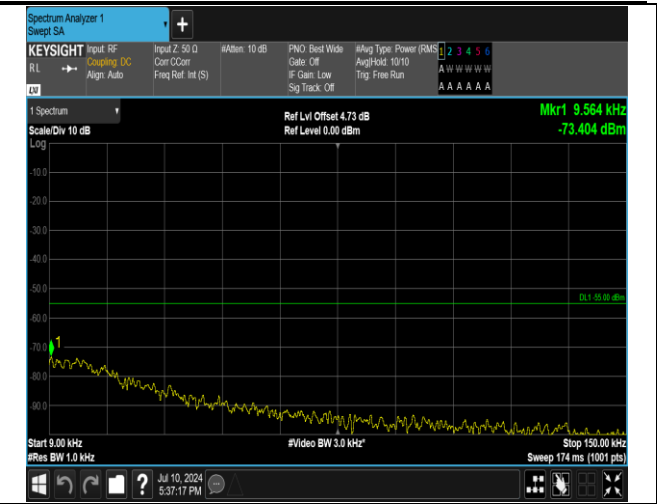
7-7-15MHz-10MHz-QPSK-QPSK-21277-21397-75RB#0-50 RB#0-0.009~0.15MHz-PASS
