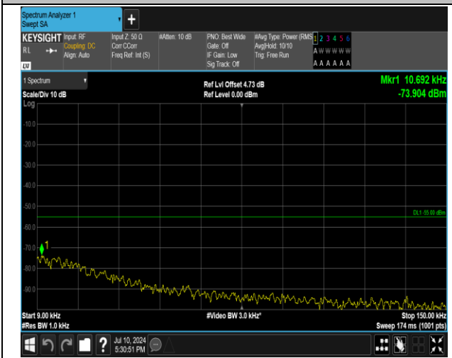
7-7-15MHz-10MHz-QPSK-QPSK-21277-21397-1RB#74-0 RB#0-0.009~0.15MHz-PASS
