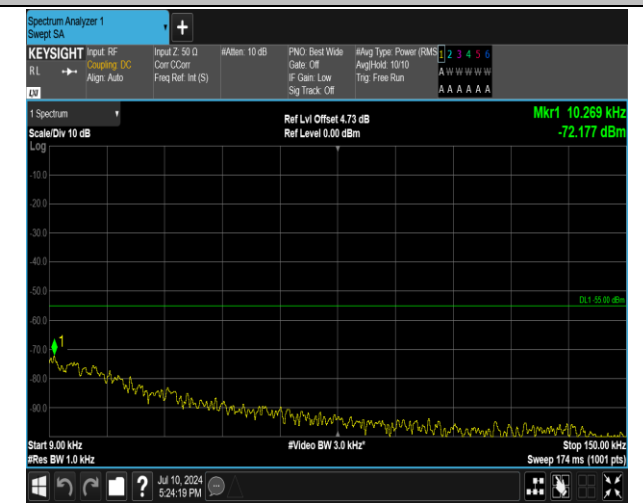
7-7-15MHz-10MHz-QPSK-QPSK-21051-21171-75RB#0-50 RB#0-0.009~0.15MHz-PASS
