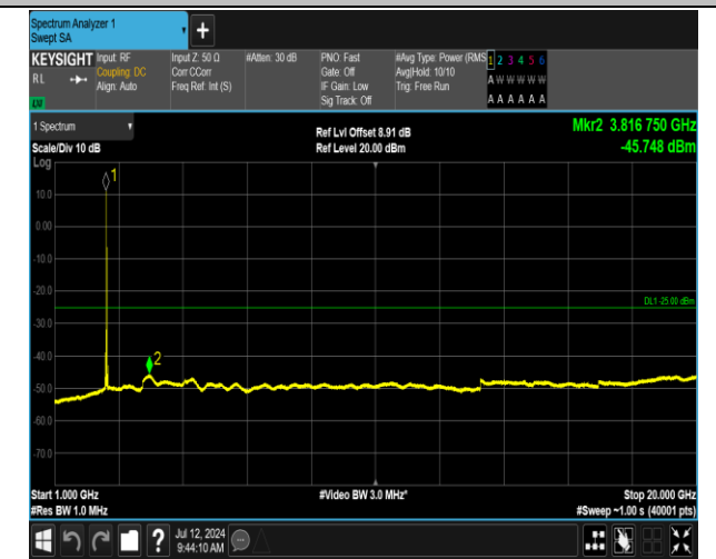
7-7-15MHz-15MHz-16QAM-16QAM-21025-21175-1RB#0-1RB#74-1000~20000MHz-PASS
