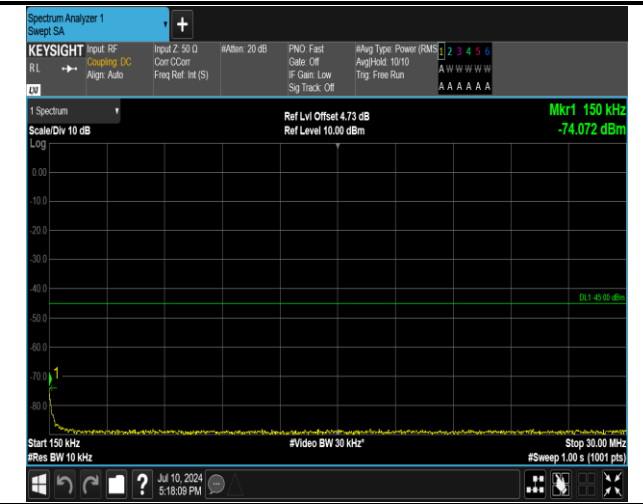
7-7-15MHz-10MHz-QPSK-QPSK-21051-21171-1RB#74-0 RB#0-0.15~30MHz-PASS
