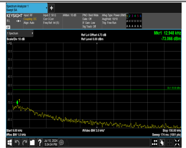
7-7-15MHz-10MHz-QPSK-QPSK-21277-21397-1RB#0-1R B#49-0.009~0.15MHz-PASS
