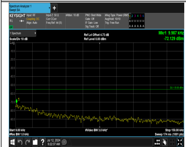
7-7-15MHz-15MHz-16QAM-16QAM-20825-20975-1RB#74-4-0RB#0-0.009~0.15MHz-PASS
