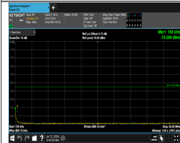
7-7-15MHz-15MHz-16QAM-16QAM-21025-21175-1RB#0-1RB#74-0.15~30MHz-PASS
