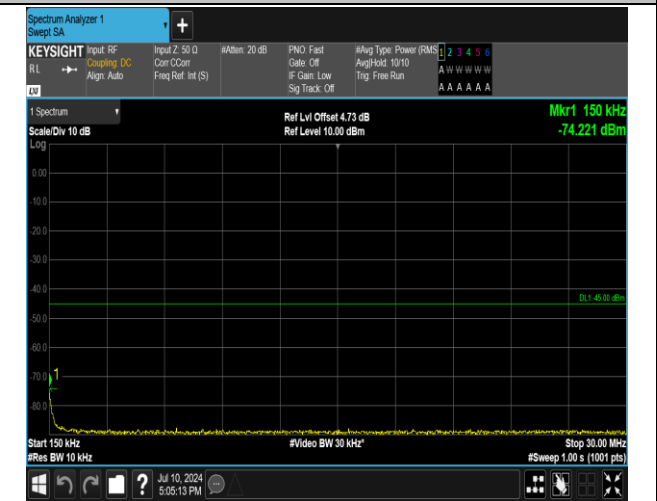
7-7-15MHz-10MHz-QPSK-QPSK-20825-20945-1RB#74-0 RB#0-0.15~30MHz-PASS
