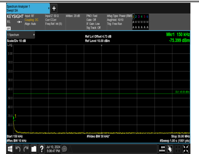
7-7-15MHz-10MHz-16QAM-16QAM-20825-20945-1RB#74-4-0RB#0-0.15~30MHz-PASS
