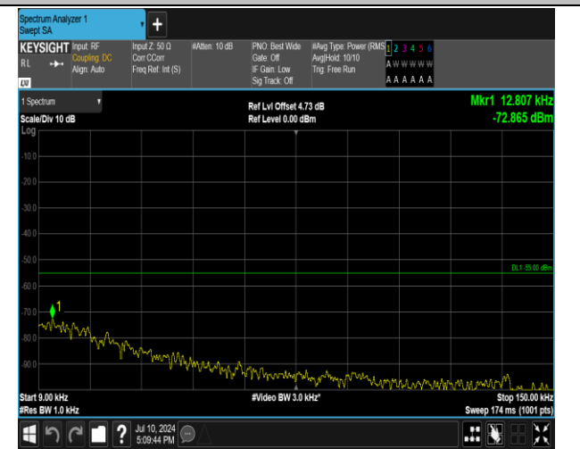
7-7-15MHz-10MHz-16QAM-16QAM-20825-20945-1RB#0-1RB#49-0.009~0.15MHz-PASS
