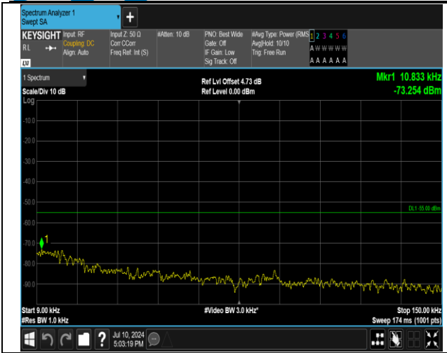
7-7-15MHz-10MHz-16QAM-16QAM-20825-20945-1RB#0-ORB#0-0.009~0.15MHz-PASS
