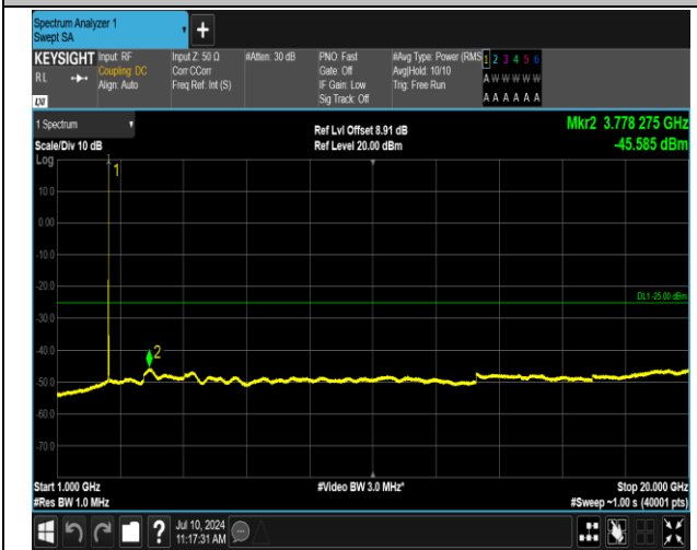
7-7-10MHz-20MHz-QPSK-QPSK-21206-21350-1RB#49-0 RB#0-1000~20000MHz-PASS
