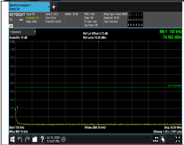
7-7-15MHz-10MHz-16QAM-16QAM-20825-20945-1RB#0-1RB#49-0.15~30MHz-PASS
