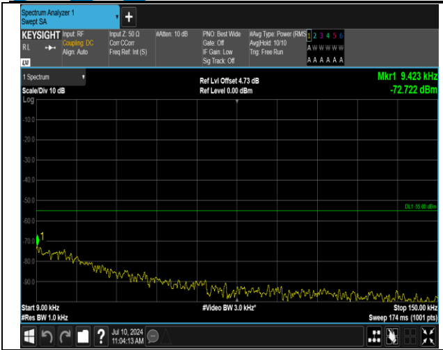
7-7-10MHz-20MHz-QPSK-QPSK-21006-21150-1RB#49-0 RB#0-0.009~0.15MHz-PASS
