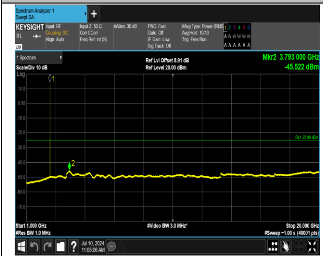
7-7-10MHz-20MHz-QPSK-QPSK-21006-21150-1RB#49-0 RB#0-1000~20000MHz-PASS
