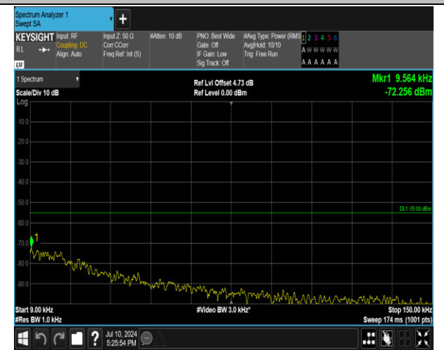
7-7-15MHz-10MHz-16QAM-16QAM-21051-21171-75RB#0 -50RB#0-0.009~0.15MHz-PASS
