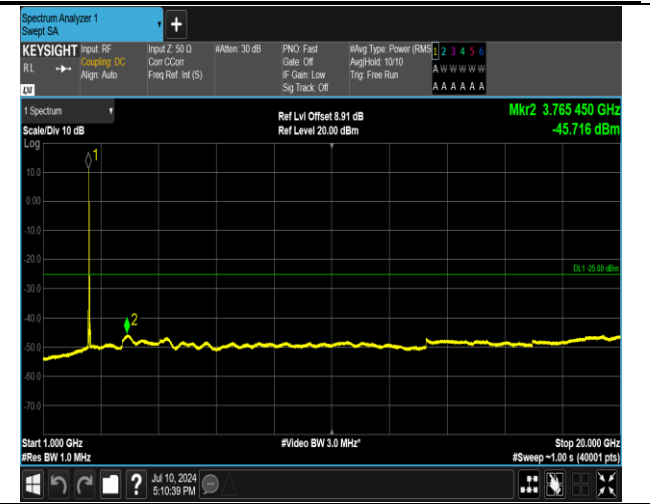
7-7-15MHz-10MHz-16QAM-16QAM-20825-20945-1RB#0-1RB#49-1000~20000MHz-PASS
