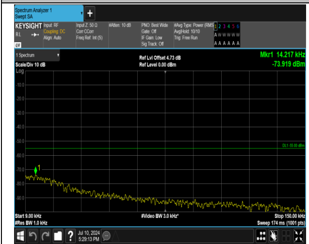
7-7-15MHz-10MHz-16QAM-16QAM-21277-21397-1RB#0- ORB#0-0.009~0.15MHz-PASS
