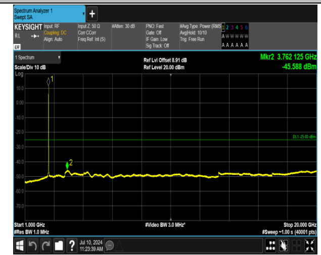
7-7-10MHz-20MHz-QPSK-QPSK-21206-21350-50RB#0-10 ORB#0-1000~20000MHz-PASS
