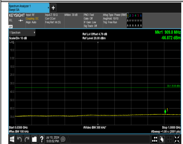
7-7-15MHz-10MHz-16QAM-16QAM-20825-20945-1RB#0-ORB#0-30~1000MHz-PASS
