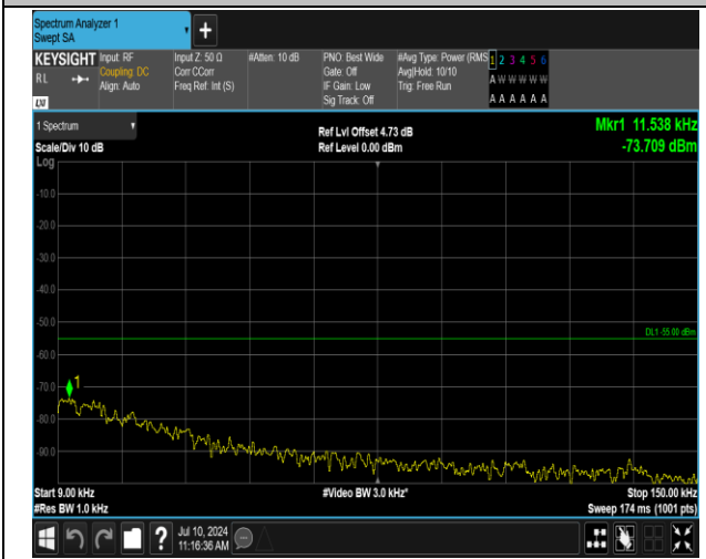
7-7-10MHz-20MHz-QPSK-QPSK-21206-21350-1RB#49-0 RB#0-0.009~0.15MHz-PASS
