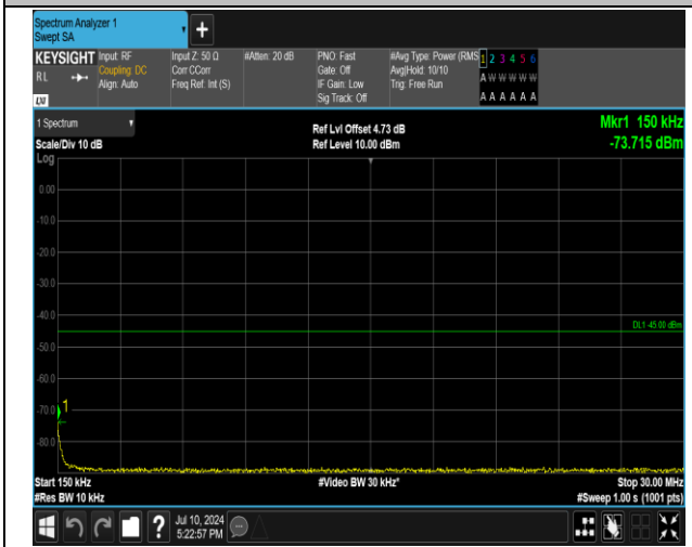
7-7-15MHz-10MHz-16QAM-16QAM-21051-21171-1RB#0-1RB#49-0.15~30MHz-PASS
