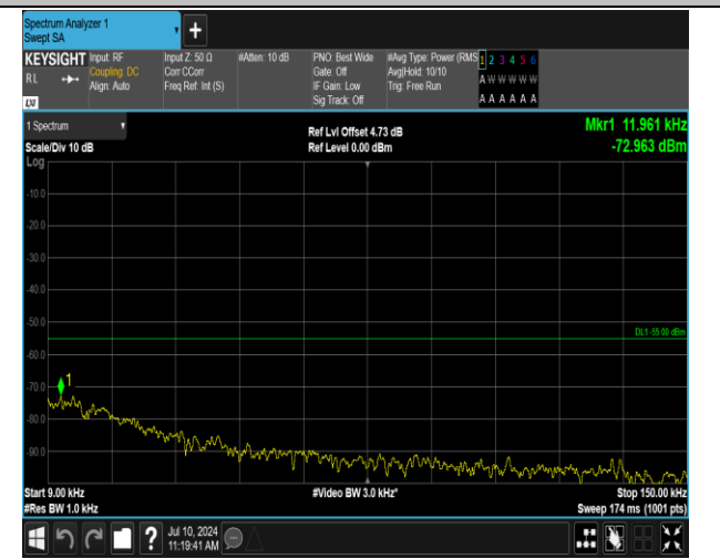
7-7-10MHz-20MHz-QPSK-QPSK-21206-21350-1RB#0-1R B#99-0.009~0.15MHz-PASS
