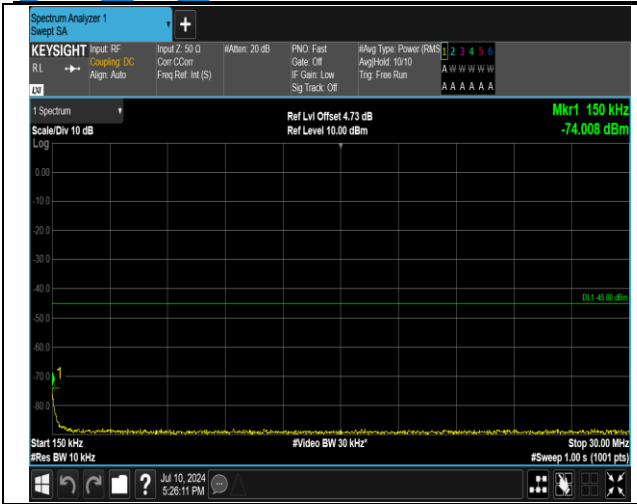
7-7-15MHz-10MHz-16QAM-16QAM-21051-21171-75RB#0 -50RB#0-0.15~30MHz-PASS
