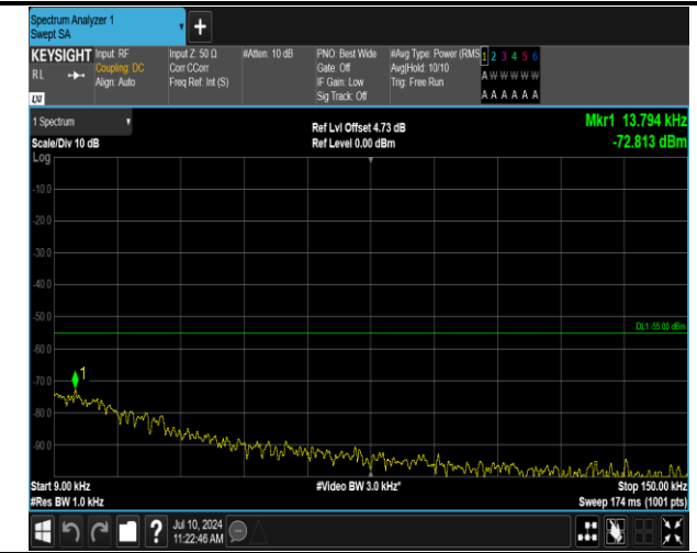
7-7-10MHz-20MHz-QPSK-QPSK-21206-21350-50RB#0-10 ORB#0-0.009~0.15MHz-PASS
