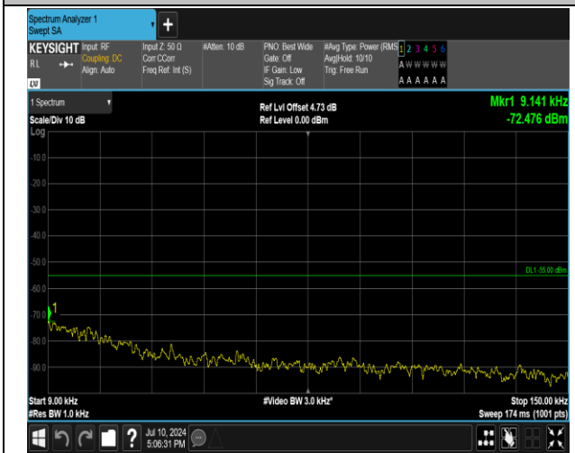
7-7-15MHz-10MHz-16QAM-16QAM-20825-20945-1RB#74-4-0RB#0-0.009~0.15MHz-PASS
