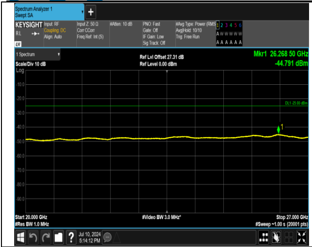
7-7-15MHz-10MHz-16QAM-16QAM-20825-20945-75RB#-0-50RB#0-20000~27000MHz-PASS
