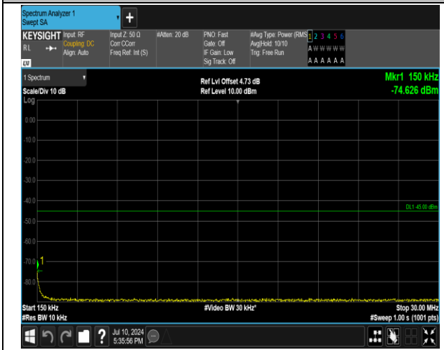
7-7-15MHz-10MHz-16QAM-16QAM-21277-21397-1RB#0-1RB#49-0.15~30MHz-PASS
