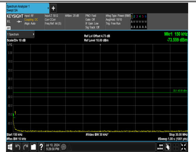
7-7-15MHz-10MHz-16QAM-16QAM-21277-21397-1RB#0- ORB#0-0.15~30MHz-PASS
