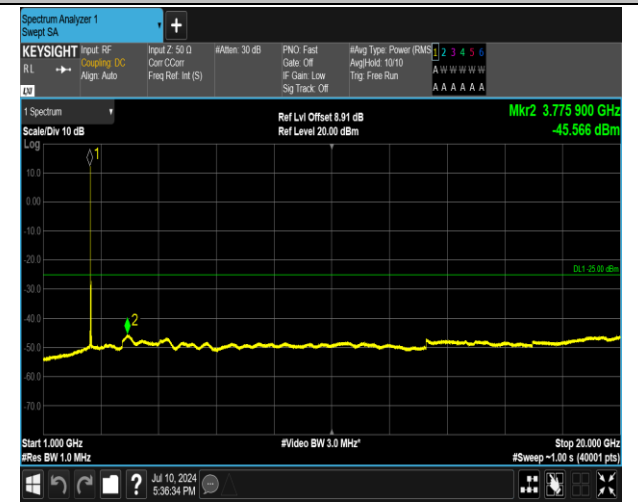
7-7-15MHz-10MHz-16QAM-16QAM-21277-21397-1RB#0-1RB#49-1000~20000MHz-PASS
