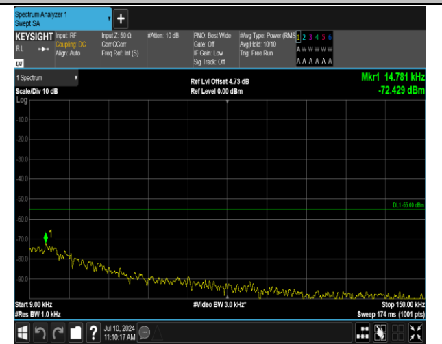
7-7-10MHz-20MHz-QPSK-QPSK-21006-21150-50RB#0-10 ORB#0-0.009~0.15MHz-PASS
