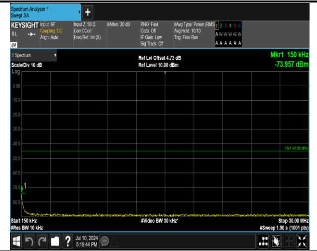
7-7-15MHz-10MHz-16QAM-16QAM-21051-21171-1RB#74 -ORB#0-0.15~30MHz-PASS
