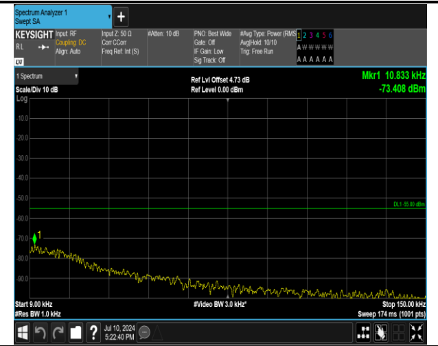
7-7-15MHz-10MHz-16QAM-16QAM-21051-21171-1RB#0-1RB#49-0.009~0.15MHz-PASS
