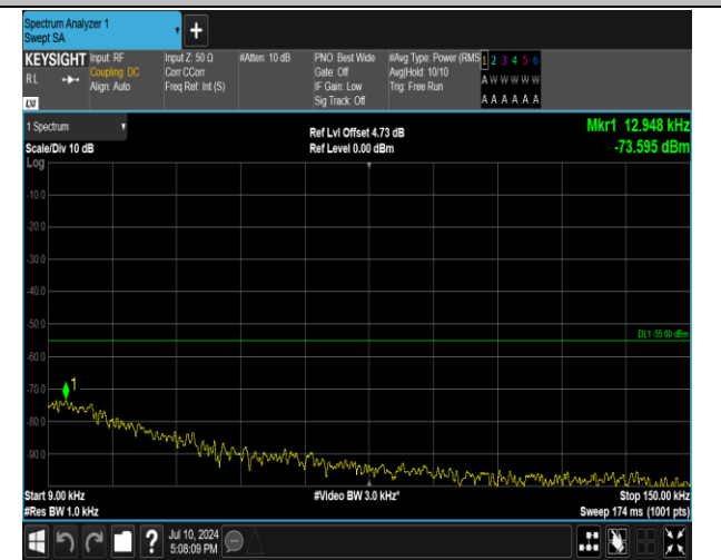
7-7-15MHz-10MHz-QPSK-QPSK-20825-20945-1RB#0-1R B#49-0.009~0.15MHz-PASS
