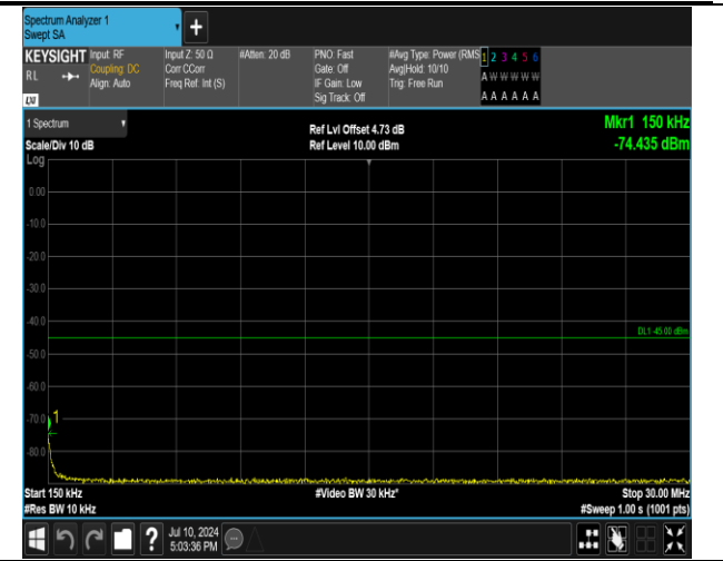
7-7-15MHz-10MHz-16QAM-16QAM-20825-20945-1RB#0-ORB#0-0.15~30MHz-PASS
