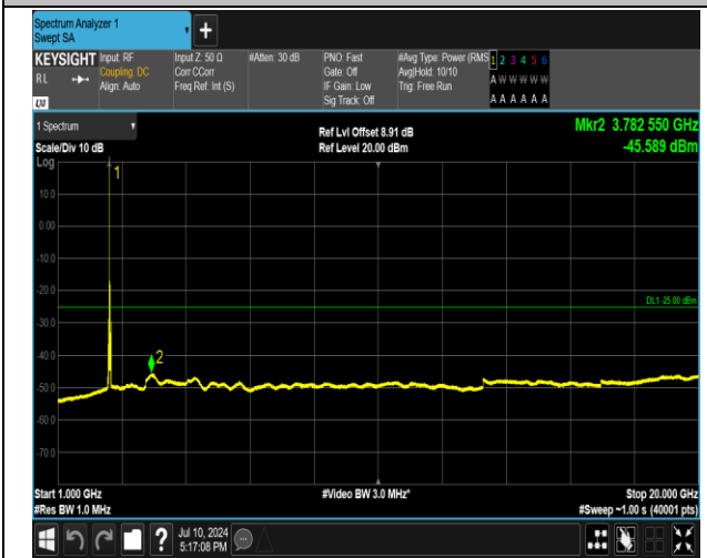
7-7-15MHz-10MHz-16QAM-16QAM-21051-21171-1RB#0-0RB#0-1000~20000MHz-PASS
