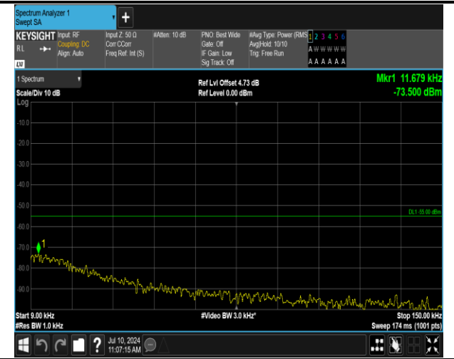
7-7-10MHz-20MHz-QPSK-QPSK-21006-21150-1RB#0-1R B#99-0.009~0.15MHz-PASS
