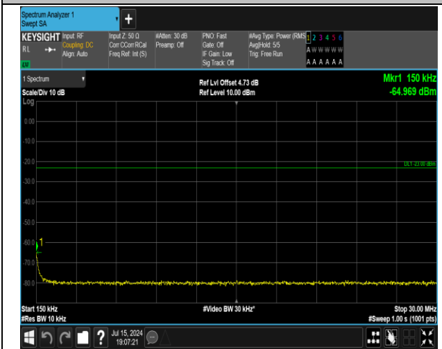
5-5-5MHz-3MHz-QPSK-QPSK-20425-20464-25RB#0-15R B#0-0.15~30MHz-PASS
