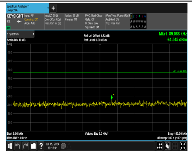
5-5-5MHz-3MHz-QPSK-QPSK-20510-20549-25RB#0-15R B#0-0.009~0.15MHz-PASS
