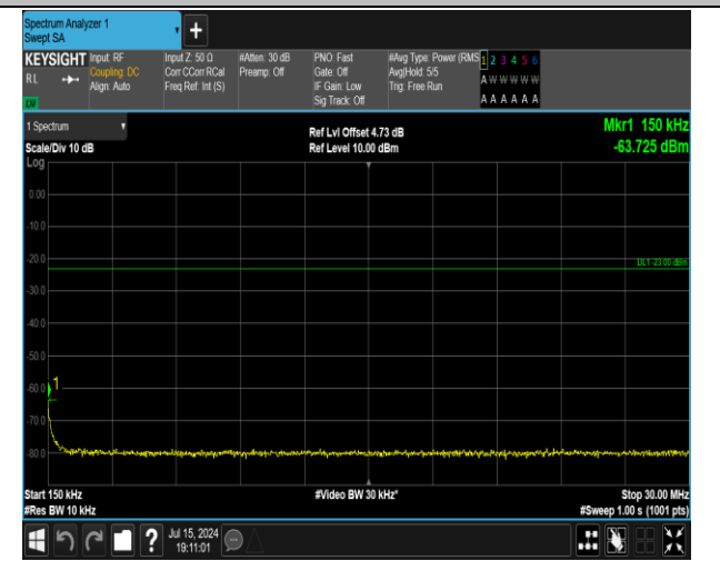
5-5-5MHz-3MHz-16QAM-16QAM-20510-20549-1RB#0-0R B#0-0.15~30MHz-PASS
