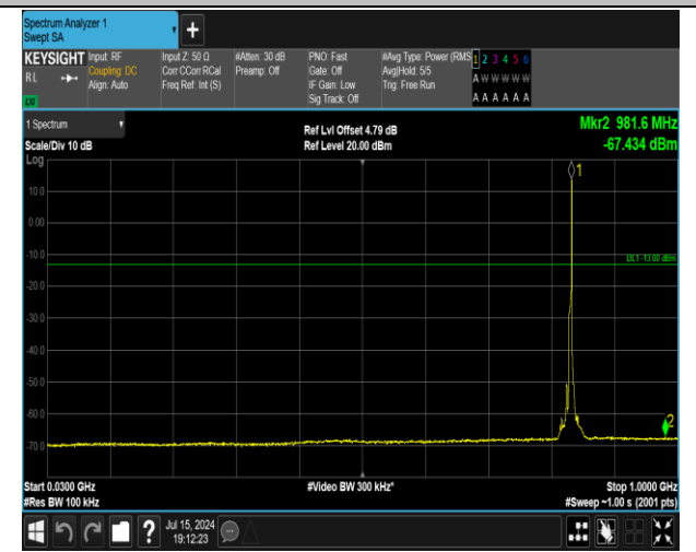
5-5-5MHz-3MHz-QPSK-QPSK-20510-20549-1RB#24-0RB #0-30~1000MHz-PASS
