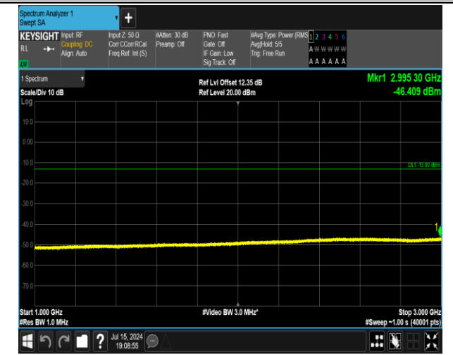
5-5-5MHz-3MHz-16QAM-16QAM-20425-20464-25RB#0-1 5RB#0-1000~3000MHz-PASS
