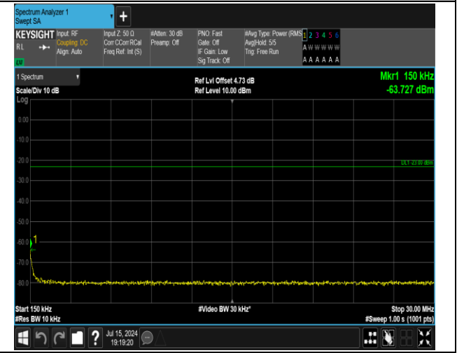
5-5-5MHz-3MHz-QPSK-QPSK-20595-20634-1RB#0-0RB# 0-0.15~30MHz-PASS
