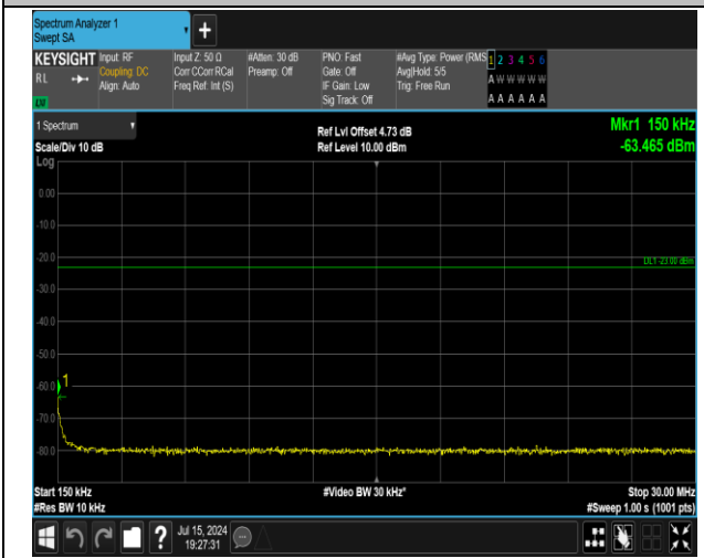
5-5-5MHz-3MHz-16QAM-16QAM-20595-20634-25RB#0-1 5RB#0-0.15~30MHz-PASS
