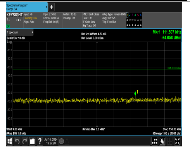
5-5-5MHz-3MHz-16QAM-16QAM-20595-20634-25RB#0-1 5RB#0-0.009~0.15MHz-PASS
