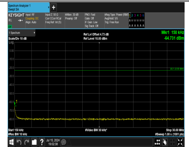
5-5-5MHz-3MHz-QPSK-QPSK-20425-20464-1RB#24-0RB #0-0.15~30MHz-PASS
