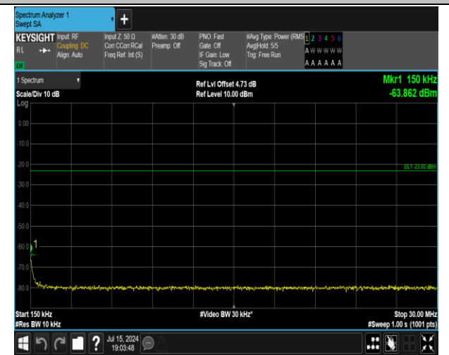
5-5-5MHz-3MHz-16QAM-16QAM-20425-20464-1RB#24-0 RB#0-0.15~30MHz-PASS
