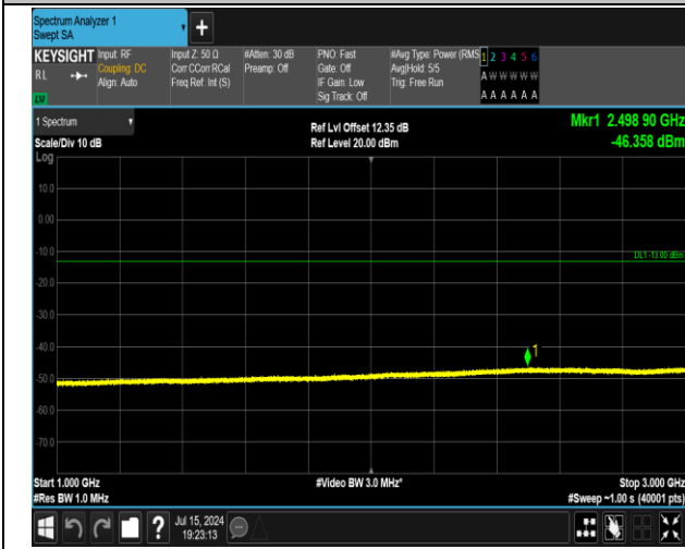
5-5-5MHz-3MHz-16QAM-16QAM-20595-20634-1RB#24-0 RB#0-1000~3000MHz-PASS
