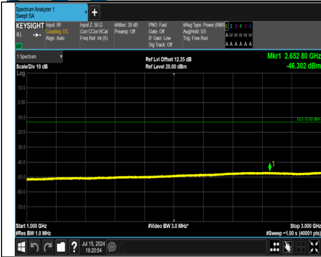
5-5-5MHz-3MHz-16QAM-16QAM-20595-20634-1RB#0-0R B#0-1000~3000MHz-PASS
