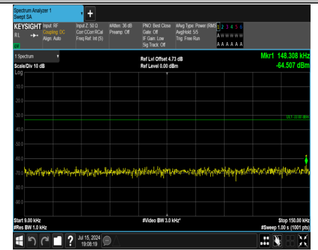
5-5-5MHz-3MHz-16QAM-16QAM-20425-20464-25RB#0-1 5RB#0-0.009~0.15MHz-PASS
