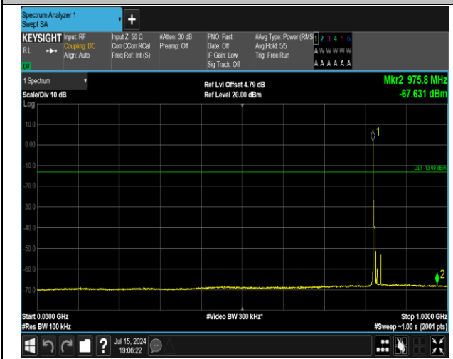
5-5-5MHz-3MHz-16QAM-16QAM-20425-20464-1RB#0-1R B#15-30~1000MHz-PASS
