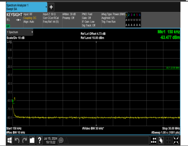
5-5-5MHz-3MHz-16QAM-16QAM-20510-20549-1RB#24-0 RB#0-0.15~30MHz-PASS
