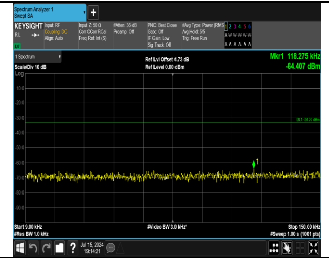
5-5-5MHz-3MHz-QPSK-QPSK-20510-20549-1RB#0-1RB# 15-0.009~0.15MHz-PASS
