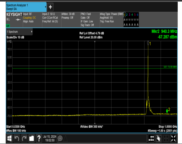
5-5-5MHz-3MHz-QPSK-QPSK-20425-20464-1RB#24-0RB #0-30~1000MHz-PASS
