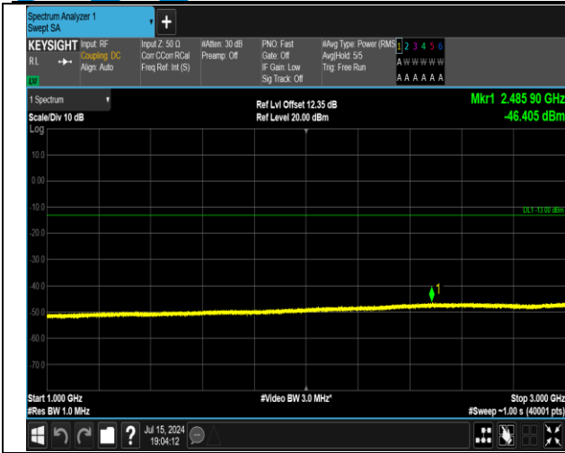
5-5-5MHz-3MHz-16QAM-16QAM-20425-20464-1RB#24-0 RB#0-1000~3000MHz-PASS
