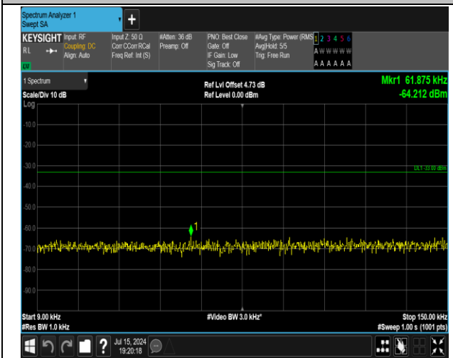
5-5-5MHz-3MHz-16QAM-16QAM-20595-20634-1RB#0-0R B#0-0.009~0.15MHz-PASS
