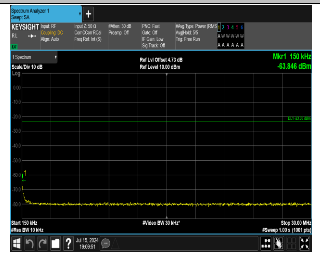
5-5-5MHz-3MHz-QPSK-QPSK-20510-20549-1RB#0-0RB# 0-0.15~30MHz-PASS
