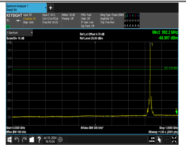
5-5-5MHz-3MHz-16QAM-16QAM-20510-20549-1RB#24-0 RB#0-30~1000MHz-PASS
