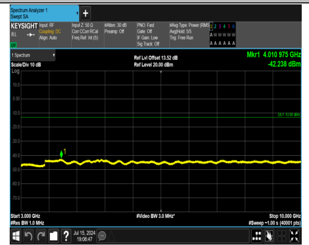
5-5-5MHz-3MHz-16QAM-16QAM-20425-20464-1RB#0-1R B#15-3000~10000MHz-PASS
