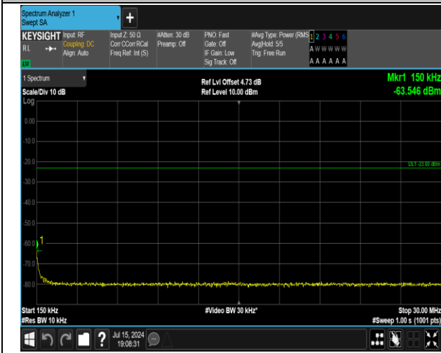
5-5-5MHz-3MHz-16QAM-16QAM-20425-20464-25RB#0-1 5RB#0-0.15~30MHz-PASS
