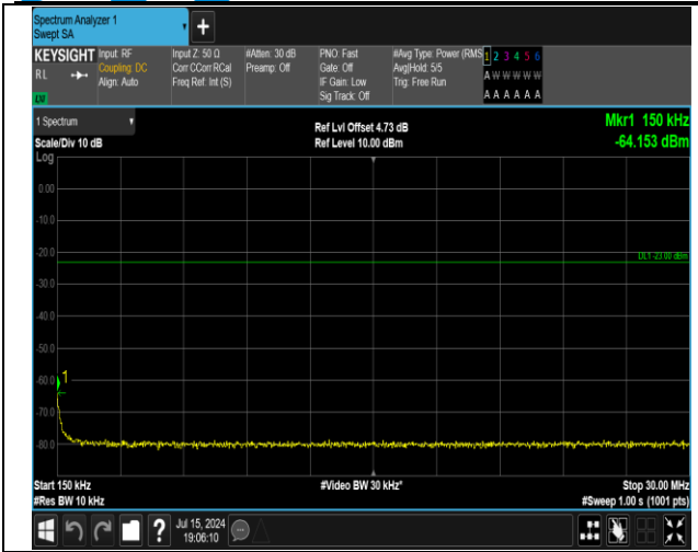
5-5-5MHz-3MHz-16QAM-16QAM-20425-20464-1RB#0-1R B#15-0.15~30MHz-PASS
