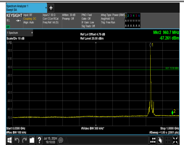
5-5-5MHz-3MHz-QPSK-QPSK-20510-20549-1RB#0-0RB# 0-30~1000MHz-PASS
