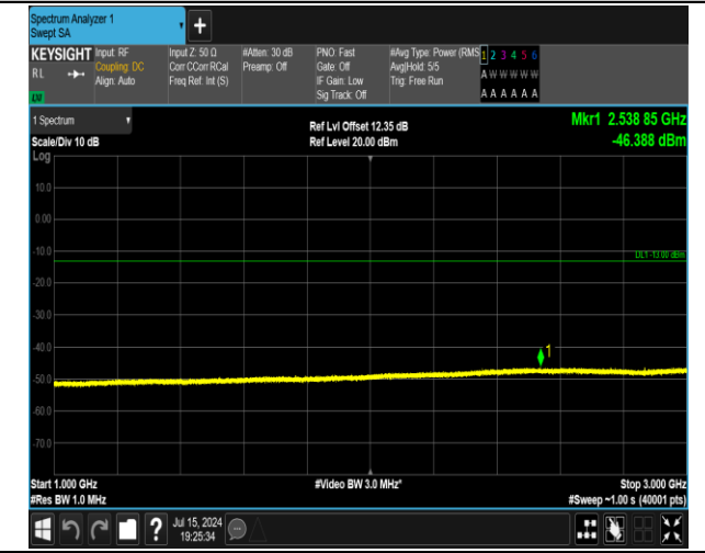
5-5-5MHz-3MHz-16QAM-16QAM-20595-20634-1RB#0-1R B#15-1000~3000MHz-PASS
