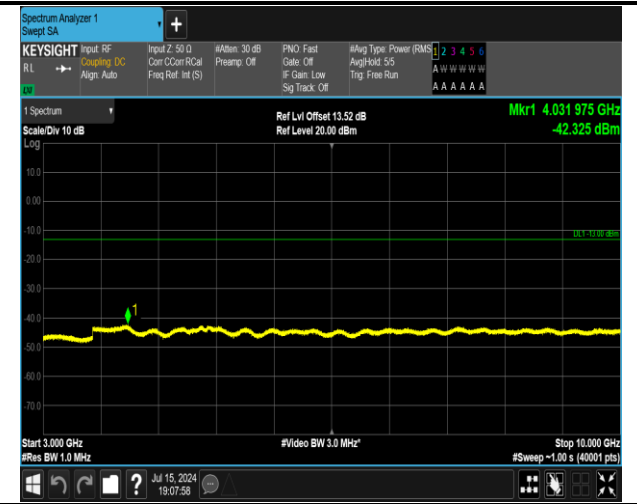
5-5-5MHz-3MHz-QPSK-QPSK-20425-20464-25RB#0-15R B#0-3000~10000MHz-PASS
