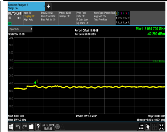
5-5-5MHz-3MHz-16QAM-16QAM-20510-20549-1RB#0-0R B#0-3000~10000MHz-PASS
