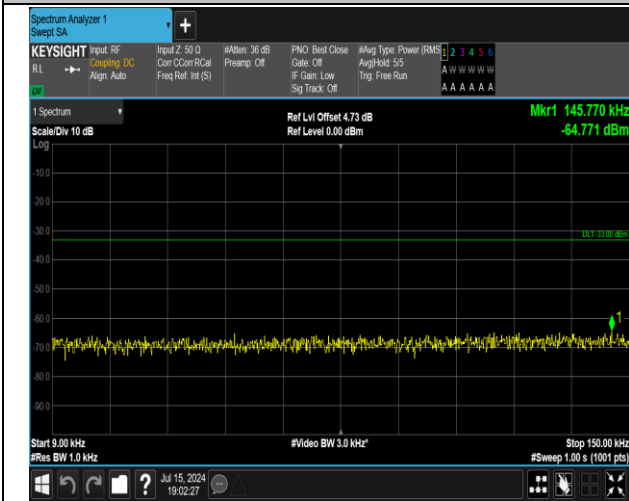
5-5-5MHz-3MHz-QPSK-QPSK-20425-20464-1RB#24-0RB #0-0.009~0.15MHz-PASS
