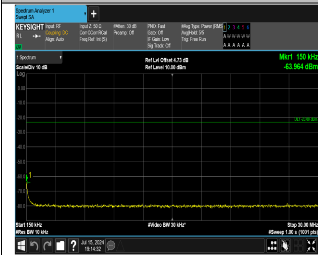
5-5-5MHz-3MHz-QPSK-QPSK-20510-20549-1RB#0-1RB# 15-0.15~30MHz-PASS
