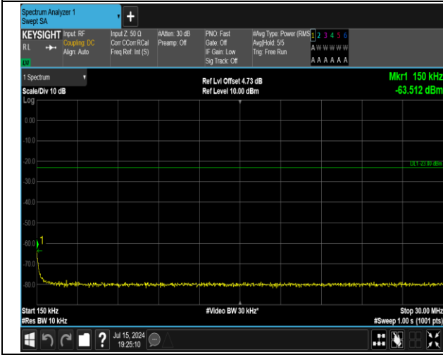
5-5-5MHz-3MHz-16QAM-16QAM-20595-20634-1RB#0-1R B#15-0.15~30MHz-PASS
