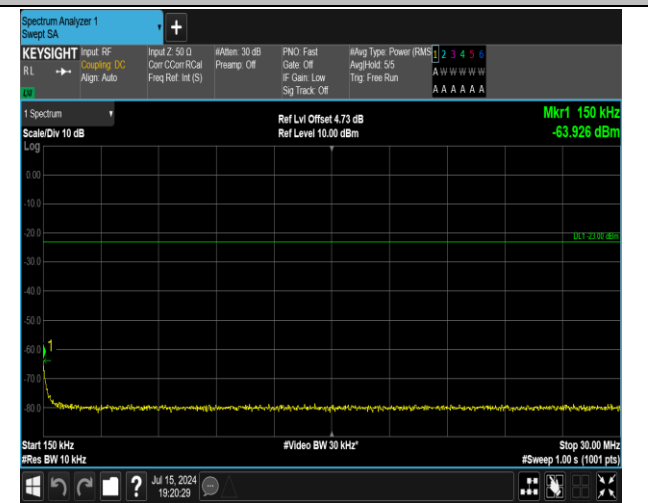
5-5-5MHz-3MHz-16QAM-16QAM-20595-20634-1RB#0-0R B#0-0.15~30MHz-PASS
