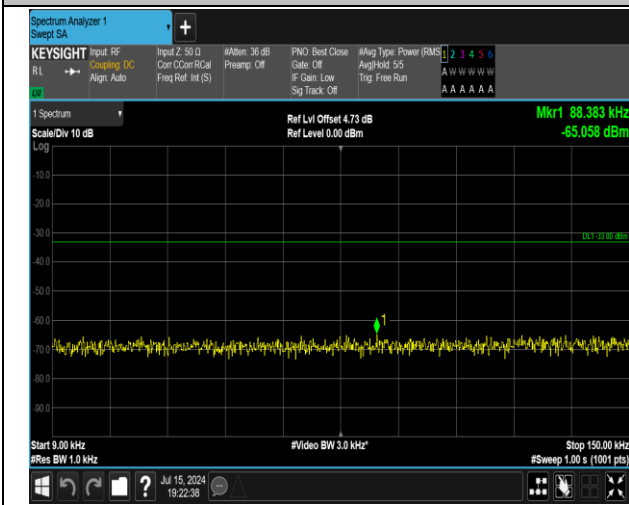
5-5-5MHz-3MHz-16QAM-16QAM-20595-20634-1RB#24-0 RB#0-0.009~0.15MHz-PASS
