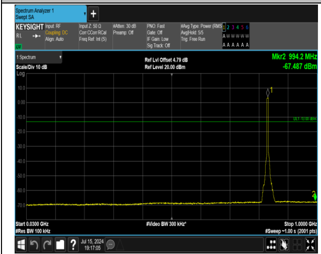
5-5-5MHz-3MHz-QPSK-QPSK-20510-20549-25RB#0-15R B#0-30~1000MHz-PASS
