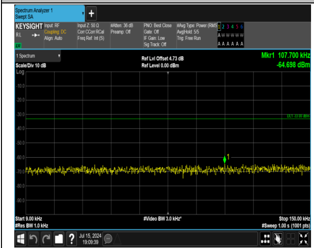
5-5-5MHz-3MHz-QPSK-QPSK-20510-20549-1RB#0-0RB# 0-0.009~0.15MHz-PASS
