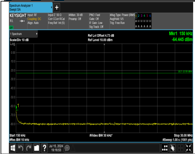
5-5-5MHz-3MHz-QPSK-QPSK-20510-20549-25RB#0-15R B#0-0.15~30MHz-PASS
