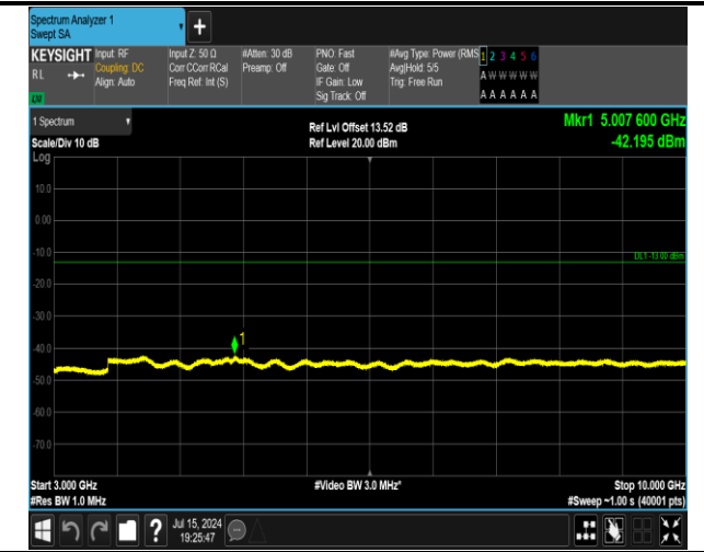
5-5-5MHz-3MHz-16QAM-16QAM-20595-20634-1RB#0-1R B#15-3000~10000MHz-PASS
