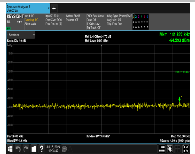
5-5-5MHz-3MHz-QPSK-QPSK-20425-20464-1RB#0-1RB# 15-0.009~0.15MHz-PASS
