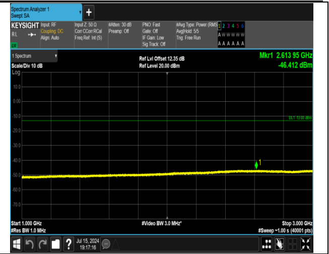
5-5-5MHz-3MHz-QPSK-QPSK-20510-20549-25RB#0-15R B#0-1000~3000MHz-PASS
