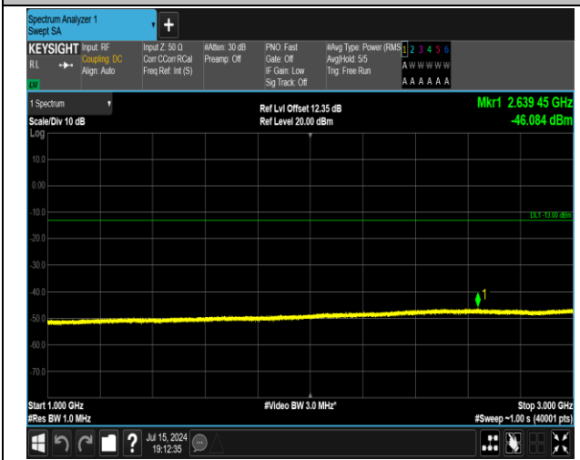
5-5-5MHz-3MHz-QPSK-QPSK-20510-20549-1RB#24-0RB #0-1000~3000MHz-PASS
