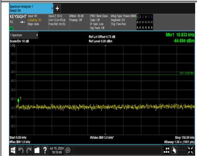
5-5-5MHz-3MHz-16QAM-16QAM-20510-20549-1RB#0-0R B#0-0.009~0.15MHz-PASS
