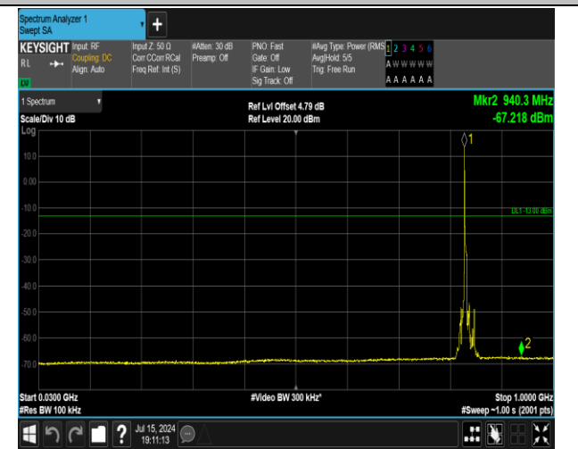
5-5-5MHz-3MHz-16QAM-16QAM-20510-20549-1RB#0-0R B#0-30~1000MHz-PASS
