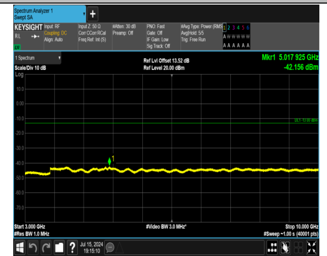
5-5-5MHz-3MHz-QPSK-QPSK-20510-20549-1RB#0-1RB# 15-3000~10000MHz-PASS
