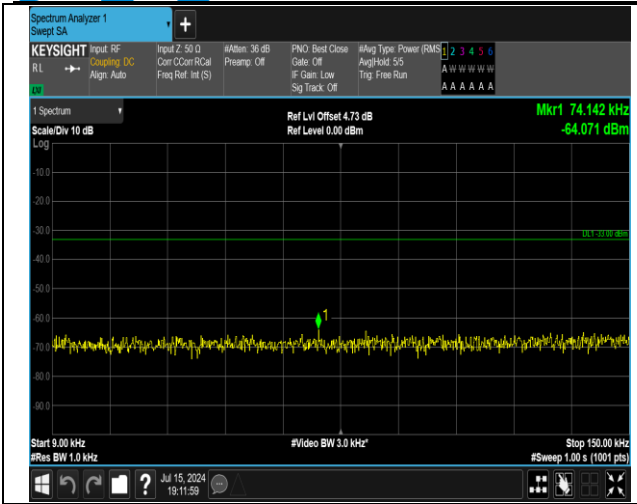
5-5-5MHz-3MHz-QPSK-QPSK-20510-20549-1RB#24-0RB #0-0.009~0.15MHz-PASS
