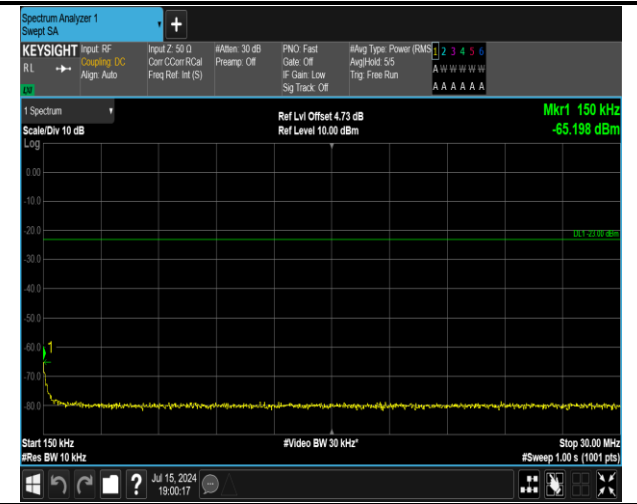
5-5-5MHz-3MHz-QPSK-QPSK-20425-20464-1RB#0-0RB# 0-0.15~30MHz-PASS
