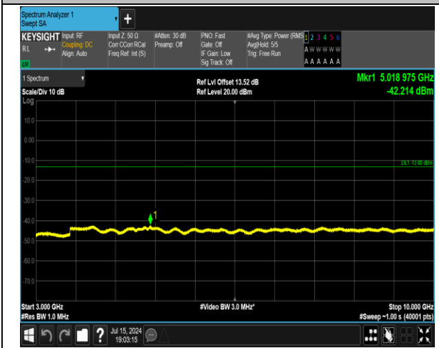
5-5-5MHz-3MHz-QPSK-QPSK-20425-20464-1RB#24-0RB #0-3000~10000MHz-PASS
