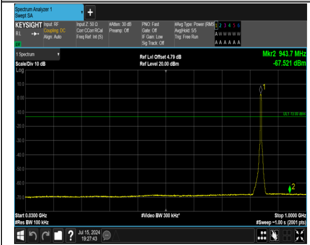
5-5-5MHz-3MHz-16QAM-16QAM-20595-20634-25RB#0-1 5RB#0-30~1000MHz-PASS
