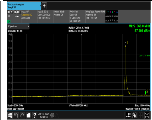
5-5-5MHz-3MHz-16QAM-16QAM-20425-20464-25RB#0-1 5RB#0-30~1000MHz-PASS
