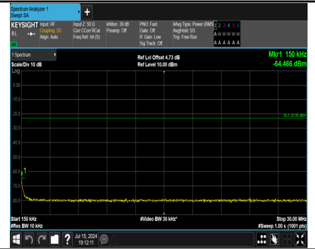
5-5-5MHz-3MHz-QPSK-QPSK-20510-20549-1RB#24-0RB #0-0.15~30MHz-PASS
