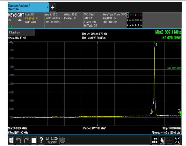
5-5-5MHz-3MHz-16QAM-16QAM-20595-20634-1RB#24-0 RB#0-30~1000MHz-PASS
