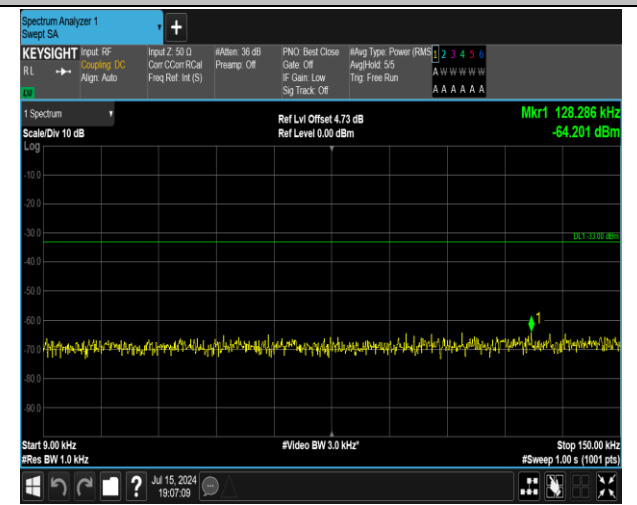
5-5-5MHz-3MHz-QPSK-QPSK-20425-20464-25RB#0-15R B#0-0.009~0.15MHz-PASS
