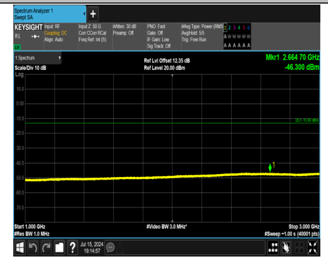
5-5-5MHz-3MHz-QPSK-QPSK-20510-20549-1RB#0-1RB# 15-1000~3000MHz-PASS
