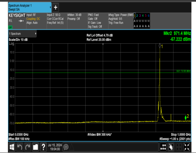
5-5-5MHz-3MHz-16QAM-16QAM-20425-20464-1RB#24-0 RB#0-30~1000MHz-PASS
