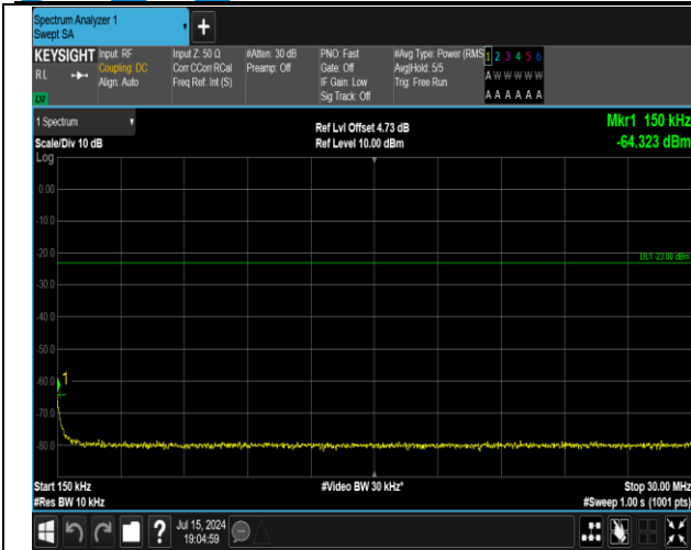
5-5-5MHz-3MHz-QPSK-QPSK-20425-20464-1RB#0-1RB# 15-0.15~30MHz-PASS
