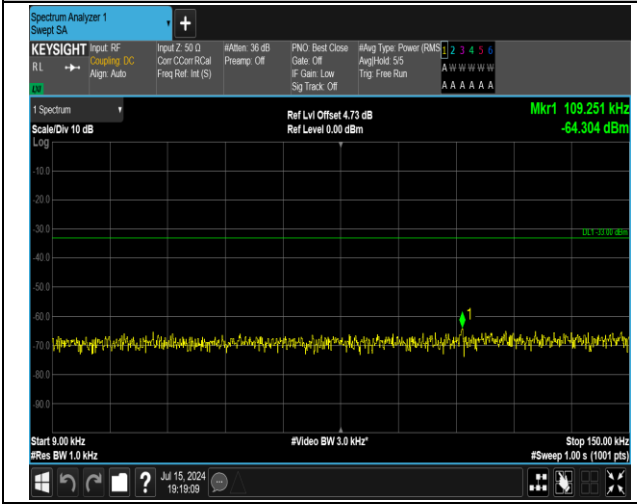
5-5-5MHz-3MHz-QPSK-QPSK-20595-20634-1RB#0-0RB# 0-0.009~0.15MHz-PASS
