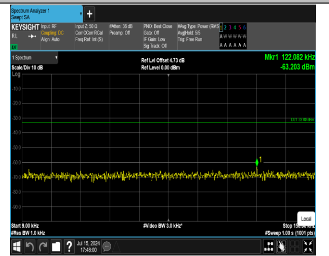
5-5-3MHz-5MHz-16QAM-16QAM-20416-20455-1RB#14-0 RB#0-0.009~0.15MHz-PASS
