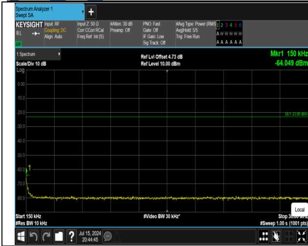
5-5-10MHz-10MHz-QPSK-QPSK-20450-20549-1RB#0-1R B#49-0.15~30MHz-PASS
