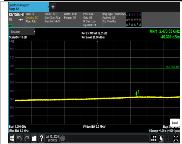
5-5-10MHz-10MHz-QPSK-QPSK-20501-20600-1RB#0-0R B#0-1000~3000MHz-PASS
