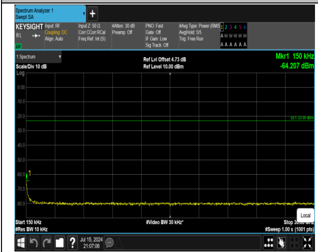
5-5-10MHz-10MHz-16QAM-16QAM-20501-20600-50RB#0 0-50RB#0-0.15~30MHz-PASS
