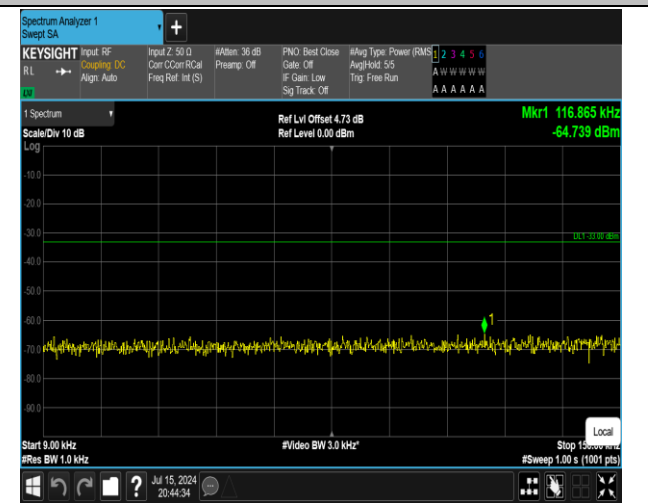
5-5-10MHz-10MHz-QPSK-QPSK-20450-20549-1RB#0-1R B#49-0.009~0.15MHz-PASS
