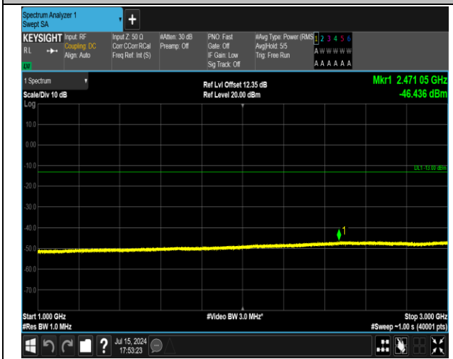
5-5-3MHz-5MHz-16QAM-16QAM-20416-20455-15RB#0-2 5RB#0-1000~3000MHz-PASS
