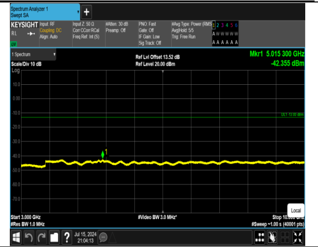
5-5-10MHz-10MHz-QPSK-QPSK-20501-20600-1RB#0-1R B#49-3000~10000MHz-PASS
