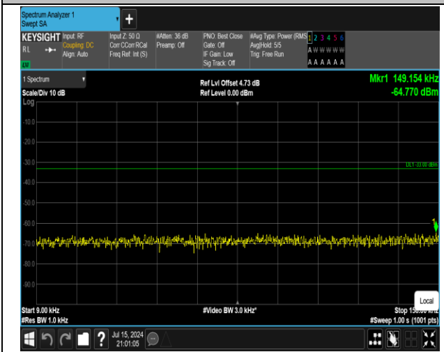
5-5-10MHz-10MHz-QPSK-QPSK-20501-20600-1RB#49-0 RB#0-0.009~0.15MHz-PASS
