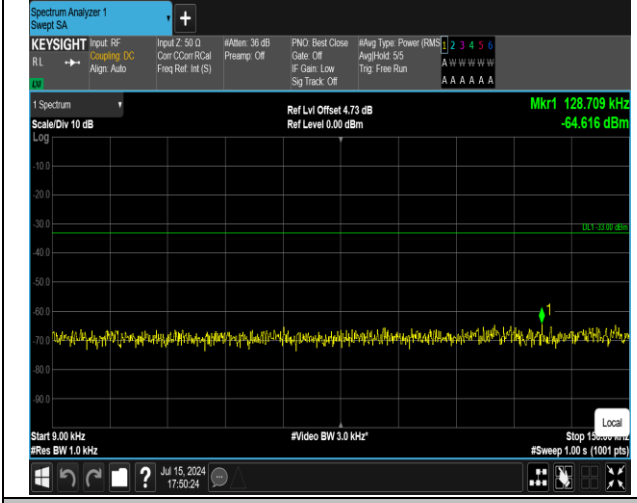
5-5-3MHz-5MHz-16QAM-16QAM-20416-20455-1RB#0-1R B#24-0.009~0.15MHz-PASS
