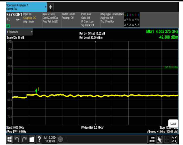
5-5-3MHz-5MHz-16QAM-16QAM-20416-20455-1RB#14-0 RB#0-3000~10000MHz-PASS
