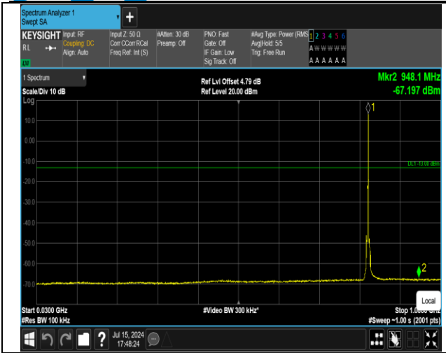
5-5-3MHz-5MHz-16QAM-16QAM-20416-20455-1RB#14-0 RB#0-30~1000MHz-PASS
