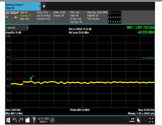
5-5-3MHz-5MHz-16QAM-16QAM-20501-20540-1RB#0-0R B#0-3000~10000MHz-PASS
