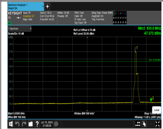
5-5-10MHz-10MHz-QPSK-QPSK-20501-20600-50RB#0-5 ORB#0-30~1000MHz-PASS
