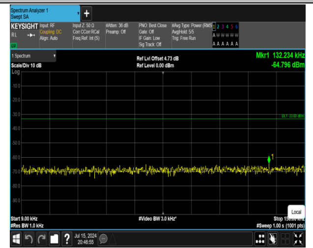
5-5-10MHz-10MHz-QPSK-QPSK-20450-20549-50RB#0-50 RB#0-0.009~0.15MHz-PASS
