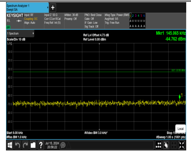
5-5-10MHz-10MHz-QPSK-QPSK-20476-20575-50RB#0-50 RB#0-0.009~0.15MHz-PASS
