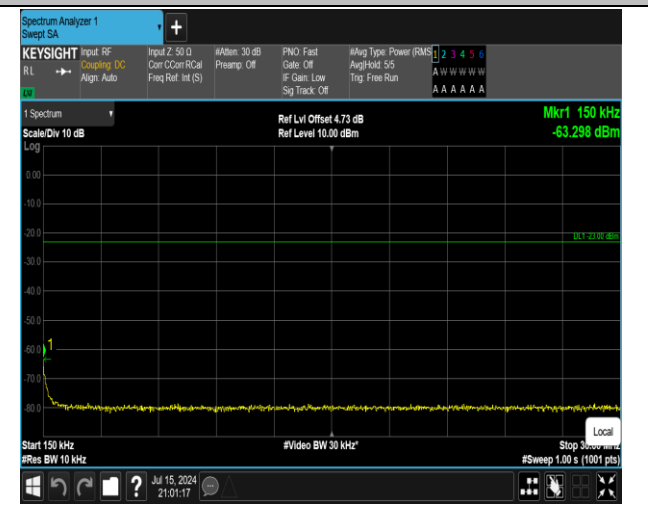
5-5-10MHz-10MHz-QPSK-QPSK-20501-20600-1RB#49-0 RB#0-0.15~30MHz-PASS
