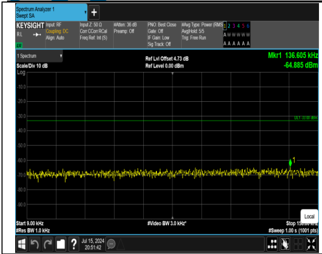
5-5-10MHz-10MHz-QPSK-QPSK-20476-20575-1RB#49-0 RB#0-0.009~0.15MHz-PASS
