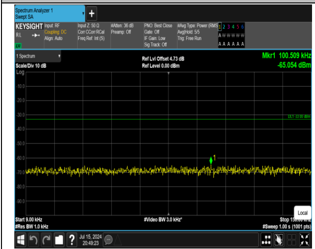
5-5-10MHz-10MHz-QPSK-QPSK-20476-20575-1RB#0-0R B#0-0.009~0.15MHz-PASS
