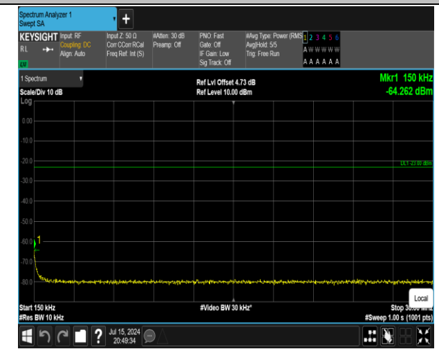
5-5-10MHz-10MHz-QPSK-QPSK-20476-20575-1RB#0-0R B#0-0.15~30MHz-PASS
