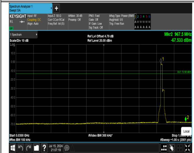
5-5-10MHz-10MHz-16QAM-16QAM-20501-20600-50RB#0 0-50RB#0-30~1000MHz-PASS
