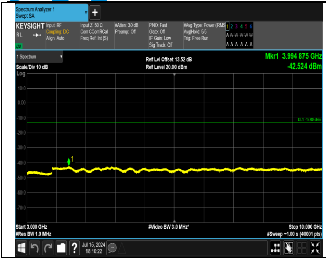
5-5-3MHz-5MHz-16QAM-16QAM-20501-20540-15RB#0-2 5RB#0-3000~10000MHz-PASS
