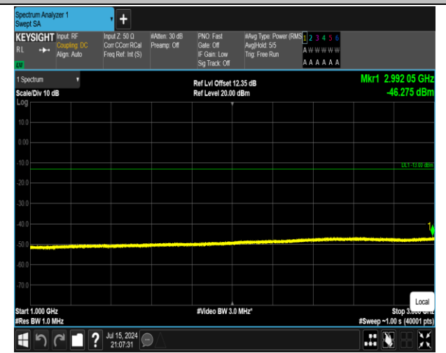
5-5-10MHz-10MHz-16QAM-16QAM-20501-20600-50RB#0 -50RB#0-1000~3000MHz-PASS
