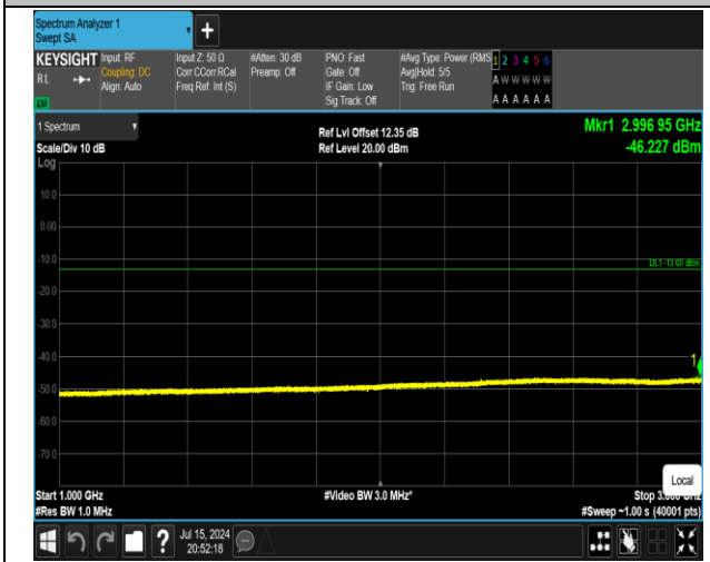
5-5-10MHz-10MHz-QPSK-QPSK-20476-20575-1RB#49-0 RB#0-1000~3000MHz-PASS
