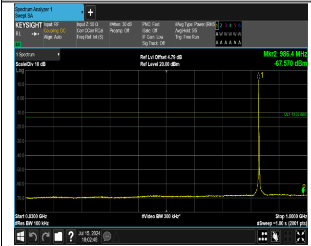
5-5-3MHz-5MHz-16QAM-16QAM-20501-20540-1RB#0-0R B#0-30~1000MHz-PASS
