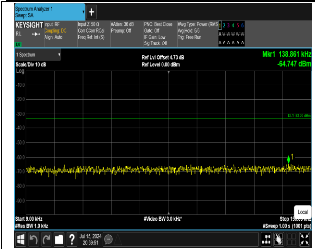
5-5-10MHz-10MHz-QPSK-QPSK-20450-20549-1RB#0-0R B#0-0.009~0.15MHz-PASS
