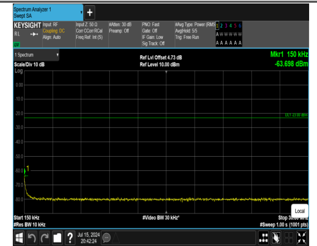
5-5-10MHz-10MHz-QPSK-QPSK-20450-20549-1RB#49-0 RB#0-0.15~30MHz-PASS
