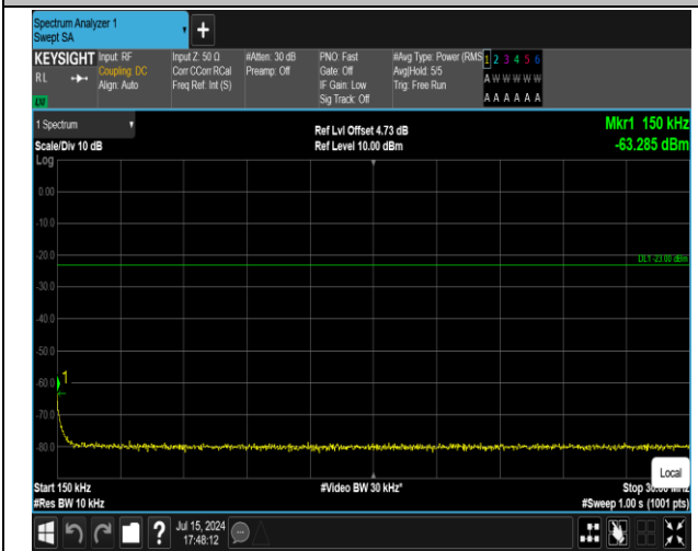
5-5-3MHz-5MHz-16QAM-16QAM-20416-20455-1RB#14-0 RB#0-0.15~30MHz-PASS
