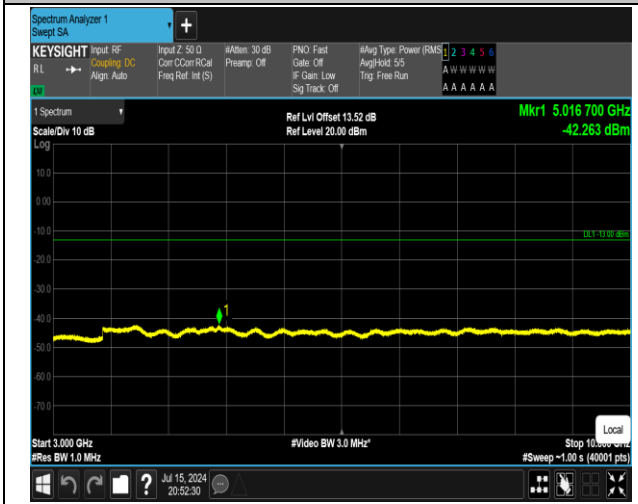
5-5-10MHz-10MHz-QPSK-QPSK-20476-20575-1RB#49-0 RB#0-3000~10000MHz-PASS
