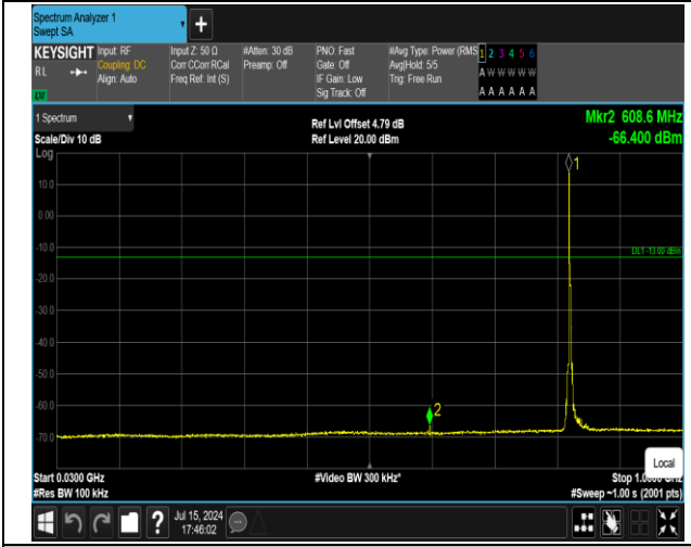
5-5-3MHz-5MHz-16QAM-16QAM-20416-20455-1RB#0-0R B#0-30~1000MHz-PASS
