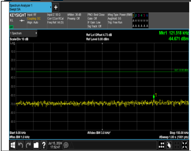
5-5-3MHz-5MHz-16QAM-16QAM-20416-20455-15RB#0-2 5RB#0-0.009~0.15MHz-PASS
