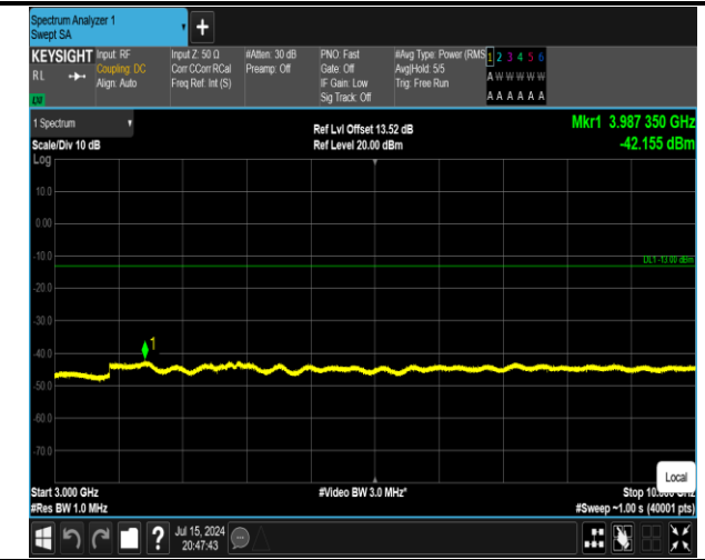
5-5-10MHz-10MHz-QPSK-QPSK-20450-20549-50RB#0-50 RB#0-3000~10000MHz-PASS
