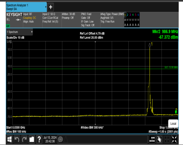
5-5-10MHz-10MHz-QPSK-QPSK-20450-20549-1RB#49-0 RB#0-30~1000MHz-PASS
