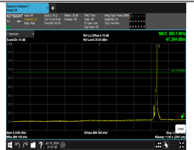
5-5-10MHz-10MHz-QPSK-QPSK-20501-20600-1RB#49-0 RB#0-30~1000MHz-PASS
