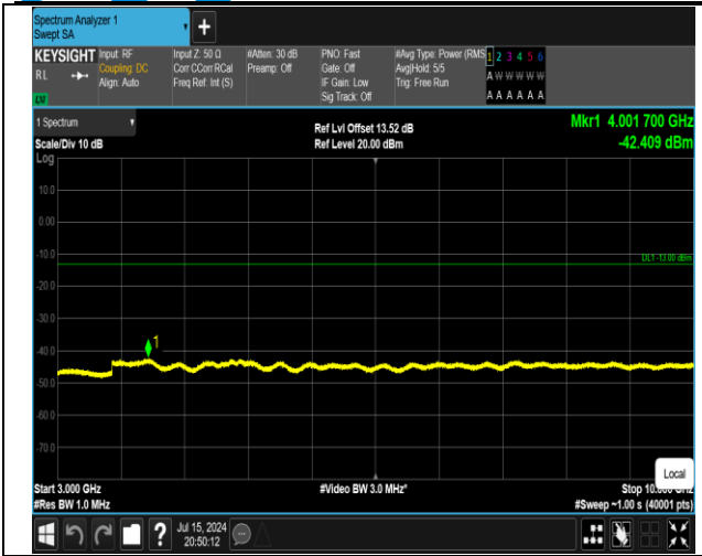
5-5-10MHz-10MHz-QPSK-QPSK-20476-20575-1RB#0-0R B#0-3000~10000MHz-PASS
