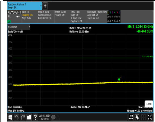
5-5-10MHz-10MHz-QPSK-QPSK-20450-20549-1RB#49-0 RB#0-1000~3000MHz-PASS
