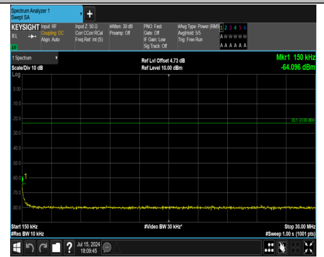
5-5-3MHz-5MHz-16QAM-16QAM-20501-20540-15RB#0-2 5RB#0-0.15~30MHz-PASS
