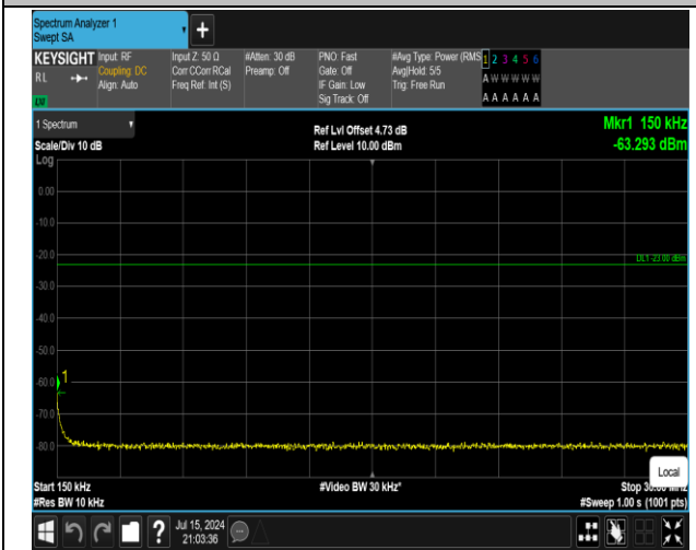
5-5-10MHz-10MHz-QPSK-QPSK-20501-20600-1RB#0-1R B#49-0.15~30MHz-PASS
