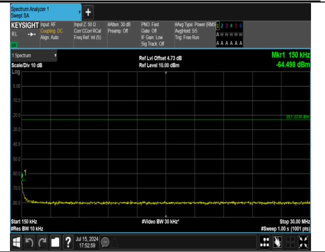
5-5-3MHz-5MHz-16QAM-16QAM-20416-20455-15RB#0-2 5RB#0-0.15~30MHz-PASS
