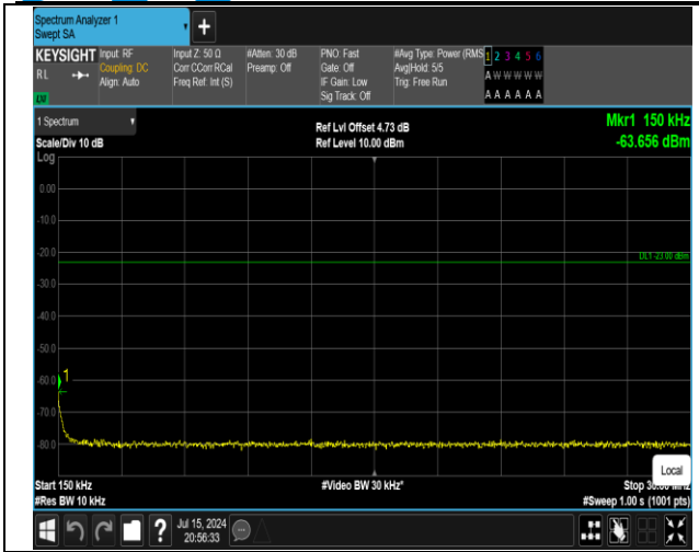
5-5-10MHz-10MHz-QPSK-QPSK-20476-20575-50RB#0-5 ORB#0-0.15~30MHz-PASS
