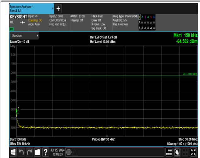
5-5-3MHz-5MHz-16QAM-16QAM-20501-20540-1RB#0-0R B#0-0.15~30MHz-PASS
