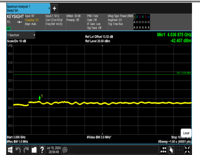
5-5-10MHz-10MHz-QPSK-QPSK-20476-20575-1RB#0-1R B#49-3000~10000MHz-PASS
