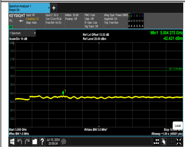
5-5-10MHz-10MHz-QPSK-QPSK-20501-20600-1RB#0-0R B#0-3000~10000MHz-PASS
