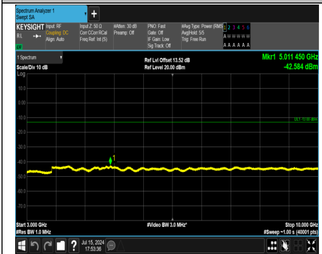
5-5-3MHz-5MHz-16QAM-16QAM-20416-20455-15RB#0-2 5RB#0-3000~10000MHz-PASS
