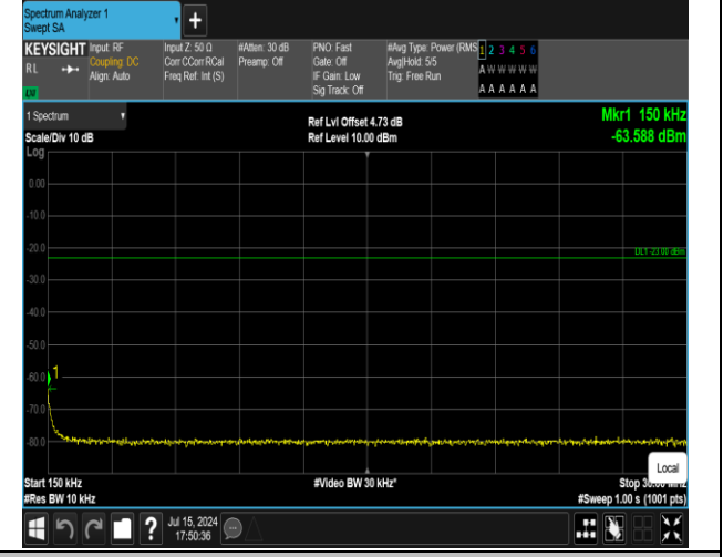
5-5-3MHz-5MHz-16QAM-16QAM-20416-20455-1RB#0-1R B#24-0.15~30MHz-PASS
