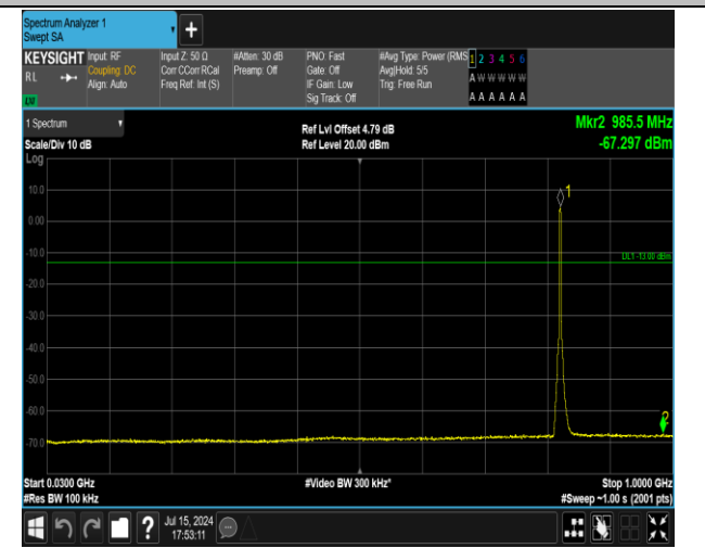
5-5-3MHz-5MHz-16QAM-16QAM-20416-20455-15RB#0-2 5RB#0-30~1000MHz-PASS
