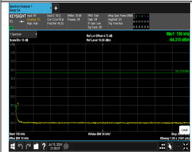
5-5-10MHz-10MHz-QPSK-QPSK-20501-20600-50RB#0-5 ORB#0-0.15~30MHz-PASS
