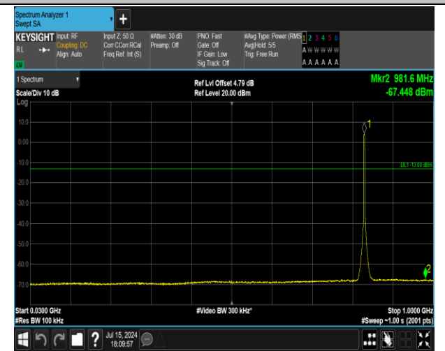
5-5-3MHz-5MHz-16QAM-16QAM-20501-20540-15RB#0-2 5RB#0-30~1000MHz-PASS
