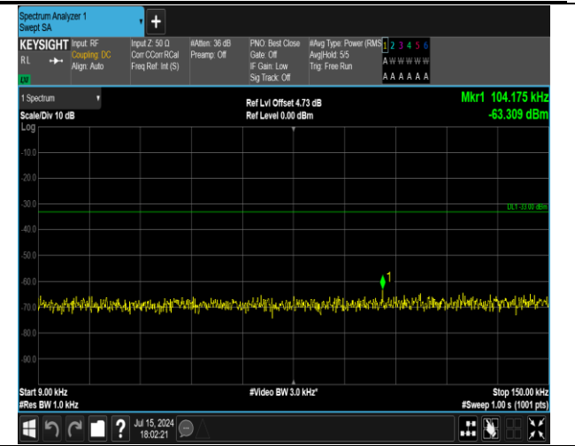
5-5-3MHz-5MHz-16QAM-16QAM-20501-20540-1RB#0-0R B#0-0.009~0.15MHz-PASS
