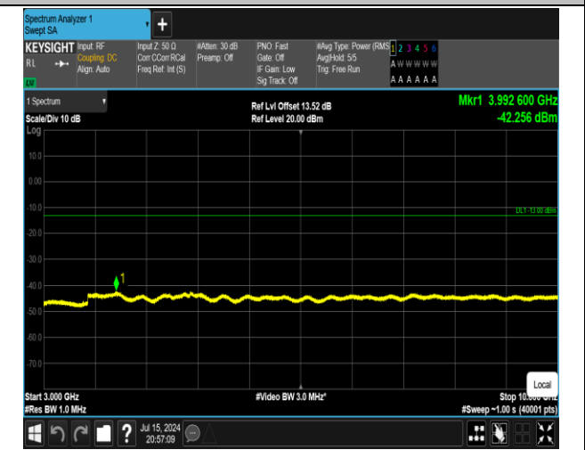
5-5-10MHz-10MHz-QPSK-QPSK-20476-20575-50RB#0-50 RB#0-3000~10000MHz-PASS
