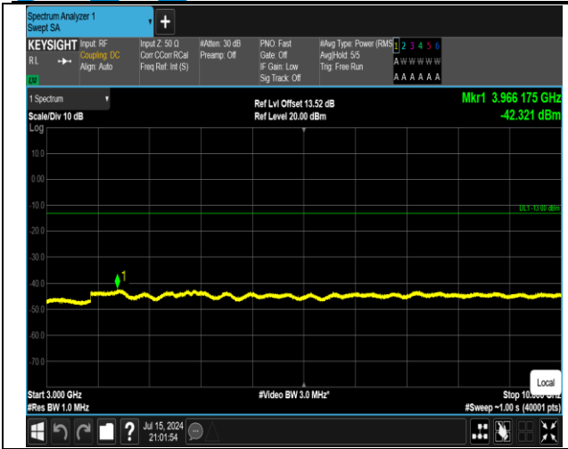
5-5-10MHz-10MHz-QPSK-QPSK-20501-20600-1RB#49-0 RB#0-3000~10000MHz-PASS
