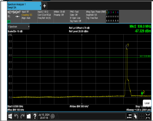
5-5-10MHz-10MHz-QPSK-QPSK-20450-20549-50RB#0-5 ORB#0-30~1000MHz-PASS
