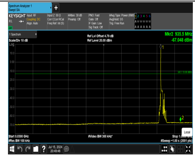
5-5-10MHz-10MHz-QPSK-QPSK-20476-20575-1RB#0-0R B#0-30~1000MHz-PASS
