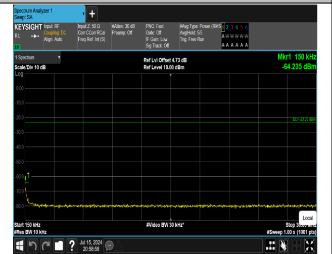
5-5-10MHz-10MHz-QPSK-QPSK-20501-20600-1RB#0-0R B#0-0.15~30MHz-PASS
