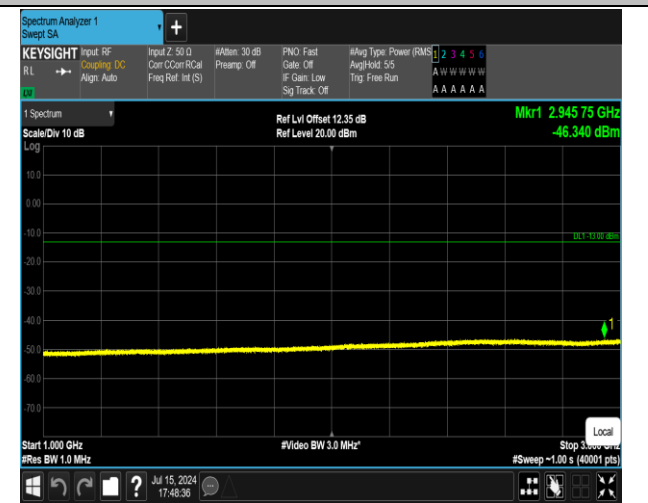
5-5-3MHz-5MHz-16QAM-16QAM-20416-20455-1RB#14-0 RB#0-1000~3000MHz-PASS
