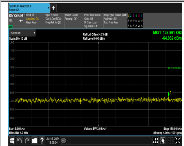
5-5-3MHz-5MHz-16QAM-16QAM-20501-20540-15RB#0-2 5RB#0-0.009~0.15MHz-PASS
