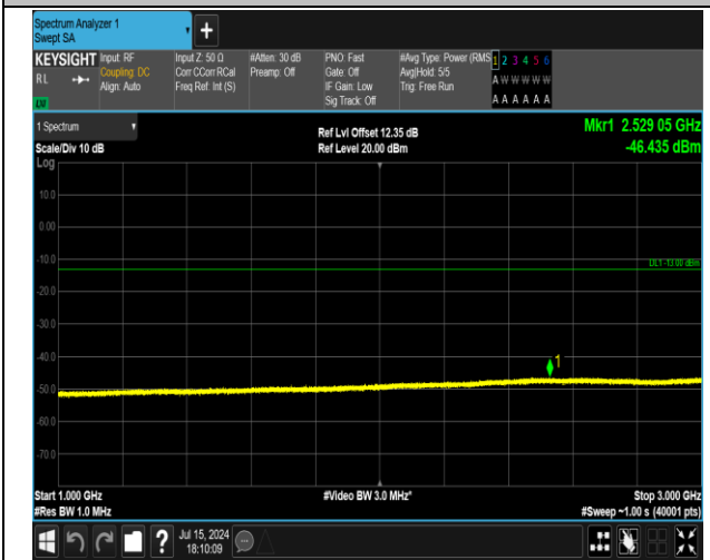
5-5-3MHz-5MHz-16QAM-16QAM-20501-20540-15RB#0-2 5RB#0-1000~3000MHz-PASS
