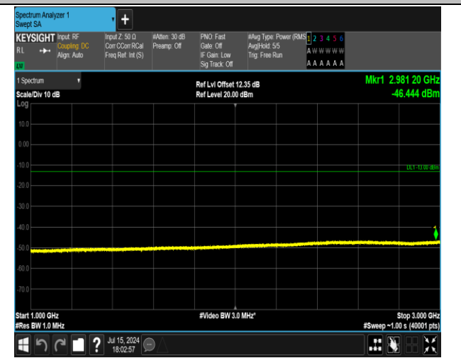
5-5-3MHz-5MHz-16QAM-16QAM-20501-20540-1RB#0-0R B#0-1000~3000MHz-PASS
