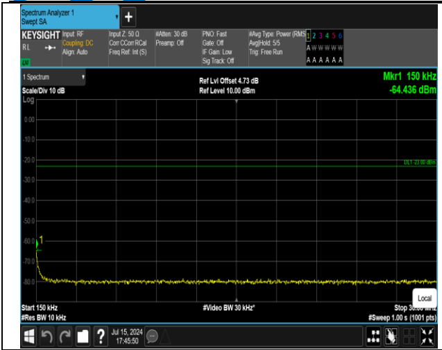
5-5-3MHz-5MHz-16QAM-16QAM-20416-20455-1RB#0-0R B#0-0.15~30MHz-PASS
