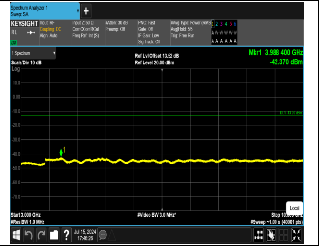
5-5-3MHz-5MHz-16QAM-16QAM-20416-20455-1RB#0-0R B#0-3000~10000MHz-PASS
