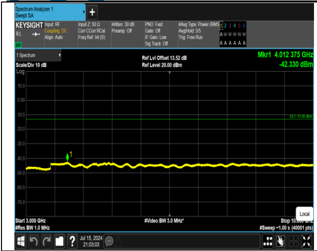
5-5-10MHz-10MHz-16QAM-16QAM-20501-20600-1RB#4 9-0RB#0-3000~10000MHz-PASS
