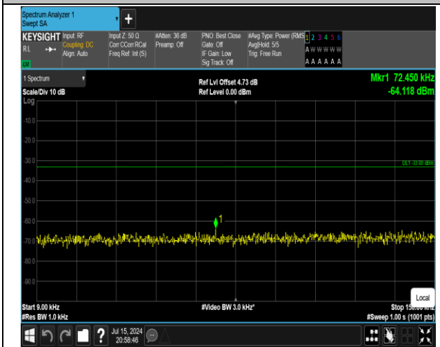
5-5-10MHz-10MHz-QPSK-QPSK-20501-20600-1RB#0-0R B#0-0.009~0.15MHz-PASS
