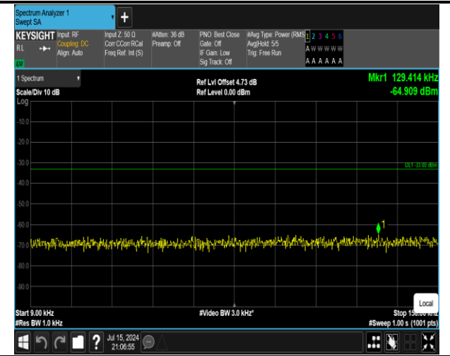
5-5-10MHz-10MHz-16QAM-16QAM-20501-20600-50RB#0 -50RB#0-0.009~0.15MHz-PASS
