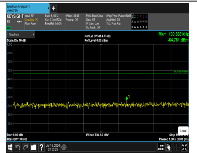
5-5-10MHz-10MHz-QPSK-QPSK-20501-20600-1RB#0-1R B#49-0.009~0.15MHz-PASS
