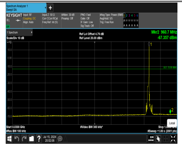
5-5-10MHz-10MHz-QPSK-QPSK-20476-20575-1RB#49-0 RB#0-30~1000MHz-PASS
