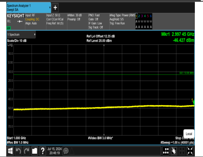
5-5-10MHz-10MHz-16QAM-16QAM-20450-20549-1RB#0-1RB#49-1000~3000MHz-PASS
