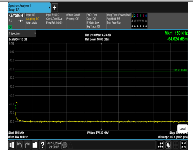
5-5-10MHz-10MHz-16QAM-16QAM-20501-20600-1RB#0-ORB#0-0.15~30MHz-PASS
