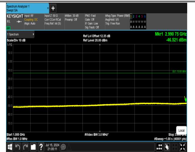
5-5-10MHz-10MHz-16QAM-16QAM-20501-20600-1RB#0-1RB#49-1000~3000MHz-PASS
