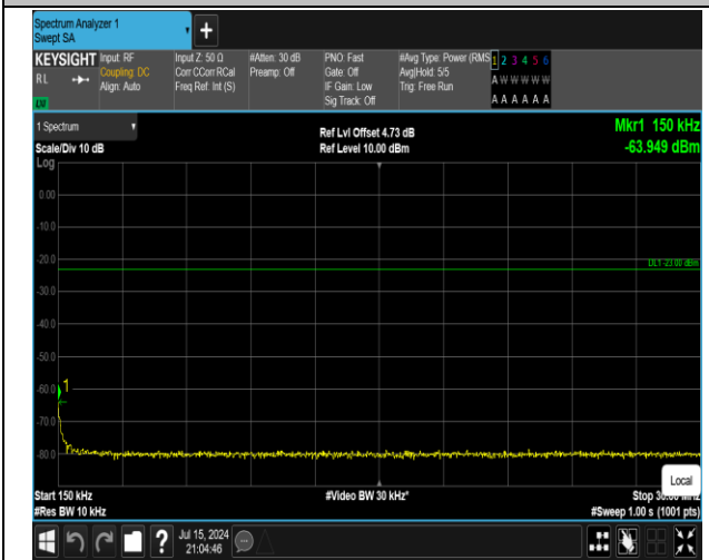
5-5-10MHz-10MHz-16QAM-16QAM-20501-20600-1RB#0-1RB#49-0.15~30MHz-PASS
