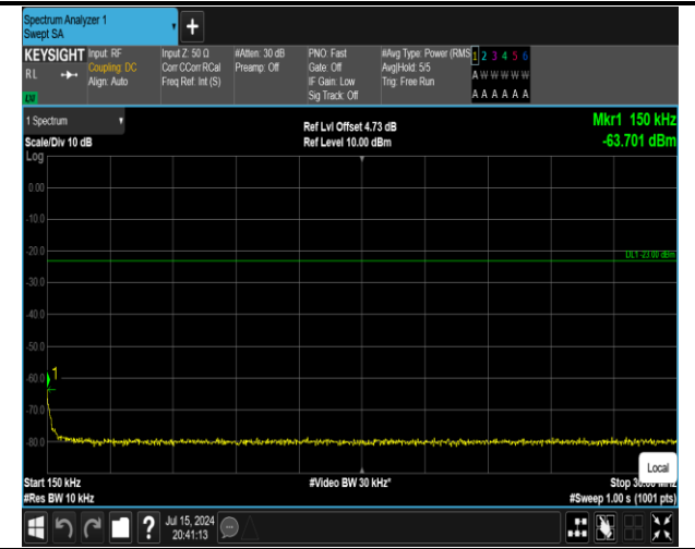
5-5-10MHz-10MHz-16QAM-16QAM-20450-20549-1RB#0-ORB#0-0.15~30MHz-PASS
