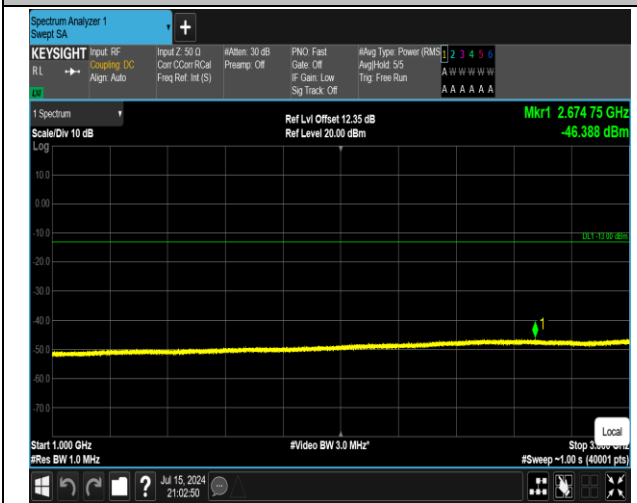
5-5-10MHz-10MHz-16QAM-16QAM-20501-20600-1RB#49-0RB#0-1000~3000MHz-PASS
