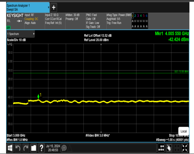
5-5-10MHz-10MHz-16QAM-16QAM-20450-20549-50RB#0-50RB#0-3000~10000MHz-PASS
