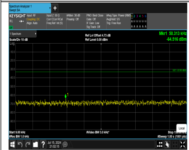
5-5-10MHz-10MHz-16QAM-16QAM-20501-20600-1RB#49-0RB#0-0.009~0.15MHz-PASS
