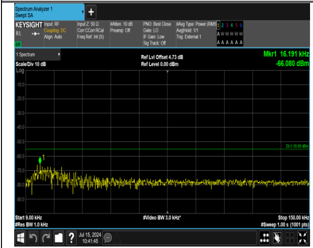
41(2555-2655)-41(2555-2655)-5MHz-20MHz-16QAM-16Q AM-40273-40390-1RB#24-0RB#0-0.009~0.15MHz-PASS
