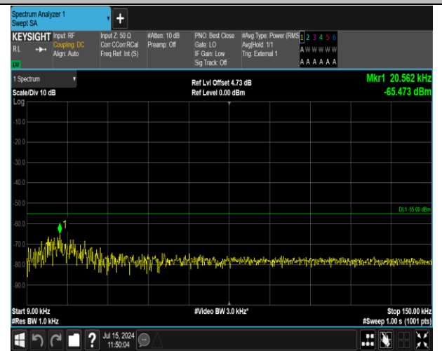
41(2555-2655)-41(2555-2655)-20MHz-5MHz-16QAM-16Q AM-40340-40457-1RB#0-0RB#0-0.009~0.15MHz-PASS
