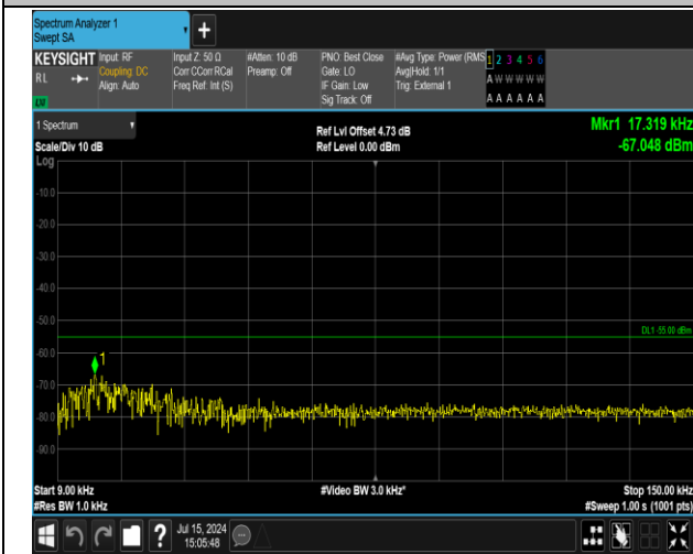
41(2555-2655)-41(2555-2655)-20MHz-20MHz-16QAM-16 QAM-40340-40538-100RB#0-100RB#0-0.009~0.15MHz-P ASS
