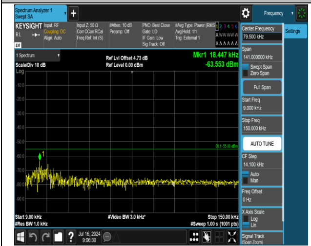
38-38-20MHz-20MHz-QPSK-QPSK-37901-38099-1RB#0-1RB#99-0.009~0.15MHz-PASS
