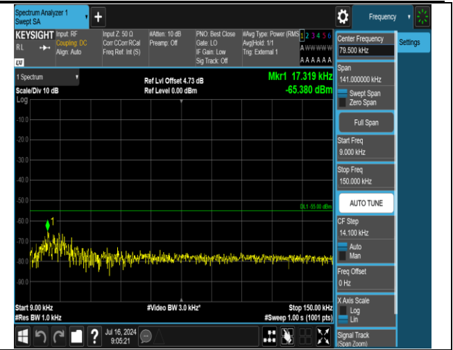
38-38-20MHz-20MHz-QPSK-QPSK-37901-38099-1RB#99-ORB#0-0.009~0.15MHz-PASS
