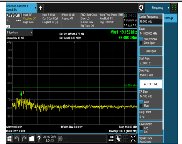
38-38-20MHz-20MHz-QPSK-QPSK-37901-38099-1RB#0-0 RB#0-0.009~0.15MHz-PASS
