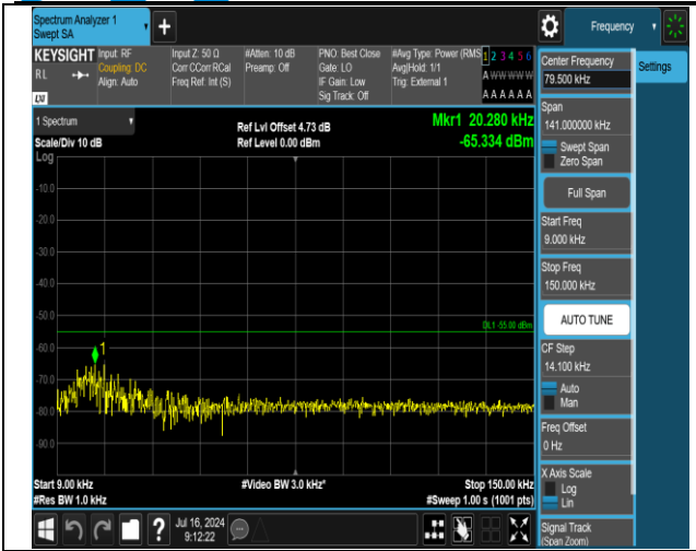
38-38-20MHz-20MHz-QPSK-QPSK-37952-38150-100RB# 0-100RB#0-0.009~0.15MHz-PASS
