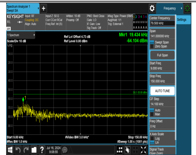
38-38-20MHz-20MHz-QPSK-QPSK-37952-38150-1RB#0-0 RB#0-0.009~0.15MHz-PASS
