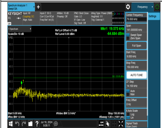
38-38-20MHz-20MHz-16QAM-16QAM-37901-38099-100R B#0-100RB#0-0.009~0.15MHz-PASS
