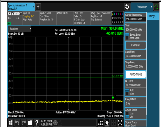
38-38-20MHz-20MHz-16QAM-16QAM-37952-38150-100R B#0-100RB#0-30~1000MHz-PASS
