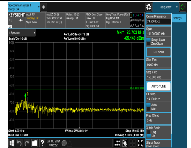
38-38-20MHz-20MHz-16QAM-16QAM-37901-38099-1RB# 99-ORB#0-0.009~0.15MHz-PASS
