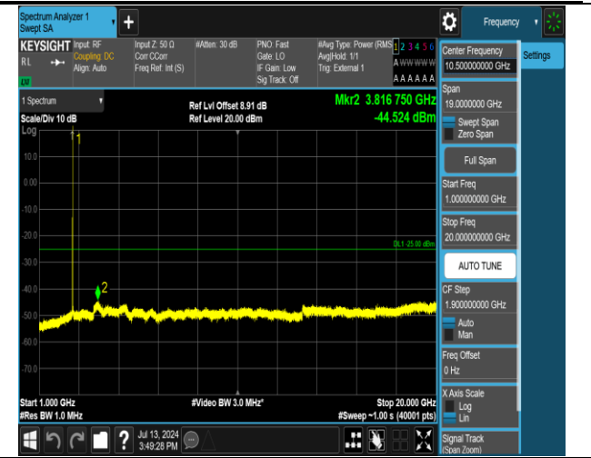
38-38-20MHz-20MHz-QPSK-QPSK-37850-38048-1RB#99- ORB#0-1000~20000MHz-PASS
