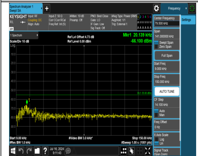
38-38-20MHz-20MHz-16QAM-16QAM-37952-38150-1RB #0-1RB#99-0.009~0.15MHz-PASS
