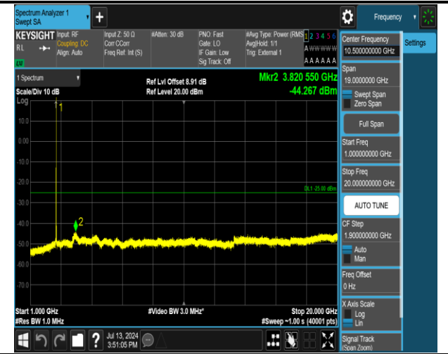
38-38-20MHz-20MHz-16QAM-16QAM-37850-38048-1RB# 99-ORB#0-1000~20000MHz-PASS
