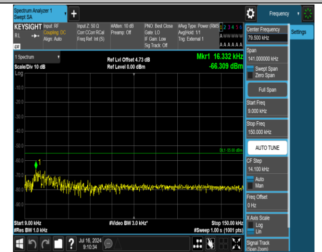
38-38-20MHz-20MHz-16QAM-16QAM-37952-38150-1RB# 99-0RB#0-0.009~0.15MHz-PASS
