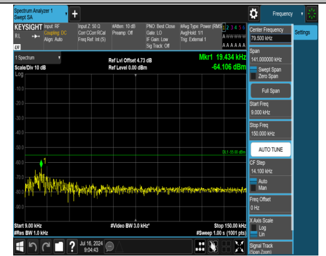
38-38-20MHz-20MHz-16QAM-16QAM-37901-38099-1RB# 0-0-ORB#0-0.009~0.15MHz-PASS
