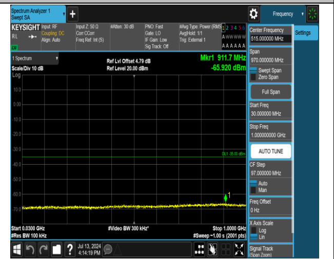
38-38-20MHz-20MHz-16QAM-16QAM-37952-38150-1RB# 0-ORB#0-30~1000MHz-PASS
