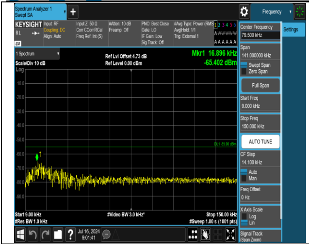
38-38-20MHz-20MHz-QPSK-QPSK-37850-38048-1RB#0-1RB#99-0.009~0.15MHz-PASS
