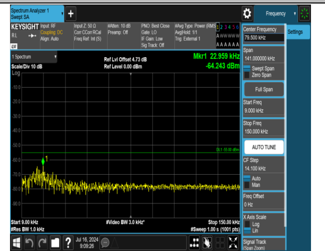
38-38-20MHz-20MHz-16QAM-16QAM-37952-38150-1RB# 0-0RB#0-0.009~0.15MHz-PASS
