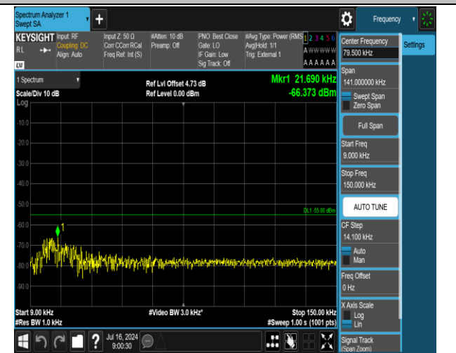
38-38-20MHz-20MHz-QPSK-QPSK-37850-38048-1RB#99-ORB#0-0.009~0.15MHz-PASS
