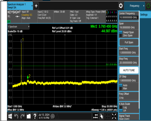
38-38-20MHz-20MHz-16QAM-16QAM-37901-38099-100R B#0-100RB#0-1000~20000MHz-PASS
