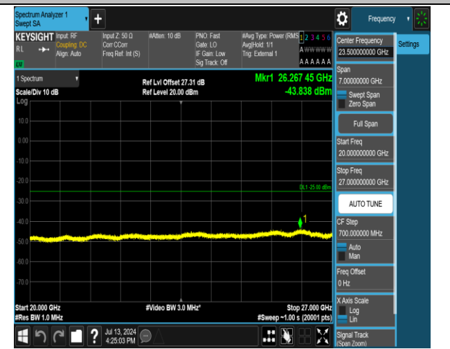
38-38-20MHz-20MHz-16QAM-16QAM-37952-38150-100R B#0-100RB#0-20000~27000MHz-PASS
