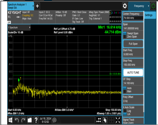
38-38-20MHz-20MHz-16QAM-16QAM-37952-38150-100R B#0-100RB#0-0.009~0.15MHz-PASS
