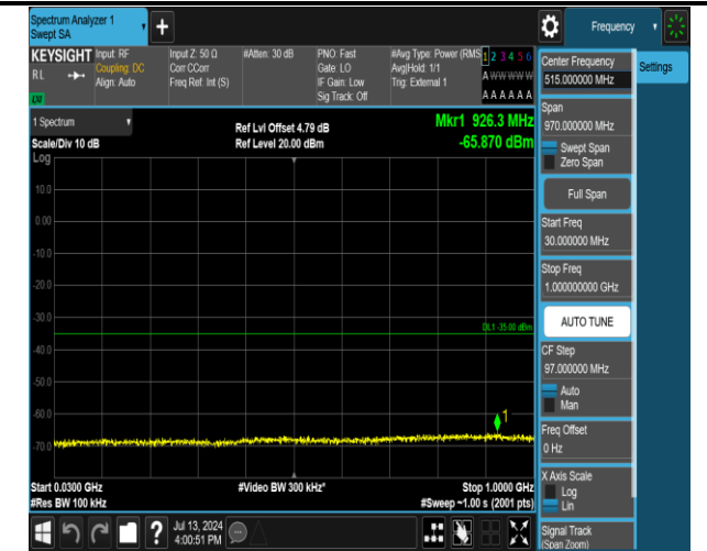
38-38-20MHz-20MHz-16QAM-16QAM-37901-38099-1RB# 0-0RB#0-30~1000MHz-PASS
