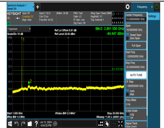
38-38-20MHz-20MHz-16QAM-16QAM-37901-38099-1RB# 99-ORB#0-1000~20000MHz-PASS
