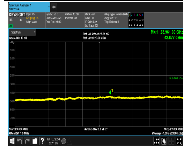
38-38-15MHz-15MHz-QPSK-QPSK-38025-38175-75RB#0-75RB#0-20000~27000MHz-PASS
