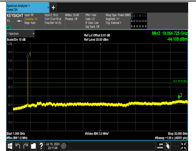
38-38-15MHz-15MHz-QPSK-QPSK-38025-38175-75RB#0- 75RB#0-1000~20000MHz-PASS
