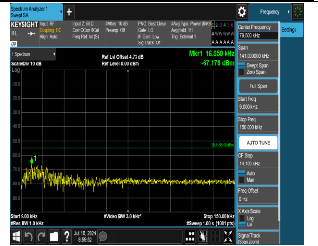
38-38-20MHz-20MHz-16QAM-16QAM-37850-38048-1RB# 0-0RB#0-0.009~0.15MHz-PASS
