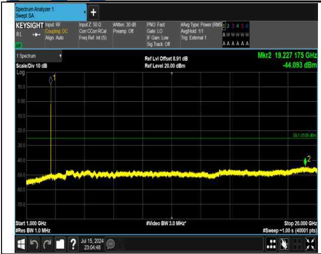
38-38-15MHz-15MHz-16QAM-16QAM-38025-38175-1RB #74-ORB#0-1000~20000MHz-PASS
