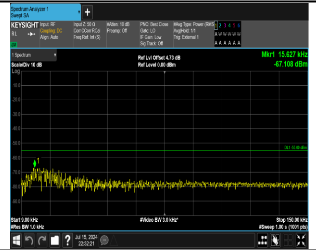
38-38-15MHz-15MHz-QPSK-QPSK-37825-37975-1RB#0-1RB#74-0.009~0.15MHz-PASS
