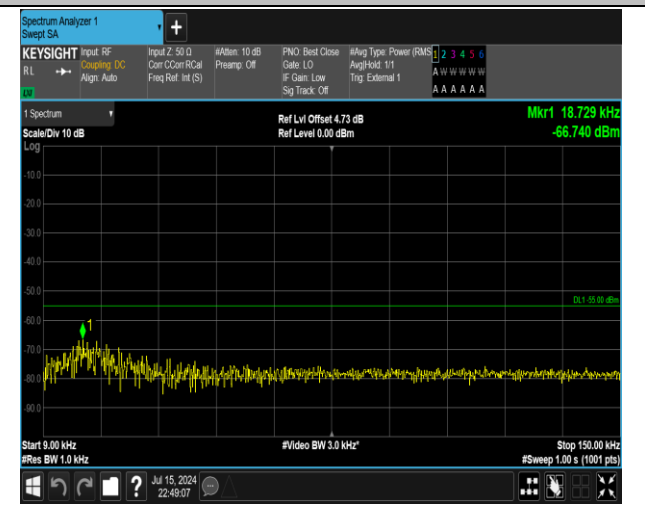
38-38-15MHz-15MHz-QPSK-QPSK-37925-38075-1RB#0-1RB#74-0.009~0.15MHz-PASS
