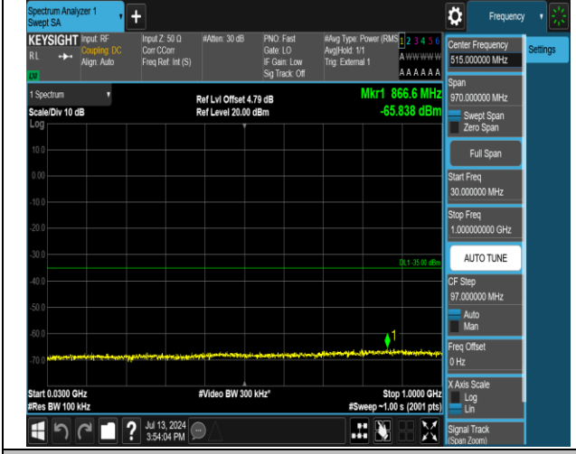
38-38-20MHz-20MHz-16QAM-16QAM-37850-38048-1RB #0-1RB#99-30~1000MHz-PASS
