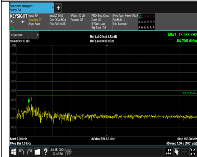
38-38-15MHz-15MHz-QPSK-QPSK-37925-38075-1RB#0-ORB#0-0.009~0.15MHz-PASS
