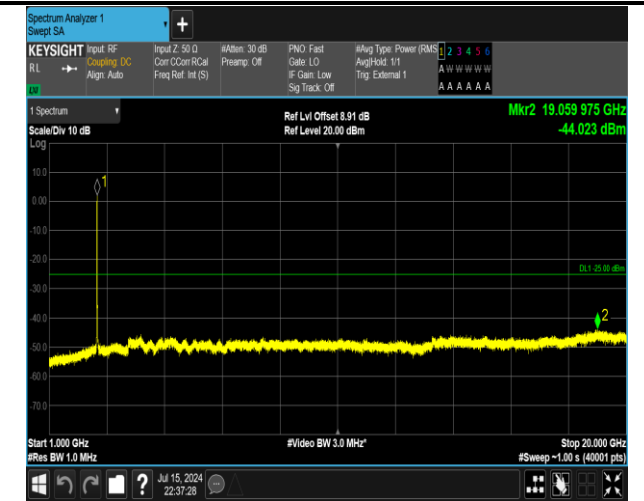
38-38-15MHz-15MHz-QPSK-QPSK-37825-37975-75RB#0-75RB#0-1000~20000MHz-PASS
