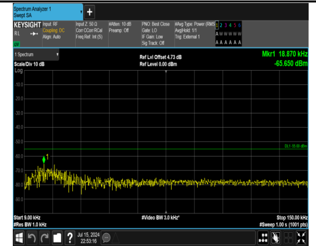
38-38-15MHz-15MHz-QPSK-QPSK-37925-38075-75RB#0- 75RB#0-0.009~0.15MHz-PASS
