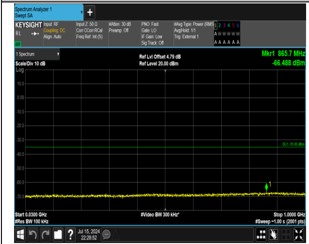
38-38-15MHz-15MHz-QPSK-QPSK-37825-37975-1RB#74 -ORB#0-30~1000MHz-PASS
