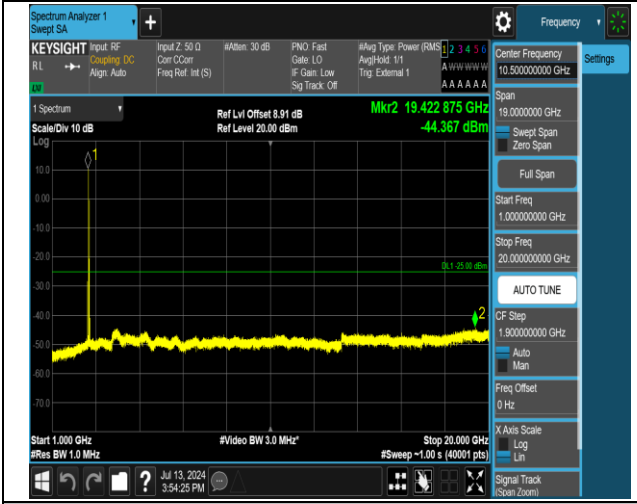
38-38-20MHz-20MHz-16QAM-16QAM-37850-38048-1RB #0-1RB#99-1000~20000MHz-PASS
