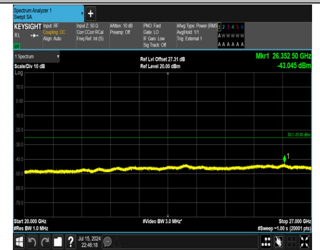
38-38-15MHz-15MHz-QPSK-QPSK-37925-38075-1RB#74-0RB#0-20000~27000MHz-PASS
