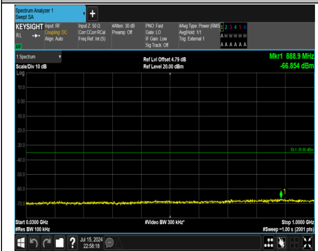
38-38-15MHz-15MHz-QPSK-QPSK-38025-38175-1RB#0-ORB#0-30~1000MHz-PASS
