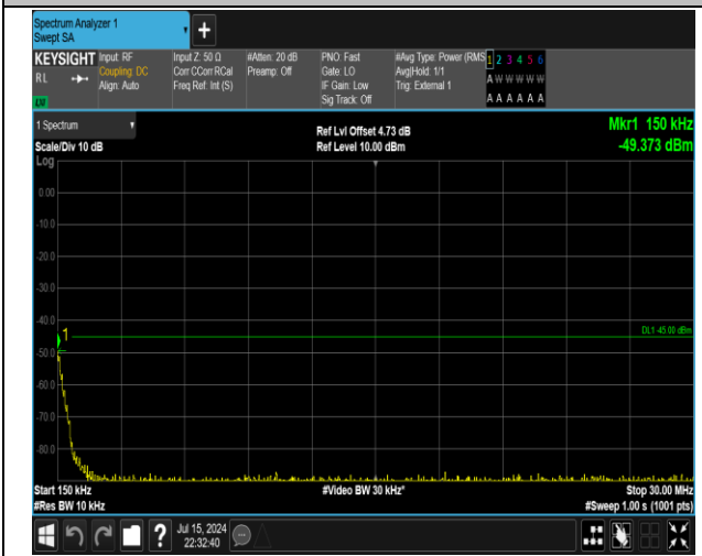
38-38-15MHz-15MHz-QPSK-QPSK-37825-37975-1RB#0-1RB#74-0.15~30MHz-PASS
