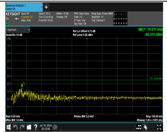
38-38-15MHz-15MHz-16QAM-16QAM-38025-38175-75RB #0-75RB#0-0.009~0.15MHz-PASS
