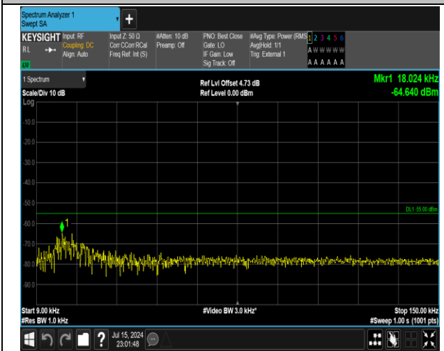
38-38-15MHz-15MHz-QPSK-QPSK-38025-38175-1RB#74-ORB#0-0.009~0.15MHz-PASS
