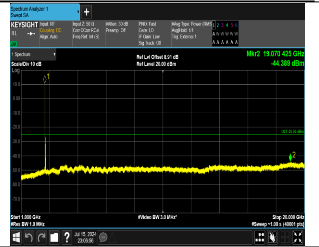
38-38-15MHz-15MHz-QPSK-QPSK-38025-38175-1RB#0-1RB#74-1000~20000MHz-PASS
