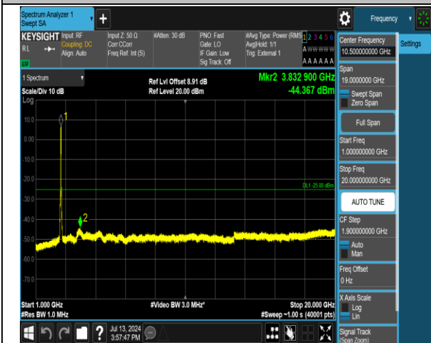
38-38-20MHz-20MHz-16QAM-16QAM-37850-38048-100R B#0-100RB#0-1000~20000MHz-PASS
