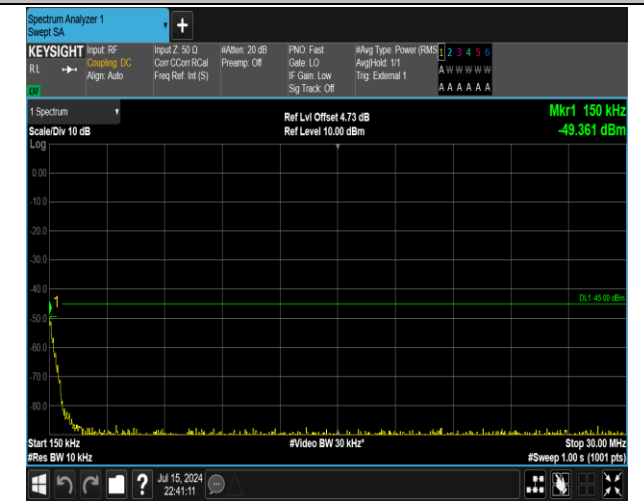
38-38-15MHz-15MHz-QPSK-QPSK-37925-38075-1RB#0-ORB#0-0.15~30MHz-PASS
