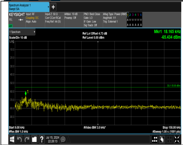
38-38-15MHz-15MHz-QPSK-QPSK-37825-37975-1RB#74 -ORB#0-0.009~0.15MHz-PASS
