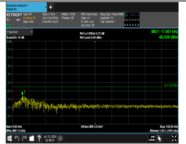
38-38-15MHz-15MHz-QPSK-QPSK-37825-37975-75RB#0- 75RB#0-0.009~0.15MHz-PASS
