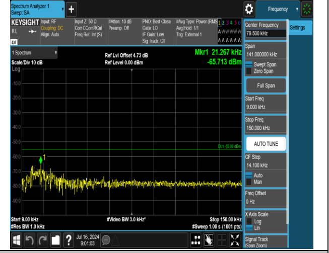
38-38-20MHz-20MHz-16QAM-16QAM-37850-38048-1RB# 99-0RB#0-0.009~0.15MHz-PASS
