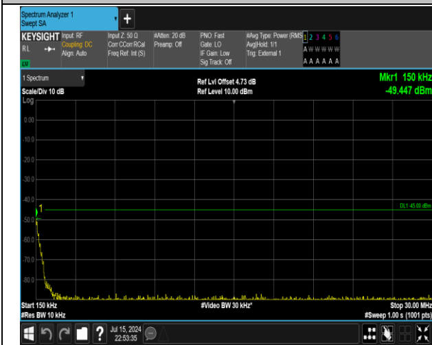
38-38-15MHz-15MHz-QPSK-QPSK-37925-38075-75RB#0 -75RB#0-0.15~30MHz-PASS
