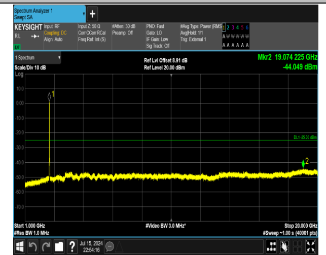
38-38-15MHz-15MHz-QPSK-QPSK-37925-38075-75RB#0- 75RB#0-1000~20000MHz-PASS
