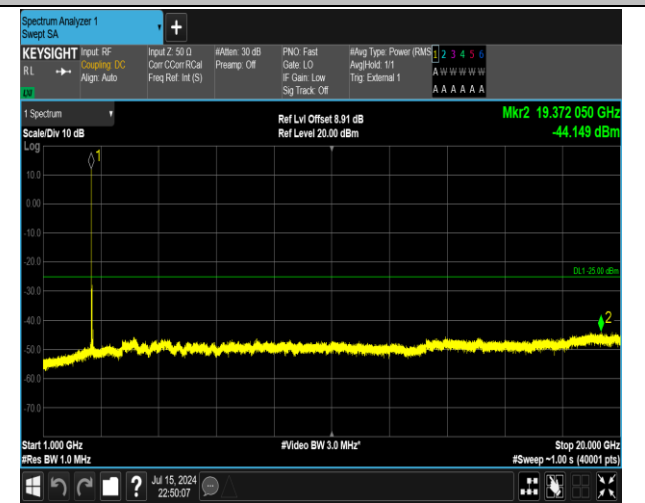
38-38-15MHz-15MHz-QPSK-QPSK-37925-38075-1RB#0-1RB#74-1000~20000MHz-PASS
