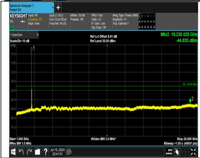
38-38-15MHz-15MHz-QPSK-QPSK-37925-38075-1RB#0-ORB#0-1000~20000MHz-PASS
