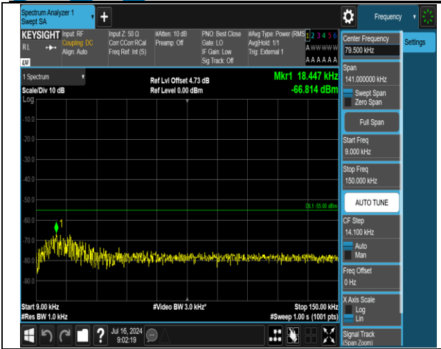
38-38-20MHz-20MHz-16QAM-16QAM-37850-38048-1RB #0-1RB#99-0.009~0.15MHz-PASS
