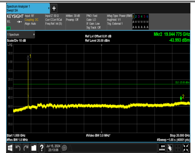
38-38-15MHz-15MHz-16QAM-16QAM-38025-38175-75RB #0-75RB#0-1000~20000MHz-PASS
