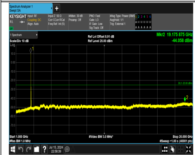
38-38-15MHz-15MHz-QPSK-QPSK-38025-38175-1RB#0-ORB#0-1000~20000MHz-PASS
