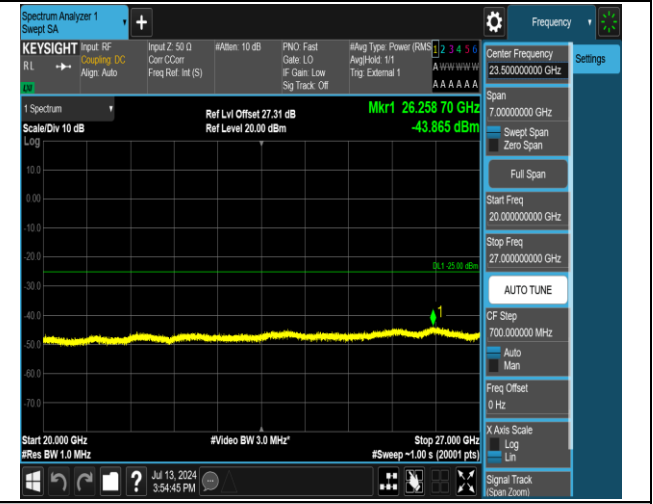
38-38-20MHz-20MHz-16QAM-16QAM-37850-38048-1RB# 0-1RB#99-20000~27000MHz-PASS
