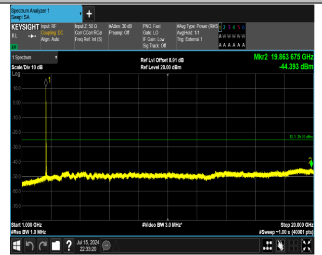
38-38-15MHz-15MHz-QPSK-QPSK-37825-37975-1RB#0-1RB#74-1000~20000MHz-PASS
