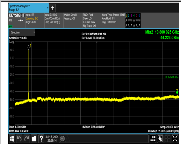
38-38-15MHz-15MHz-QPSK-QPSK-37825-37975-1RB#74 -ORB#0-1000~20000MHz-PASS
