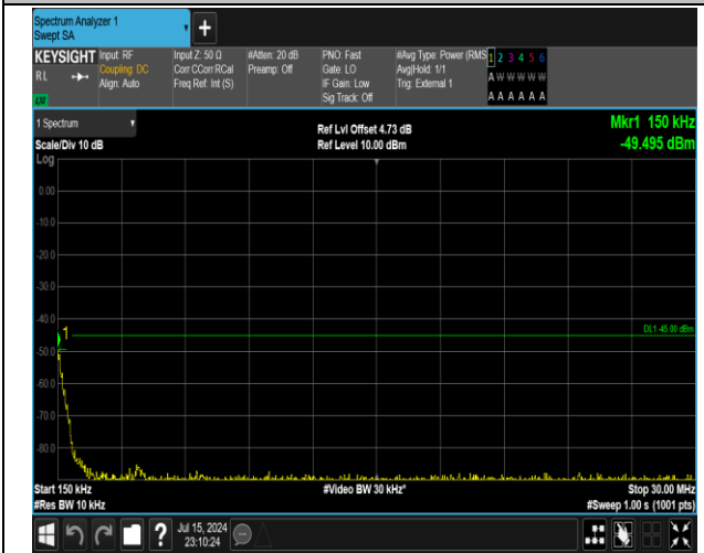
38-38-15MHz-15MHz-QPSK-QPSK-38025-38175-75RB#0 -75RB#0-0.15~30MHz-PASS
