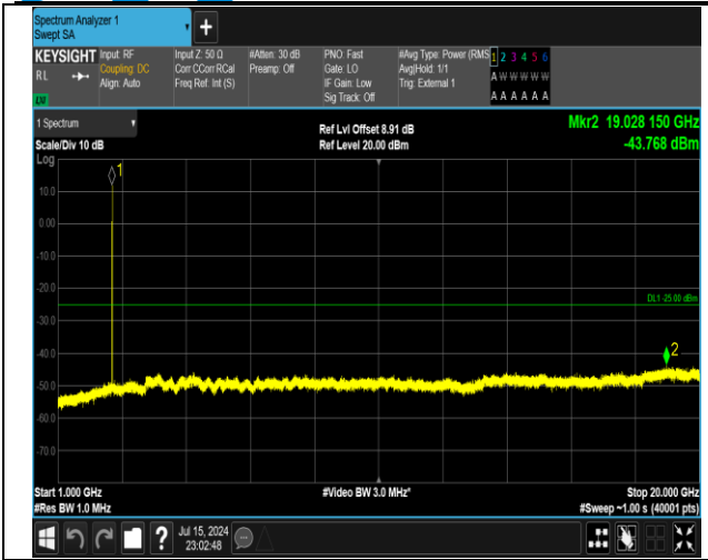
38-38-15MHz-15MHz-QPSK-QPSK-38025-38175-1RB#74 -ORB#0-1000~20000MHz-PASS
