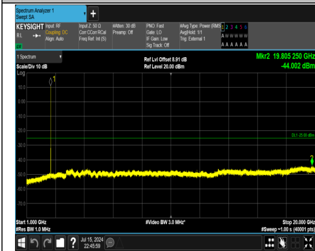
38-38-15MHz-15MHz-QPSK-QPSK-37925-38075-1RB#74-0RB#0-1000~20000MHz-PASS
