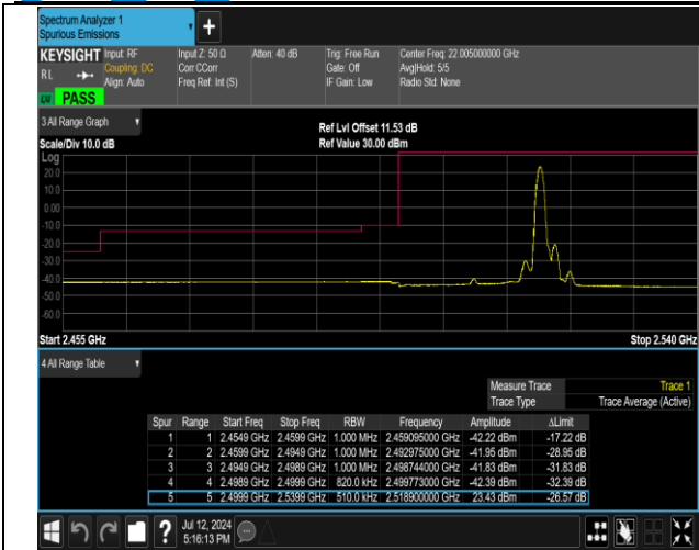
7-7-20MHz-20MHz-QPSK@QPSK-QPSK@QPSK-20850-2 1048-1RB#99@100RB#0-0RB#0@100RB#0-PASS
