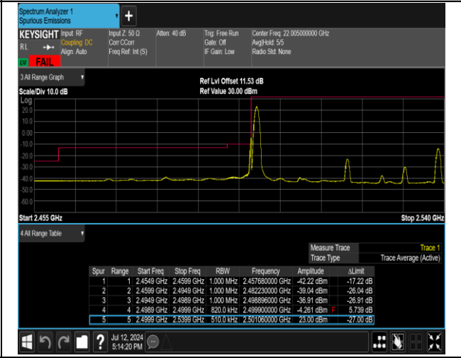
7-7-20MHz-20MHz-QPSK@QPSK-QPSK@QPSK-20850-21048-1RB#0@100RB#0-0RB#0@100RB#0-FAIL
