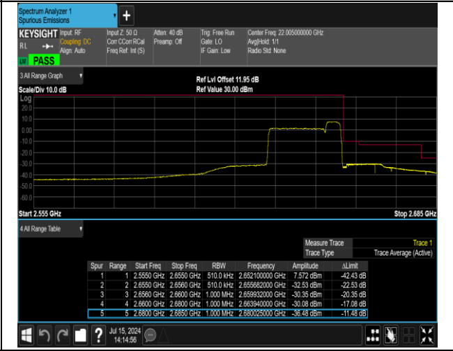
41(2555-2655)-41(2555-2655)-20MHz-5MHz-16QAM@16 QAM-16QAM@16QAM-41090-41207-100RB#0@100RB#0-25RB#0@25RB#0-PASS
