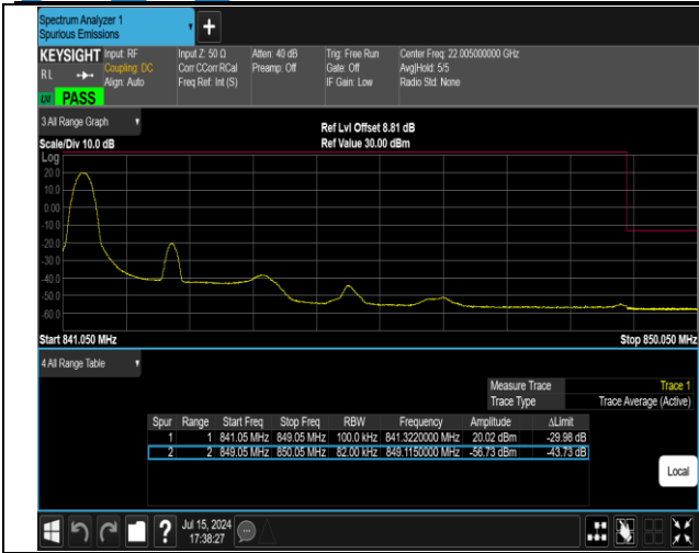
5-5-3MHz-5MHz-QPSK@QPSK-QPSK@QPSK-20586-206 25-1RB#0@15RB#0-0RB#0@25RB#0-PASS
