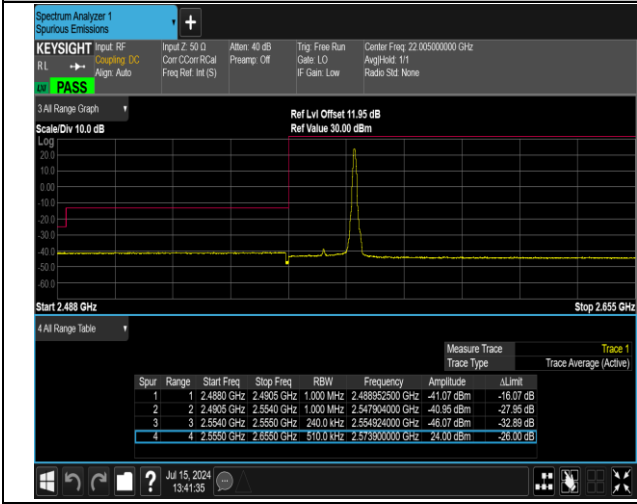
41(2555-2655)-41(2555-2655)-20MHz-5MHz-16QAM@16 QAM-16QAM@16QAM-40340-40475-1RB#99@100RB#0-0RB#0@25RB#0-PASS
