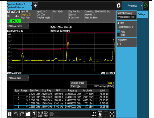
38-38-20MHz-20MHz-QPSK@QPSK-QPSK@QPSK-378 50-38048-1RB#0@100RB#0-1RB#99@100RB#0-PASS
