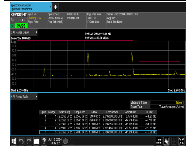
41(2555-2655)-41(2555-2655)-20MHz-20MHz-16QAM@16 QAM-16QAM@16QAM-40942-41140-1RB#0@100RB#0-1 RB#99@100RB#0-PASS
