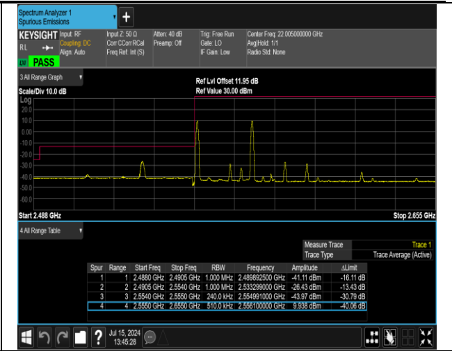
41(2555-2655)-41(2555-2655)-20MHz-5MHz-16QAM@16 QAM-16QAM@16QAM-40340-40475-1RB#0@100RB#0-1RB#24@25RB#0-PASS
