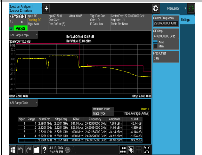
38-38-20MHz-20MHz-QPSK@QPSK-QPSK@QPSK-379 52-38150-100RB#0@100RB#0-100RB#0@100RB#0-PA SS
