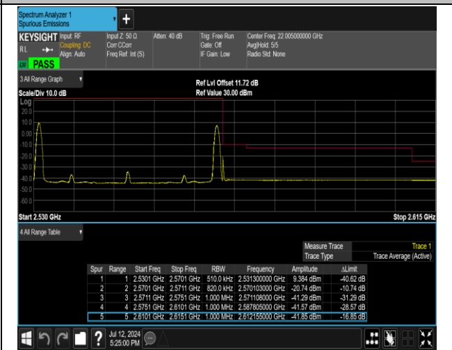
7-7-20MHz-20MHz-QPSK@QPSK-QPSK@QPSK-21152- 21350-1RB#0@100RB#0-1RB#99@100RB#0-PASS
