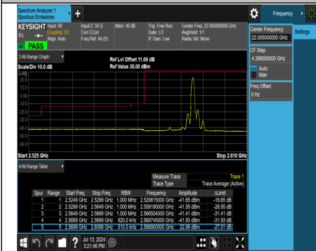
38-38-20MHz-20MHz-QPSK@QPSK-QPSK@QPSK-37850 -38048-1RB#0@100RB#0-0RB#0@100RB#0-PASS
