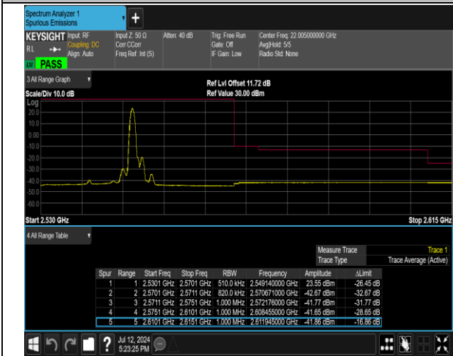
7-7-20MHz-20MHz-QPSK@QPSK-QPSK@QPSK-21152-2 1350-1RB#99@100RB#0-0RB#0@100RB#0-PASS
