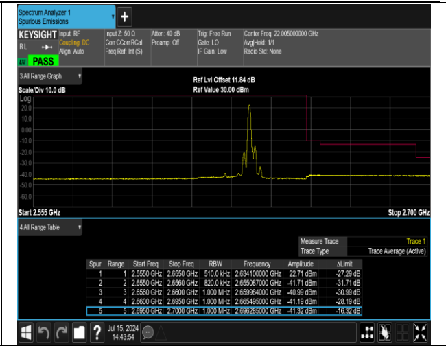
41(2555-2655)-41(2555-2655)-20MHz-20MHz-16QAM@16 QAM-16QAM@16QAM-40942-41140-1RB#99@100RB#0-0RB#0@100RB#0-PASS
