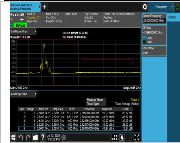
38-38-20MHz-20MHz-QPSK@QPSK-QPSK@QPSK-37952 -38150-1RB#99@100RB#0-0RB#0@100RB#0-PASS
