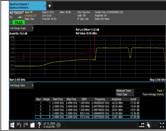
7-7-20MHz-20MHz-QPSK@QPSK-QPSK@QPSK-20850-2 1048-100RB#0@100RB#0-100RB#0@100RB#0-PASS
