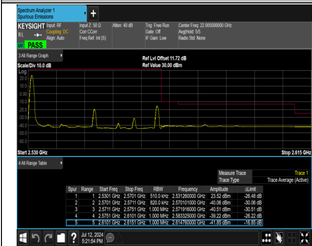
7-7-20MHz-20MHz-QPSK@QPSK-QPSK@QPSK-21152-2 1350-1RB#0@100RB#0-0RB#0@100RB#0-PASS
