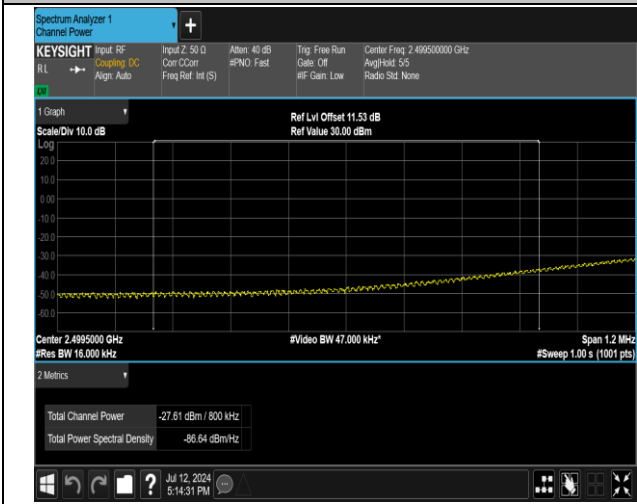
7-7-20MHz-20MHz-QPSK@QPSK-QPSK@QPSK-20850-2 1048-1RB#0@100RB#0-0RB#0@100RB#0-PASS_Final1
