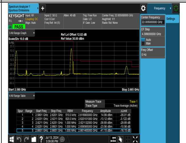
38-38-20MHz-20MHz-QPSK@QPSK-QPSK@QPSK-379 52-38150-1RB#0@100RB#0-1RB#99@100RB#0-PASS
