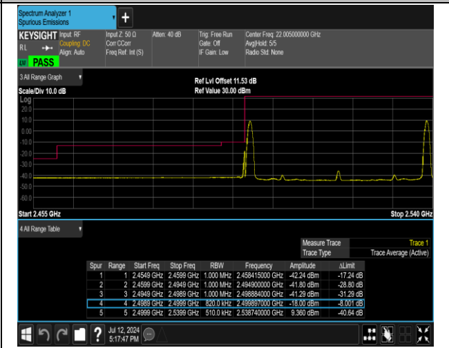
7-7-20MHz-20MHz-QPSK@QPSK-QPSK@QPSK-20850-21048-1RB#0@100RB#0-1RB#99@100RB#0-PASS
