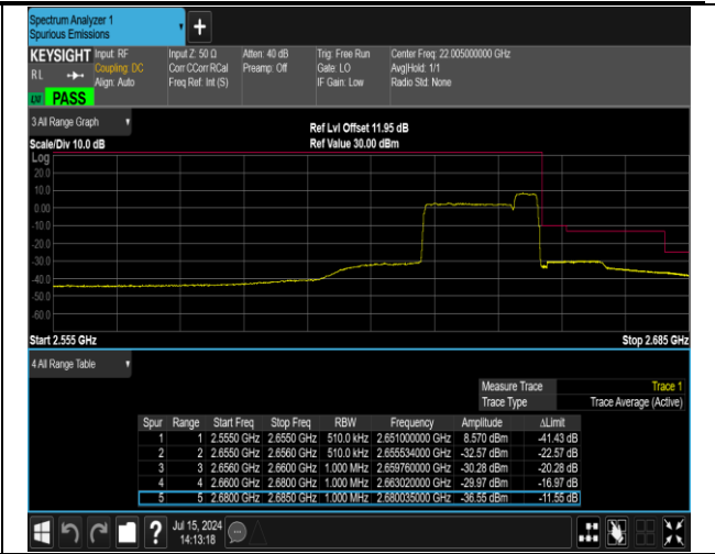
41(2555-2655)-41(2555-2655)-20MHz-5MHz-QPSK@QP SK-QPSK@QPSK-41090-41207-100RB#0@100RB#0-25 RB#0@25RB#0-PASS
