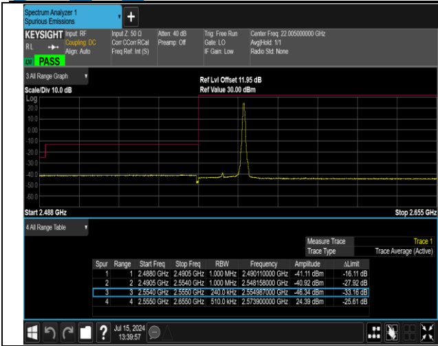
41(2555-2655)-41(2555-2655)-20MHz-5MHz-QPSK@QPS K-QPSK@QPSK-40340-40475-1RB#99@100RB#0-0RB#0 @25RB#0-PASS
