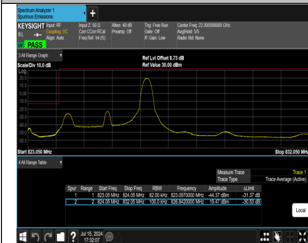
5-5-3MHz-5MHz-16QAM@16QAM-16QAM@16QAM-2041 6-20455-1RB#14@15RB#0-0RB#0@25RB#0-PASS
