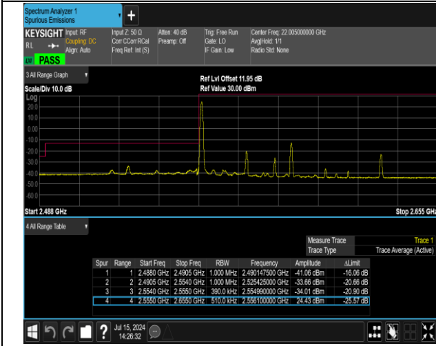
41(2555-2655)-41(2555-2655)-20MHz-20MHz-QPSK@QP SK-QPSK@QPSK-40340-40538-1RB#0@100RB#0-0RB#0 @100RB#0-PASS
