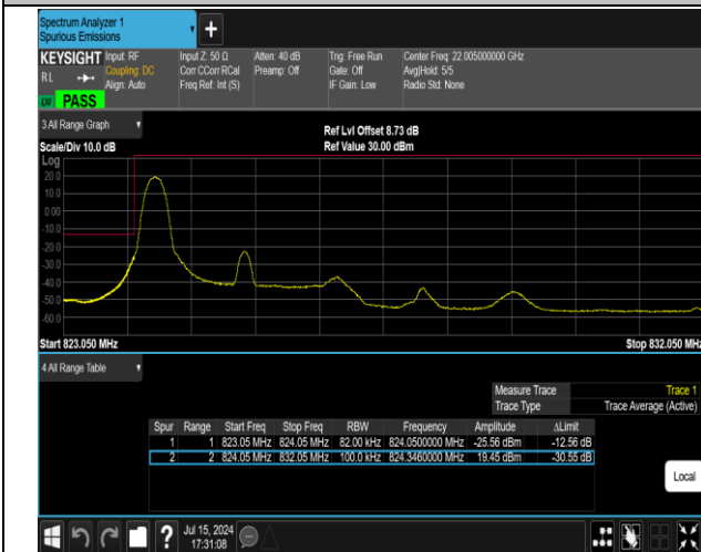
5-5-3MHz-5MHz-16QAM@16QAM-16QAM@16QAM-2041 6-20455-1RB#0@15RB#0-0RB#0@25RB#0-PASS
