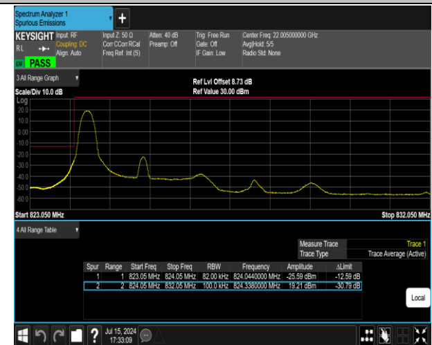
5-5-3MHz-5MHz-16QAM@16QAM-16QAM@16QAM-204 16-20455-1RB#0@15RB#0-1RB#24@25RB#0-PASS
