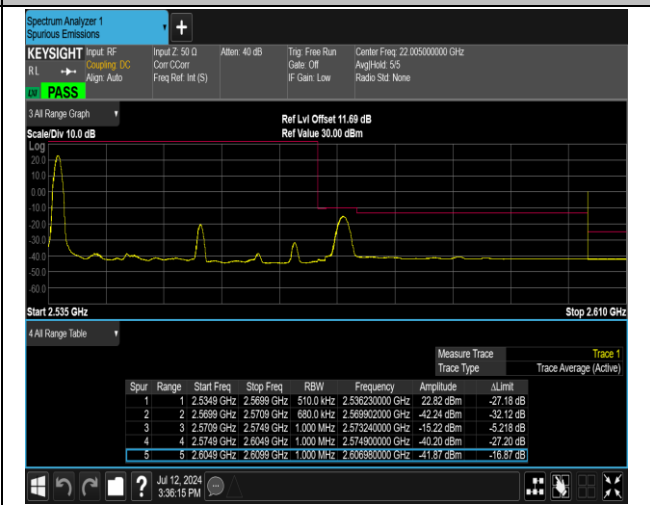
7-7-20MHz-15MHz-16QAM@16QAM-16QAM@16QAM-2 1201-21372-1RB#0@100RB#0-0RB#0@75RB#0-PASS
