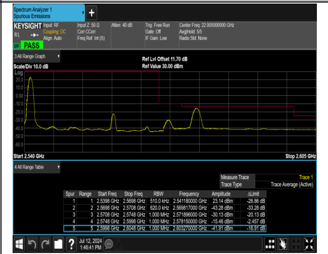
7-7-20MHz-10MHz-16QAM@16QAM-16QAM@16QAM-2 1251-21395-1RB#0@100RB#0-0RB#0@50RB#0-PASS
