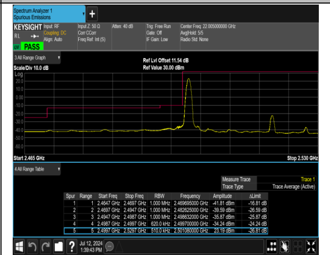
7-7-20MHz-10MHz-QPSK@QPSK-QPSK@QPSK-20850- 20994-1RB#0@100RB#0-0RB#0@50RB#0-PASS
