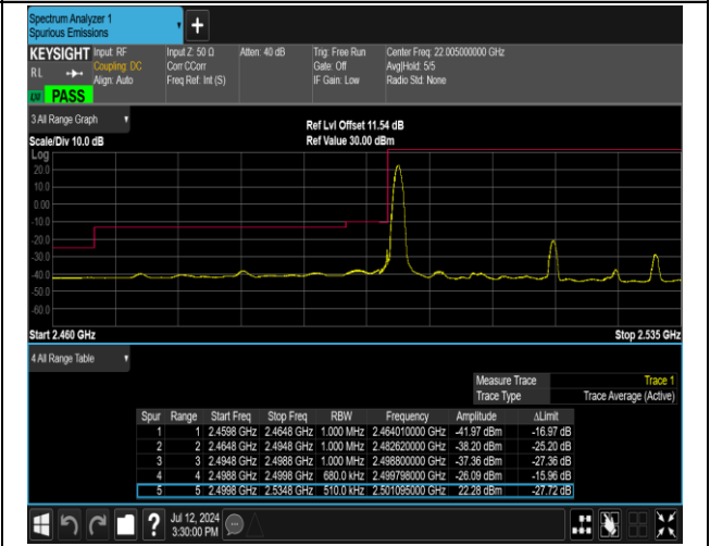
7-7-20MHz-15MHz-16QAM@16QAM-16QAM@16QAM-2 0850-21021-1RB#0@100RB#0-0RB#0@75RB#0-PASS
