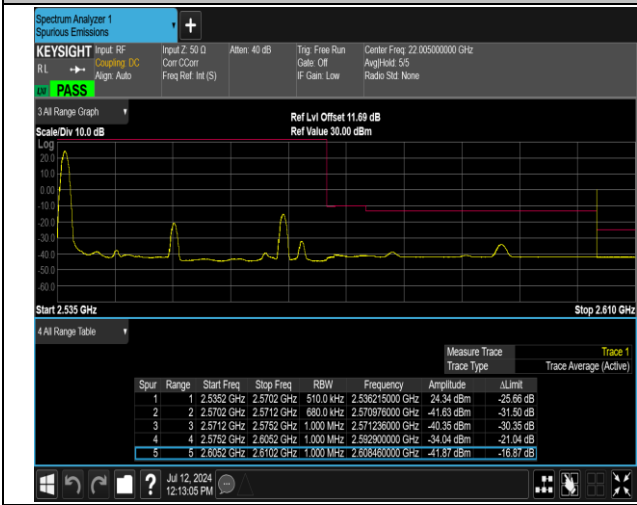
7-7-15MHz-20MHz-QPSK@QPSK-QPSK@QPSK-21179-2 1350-1RB#0@75RB#0-0RB#0@100RB#0-PASS
