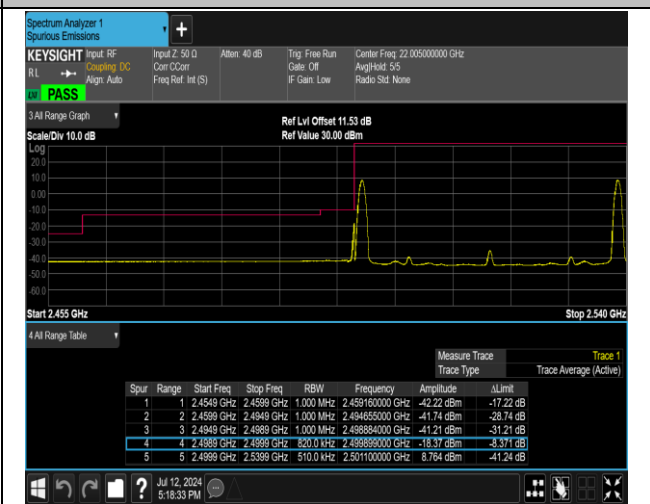
7-7-20MHz-20MHz-16QAM@16QAM-16QAM@16QAM-2 0850-21048-1RB#0@100RB#0-1RB#99@100RB#0-PAS
