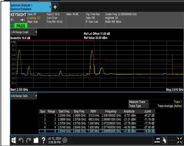
7-7-20MHz-15MHz-QPSK@QPSK-QPSK@QPSK-21201-2 1372-1RB#0@100RB#0-1RB#74@75RB#0-PASS
