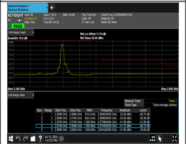
7-7-20MHz-10MHz-QPSK@QPSK-QPSK@QPSK-21251- 21395-1RB#99@100RB#0-0RB#0@50RB#0-PASS
