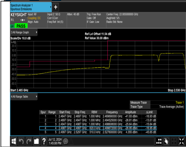
7-7-20MHz-10MHz-16QAM@16QAM-16QAM@16QAM-20 850-20994-100RB#0@100RB#0-50RB#0@50RB#0-PASS
