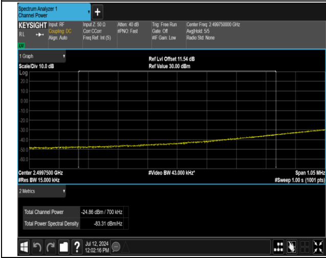
7-7-15MHz-20MHz-QPSK@QPSK-QPSK@QPSK-20828-2 0999-1RB#0@75RB#0-0RB#0@100RB#0-PASS_Final1
