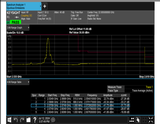
7-7-20MHz-15MHz-16QAM@16QAM-16QAM@16QAM-2 1201-21372-1RB#99@100RB#0-0RB#0@75RB#0-PASS
