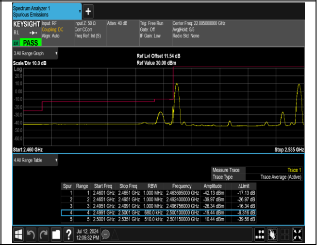
7-7-15MHz-20MHz-QPSK@QPSK-QPSK@QPSK-20828- 20999-1RB#0@75RB#0-1RB#99@100RB#0-PASS
