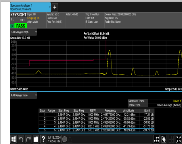
7-7-20MHz-10MHz-QPSK@QPSK-QPSK@QPSK-20850-2 0994-1RB#0@100RB#0-1RB#49@50RB#0-PASS
