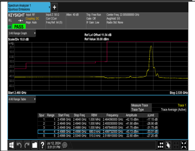
7-7-20MHz-15MHz-16QAM@16QAM-16QAM@16QAM-2 0850-21021-1RB#99@100RB#0-0RB#0@75RB#0-PASS
