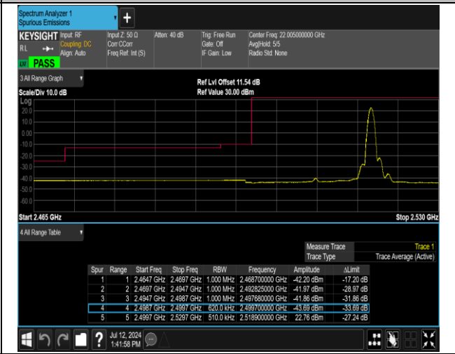
7-7-20MHz-10MHz-16QAM@16QAM-16QAM@16QAM-2 0850-20994-1RB#99@100RB#0-0RB#0@50RB#0-PASS
