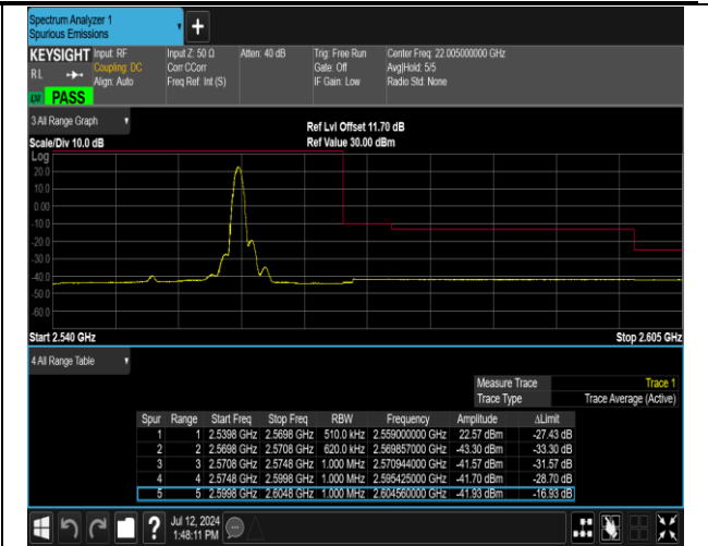
7-7-20MHz-10MHz-16QAM@16QAM-16QAM@16QAM-2 1251-21395-1RB#99@100RB#0-0RB#0@50RB#0-PASS
