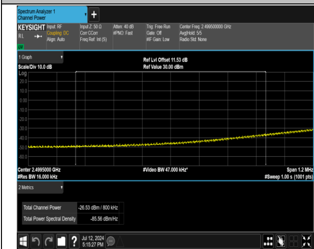
7-7-20MHz-20MHz-16QAM@16QAM-16QAM@16QAM-20 850-21048-1RB#0@100RB#0-0RB#0@100RB#0-PASS_Fi
