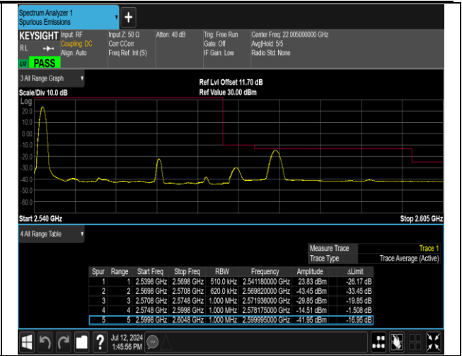
7-7-20MHz-10MHz-QPSK@QPSK-QPSK@QPSK-21251- 21395-1RB#0@100RB#0-0RB#0@50RB#0-PASS
