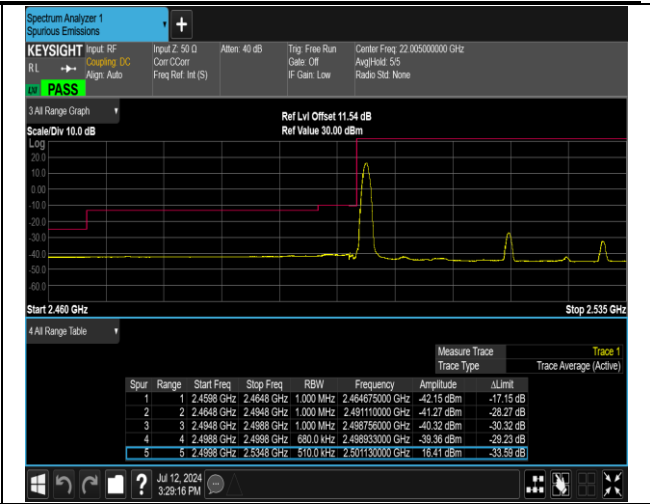
7-7-20MHz-15MHz-QPSK@QPSK-QPSK@QPSK-20850- 21021-1RB#0@100RB#0-0RB#0@75RB#0-PASS
