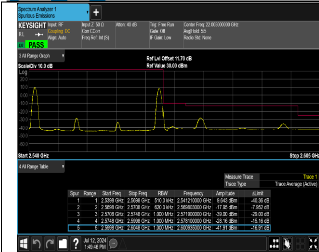
7-7-20MHz-10MHz-16QAM@16QAM-16QAM@16QAM-21 251-21395-1RB#0@100RB#0-1RB#49@50RB#0-PASS
