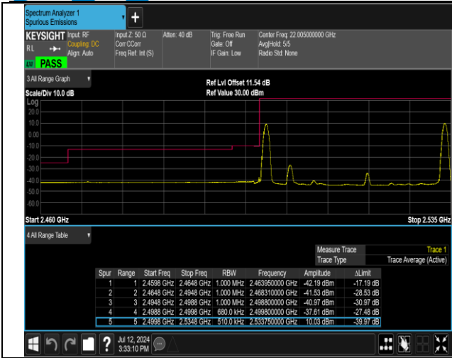
7-7-20MHz-15MHz-16QAM@16QAM-16QAM@16QAM-20 850-21021-1RB#0@100RB#0-1RB#74@75RB#0-PASS
