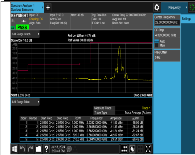
38-38-15MHz-15MHz-QPSK@QPSK-QPSK@QPSK-37825 -37975-1RB#74@75RB#0-0RB#0@75RB#0-PASS
