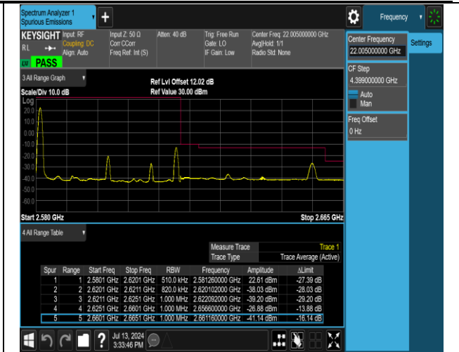
38-38-20MHz-20MHz-16QAM@16QAM-16QAM@16QAM-37952-38150-1RB#0@100RB#0-0RB#0@100RB#0-PAS S
