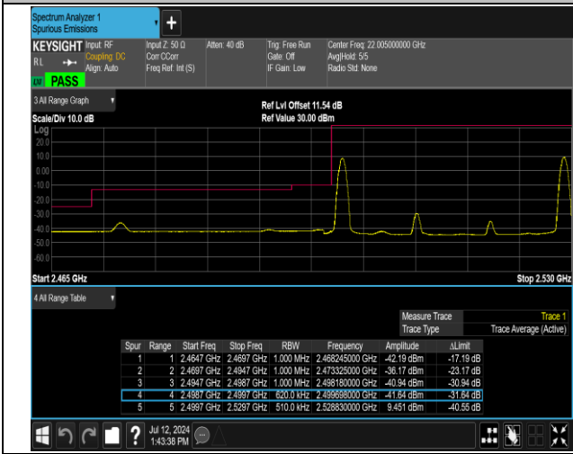
7-7-20MHz-10MHz-16QAM@16QAM-16QAM@16QAM-20 850-20994-1RB#0@100RB#0-1RB#49@50RB#0-PASS
