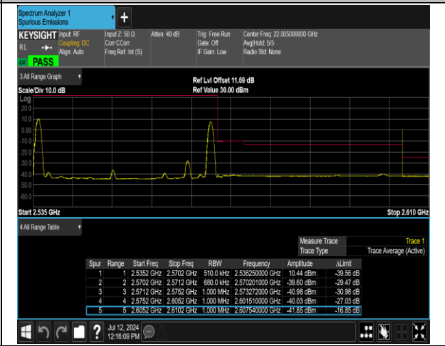
7-7-15MHz-20MHz-QPSK@QPSK-QPSK@QPSK-21179- 21350-1RB#0@75RB#0-1RB#99@100RB#0-PASS
