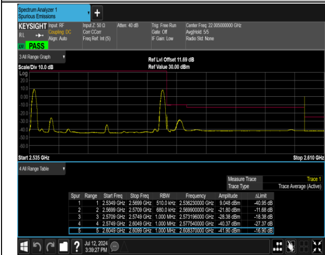
7-7-20MHz-15MHz-16QAM@16QAM-16QAM@16QAM-21 201-21372-1RB#0@100RB#0-1RB#74@75RB#0-PASS
