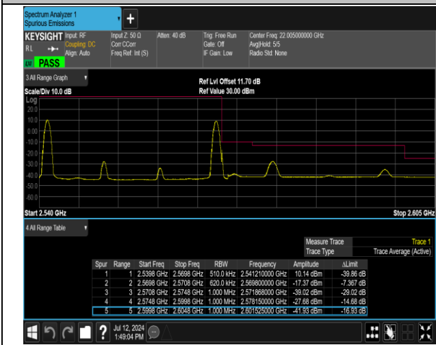
7-7-20MHz-10MHz-QPSK@QPSK-QPSK@QPSK-21251-2 1395-1RB#0@100RB#0-1RB#49@50RB#0-PASS
