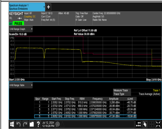
7-7-15MHz-20MHz-16QAM@16QAM-16QAM@16QAM-21 179-21350-75RB#0@75RB#0-100RB#0@100RB#0-PASS
