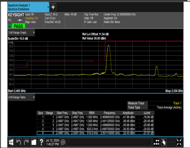
7-7-20MHz-10MHz-16QAM@16QAM-16QAM@16QAM-2 0850-20994-1RB#0@100RB#0-0RB#0@50RB#0-PASS
