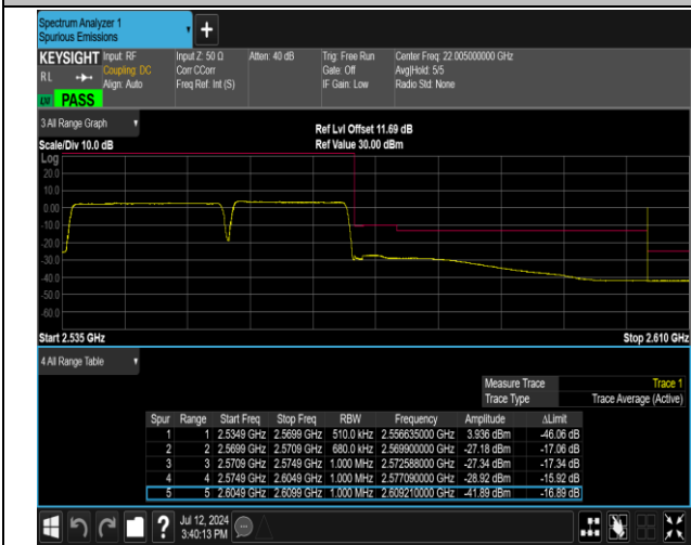
7-7-20MHz-15MHz-QPSK@QPSK-QPSK@QPSK-21201-2 1372-100RB#0@100RB#0-75RB#0@75RB#0-PASS
