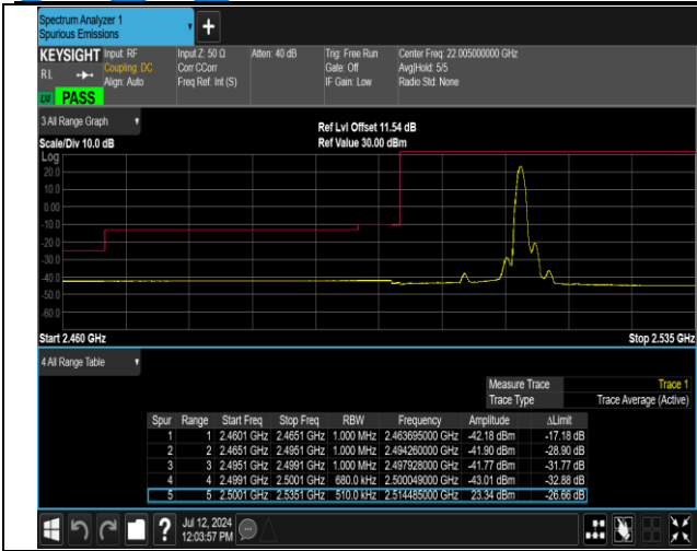
7-7-15MHz-20MHz-QPSK@QPSK-QPSK@QPSK-20828-2 0999-1RB#74@75RB#0-0RB#0@100RB#0-PASS
