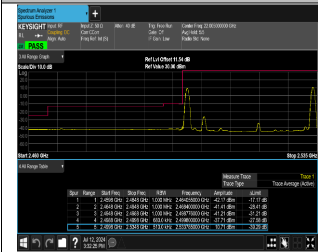
7-7-20MHz-15MHz-QPSK@QPSK-QPSK@QPSK-20850-2 1021-1RB#0@100RB#0-1RB#74@75RB#0-PASS
