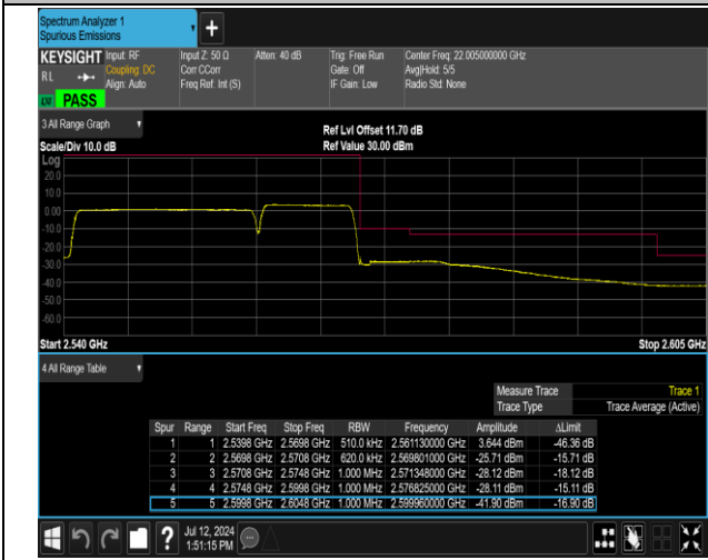
7-7-20MHz-10MHz-16QAM@16QAM-16QAM@16QAM-21 251-21395-100RB#0@100RB#0-50RB#0@50RB#0-PASS
