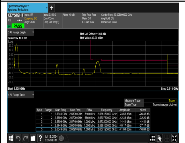
7-7-20MHz-15MHz-QPSK@QPSK-QPSK@QPSK-21201- 21372-1RB#0@100RB#0-0RB#0@75RB#0-PASS
