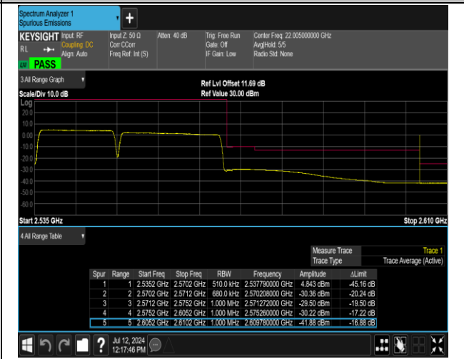
7-7-15MHz-20MHz-QPSK@QPSK-QPSK@QPSK-21179- 21350-75RB#0@75RB#0-100RB#0@100RB#0-PASS
