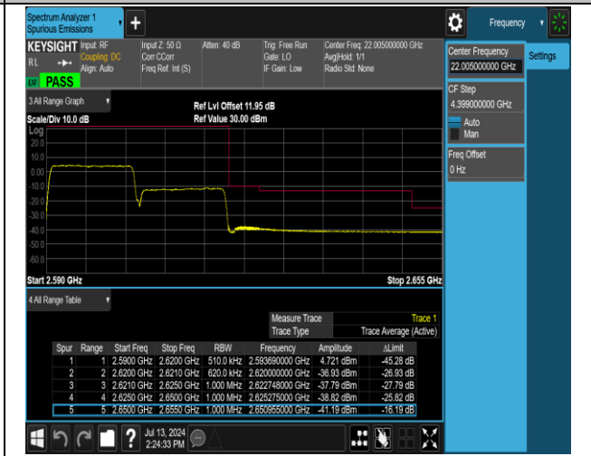
38-38-15MHz-15MHz-QPSK@QPSK-QPSK@QPSK-380 25-38175-75RB#0@75RB#0-75RB#0@75RB#0-PASS
