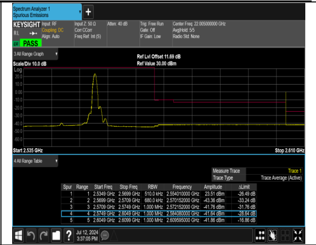
7-7-20MHz-15MHz-QPSK@QPSK-QPSK@QPSK-21201- 21372-1RB#99@100RB#0-0RB#0@75RB#0-PASS
