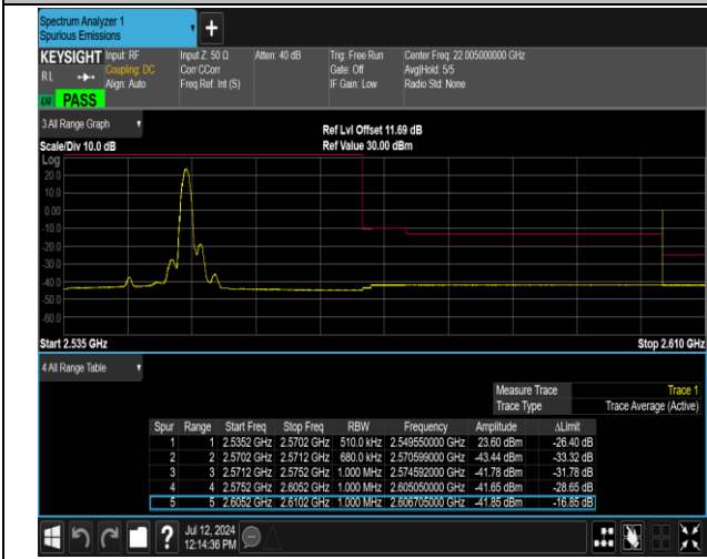
7-7-15MHz-20MHz-QPSK@QPSK-QPSK@QPSK-21179-2 1350-1RB#74@75RB#0-0RB#0@100RB#0-PASS
