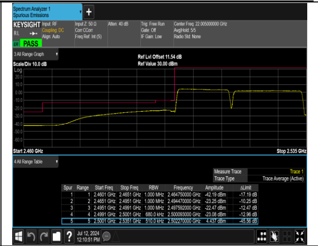
7-7-15MHz-20MHz-QPSK@QPSK-QPSK@QPSK-20828- 20999-75RB#0@75RB#0-100RB#0@100RB#0-PASS
