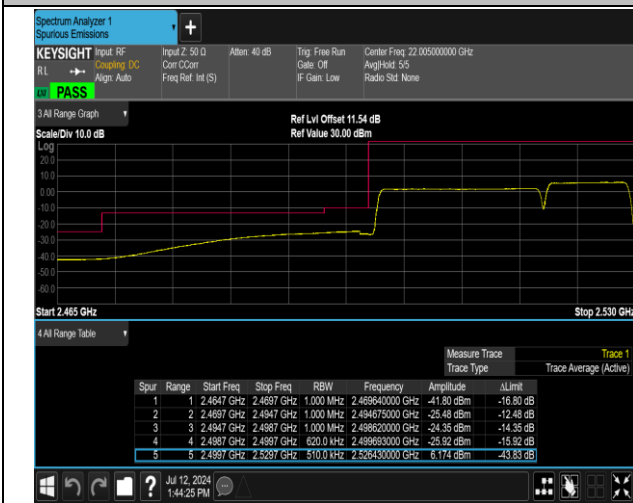
7-7-20MHz-10MHz-QPSK@QPSK-QPSK@QPSK-20850-2 0994-100RB#0@100RB#0-50RB#0@50RB#0-PASS
