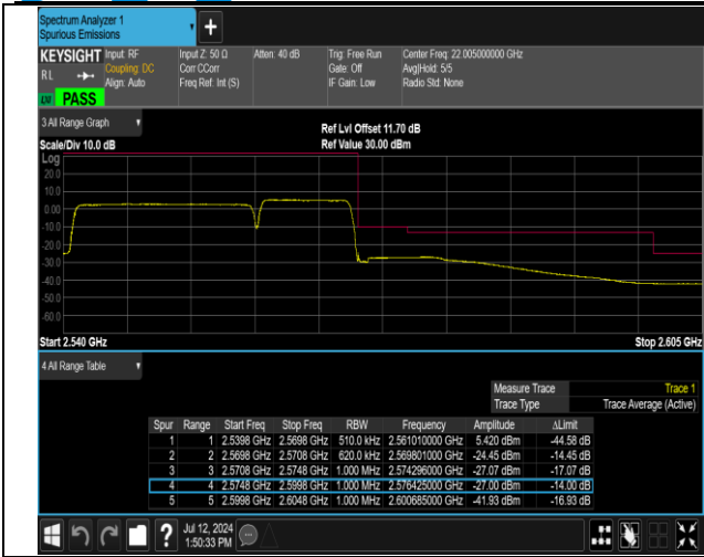
7-7-20MHz-10MHz-QPSK@QPSK-QPSK@QPSK-21251-2 1395-100RB#0@100RB#0-50RB#0@50RB#0-PASS
