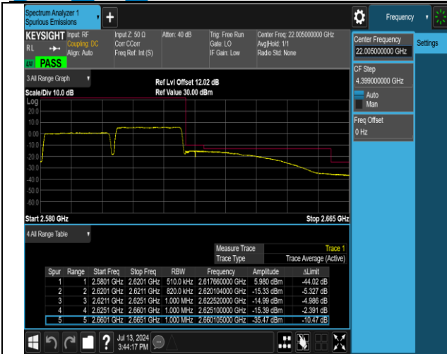
38-38-20MHz-20MHz-16QAM@16QAM-16QAM@16QAM-37952-38150-100RB#0@100RB#0-100RB#0@100RB#0-P ASS
