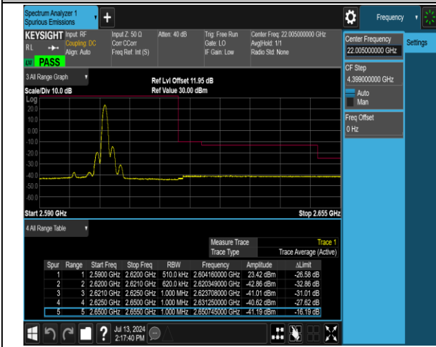
38-38-15MHz-15MHz-QPSK@QPSK-QPSK@QPSK-38025 -38175-1RB#74@75RB#0-0RB#0@75RB#0-PASS
