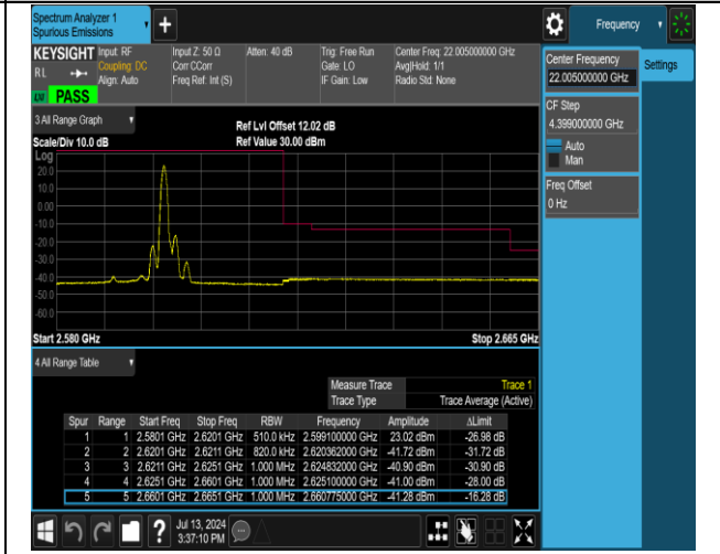
38-38-20MHz-20MHz-16QAM@16QAM-16QAM@16QAM-37952-38150-1RB#99@100RB#0-0RB#0@100RB#0-PA SS
