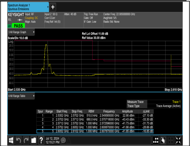
7-7-15MHz-20MHz-16QAM@16QAM-16QAM@16QAM-2 1179-21350-1RB#74@75RB#0-0RB#0@100RB#0-PASS
