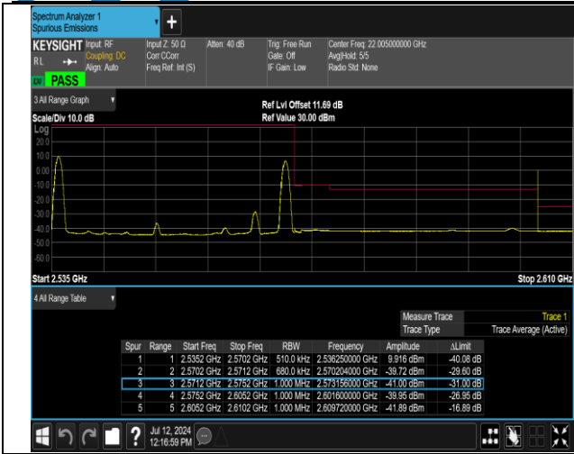
7-7-15MHz-20MHz-16QAM@16QAM-16QAM@16QAM-21 179-21350-1RB#0@75RB#0-1RB#99@100RB#0-PASS
