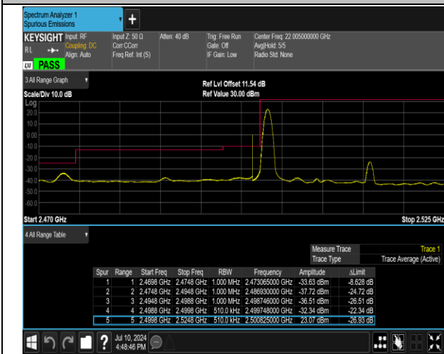
7-7-15MHz-10MHz-16QAM@16QAM-16QAM@16QAM-20 825-20945-1RB#0@75RB#0-0RB#0@50RB#0-PASS
