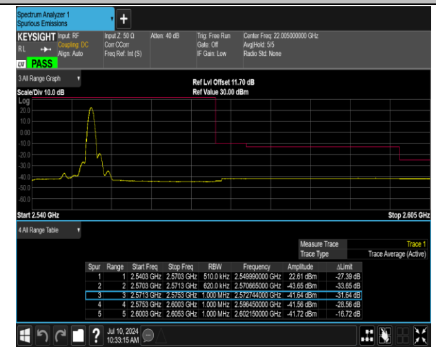
7-7-10MHz-20MHz-16QAM@16QAM-16QAM@16QAM-2 1206-21350-1RB#49@50RB#0-0RB#0@100RB#0-PASS
