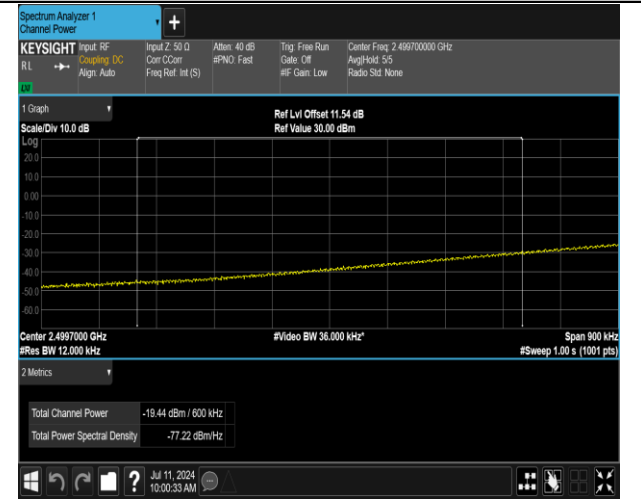
7-7-15MHz-15MHz-QPSK@QPSK-QPSK@QPSK-20825-20975-1RB#0@75RB#0-0RB#0@75RB#0-PASS_Final1
