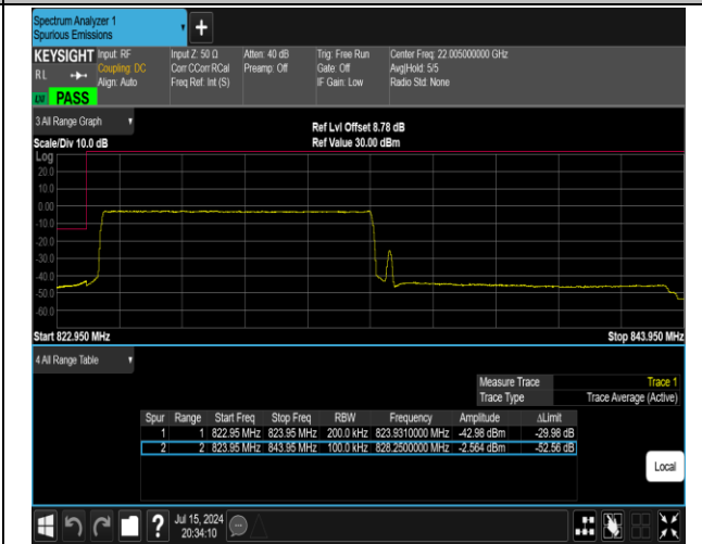
5-5-10MHz-10MHz-QPSK@QPSK-QPSK@QPSK-20450- 20549-50RB#0@50RB#0-50RB#0@50RB#0-PASS
