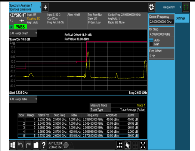
38-38-15MHz-15MHz-16QAM@16QAM-16QAM@16QAM-37825-37975-1RB#0@75RB#0-1RB#74@75RB#0-PASS
