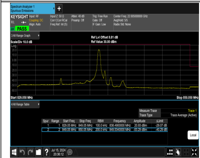
5-5-10MHz-10MHz-QPSK@QPSK-QPSK@QPSK-20501-2 0600-1RB#49@50RB#0-0RB#0@50RB#0-PASS
