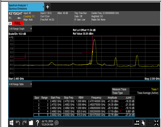
7-7-10MHz-20MHz-16QAM@16QAM-16QAM@16QAM-20 805-20949-1RB#0@50RB#0-0RB#0@100RB#0
