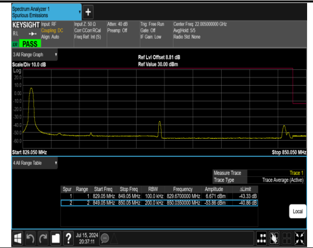
5-5-10MHz-10MHz-QPSK@QPSK-QPSK@QPSK-20501- 20600-1RB#0@50RB#0-1RB#49@50RB#0-PASS
