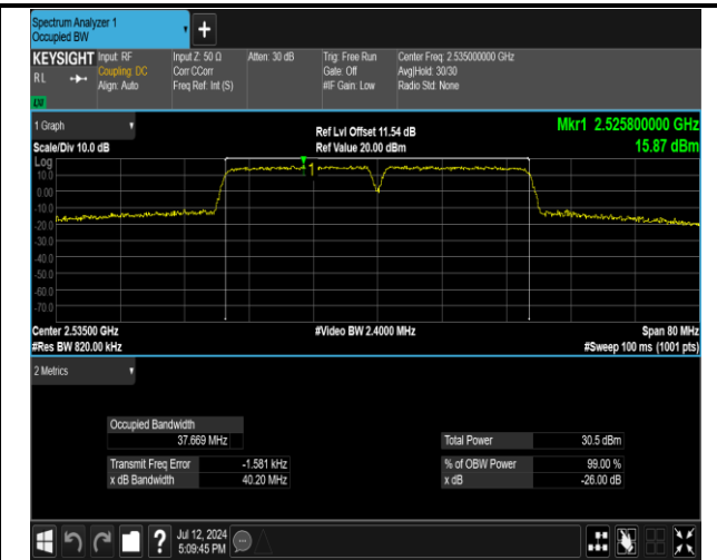
7-7-20MHz-20MHz-16QAM-16QAM-21001-21199-100RB# 0-100RB#0-PASS
