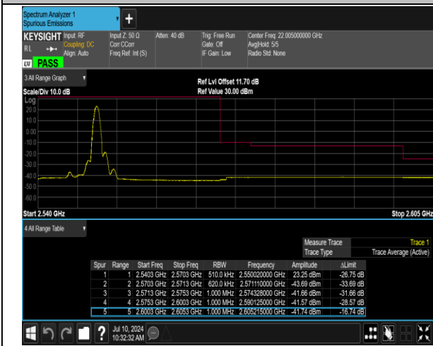
7-7-10MHz-20MHz-QPSK@QPSK-QPSK@QPSK-21206-2 1350-1RB#49@50RB#0-0RB#0@100RB#0-PASS
