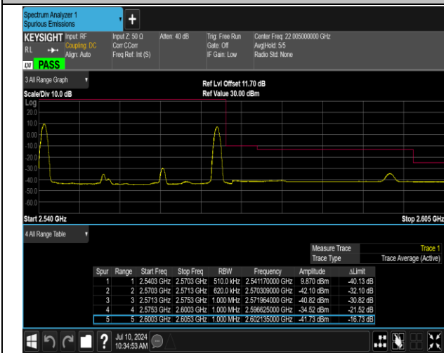
7-7-10MHz-20MHz-16QAM@16QAM-16QAM@16QAM-21 206-21350-1RB#0@50RB#0-1RB#99@100RB#0-PASS
