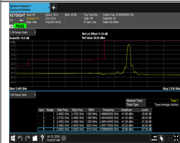
7-7-10MHz-20MHz-QPSK@QPSK-QPSK@QPSK-20805-2 0949-1RB#49@50RB#0-0RB#0@100RB#0-PASS
