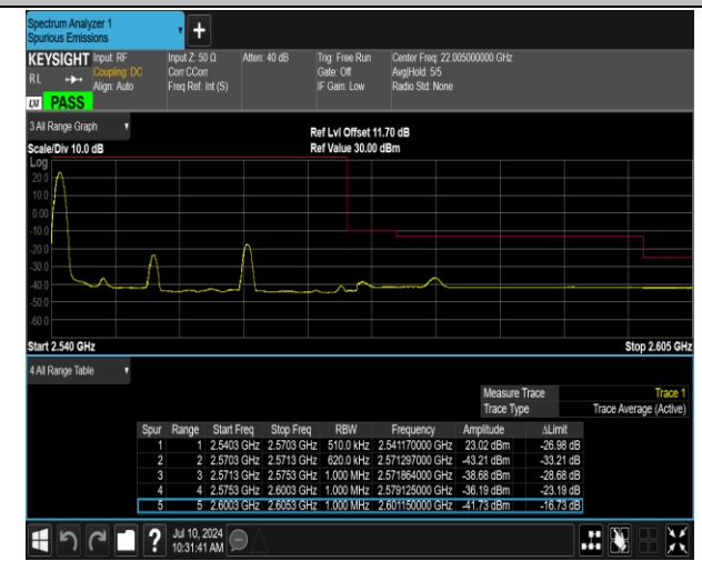
7-7-10MHz-20MHz-16QAM@16QAM-16QAM@16QAM-2 1206-21350-1RB#0@50RB#0-0RB#0@100RB#0-PASS
