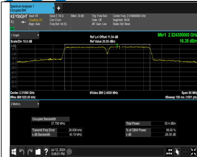
7-7-20MHz-20MHz-16QAM-16QAM-20850-21048-100RB# 0-100RB#0-PASS
