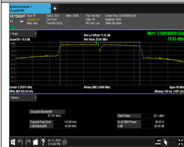
7-7-20MHz-20MHz-16QAM-16QAM-21152-21350-100RB# 0-100RB#0-PASS
