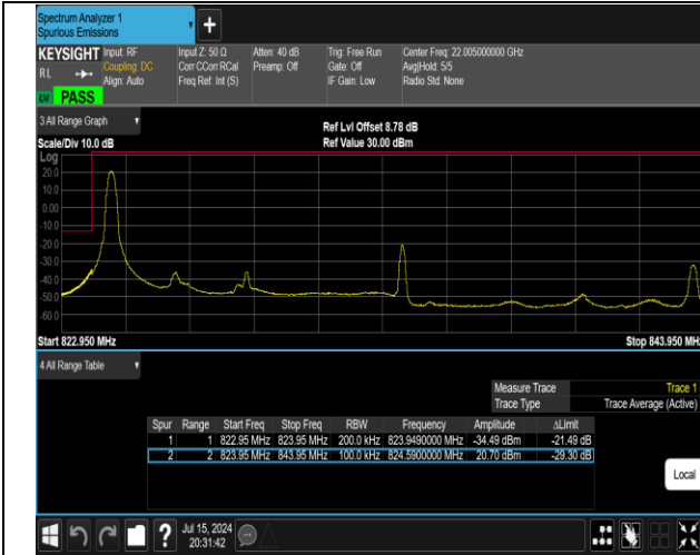
5-5-10MHz-10MHz-16QAM@ 16QAM-16QAM@ 16QAM-20 450-20549-1RB#0@50RB#0-0RB#0@50RB#0-PASS
