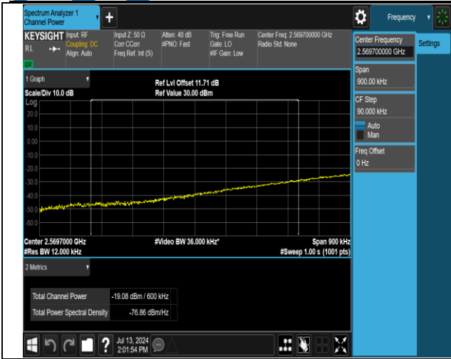
38-38-15MHz-15MHz-16QAM@16QAM-16QAM@16QAM-37825-37975-1RB#0@75RB#0-0RB#0@75RB#0-PASS_Fi nal1
