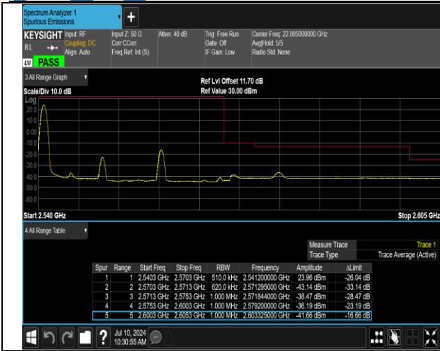
7-7-10MHz-20MHz-QPSK@QPSK-QPSK@QPSK-21206-2 1350-1RB#0@50RB#0-0RB#0@100RB#0-PASS
