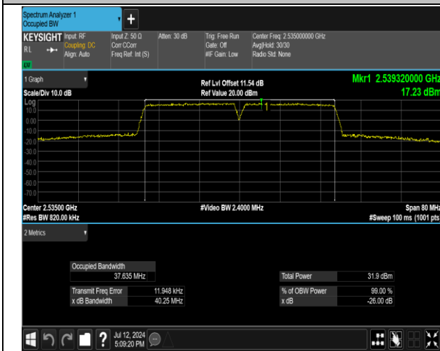
7-7-20MHz-20MHz-QPSK-QPSK-21001-21199-100RB#0- 100RB#0-PASS
