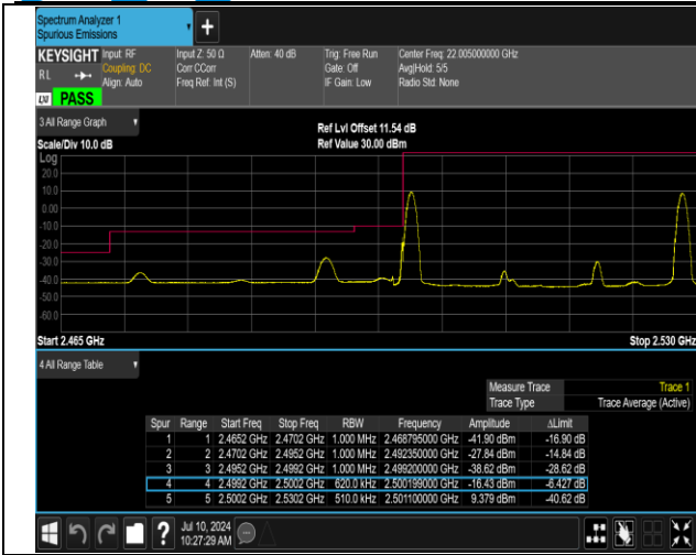
7-7-10MHz-20MHz-16QAM@16QAM-16QAM@16QAM-20 805-20949-1RB#0@50RB#0-1RB#99@100RB#0-PASS
