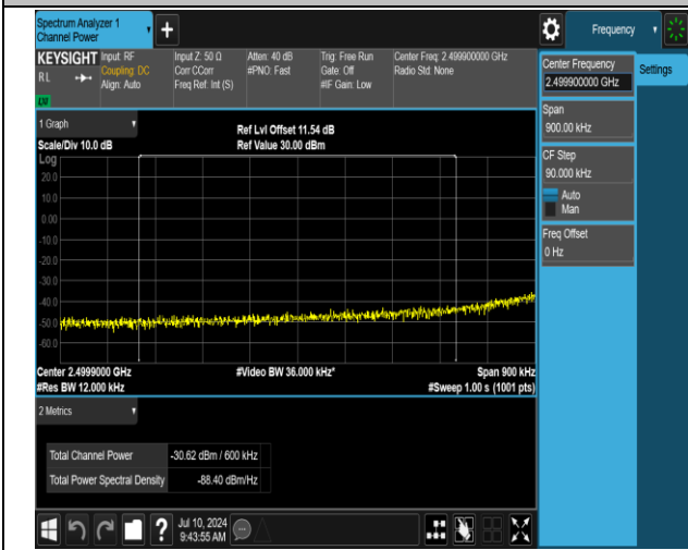
7-7-10MHz-20MHz-QPSK@QPSK-QPSK@QPSK-20805-2 0949-1RB#0@50RB#0-0RB#0@100RB#0-PASS_Final1
