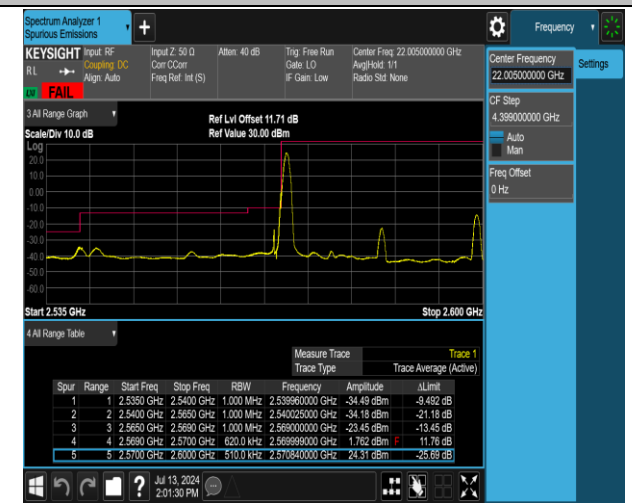
38-38-15MHz-15MHz-16QAM@16QAM-16QAM@16QAM -37825-37975-1RB#0@75RB#0-0RB#0@75RB#0-pass
