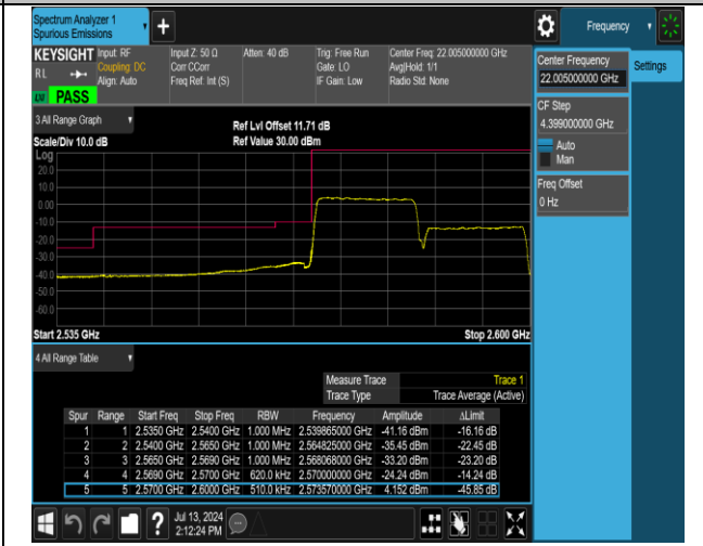
38-38-15MHz-15MHz-16QAM@16QAM-16QAM@16QAM-37825-37975-75RB#0@75RB#0-75RB#0-PAS S
