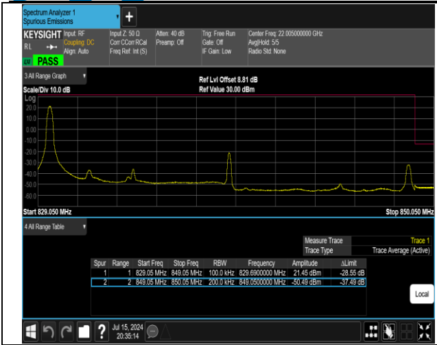
5-5-10MHz-10MHz-QPSK@QPSK-QPSK@QPSK-20501-2 0600-1RB#0@50RB#0-0RB#0@50RB#0-PASS
