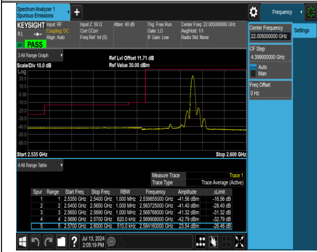
38-38-15MHz-15MHz-16QAM@16QAM-16QAM@16QAM-37825-37975-1RB#74@75RB#0-0RB#0@75RB#0-PASS
