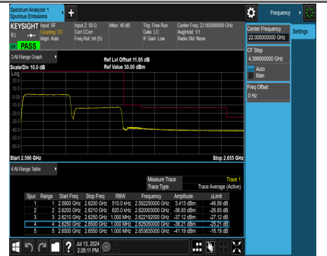
38-38-15MHz-15MHz-16QAM@16QAM-16QAM@16QAM-38025-38175-75RB#0@75RB#0-75RB#0@75RB#0-PASS
