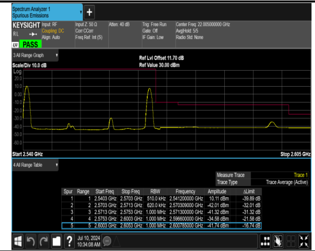
7-7-10MHz-20MHz-QPSK@QPSK-QPSK@QPSK-21206- 21350-1RB#0@50RB#0-1RB#99@100RB#0-PASS
