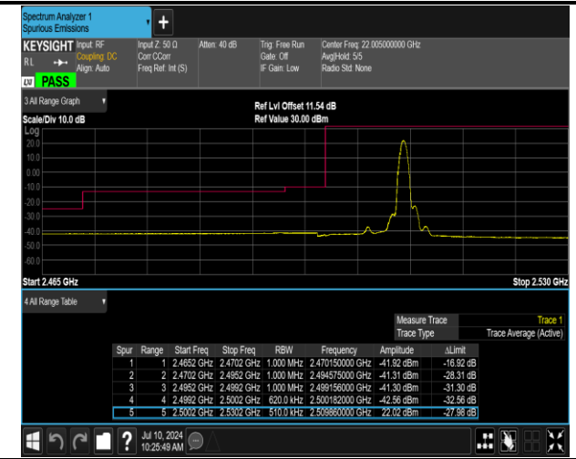
7-7-10MHz-20MHz-16QAM@16QAM-16QAM@16QAM-2 0805-20949-1RB#49@50RB#0-0RB#0@100RB#0-PASS
