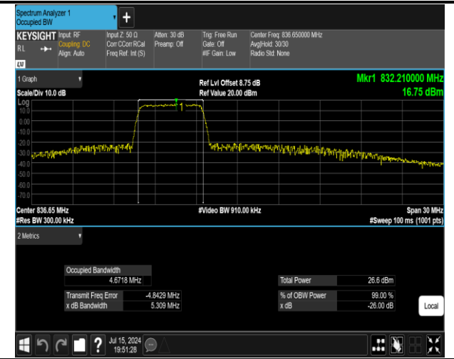
5-5-5MHz-10MHz-16QAM-16QAM-20478-20550-25RB#0-50RB#0-PASS
