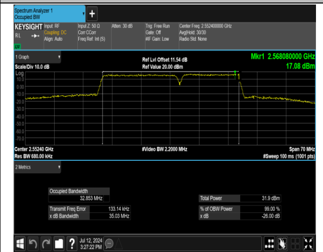
7-7-20MHz-15MHz-QPSK-QPSK-21201-21372-100RB#0-75RB#0-PASS
