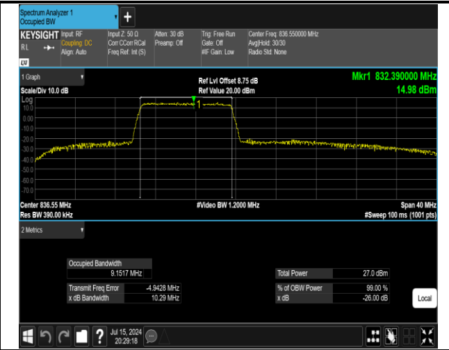
5-5-10MHz-10MHz-16QAM-16QAM-20476-20575-50RB#0 -50RB#0-PASS
