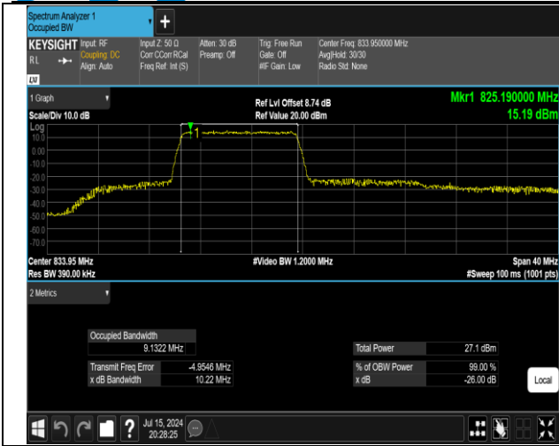
5-5-10MHz-10MHz-16QAM-16QAM-20450-20549-50RB#0 -50RB#0-PASS
