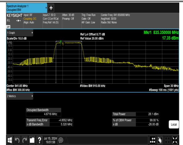
5-5-5MHz-10MHz-QPSK-QPSK-20528-20600-25RB#0-50RB#0-PASS
