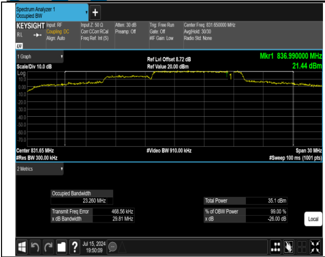
5-5-5MHz-10MHz-16QAM-16QAM-20428-20500-25RB#0-50RB#0-PASS
