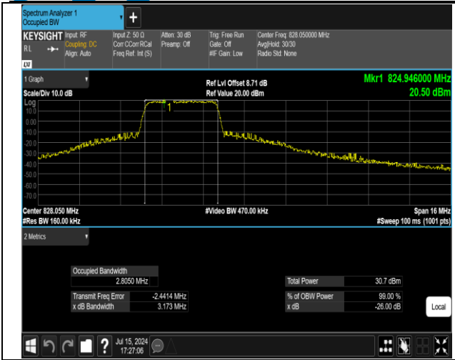
5-5-3MHz-5MHz-16QAM-16QAM-20416-20455-15RB#0-2 5RB#0-PASS
