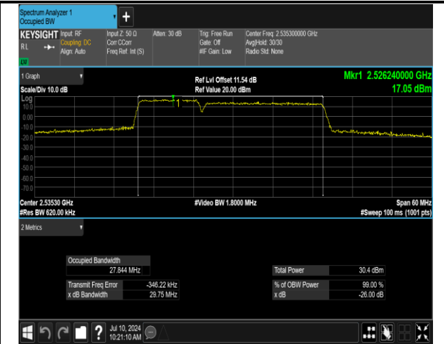
7-7-10MHz-20MHz-16QAM-16QAM-21006-21150-50RB#0 -100RB#0-PASS
