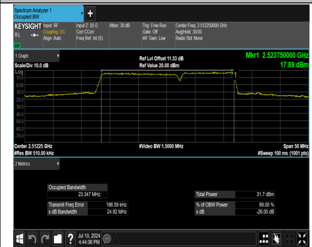
7-7-15MHz-10MHz-QPSK-QPSK-20825-20945-75RB#0-5 0RB#0-PASS
