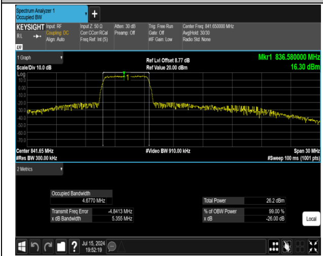
5-5-5MHz-10MHz-16QAM-16QAM-20528-20600-25RB#0-50RB#0-PASS
