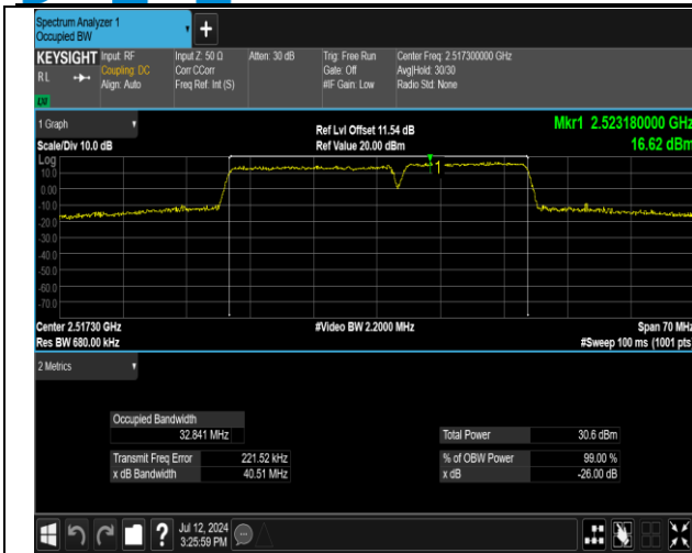
7-7-20MHz-15MHz-16QAM-16QAM-20850-21021-100RB# 0-75RB#0-PASS
