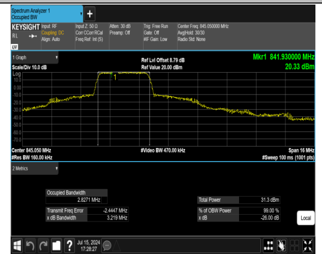
5-5-3MHz-5MHz-QPSK-QPSK-20586-20625-15RB#0-25R B#0-PASS
