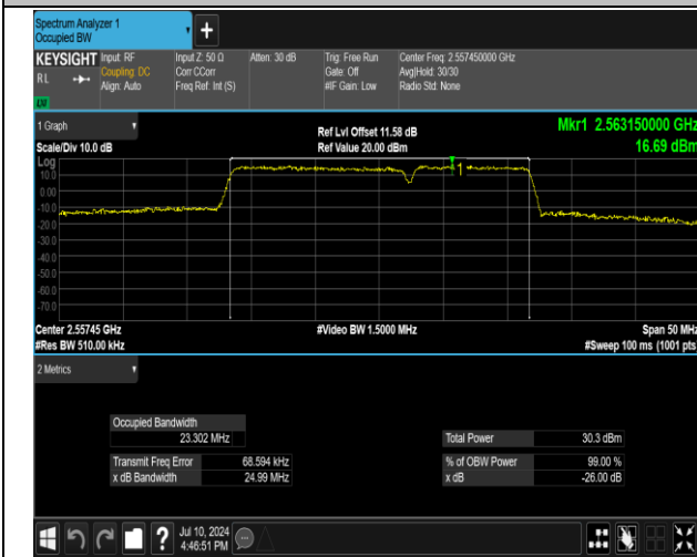
7-7-15MHz-10MHz-16QAM-16QAM-21277-21397-75RB#0 -50RB#0-PASS
