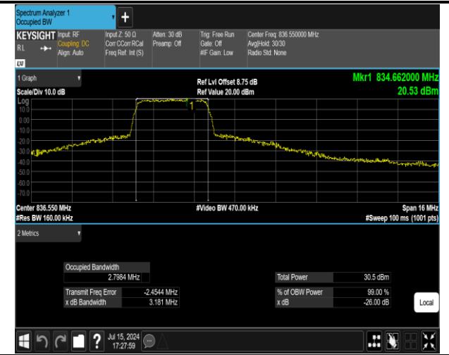
5-5-3MHz-5MHz-16QAM-16QAM-20501-20540-15RB#0-2 5RB#0-PASS
