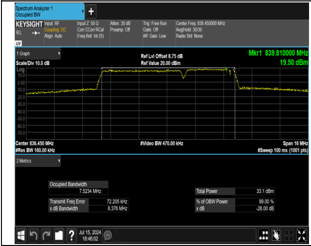
5-5-5MHz-3MHz-QPSK-QPSK-20510-20549-25RB#0-15R B#0-PASS
