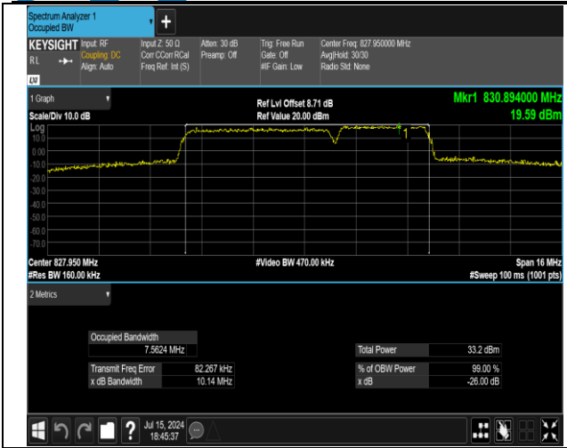
5-5-5MHz-3MHz-16QAM-16QAM-20425-20464-25RB#0-1 5RB#0-PASS
