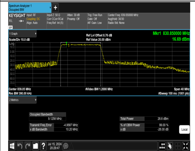
5-5-10MHz-10MHz-QPSK-QPSK-20501-20600-50RB#0-5 0RB#0-PASS
