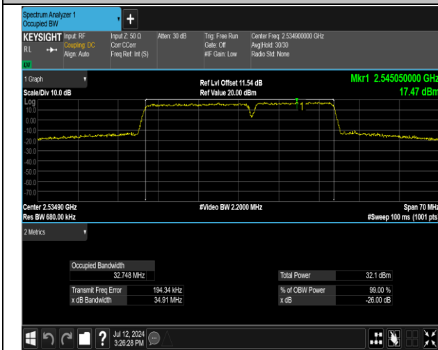
7-7-20MHz-15MHz-QPSK-QPSK-21026-21197-100RB#0-75RB#0-PASS
