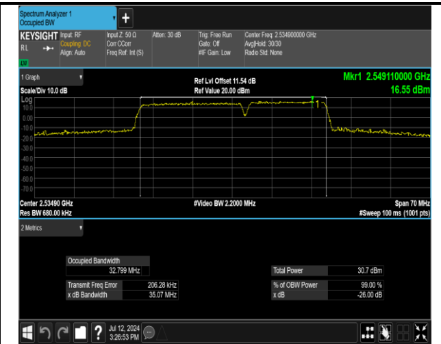
7-7-20MHz-15MHz-16QAM-16QAM-21026-21197-100RB# 0-75RB#0-PASS
