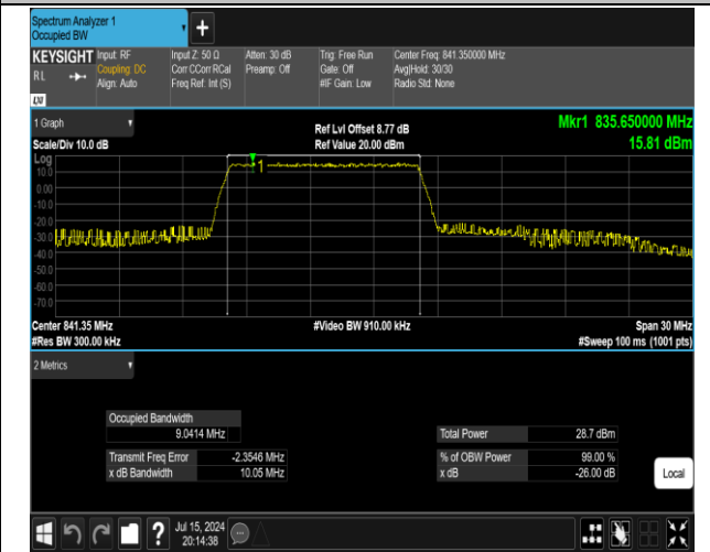
5-5-10MHz-5MHz-QPSK-QPSK-20550-20622-50RB#0-25RB#0-PASS
