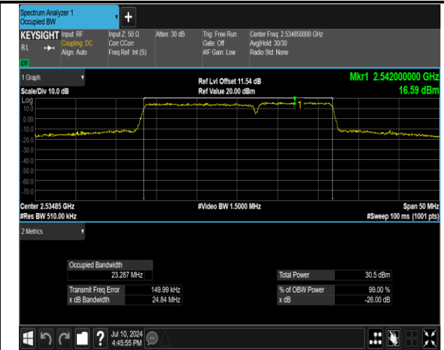
7-7-15MHz-10MHz-16QAM-16QAM-21051-21171-75RB#0 -50RB#0-PASS
