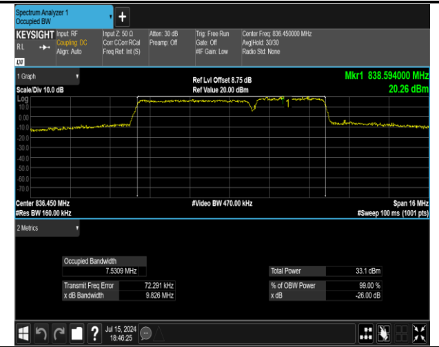
5-5-5MHz-3MHz-16QAM-16QAM-20510-20549-25RB#0-1 5RB#0-PASS
