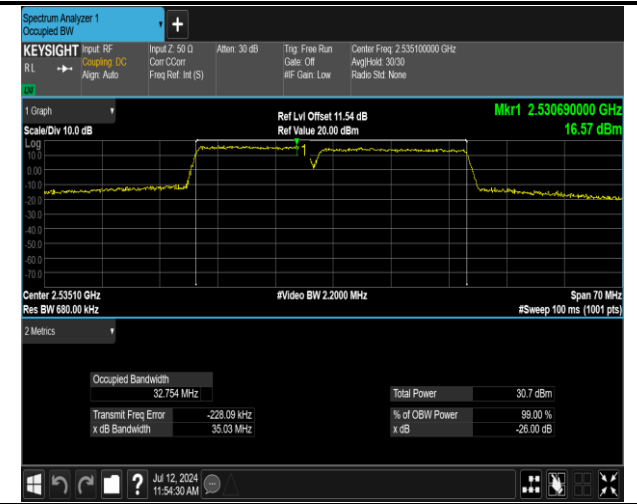
7-7-15MHz-20MHz-16QAM-16QAM-21003-21174-75RB#0 -100RB#0-PASS
