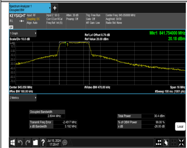
5-5-3MHz-5MHz-16QAM-16QAM-20586-20625-15RB#0-2 5RB#0-PASS
