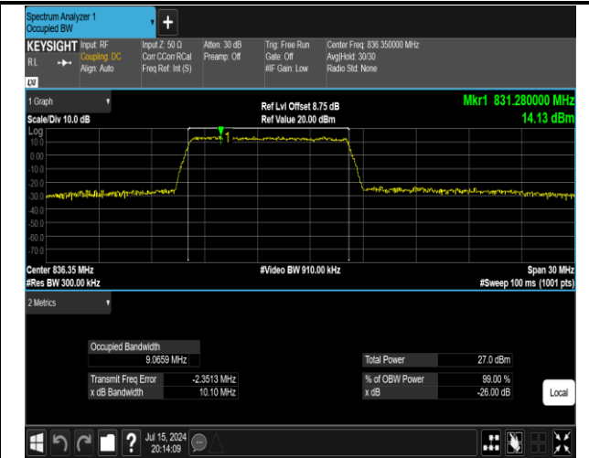
5-5-10MHz-5MHz-16QAM-16QAM-20500-20572-50RB#0-25RB#0-PASS
