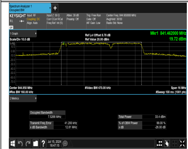
5-5-5MHz-3MHz-16QAM-16QAM-20595-20634-25RB#0-1 5RB#0-PASS
