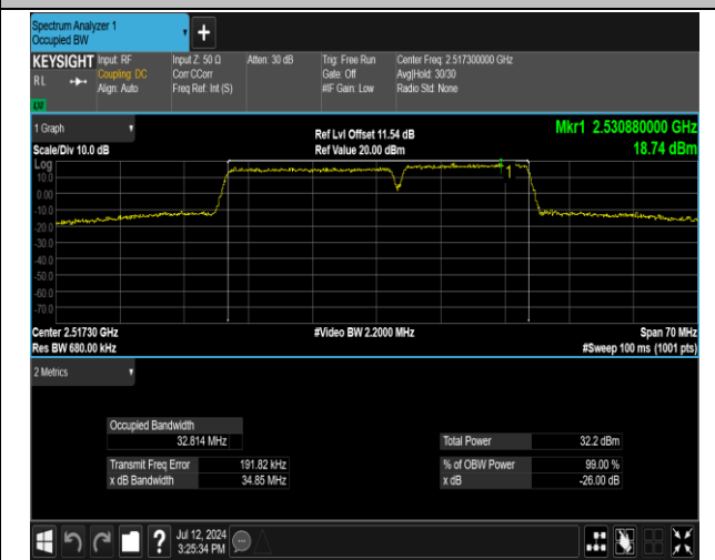
7-7-20MHz-15MHz-QPSK-QPSK-20850-21021-100RB#0-75RB#0-PASS
