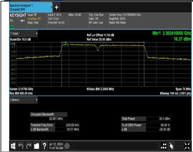
7-7-15MHz-20MHz-16QAM-16QAM-20828-20999-75RB#0 -100RB#0-PASS
