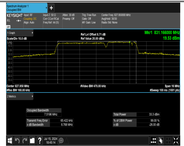
5-5-5MHz-3MHz-QPSK-QPSK-20425-20464-25RB#0-15R B#0-PASS
