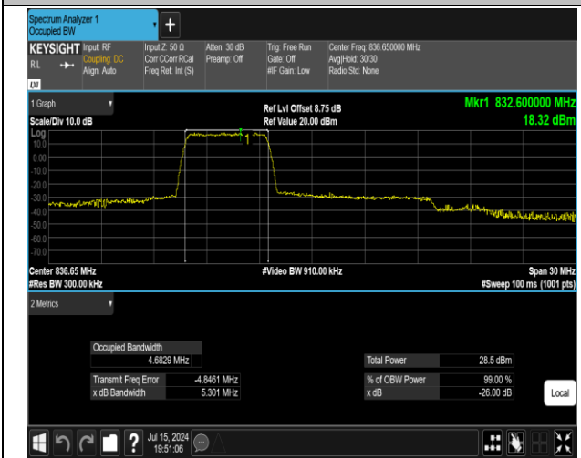
5-5-5MHz-10MHz-QPSK-QPSK-20478-20550-25RB#0-50RB#0-PASS
