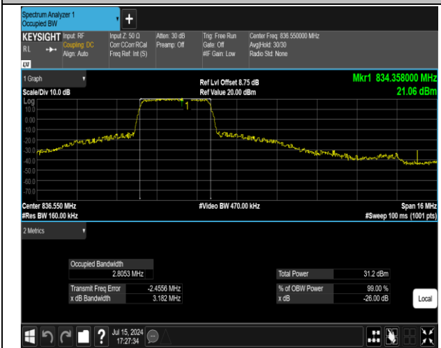
5-5-3MHz-5MHz-QPSK-QPSK-20501-20540-15RB#0-25R B#0-PASS
