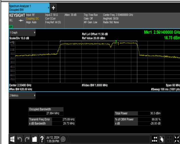
7-7-20MHz-10MHz-16QAM-16QAM-21251-21395-100RB# 0-50RB#0-PASS
