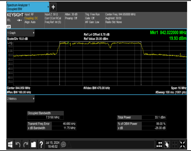
5-5-5MHz-3MHz-QPSK-QPSK-20595-20634-25RB#0-15R B#0-PASS
