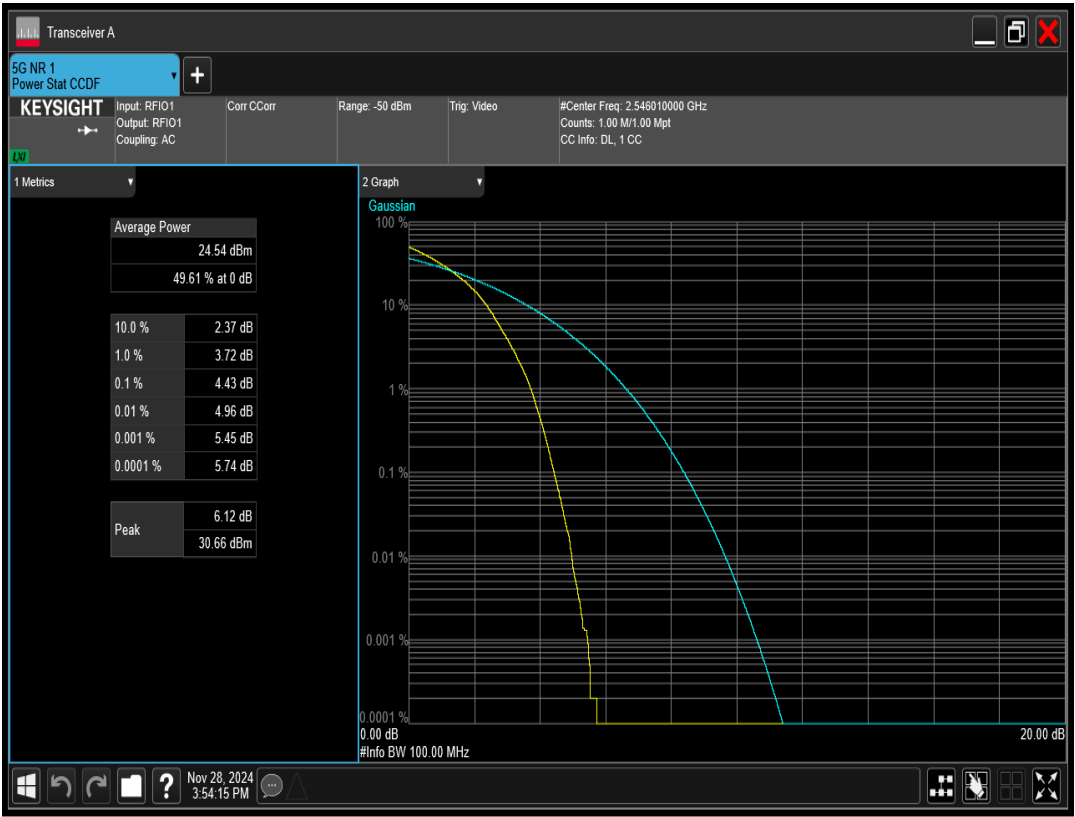
n41 SCS=30kHz DFT_BPSK BW=100MHz Channel=509202 RB=270@0
