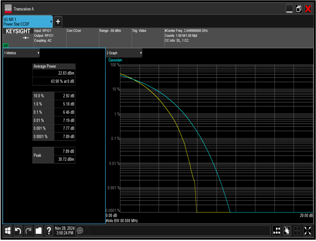
n41 SCS=30kHz DFT_QAM64 BW=80MHz Channel=529998 RB=216@0
