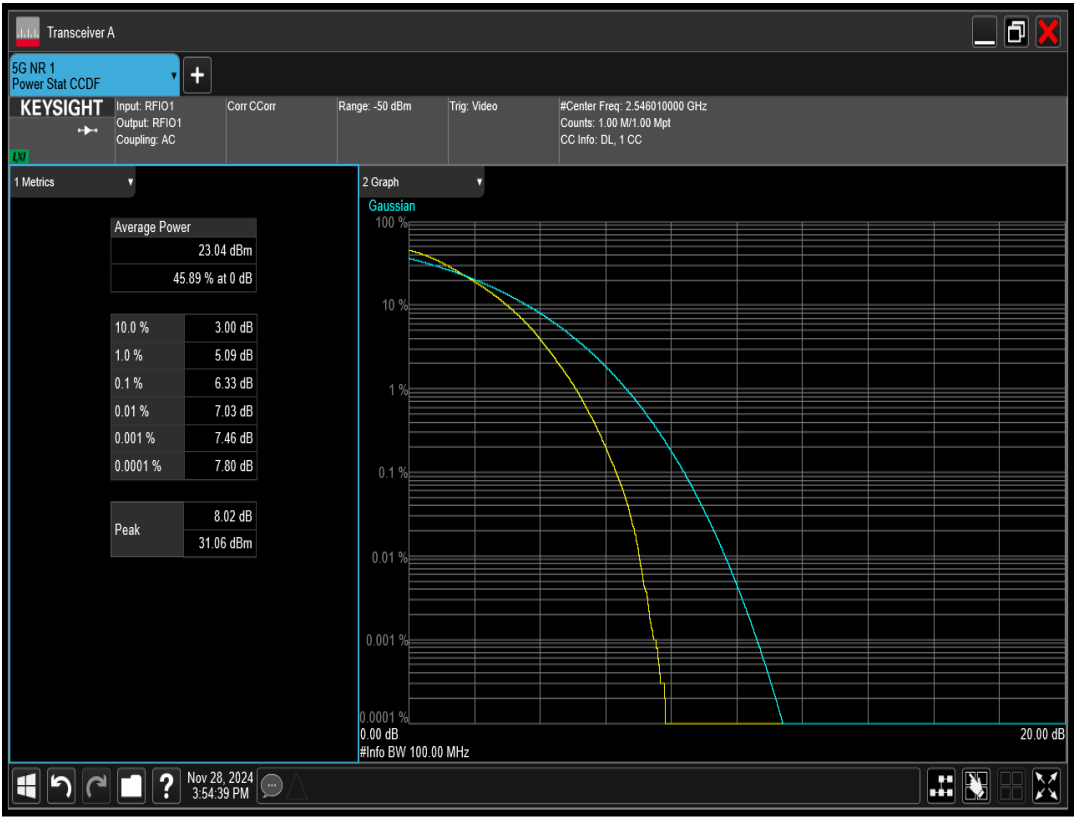
n41 SCS=30kHz DFT_QAM16 BW=100MHz Channel=509202 RB=270@0
