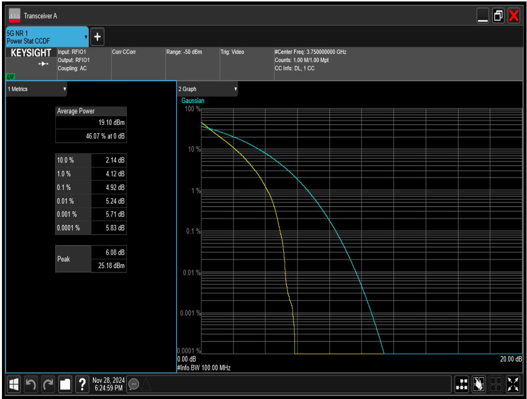
n77 SCS=30kHz DFT_BPSK BW=100MHz Channel=650000 RB=270@0
