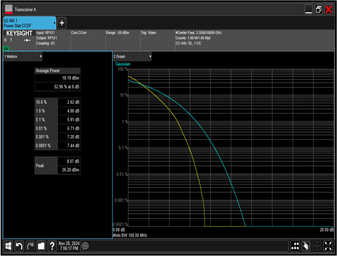
n78 SCS=30kHz DFT_QPSK BW=100MHz Channel=623334 RB=270@0
