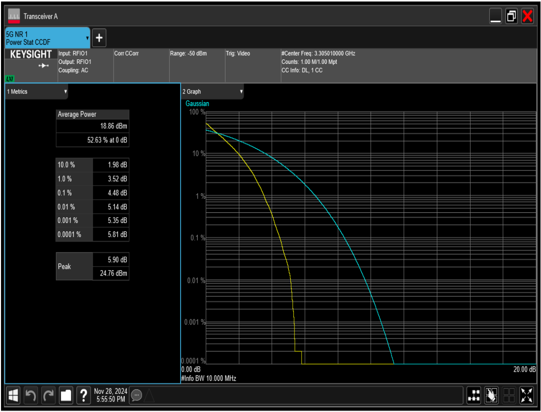
n77 SCS=30kHz DFT_BPSK BW=10MHz Channel=620334 RB=24@0
